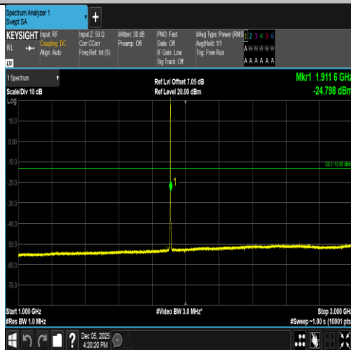
Band2-1.4MHz-QPSK-19193-1RB#5-1000~3000-PASS
