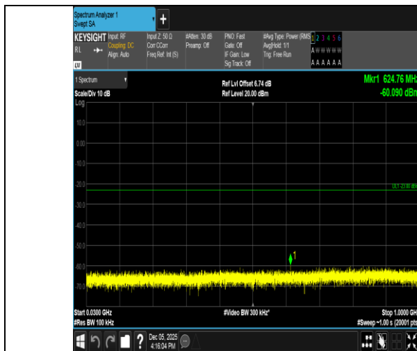
Band2-1.4MHz-QPSK-18900-6RB#0-30~1000-PASS
