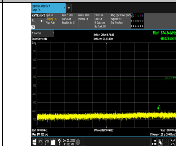
Band2-1.4MHz-16QAM-18900-1RB#0-30~1000-PASS
