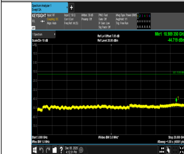
Band2-1.4MHz-QPSK-18900-1RB#0-3000~20000-PASS
