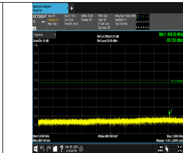
Band2-1.4MHz-QPSK-18900-1RB#5-30~1000-PASS
