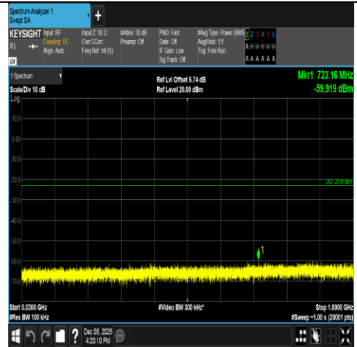
Band2-1.4MHz-QPSK-19193-1RB#5-30~1000-PASS
