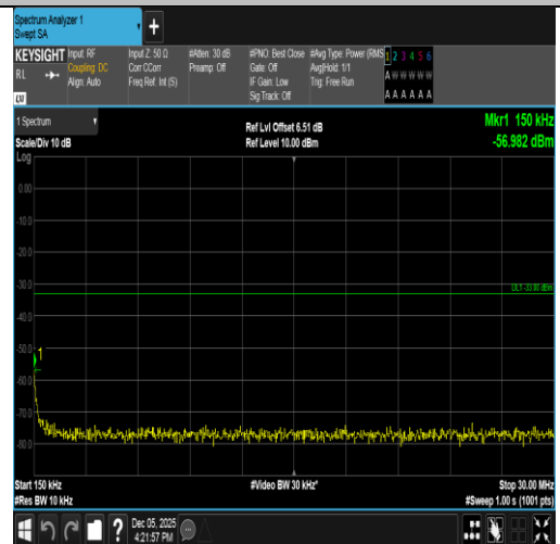
Band2-1.4MHz-QPSK-19193-6RB#0-0.15~30-PASS
