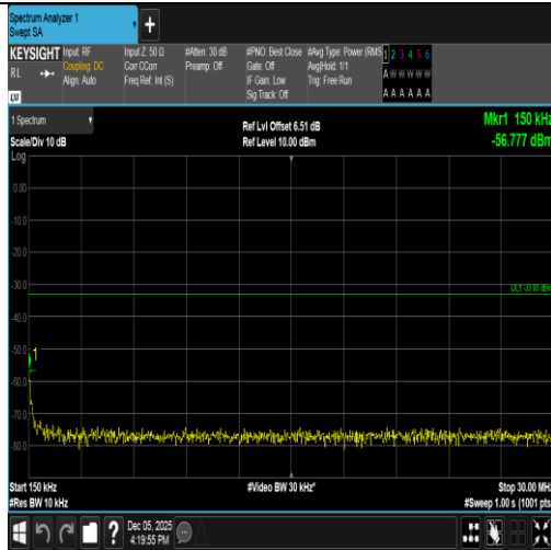
Band2-1.4MHz-QPSK-19193-1RB#5-0.15~30-PASS
