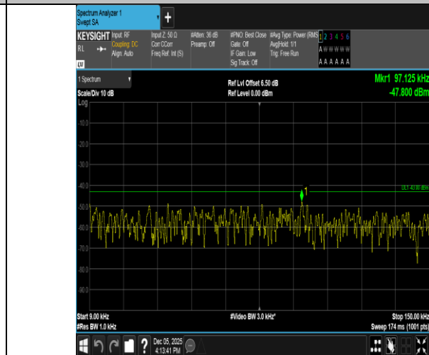
Band2-1.4MHz-QPSK-18900-1RB#5-0.009~0.15-PASS
