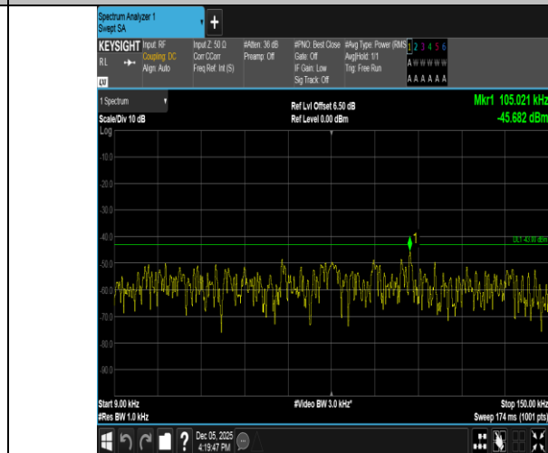
Band2-1.4MHz-QPSK-19193-1RB#5-0.009~0.15-PASS
