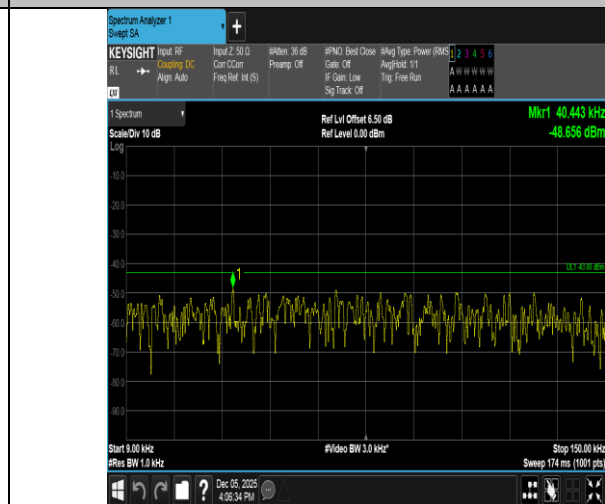
Band2-1.4MHz-16QAM-18607-1RB#0-0.009~0.15-PASS
