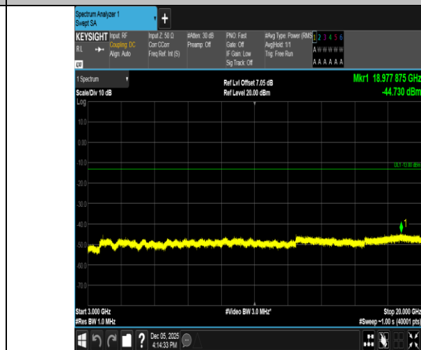
Band2-1.4MHz-QPSK-18900-1RB#5-3000~20000-PASS
