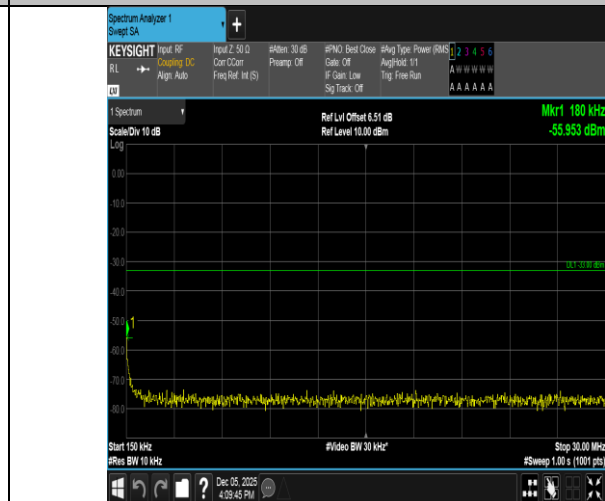
Band2-1.4MHz-QPSK-18607-6RB#0-0.15~30-PASS
