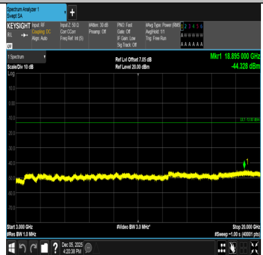
Band2-1.4MHz-QPSK-19193-1RB#5-3000~20000-PASS
