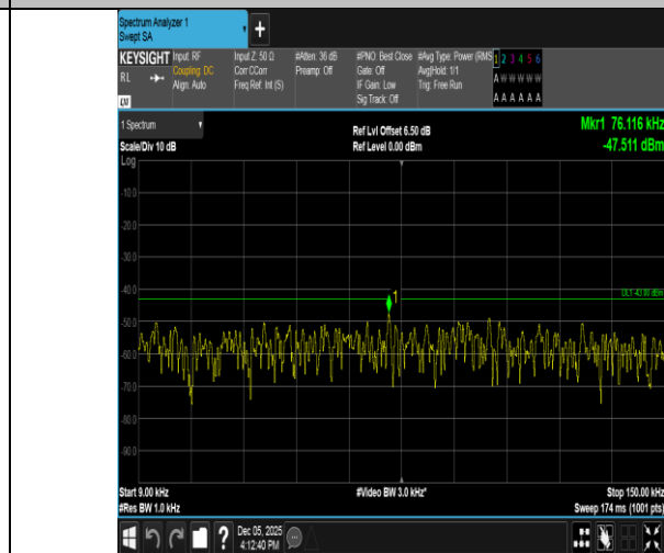
Band2-1.4MHz-16QAM-18900-1RB#0-0.009~0.15-PASS
