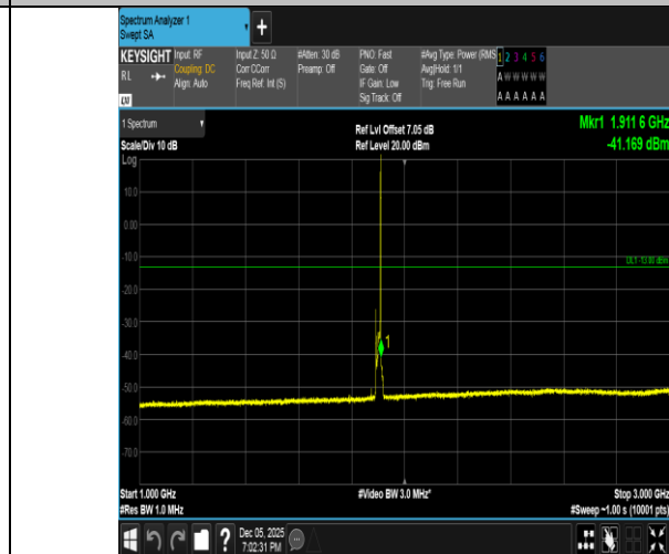
Band2-10MHz-16QAM-19150-1RB#49-1000~3000-PASS
