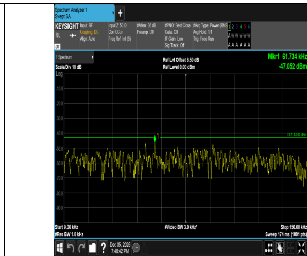
Band2-15MHz-16QAM-18675-75RB#0-0.009~0.15-PASS
