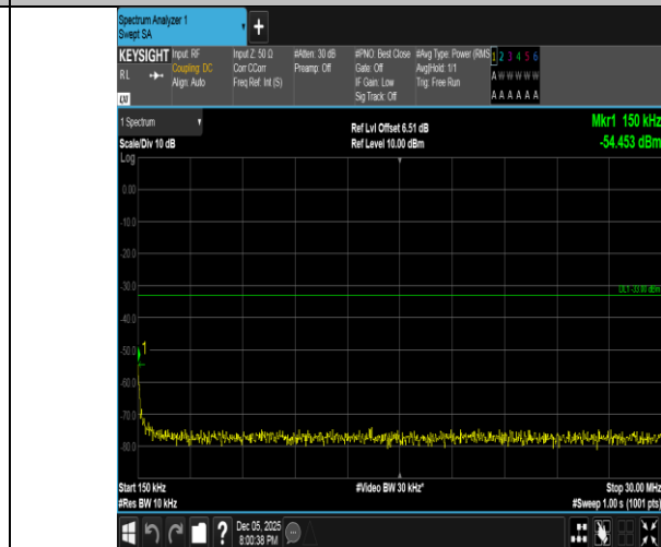
Band2-15MHz-QPSK-18900-75RB#0-0.15~30-PASS
