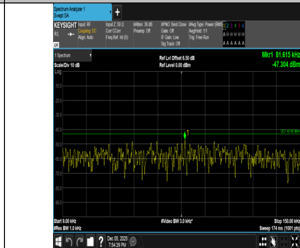
Band2-15MHz-QPSK-18900-1RB#74-0.009~0.15-PASS
