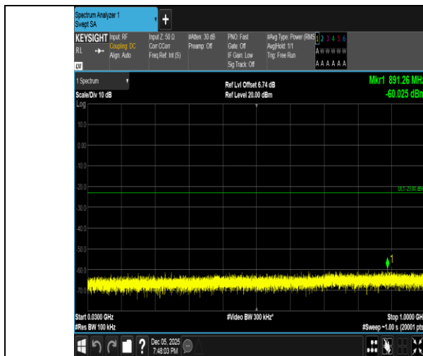
Band2-15MHz-QPSK-18675-75RB#0-30~1000-PASS
