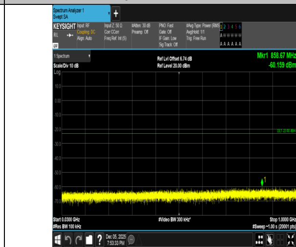
Band2-15MHz-16QAM-18900-1RB#0-30~1000-PASS
