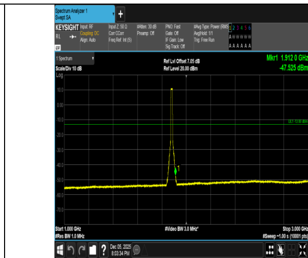
Band2-15MHz-QPSK-18900-75RB#0-1000~3000-PASS
