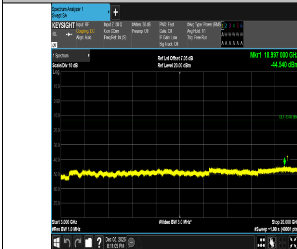
Band2-15MHz-QPSK-19125-1RB#0-3000~20000-PASS
