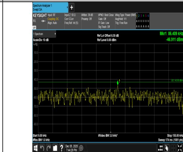
Band2-15MHz-QPSK-18675-1RB#74-0.009~0.15-PASS
