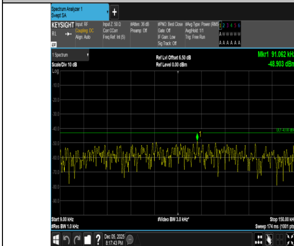
Band2-15MHz-QPSK-19125-75RB#0-0.009~0.15-PASS
