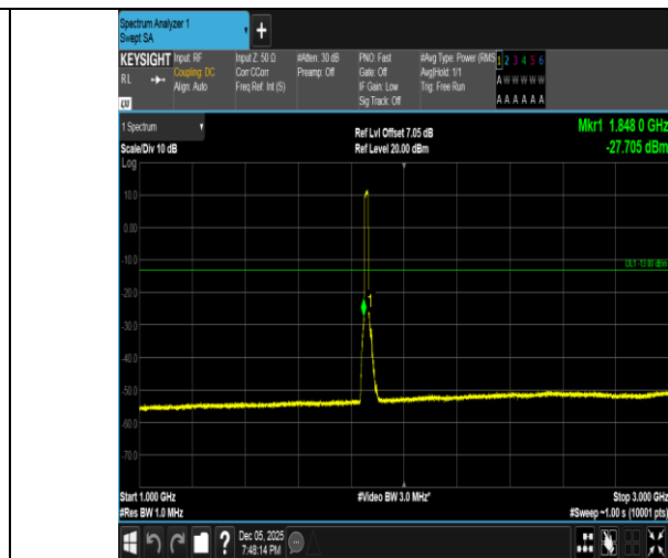
Band2-15MHz-QPSK-18675-75RB#0-1000~3000-PASS
