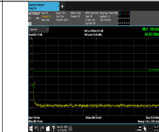
Band2-15MHz-QPSK-19125-75RB#0-0.15~30-PASS
