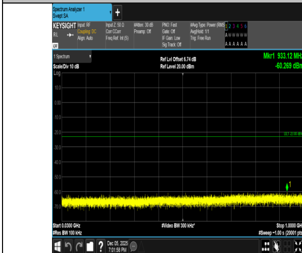
Band2-10MHz-16QAM-19150-1RB#49-30~1000-PASS
