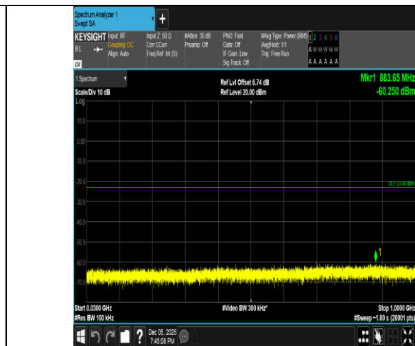
Band2-15MHz-QPSK-18675-1RB#74-30~1000-PASS
