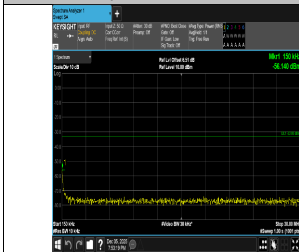
Band2-15MHz-16QAM-18900-1RB#0-0.15~30-PASS
