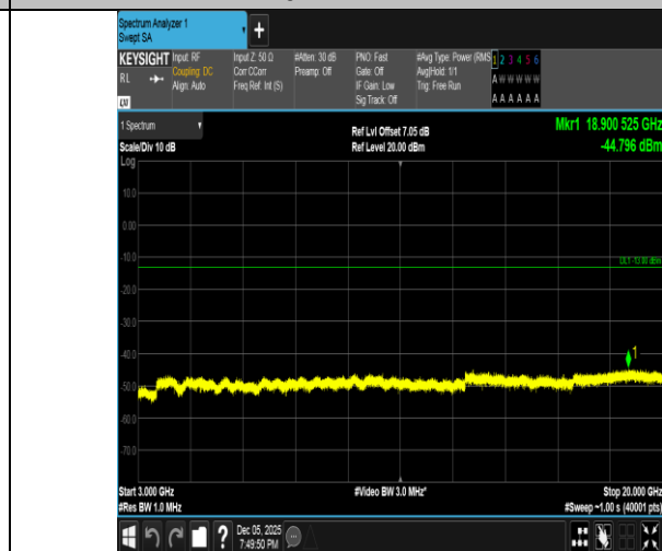
Band2-15MHz-16QAM-18675-75RB#0-3000~20000-PASS
