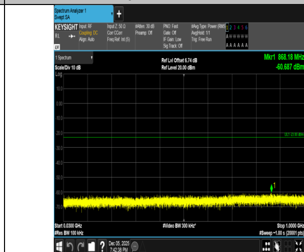
Band2-15MHz-16QAM-18675-1RB#0-30~1000-PASS
