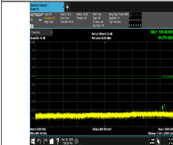
Band2-15MHz-16QAM-18900-1RB#74-30~1000-PASS
