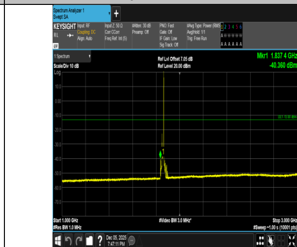
Band2-15MHz-16QAM-18675-1RB#74-1000~3000-PASS
