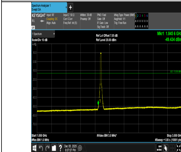
Band2-15MHz-16QAM-18900-75RB#0-1000~3000-PASS
