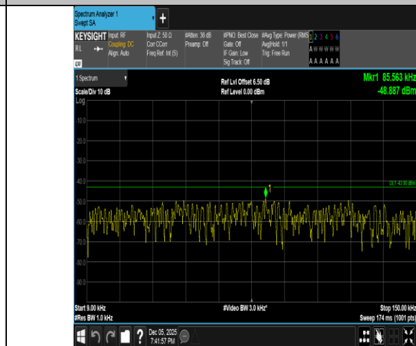
Band2-15MHz-16QAM-18675-1RB#0-0.009~0.15-PASS
