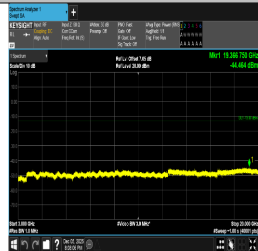
Band2-15MHz-16QAM-18900-75RB#0-3000~20000-PASS
