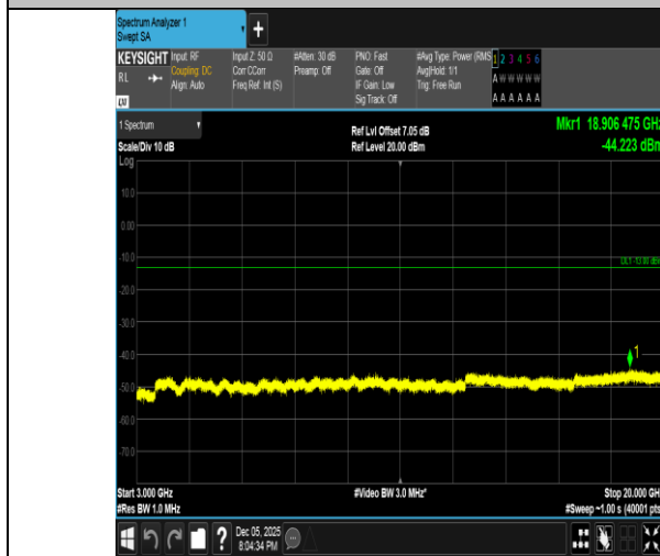
Band2-15MHz-QPSK-18900-75RB#0-3000~20000-PASS
