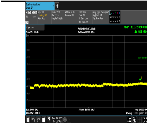
Band2-15MHz-QPSK-18675-1RB#0-3000~20000-PASS
