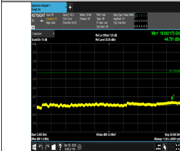
Band2-20MHz-QPSK-19100-1RB#0-3000~20000-PASS
