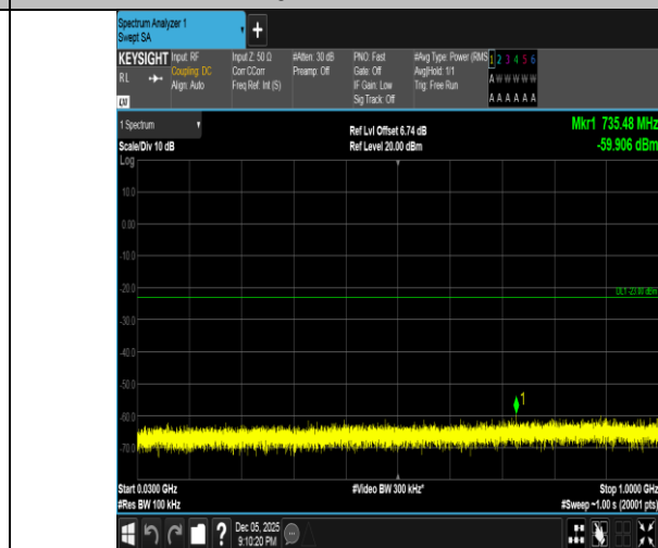
Band2-20MHz-16QAM-19100-1RB#0-30~1000-PASS
