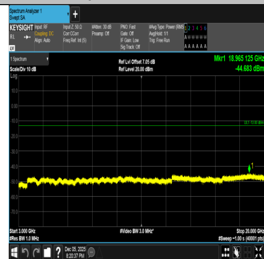
Band2-15MHz-16QAM-19125-75RB#0-3000~20000-PASS
