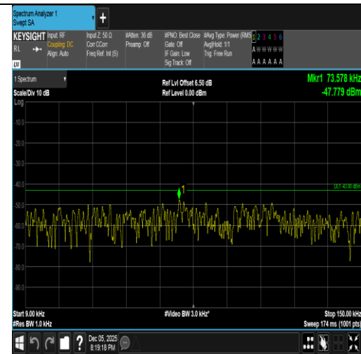
Band2-15MHz-16QAM-19125-75RB#0-0.009~0.15-PASS
