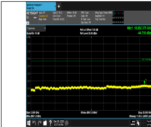
Band2-15MHz-16QAM-19125-1RB#74-3000~20000-PASS
