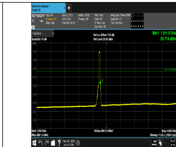
Band2-20MHz-QPSK-19100-100RB#0-1000~3000-PASS
