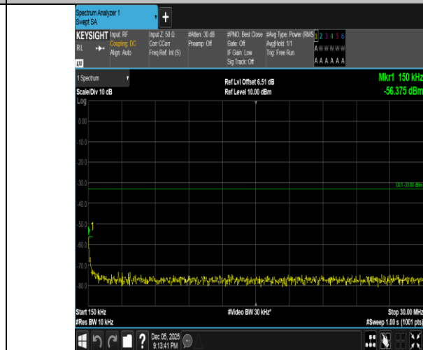
Band2-20MHz-QPSK-19100-100RB#0-0.15~30-PASS
