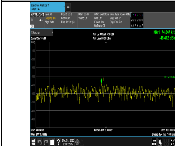
Band2-20MHz-QPSK-19100-100RB#0-0.009~0.15-PASS
