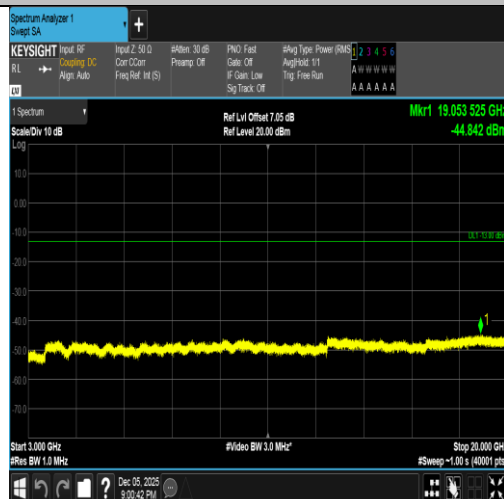
Band2-20MHz-QPSK-18900-1RB#0-3000~20000-PASS
