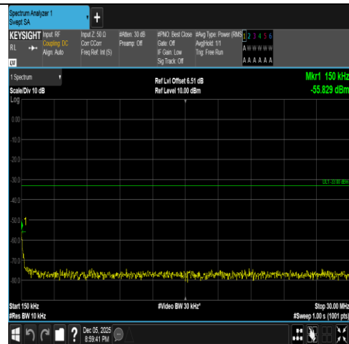
Band2-20MHz-QPSK-18900-1RB#0-0.15~30-PASS
