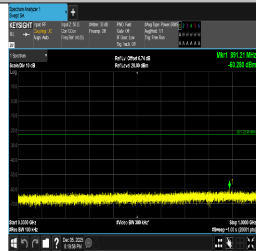
Band2-15MHz-16QAM-19125-75RB#0-30~1000-PASS
