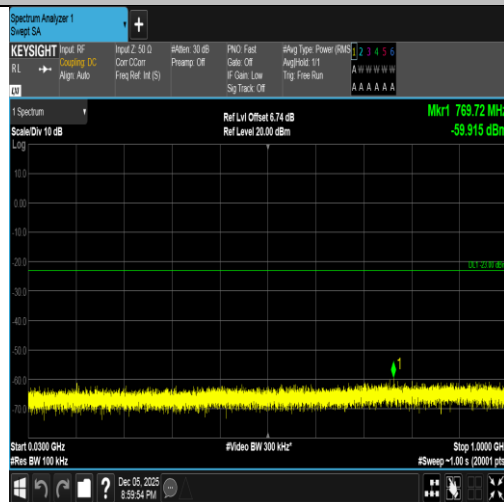
Band2-20MHz-QPSK-18900-1RB#0-30~1000-PASS
