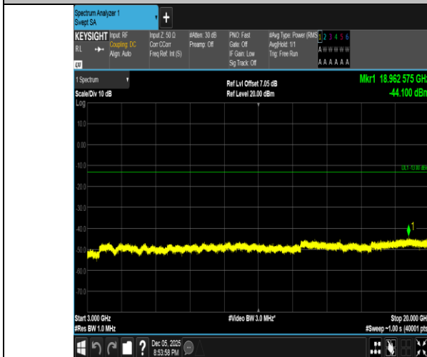
Band2-20MHz-QPSK-18700-1RB#0-3000~20000-PASS
