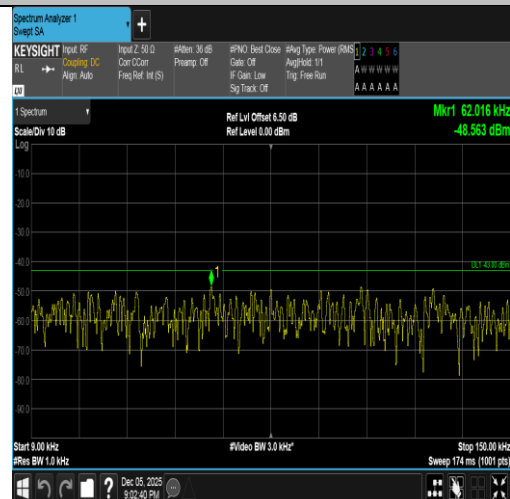
Band2-20MHz-QPSK-18900-1RB#99-0.009~0.15-PASS
