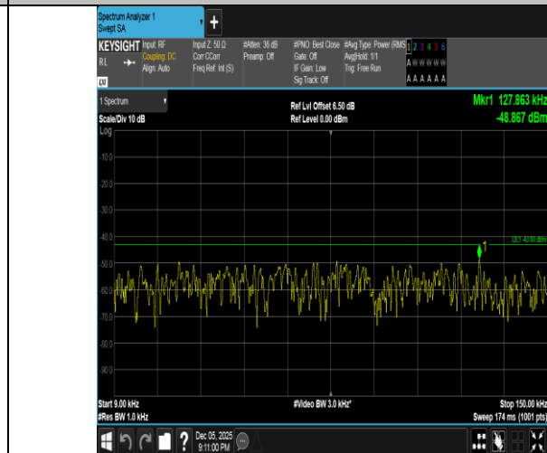
Band2-20MHz-QPSK-19100-1RB#99-0.009~0.15-PASS
