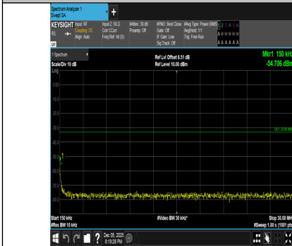
Band2-15MHz-16QAM-19125-75RB#0-0.15~30-PASS
