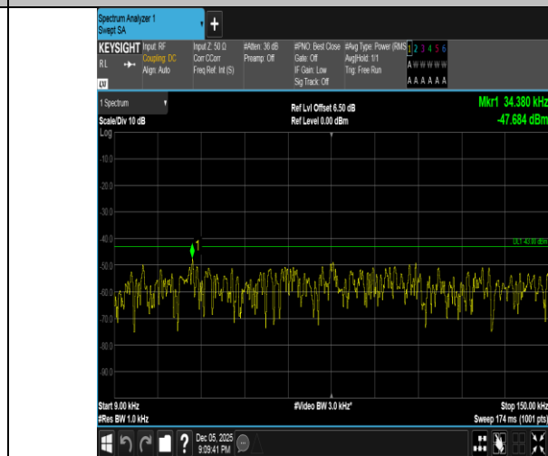
Band2-20MHz-16QAM-19100-1RB#0-0.009~0.15-PASS
