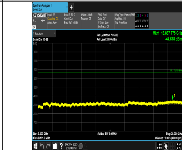
Band2-20MHz-16QAM-19100-100RB#0-3000~20000-PASS
