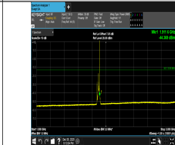
Band2-20MHz-16QAM-19100-1RB#99-1000~3000-PASS
