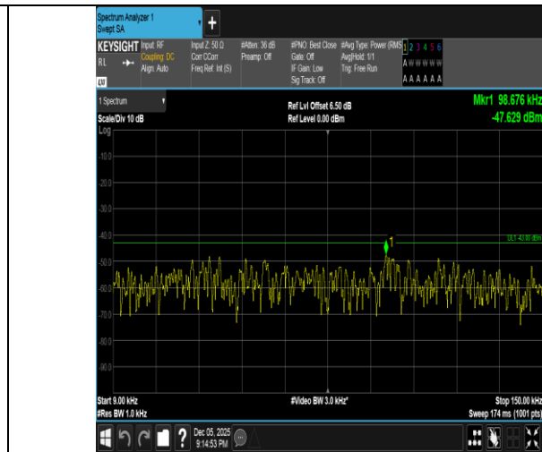
Band2-20MHz-16QAM-19100-100RB#0-0.009~0.15-PASS
