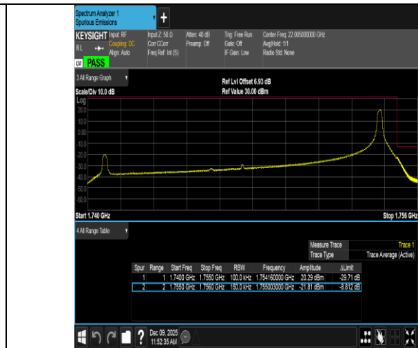
Band4-15MHz-QPSK-20325-1RB#74-PASS
