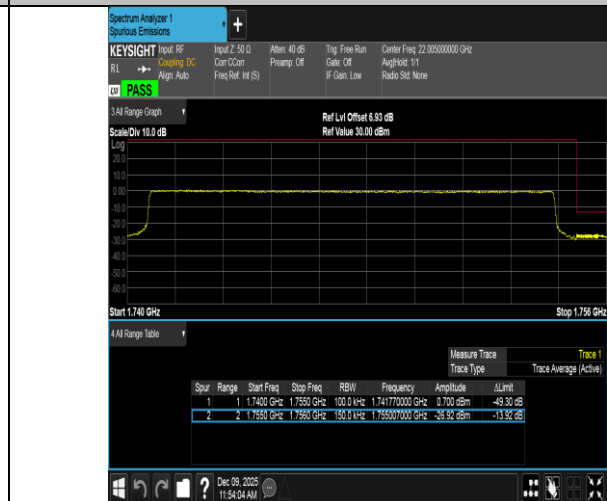
Band4-15MHz-16QAM-20325-75RB#0-PASS
