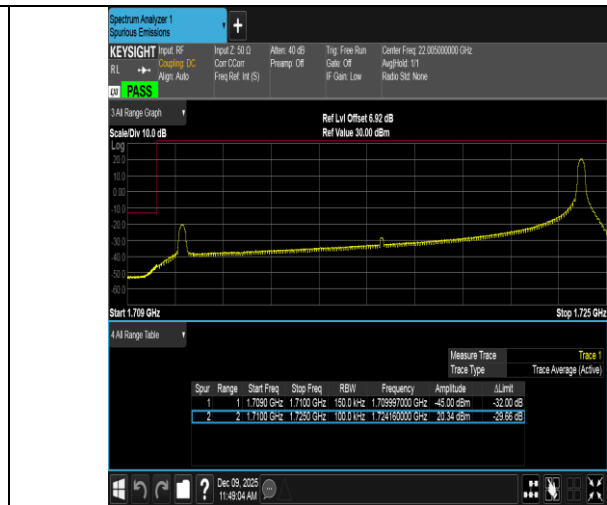
Band4-15MHz-QPSK-20025-1RB#74-PASS
