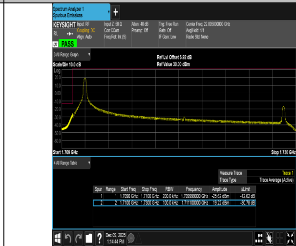
Band4-20MHz-16QAM-20050-1RB#0-PASS
