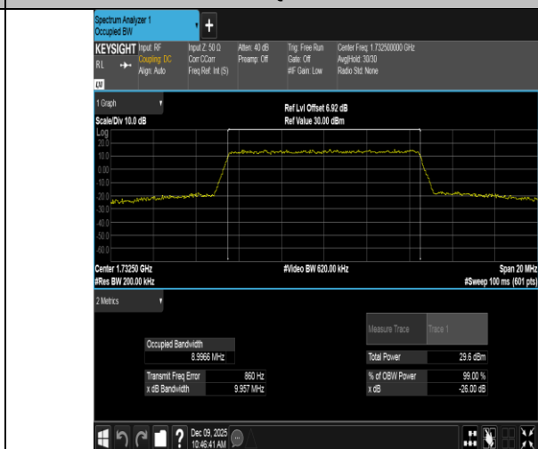
Band4-10MHz-16QAM-20175-50RB#0-PASS
