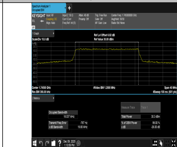
Band4-20MHz-16QAM-20300-100RB#0-PASS
