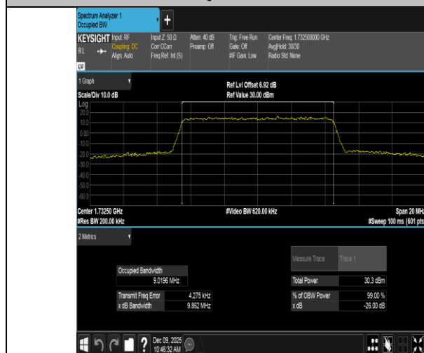
Band4-10MHz-QPSK-20175-50RB#0-PASS
