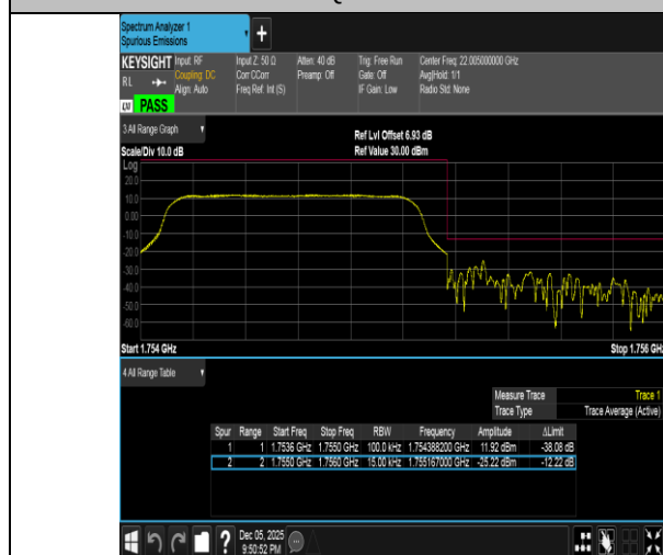
Band4-1.4MHz-OPSK-20393-6RB#0-PASS
