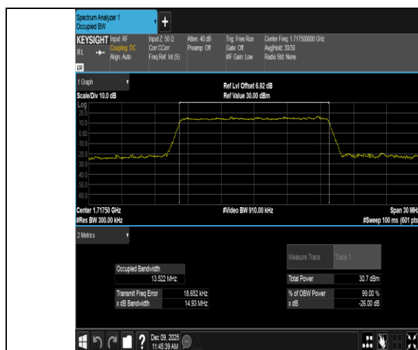
Band4-15MHz-QPSK-20025-75RB#0-PASS
