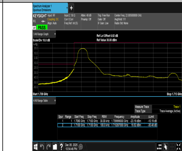
Band4-3MHz-16QAM-19965-1RB#0-PASS
