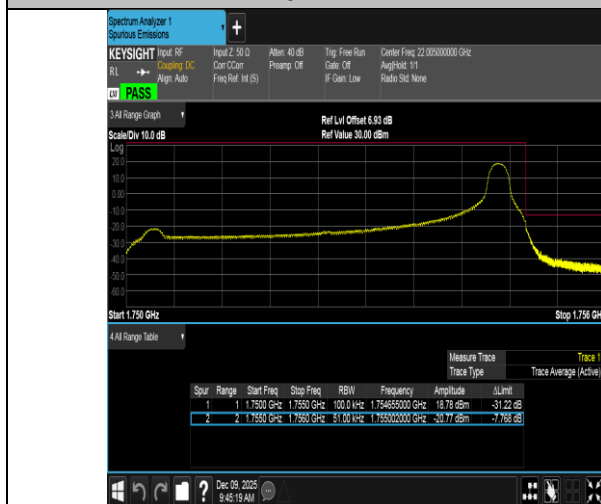
Band4-5MHz-16QAM-20375-1RB#24-PASS
