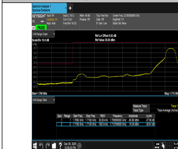
Band4-3MHz-16QAM-19965-1RB#14-PASS
