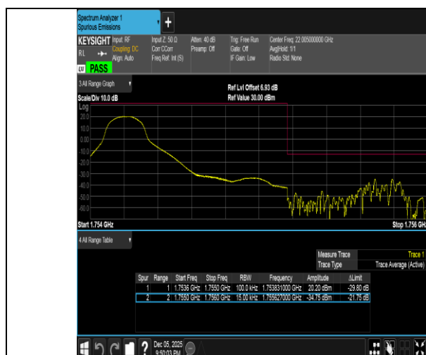
Band4-1.4MHz-OPSK-20393-1RB#0-PASS
