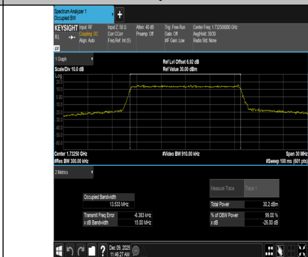
Band4-15MHz-16QAM-20175-75RB#0-PASS
