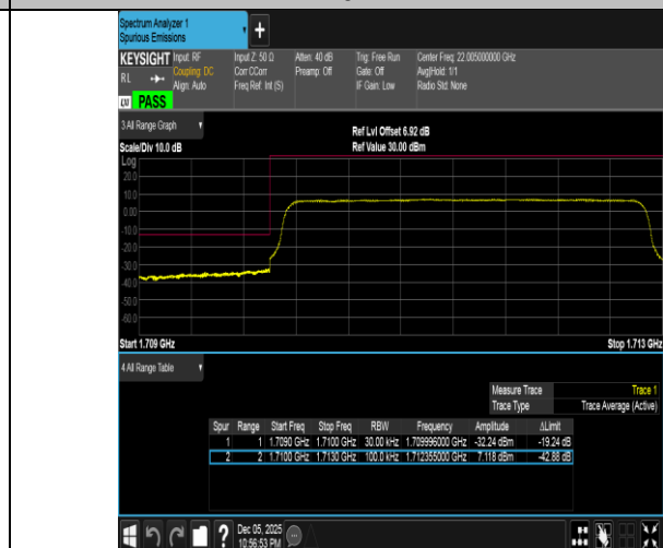
Band4-3MHz-16QAM-19965-15RB#0-PASS
