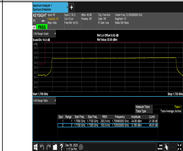
Band4-20MHz-16QAM-20050-100RB#0-PASS
