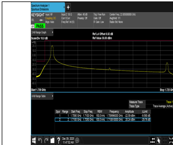
Band4-15MHz-QPSK-20025-1RB#0-PASS
