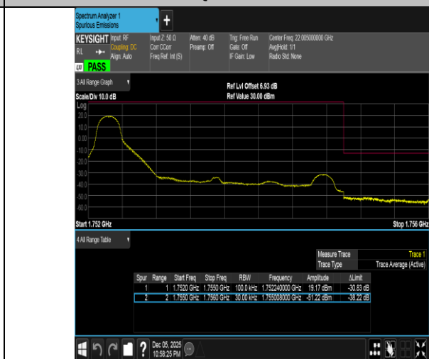
Band4-3MHz-16QAM-20385-1RB#0-PASS
