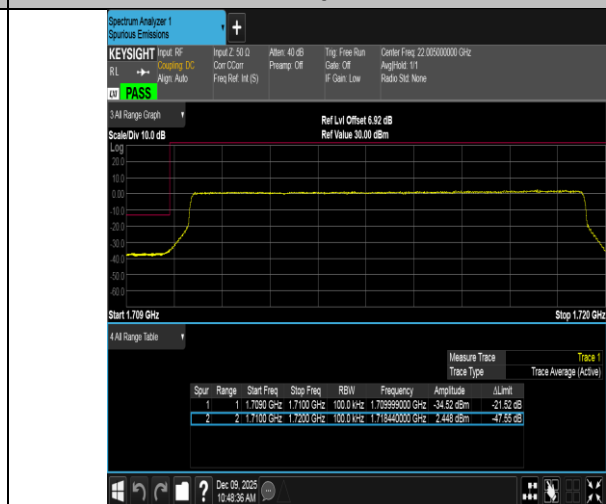
Band4-10MHz-16QAM-20000-50RB#0-PASS
