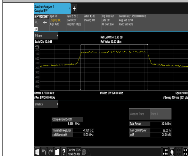
Band4-10MHz-QPSK-20350-50RB#0-PASS
