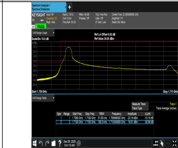
Band4-5MHz-16QAM-19975-1RB#0-PASS
