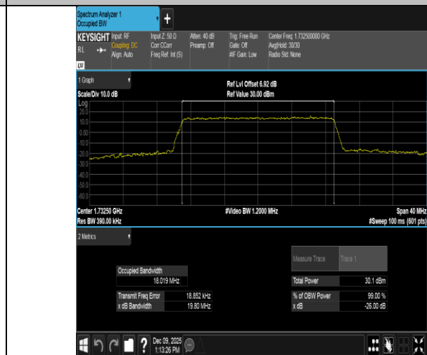
Band4-20MHz-16QAM-20175-100RB#0-PASS
