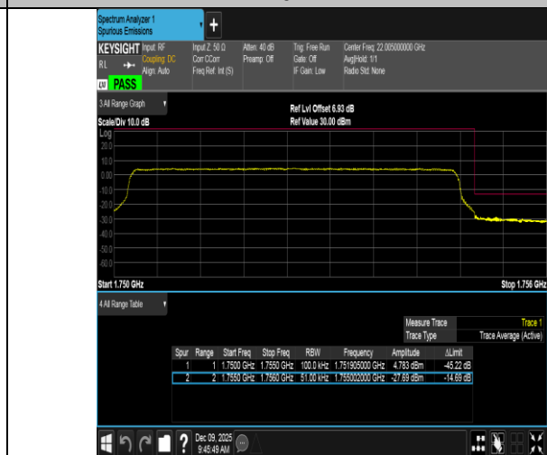
Band4-5MHz-16QAM-20375-25RB#0-PASS
