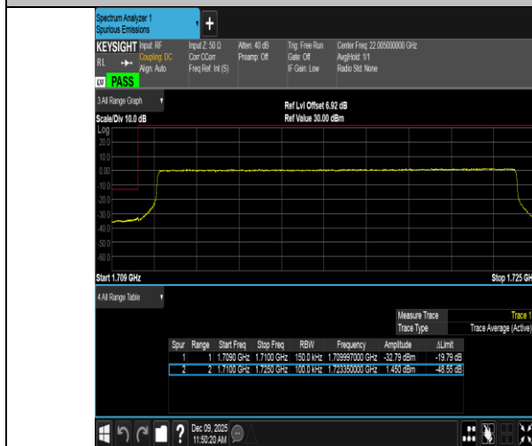
Band4-15MHz-QPSK-20025-75RB#0-PASS
