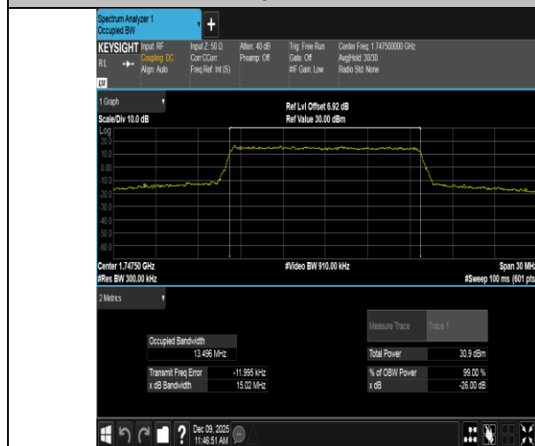
Band4-15MHz-QPSK-20325-75RB#0-PASS
