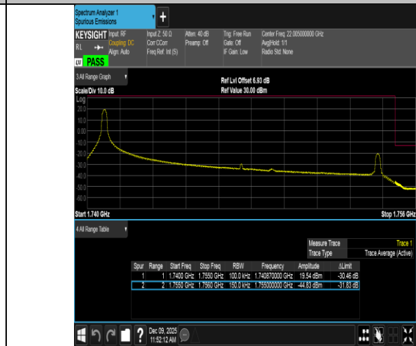
Band4-15MHz-16QAM-20325-1RB#0-PASS
