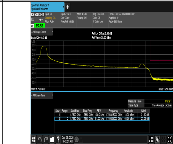
Band4-5MHz-16QAM-20375-1RB#0-PASS
