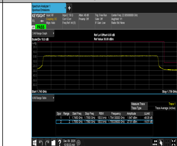
Band4-10MHz-16QAM-20350-50RB#0-PASS
