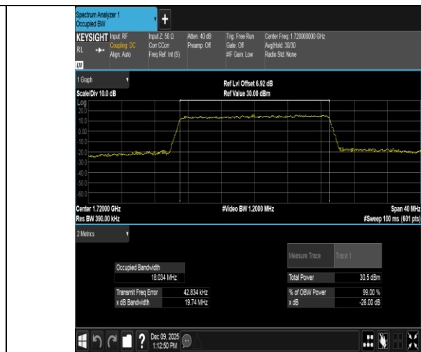
Band4-20MHz-16QAM-20050-100RB#0-PASS
