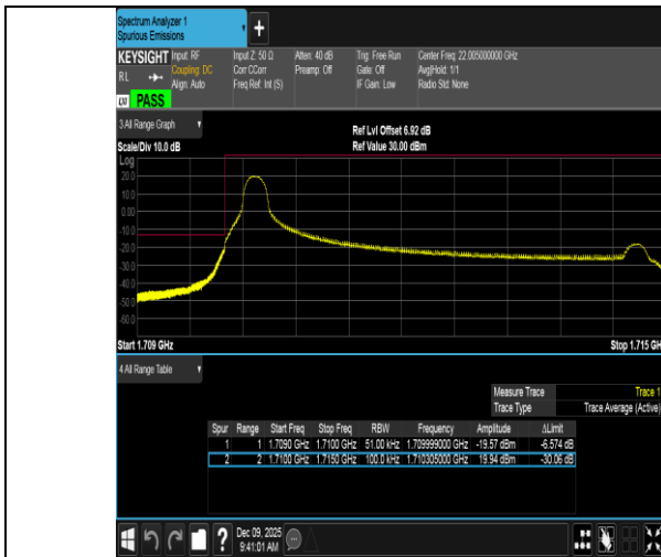
Band4-5MHz-QPSK-19975-1RB#0-PASS
