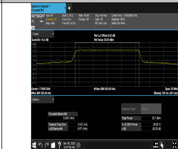
Band4-10MHz-16QAM-20350-50RB#0-PASS
