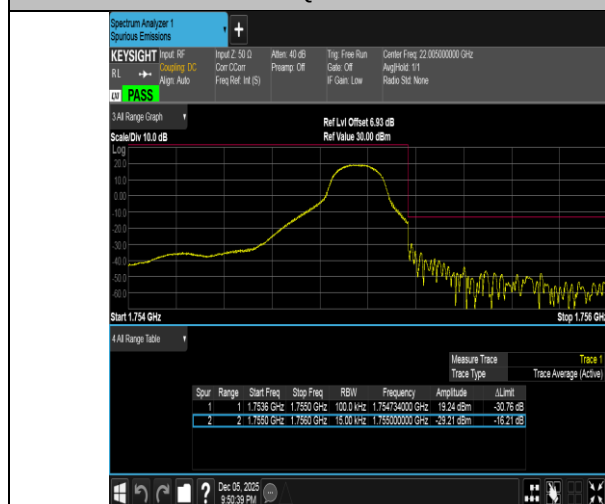
Band4-1.4MHz-16OAM-20393-1RB#5-PASS
