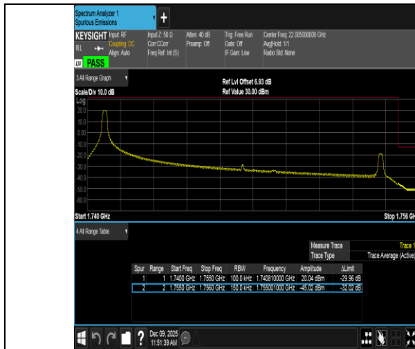
Band4-15MHz-QPSK-20325-1RB#0-PASS
