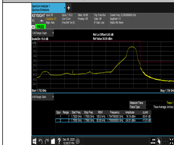
Band4-3MHz-16QAM-20385-1RB#14-PASS
