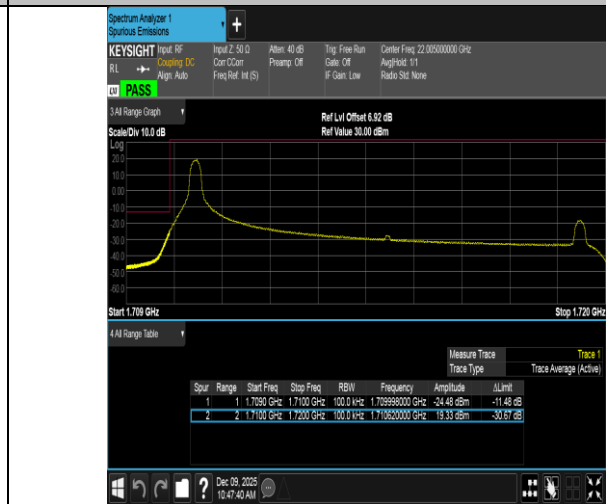
Band4-10MHz-16QAM-20000-1RB#0-PASS
