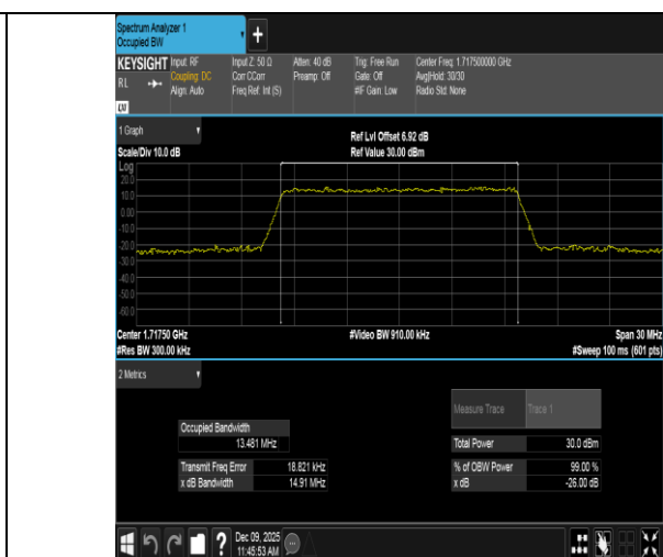
Band4-15MHz-16QAM-20025-75RB#0-PASS
