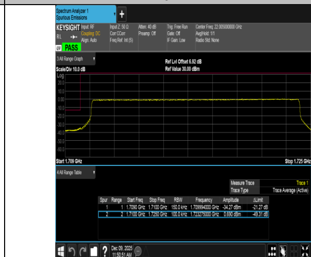
Band4-15MHz-16QAM-20025-75RB#0-PASS
