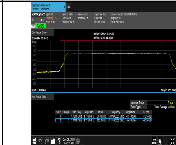
Band4-5MHz-16QAM-19975-25RB#0-PASS
