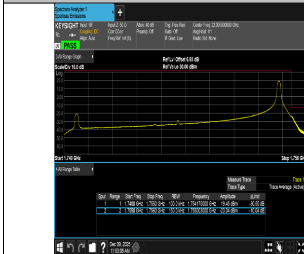
Band4-15MHz-16QAM-20325-1RB#74-PASS
