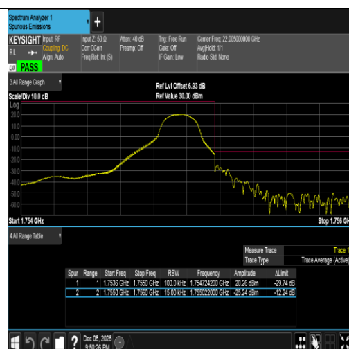
Band4-1.4MHz-OPSK-20393-1RB#5-PASS
