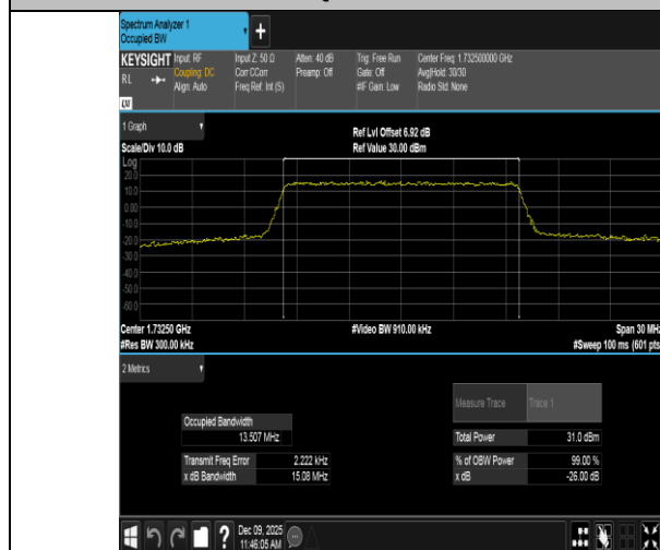
Band4-15MHz-QPSK-20175-75RB#0-PASS
