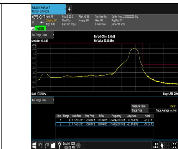
Band4-3MHz-QPSK-20385-1RB#14-PASS
