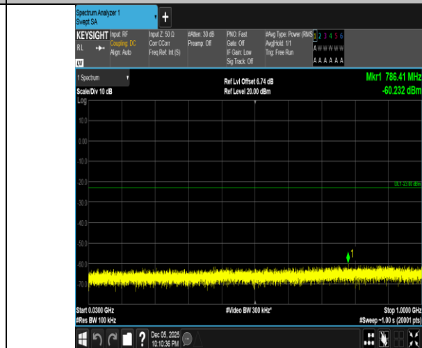
Band4-1.4MHz-16QAM-20393-1RB#0-30~1000-PASS
