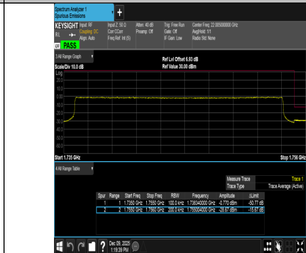
Band4-20MHz-16QAM-20300-100RB#0-PASS
