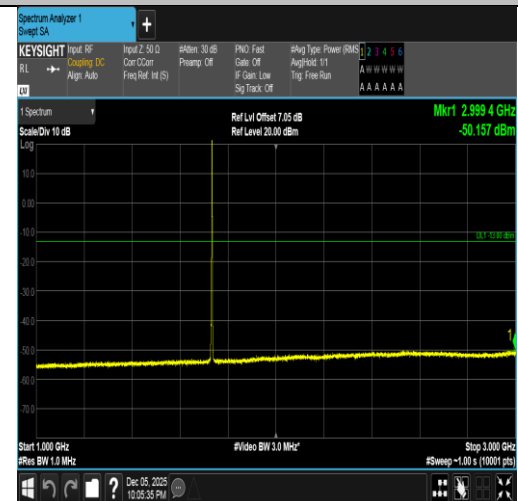
Band4-1.4MHz-16QAM-20175-1RB#5-1000~3000-PASS
