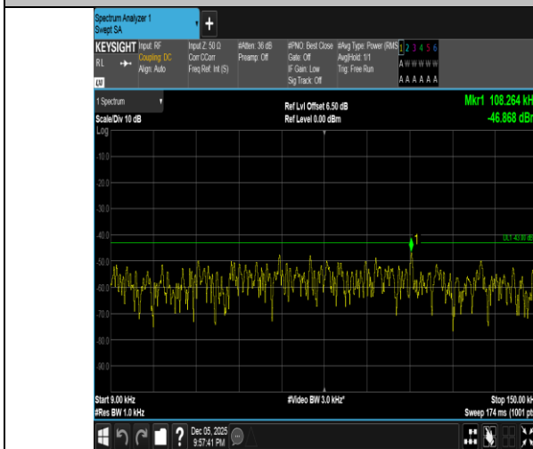
Band4-1.4MHz-16QAM-19957-1RB#5-0.009~0.15-PASS
