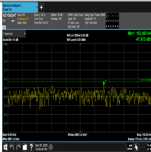
Band4-1.4MHz-16QAM-20175-1RB#5-0.009~0.15-PASS
