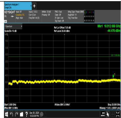
Band4-1.4MHz-16QAM-20175-1RB#0-3000~20000-PASS
