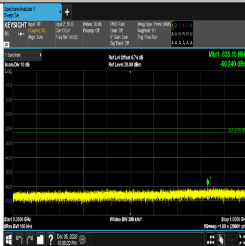
Band4-1.4MHz-16QAM-20175-1RB#5-30~1000-PASS
