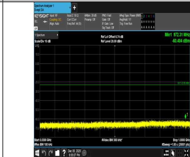
Band4-1.4MHz-16QAM-19957-1RB#0-30~1000-PASS
