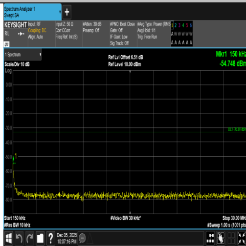
Band4-1.4MHz-16QAM-20175-6RB#0-0.15~30-PASS
