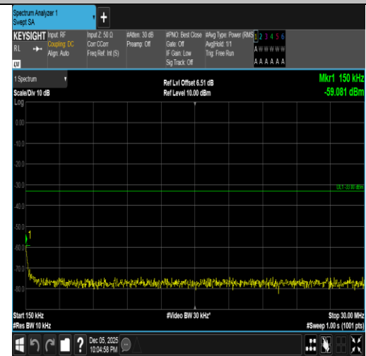
Band4-1.4MHz-16QAM-20175-1RB#5-0.15~30-PASS
