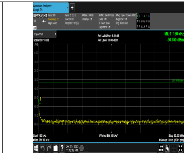
Band4-3MHz-QPSK-20175-1RB#0-0.15~30-PASS
