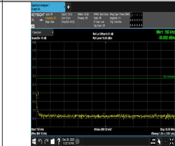
Band4-3MHz-16QAM-19965-1RB#14-0.15~30-PASS
