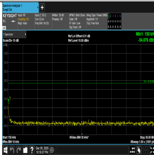
Band4-1.4MHz-16QAM-20393-6RB#0-0.15~30-PASS
