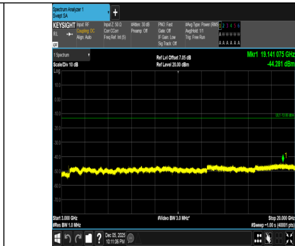
Band4-1.4MHz-16QAM-20393-1RB#0-3000~20000-PASS
