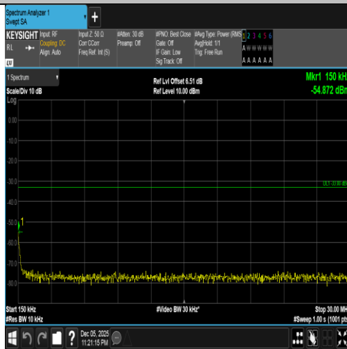
Band4-3MHz-16QAM-20175-15RB#0-0.15~30-PASS
