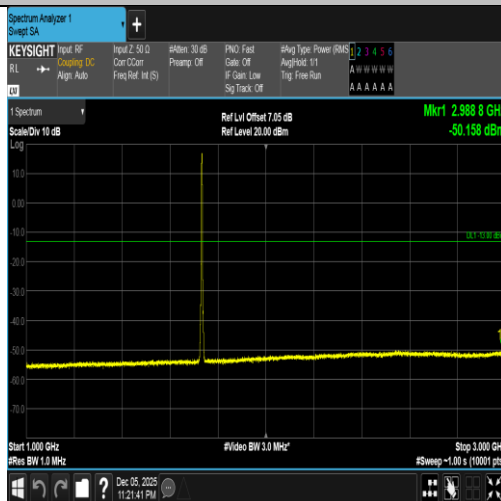
Band4-3MHz-16QAM-20175-15RB#0-1000~3000-PASS
