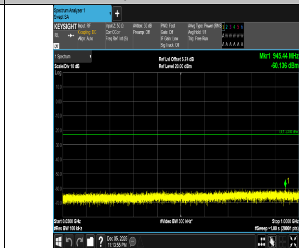
Band4-3MHz-16QAM-20175-1RB#0-30~1000-PASS
