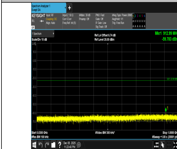
Band4-3MHz-QPSK-20385-1RB#0-30~1000-PASS
