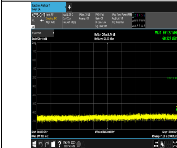
Band4-3MHz-16QAM-19965-1RB#14-30~1000-PASS
