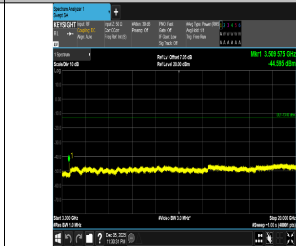
Band4-3MHz-QPSK-20385-1RB#14-3000~20000-PASS
