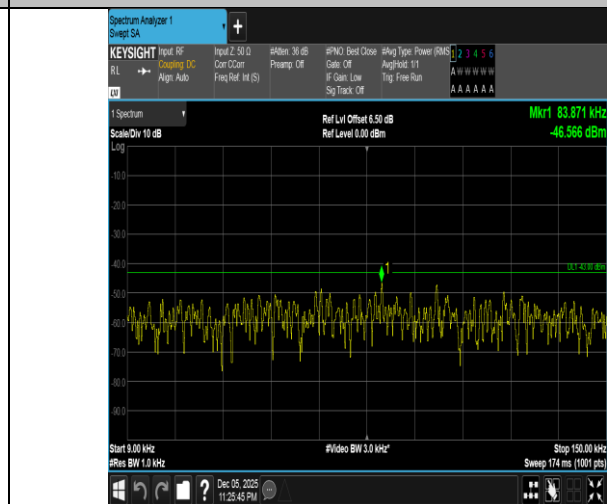
Band4-3MHz-16QAM-20385-1RB#0-0.009~0.15-PASS
