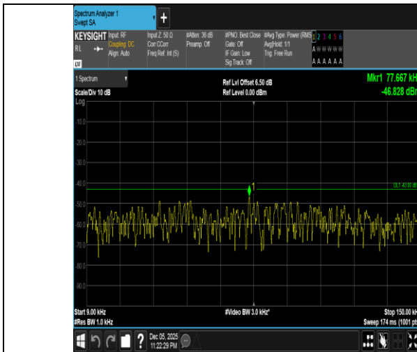
Band4-3MHz-QPSK-20385-1RB#0-0.009~0.15-PASS
