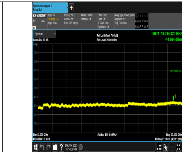
Band4-3MHz-16QAM-20175-1RB#0-3000~20000-PASS
