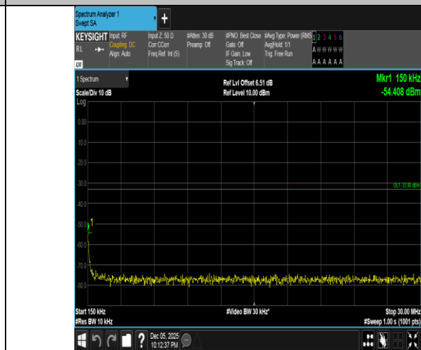
Band4-1.4MHz-16QAM-20393-1RB#5-0.15~30-PASS
