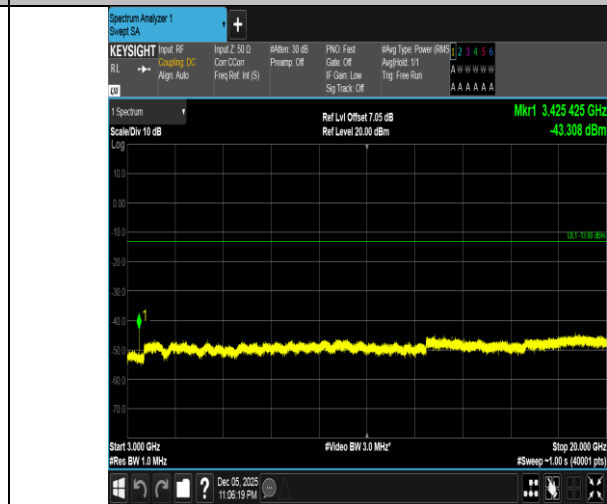
Band4-3MHz-QPSK-19965-1RB#14-3000~20000-PASS
