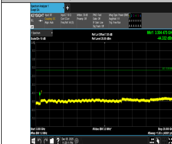
Band4-3MHz-QPSK-20385-1RB#0-3000~20000-PASS
