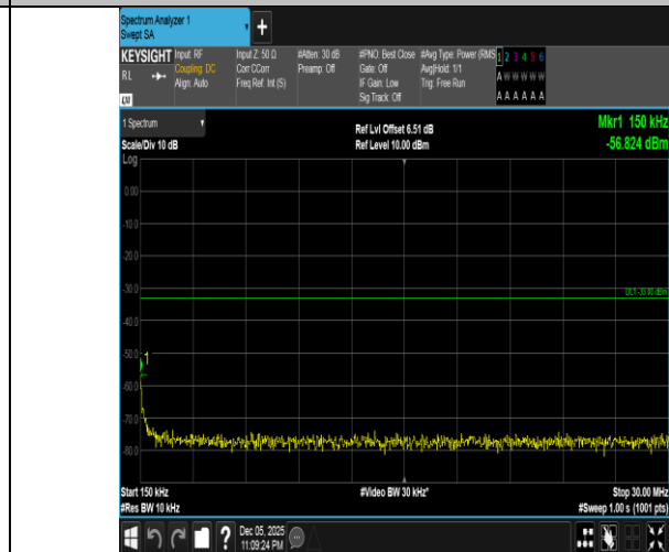
Band4-3MHz-QPSK-19965-15RB#0-0.15~30-PASS
