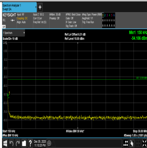
Band4-3MHz-16QAM-19965-15RB#0-0.15~30-PASS
