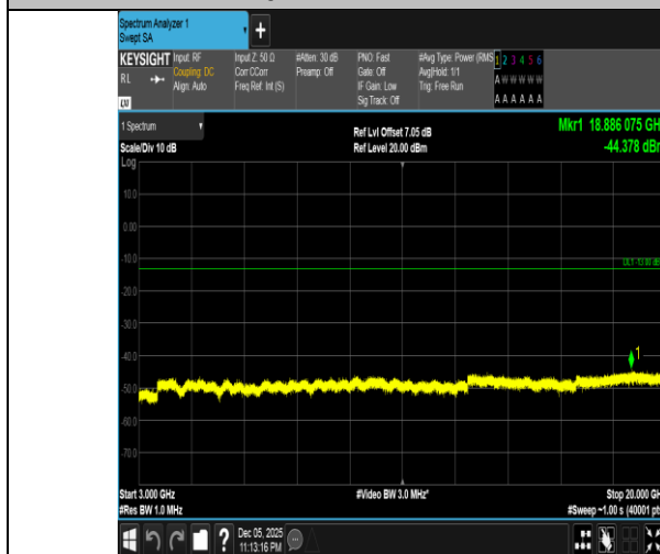
Band4-3MHz-QPSK-20175-1RB#0-3000~20000-PASS
