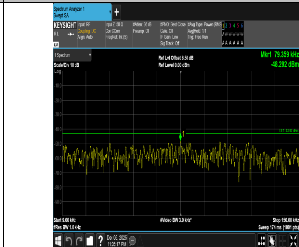
Band4-3MHz-QPSK-19965-1RB#14-0.009~0.15-PASS
