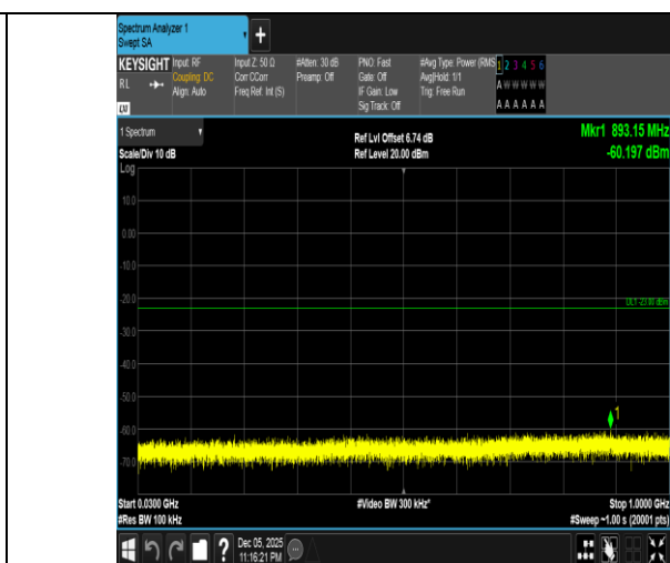
Band4-3MHz-QPSK-20175-1RB#14-30~1000-PASS
