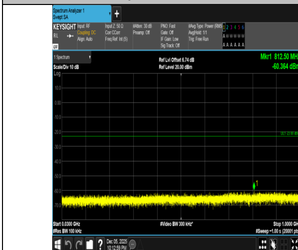
Band4-1.4MHz-16QAM-20393-1RB#5-30~1000-PASS
