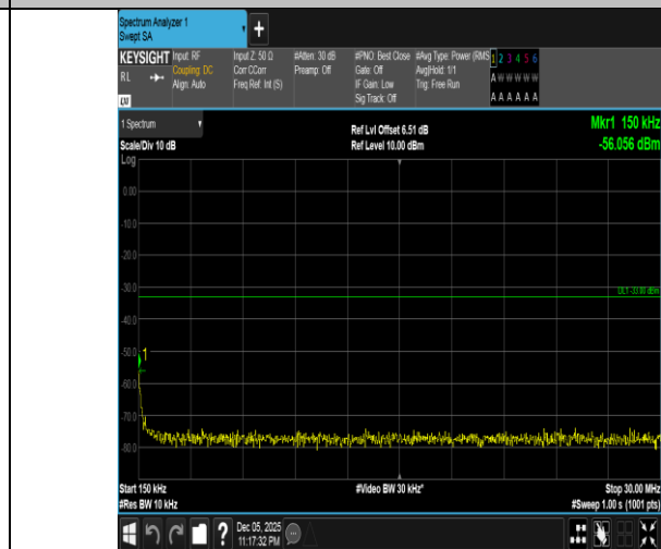
Band4-3MHz-16QAM-20175-1RB#14-0.15~30-PASS
