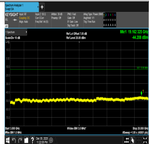
Band4-3MHz-16QAM-20175-15RB#0-3000~20000-PASS
