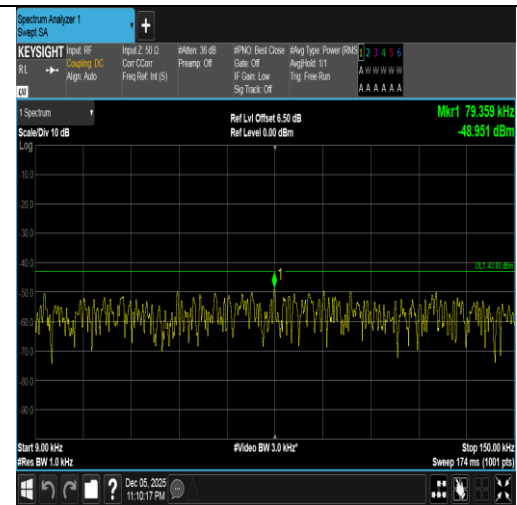
Band4-3MHz-16QAM-19965-15RB#0-0.009~0.15-PASS
