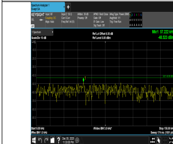
Band4-3MHz-QPSK-20385-15RB#0-0.009~0.15-PASS
