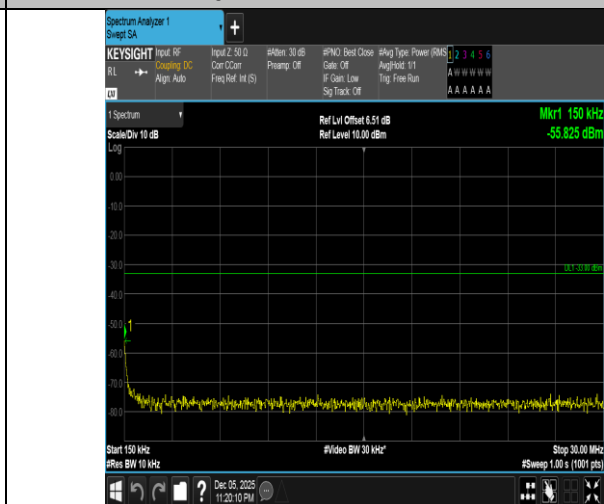
Band4-3MHz-QPSK-20175-15RB#0-0.15~30-PASS
