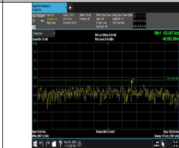
Band4-3MHz-16QAM-20175-1RB#0-0.009~0.15-PASS
