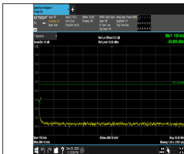
Band4-3MHz-QPSK-20175-1RB#14-0.15~30-PASS
