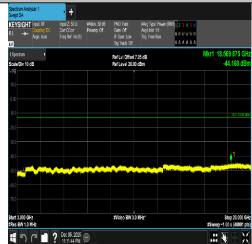
Band4-3MHz-16QAM-19965-15RB#0-3000~20000-PASS
