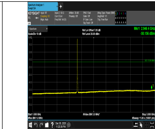
Band4-3MHz-QPSK-20175-15RB#0-1000~3000-PASS
