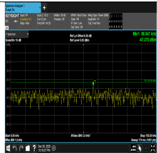
Band4-1.4MHz-16QAM-20393-6RB#0-0.009~0.15-PASS
