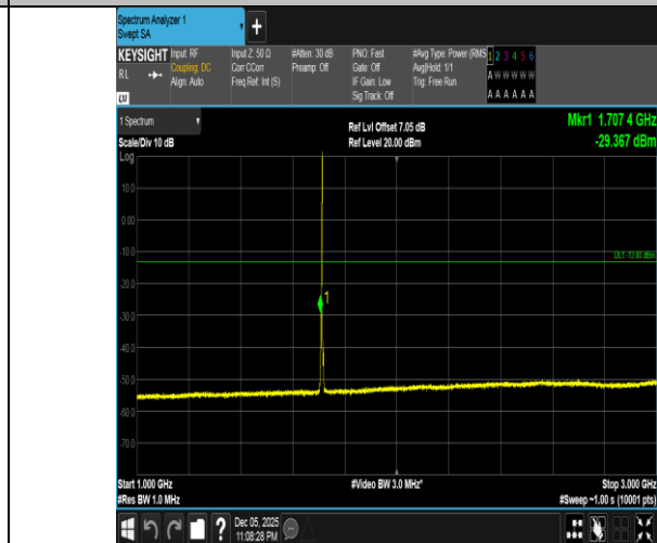
Band4-3MHz-16QAM-19965-1RB#14-1000~3000-PASS
