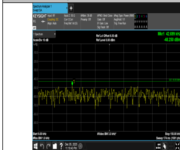
Band4-3MHz-QPSK-20175-15RB#0-0.009~0.15-PASS
