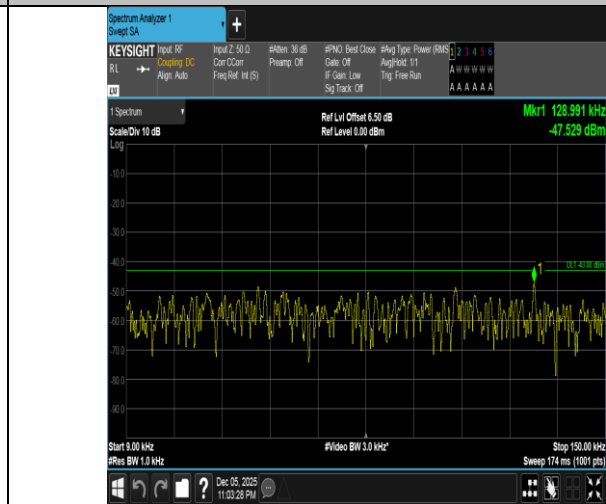
Band4-3MHz-16QAM-19965-1RB#0-0.009~0.15-PASS
