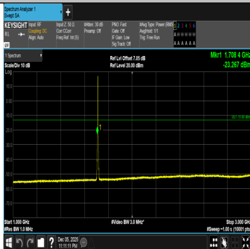
Band4-3MHz-16QAM-19965-15RB#0-1000~3000-PASS
