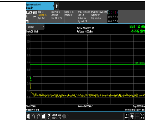
Band4-3MHz-QPSK-19965-1RB#0-0.15~30-PASS
