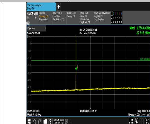
Band4-1.4MHz-16QAM-20393-1RB#5-1000~3000-PASS
