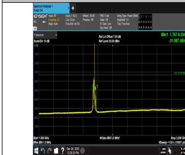
Band4-15MHz-QPSK-20325-1RB#74-1000~3000-PASS
