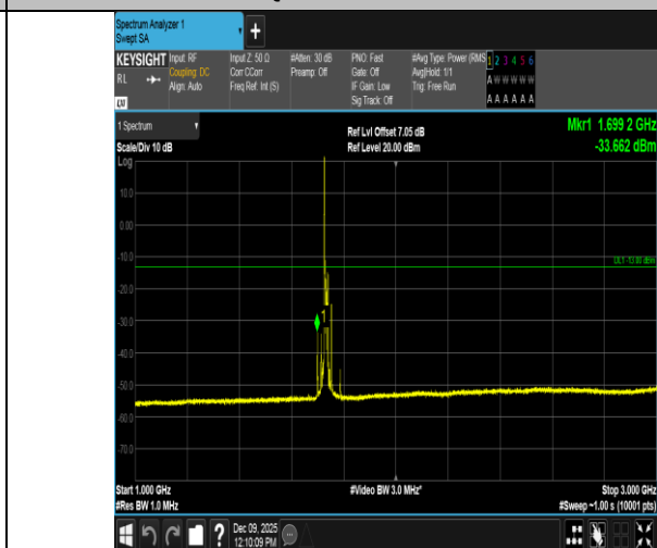
Band4-15MHz-QPSK-20175-1RB#0-1000~3000-PASS
