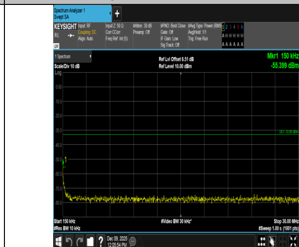
Band4-15MHz-QPSK-2025-75RB#0-0.15~30-PASS
