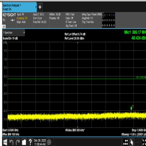
Band4-10MHz-16QAM-20350-1RB#49-30~1000-PASS
