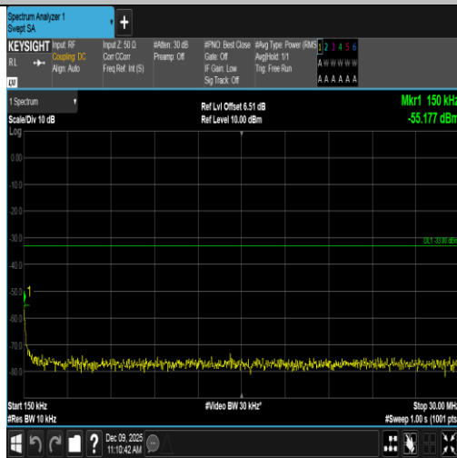
Band4-10MHz-16QAM-20350-50RB#0-0.15~30-PASS
