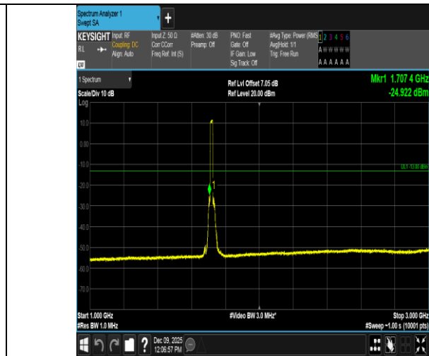
Band4-15MHz-QPSK-2025-75RB#0-1000~3000-PASS
