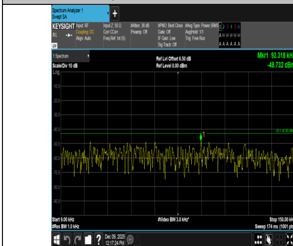
Band4-15MHz-QPSK-20175-75RB#0-0.009~0.15-PASS
