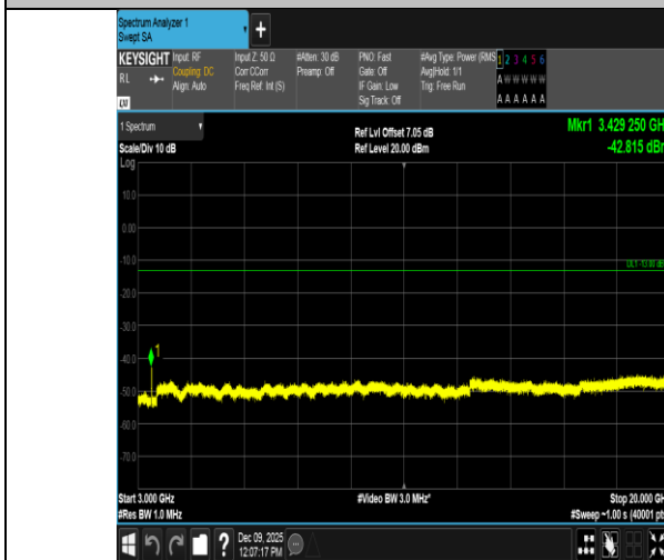
Band4-15MHz-QPSK-2025-75RB#0-3000~20000-PASS
