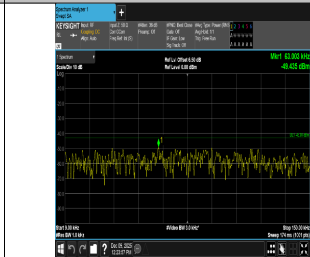
Band4-15MHz-16QAM-20325-1RB#0-0.009~0.15-PASS
