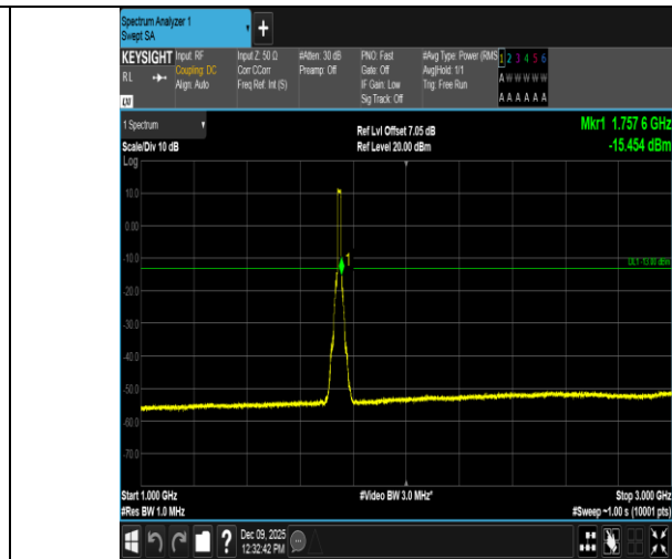
Band4-15MHz-QPSK-20325-75RB#0-1000~3000-PASS
