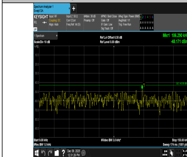
Band4-15MHz-QPSK-20325-75RB#0-0.009~0.15-PASS
