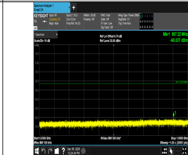
Band4-15MHz-16QAM-20325-1RB#0-30~1000-PASS
