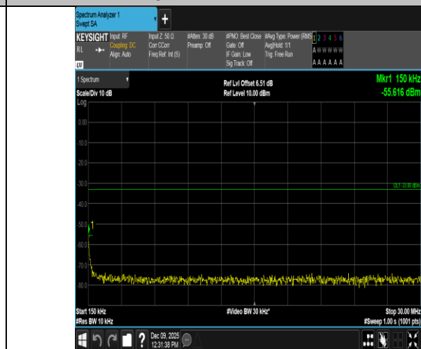
Band4-15MHz-QPSK-20325-75RB#0-0.15~30-PASS
