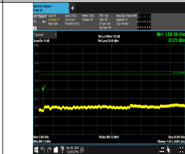
Band4-15MHz-QPSK-20325-1RB#74-3000~20000-PASS
