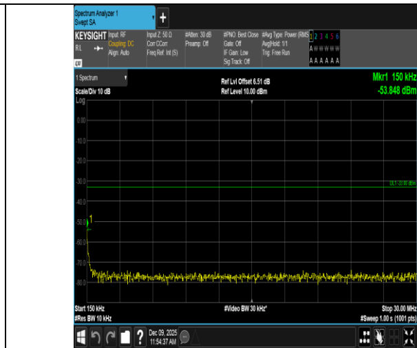
Band4-15MHz-QPSK-2025-1RB#0-0.15~30-PASS
