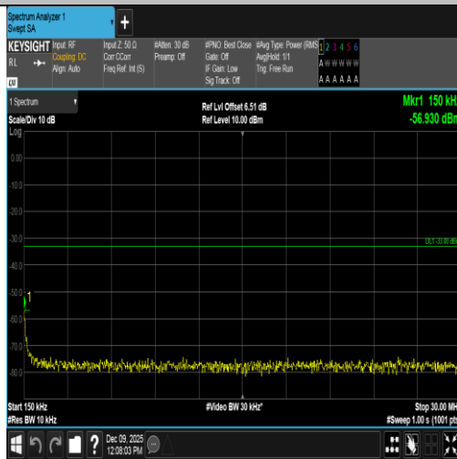
Band4-15MHz-16QAM-2025-75RB#0-0.15~30-PASS
