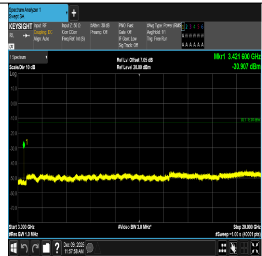
Band4-15MHz-16QAM-20025-1RB#0-3000~20000-PASS
