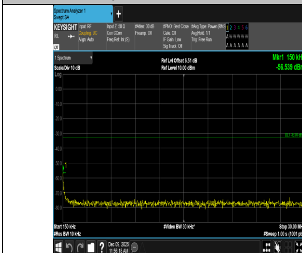
Band4-15MHz-16QAM-2025-1RB#0-0.15~30-PASS
