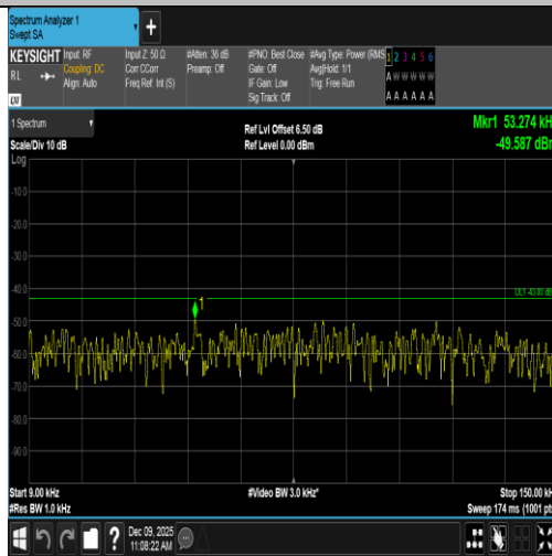
Band4-10MHz-16QAM-20350-1RB#49-0.009~0.15-PASS
