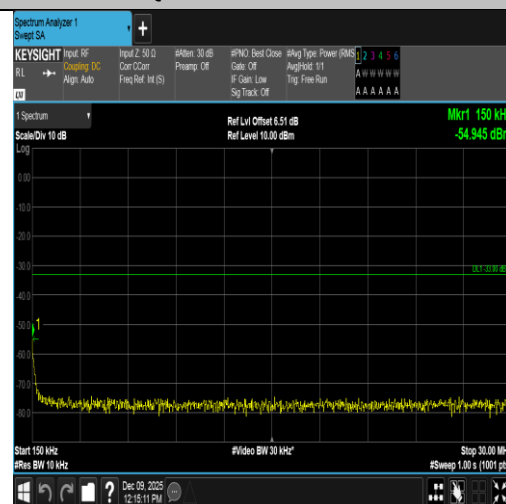
Band4-15MHz-16QAM-20175-1RB#74-0.15~30-PASS
