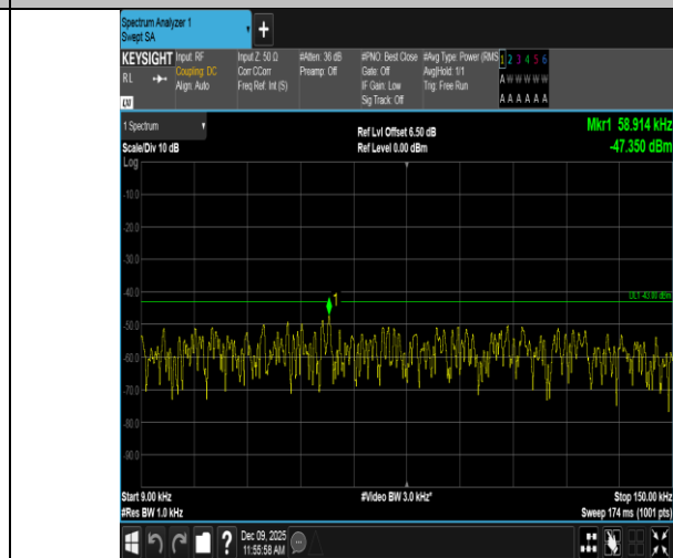
Band4-15MHz-16QAM-2025-1RB#0-0.009~0.15-PASS
