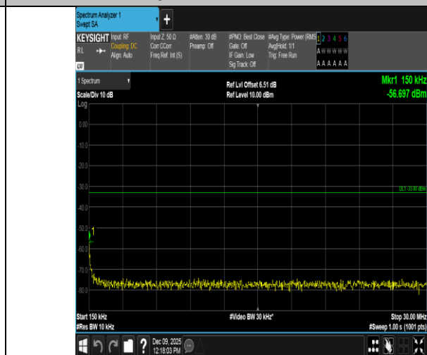
Band4-15MHz-QPSK-20175-75RB#0-0.15~30-PASS
