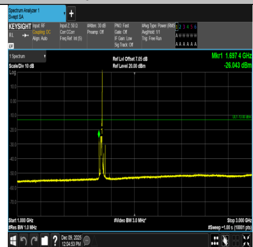
Band4-15MHz-16QAM-20025-1RB#74-1000~3000-PASS
