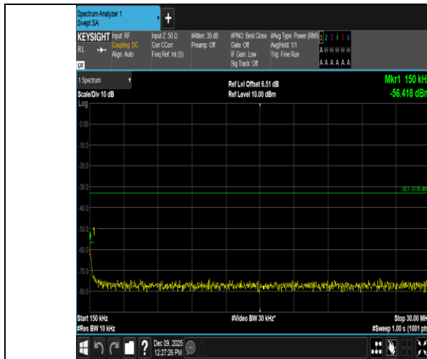
Band4-15MHz-QPSK-20325-1RB#74-0.15~30-PASS
