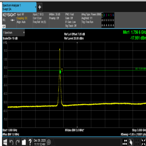
Band4-10MHz-16QAM-20350-50RB#0-1000~3000-PASS
