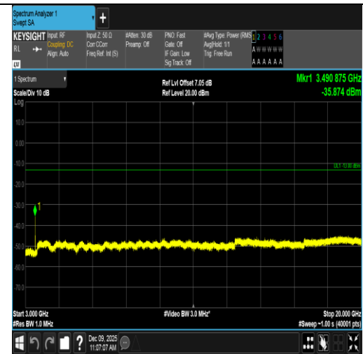
Band4-10MHz-16QAM-20350-1RB#0-3000~20000-PASS
