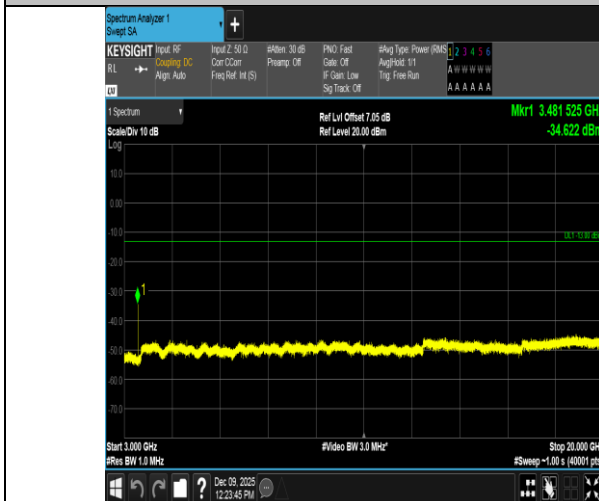
Band4-15MHz-QPSK-20325-1RB#0-3000~20000-PASS
