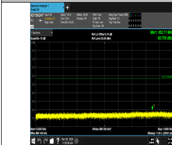
Band4-15MHz-QPSK-2025-1RB#0-30~1000-PASS
