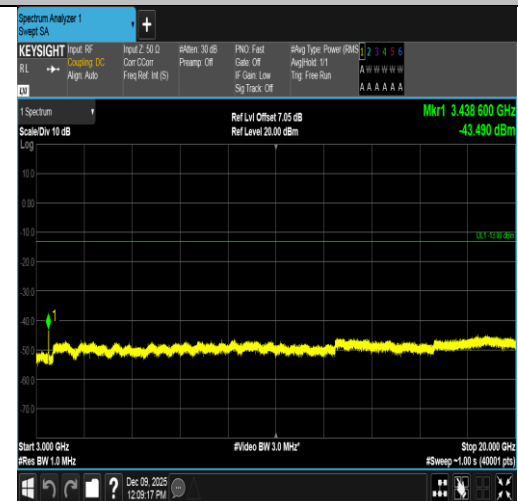
Band4-15MHz-16QAM-2025-75RB#0-3000~20000-PASS
