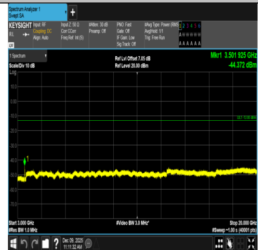
Band4-10MHz-16QAM-20350-50RB#0-3000~20000-PASS
