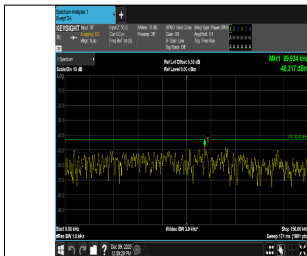
Band4-15MHz-QPSK-20175-1RB#0-0.009~0.15-PASS
