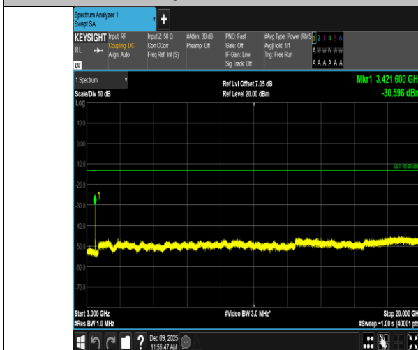
Band4-15MHz-QPSK-2025-1RB#0-3000~20000-PASS
