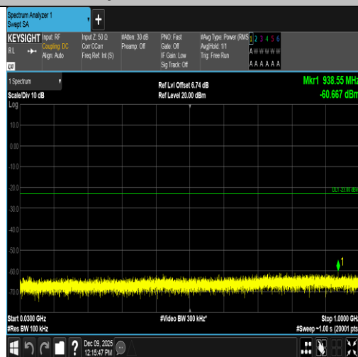
Band4-15MHz-16QAM-20175-1RB#74-30~1000-PASS
