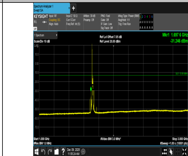
Band4-15MHz-QPSK-2025-1RB#0-1000~3000-PASS
