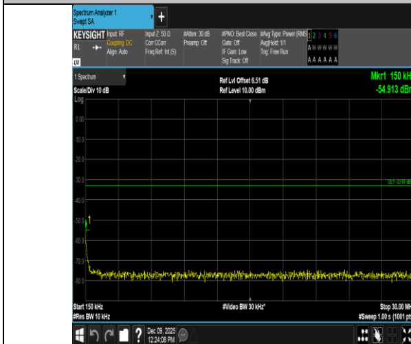
Band4-15MHz-16QAM-20325-1RB#0-0.15~30-PASS
