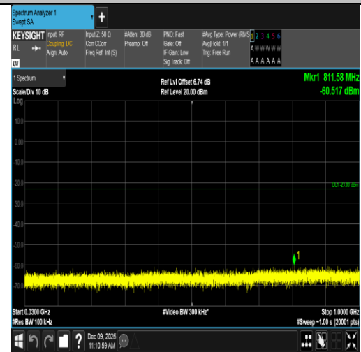
Band4-10MHz-16QAM-20350-50RB#0-30~1000-PASS
