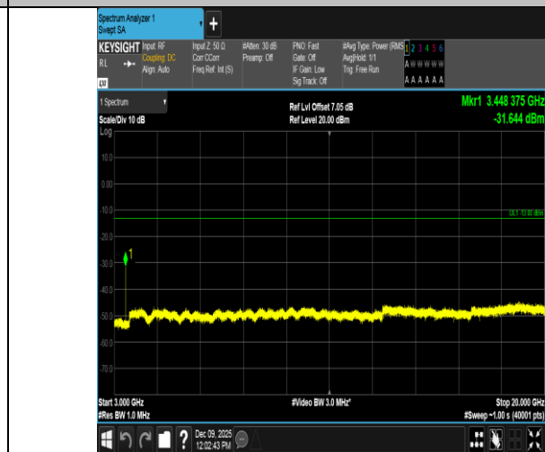
Band4-15MHz-QPSK-2025-1RB#74-3000~20000-PASS
