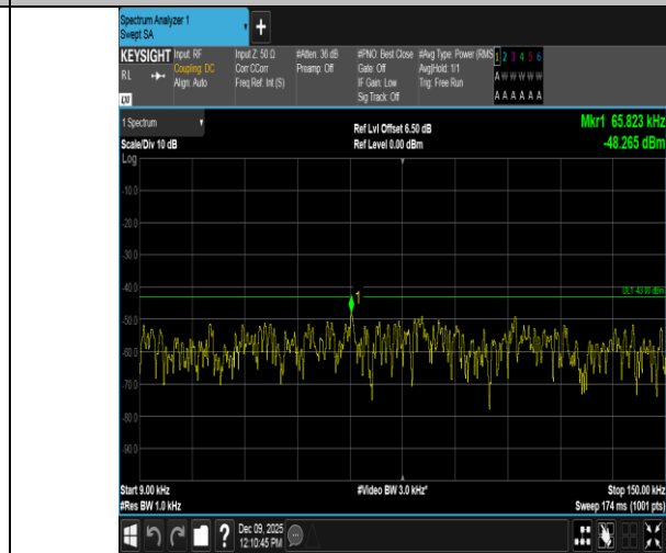
Band4-15MHz-16QAM-20175-1RB#0-0.009~0.15-PASS
