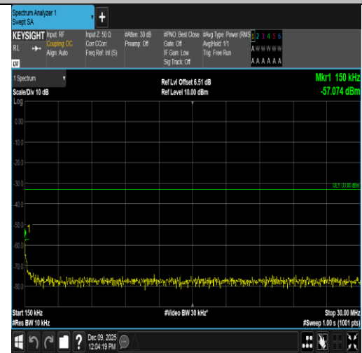
Band4-15MHz-16QAM-20025-1RB#74-0.15~30-PASS
