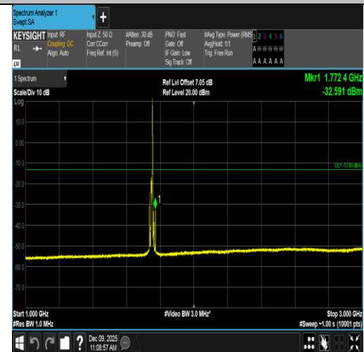
Band4-10MHz-16QAM-20350-1RB#49-1000~3000-PASS
