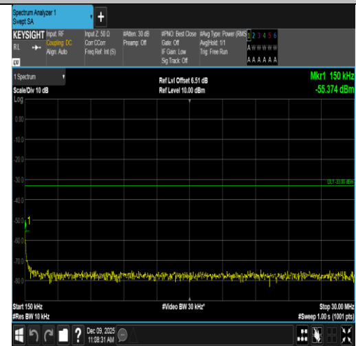
Band4-10MHz-16QAM-20350-1RB#49-0.15~30-PASS
