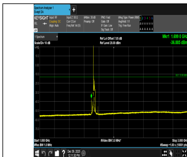
Band4-15MHz-16QAM-20175-1RB#0-1000~3000-PASS
