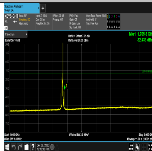
Band4-15MHz-16QAM-20175-1RB#74-1000~3000-PASS
