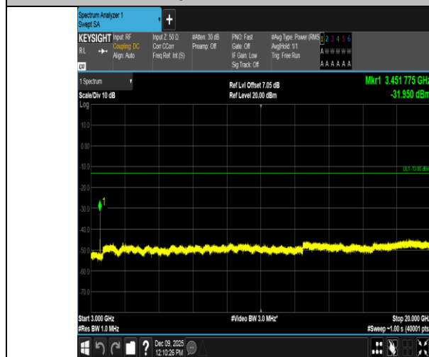
Band4-15MHz-QPSK-20175-1RB#0-3000~20000-PASS
