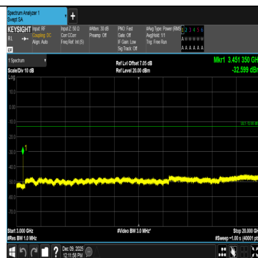
Band4-15MHz-16QAM-20175-1RB#0-3000~20000-PASS
