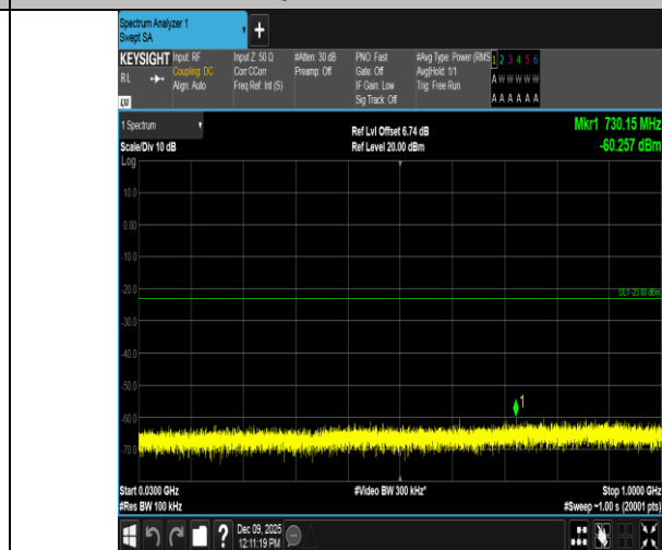
Band4-15MHz-16QAM-20175-1RB#0-30~1000-PASS
