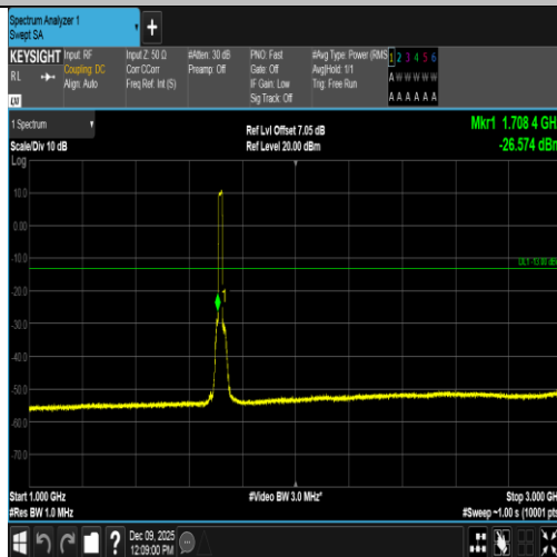
Band4-15MHz-16QAM-2025-75RB#0-1000~3000-PASS
