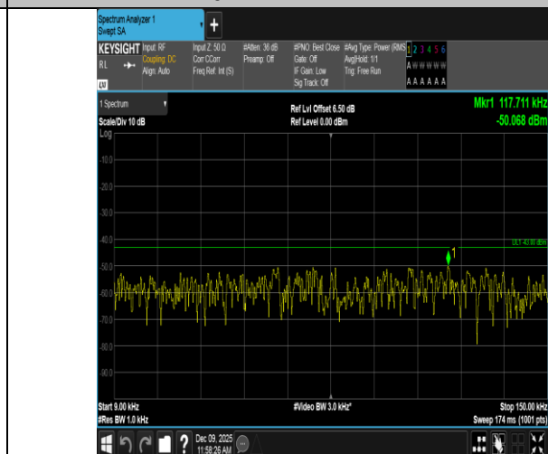
Band4-15MHz-QPSK-2025-1RB#74-0.009~0.15-PASS
