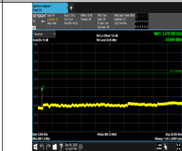
Band4-15MHz-QPSK-20175-1RB#74-3000~20000-PASS
