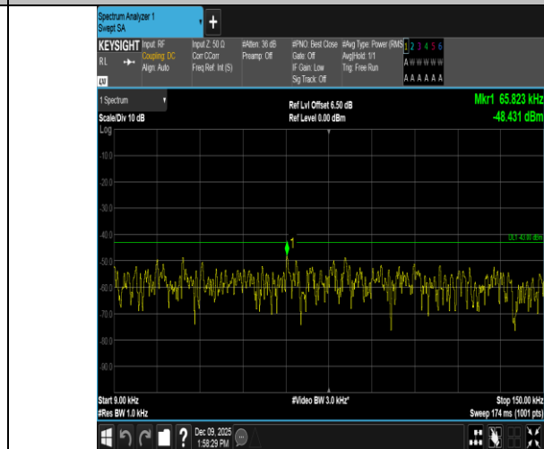
Band4-20MHz-QPSK-20300-1RB#99-0.009~0.15-PASS
