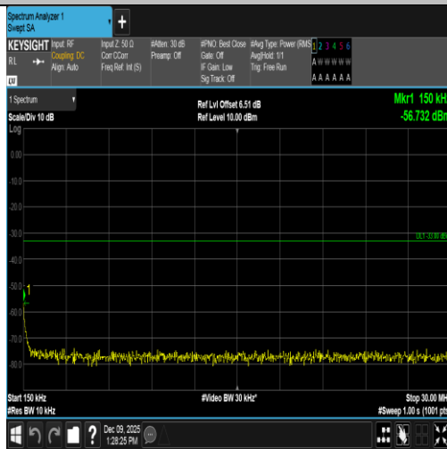
Band4-20MHz-16QAM-20050-100RB#0-0.15~30-PASS
