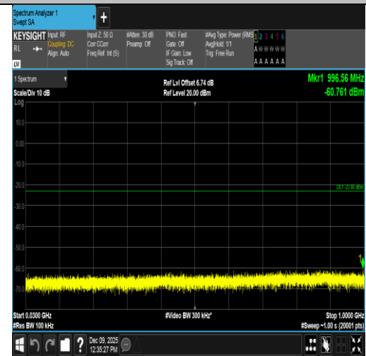
Band4-15MHz-16QAM-20325-75RB#0-30~1000-PASS
