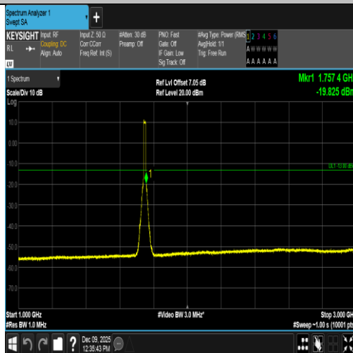
Band4-15MHz-16QAM-20325-75RB#0-1000~3000-PASS
