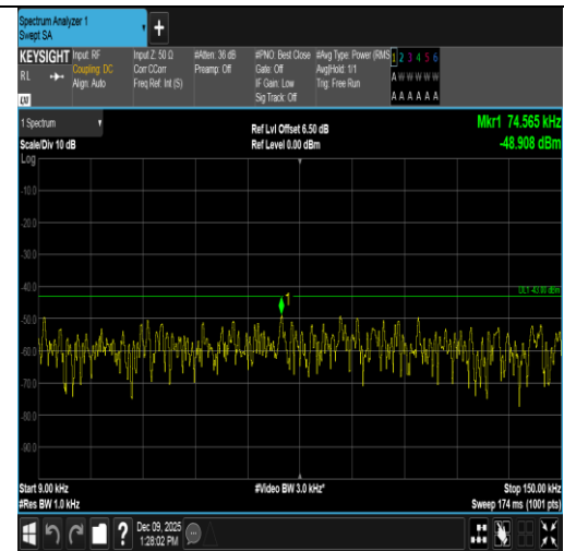
Band4-20MHz-16QAM-20050-100RB#0-0.009~0.15-PASS
