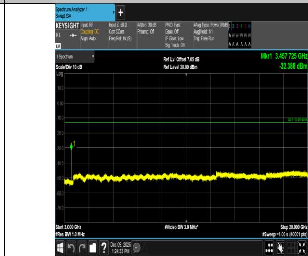
Band4-20MHz-QPSK-20050-1RB#99-3000~20000-PASS
