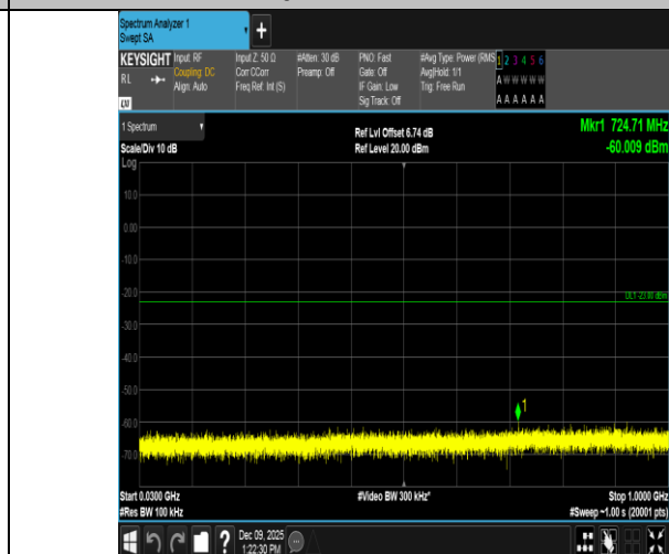
Band4-20MHz-16QAM-20050-1RB#0-30~1000-PASS
