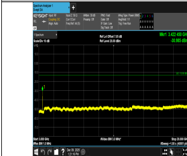
Band4-20MHz-QPSK-20050-1RB#0-3000~20000-PASS
