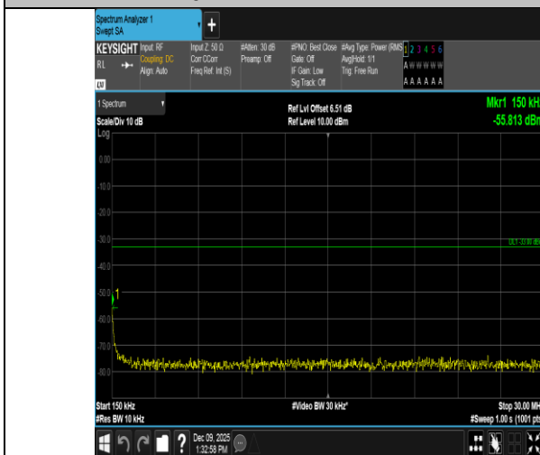
Band4-20MHz-16QAM-20175-1RB#0-0.15~30-PASS
