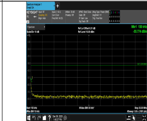
Band4-20MHz-QPSK-20175-100RB#0-0.15~30-PASS
