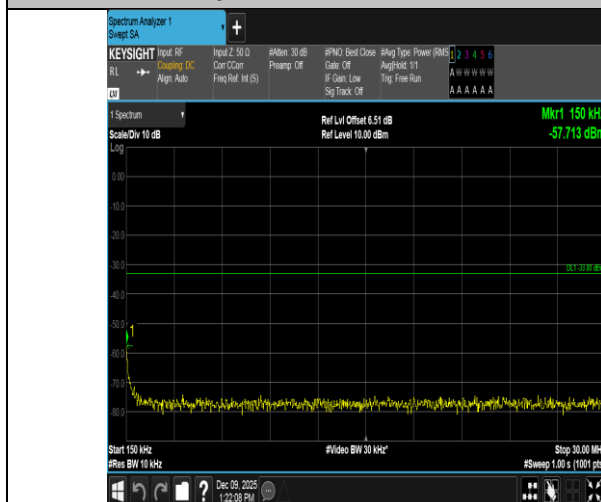
Band4-20MHz-16QAM-20050-1RB#0-0.15~30-PASS
