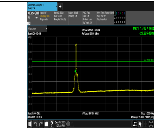
Band4-20MHz-QPSK-20050-100RB#0-1000~3000-PASS
