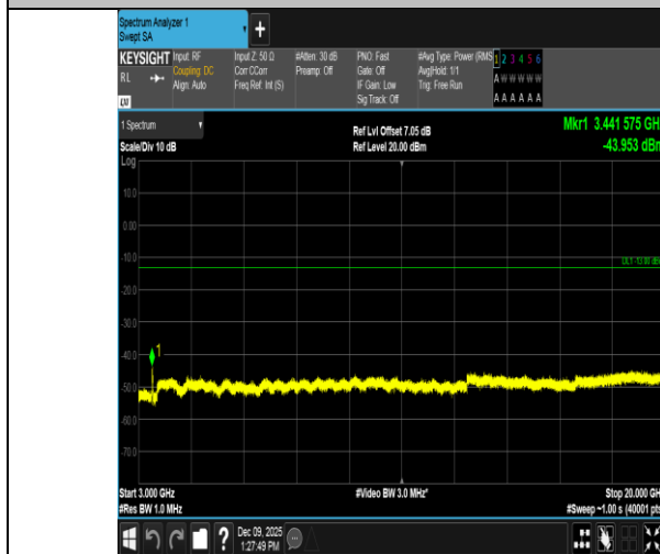
Band4-20MHz-QPSK-20050-100RB#0-3000~20000-PASS
