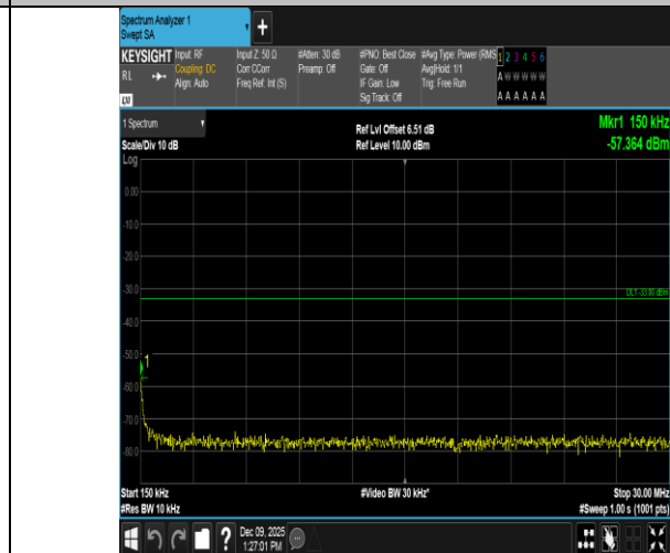
Band4-20MHz-QPSK-20050-100RB#0-0.15~30-PASS
