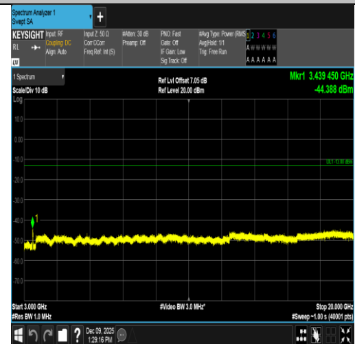
Band4-20MHz-16QAM-20050-100RB#0-3000~20000-PASS
