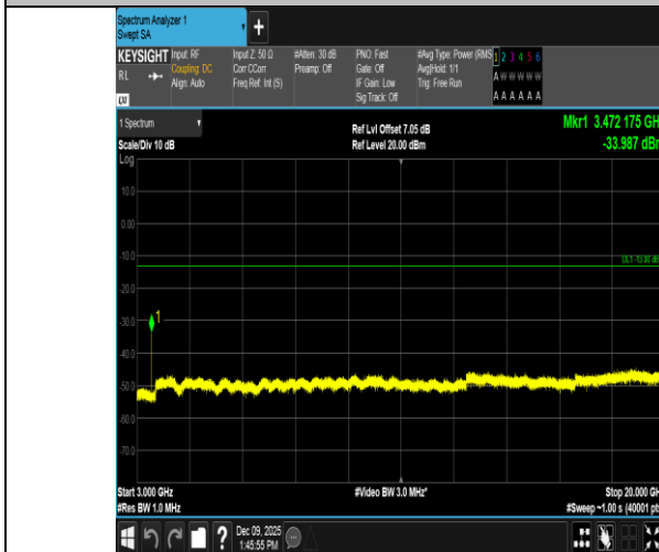
Band4-20MHz-QPSK-20300-1RB#0-3000~20000-PASS
