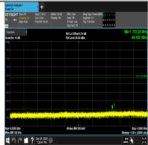
Band4-20MHz-16QAM-20050-100RB#0-30~1000-PASS
