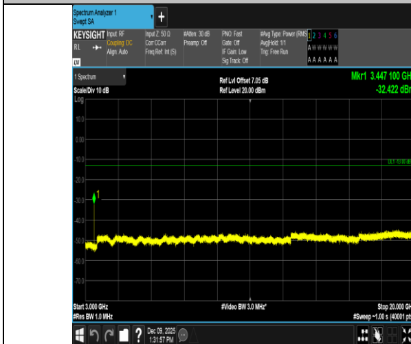
Band4-20MHz-QPSK-20175-1RB#0-3000~20000-PASS
