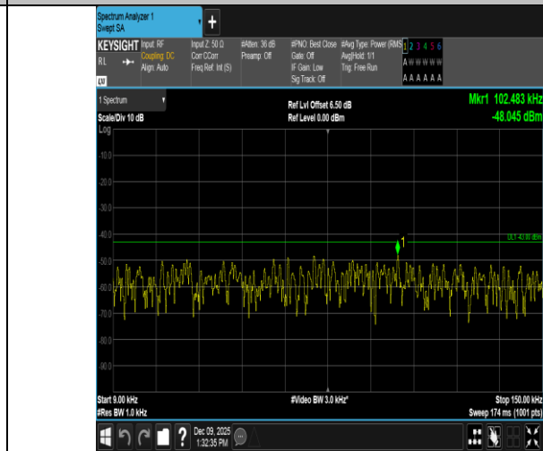
Band4-20MHz-16QAM-20175-1RB#0-0.009~0.15-PASS
