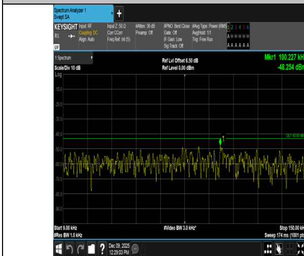
Band4-15MHz-16QAM-20325-1RB#74-0.009~0.15-PASS
