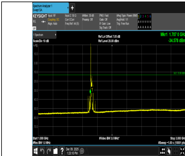
Band4-20MHz-16QAM-20050-1RB#0-1000~3000-PASS
