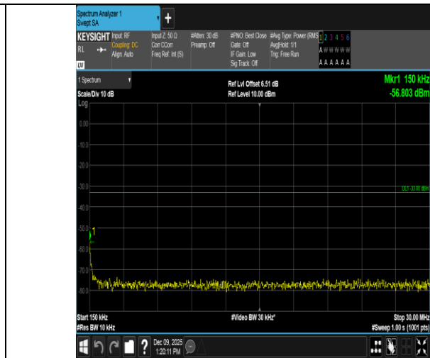
Band4-20MHz-QPSK-20050-1RB#0-0.15~30-PASS
