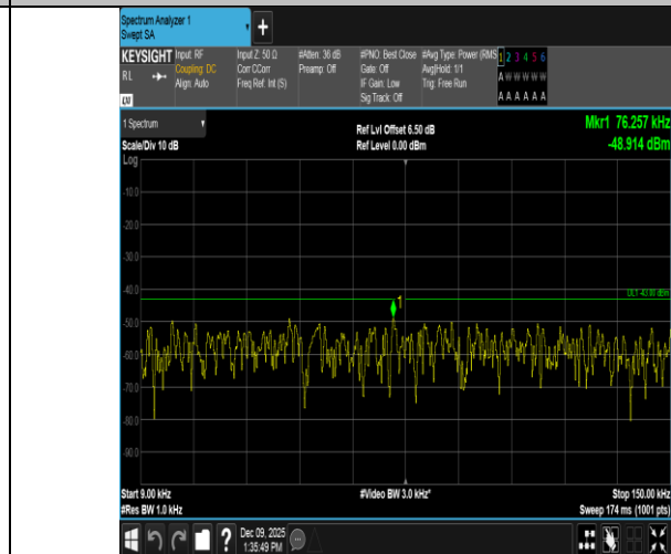
Band4-20MHz-QPSK-20175-1RB#99-0.009~0.15-PASS
