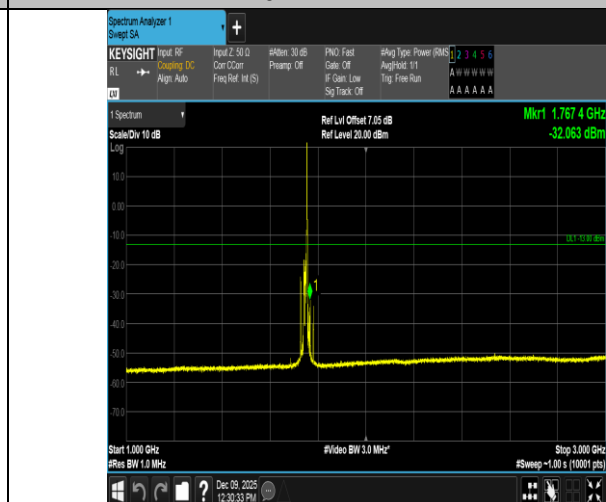
Band4-15MHz-16QAM-20325-1RB#74-1000~3000-PASS
