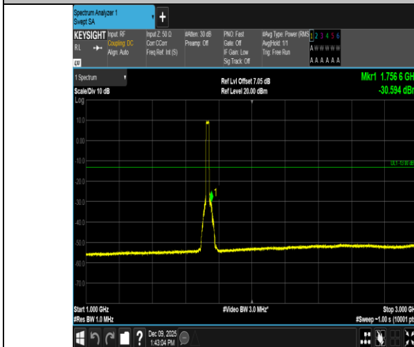
Band4-20MHz-16QAM-20175-100RB#0-1000~3000-PASS
