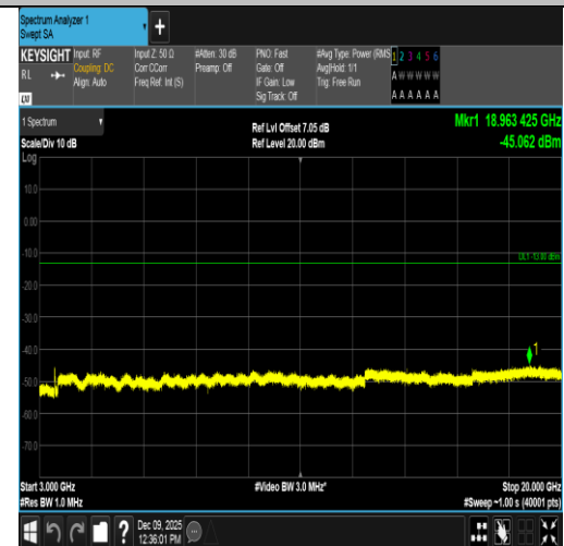
Band4-15MHz-16QAM-20325-75RB#0-3000~20000-PASS
