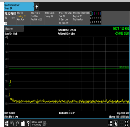
Band4-20MHz-16QAM-20050-1RB#99-0.15~30-PASS
