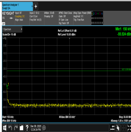
Band4-15MHz-16QAM-20325-75RB#0-0.15~30-PASS
