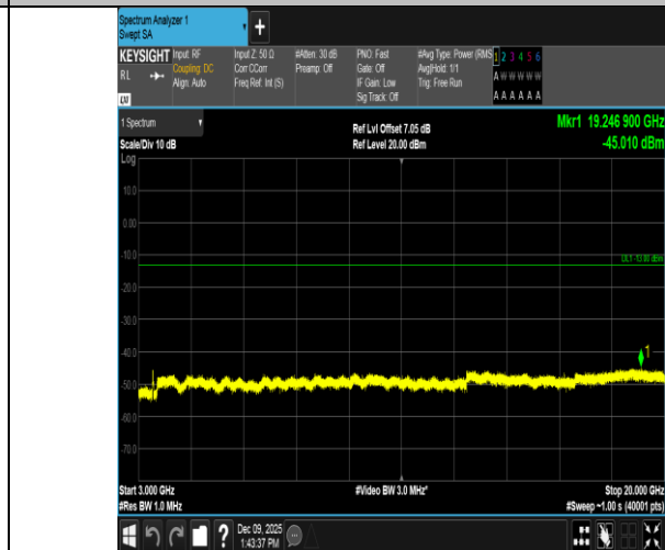
Band4-20MHz-16QAM-20175-100RB#0-3000~20000-PASS
