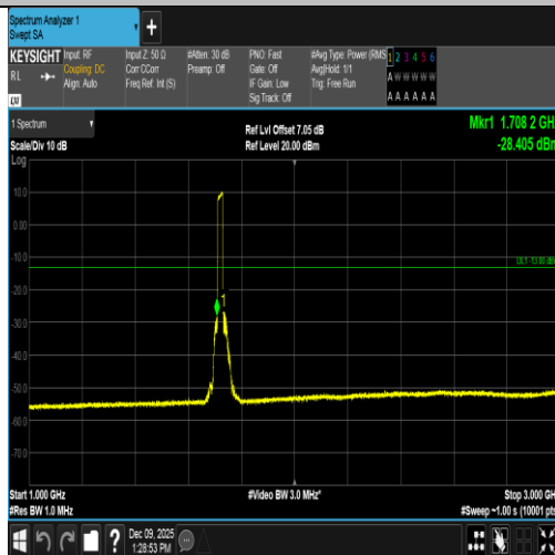
Band4-20MHz-16QAM-20050-100RB#0-1000~3000-PASS
