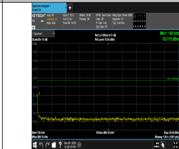
Band4-15MHz-16QAM-20325-1RB#74-0.15~30-PASS
