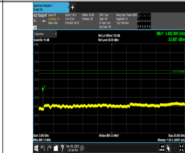
Band4-20MHz-QPSK-20175-1RB#99-3000~20000-PASS
