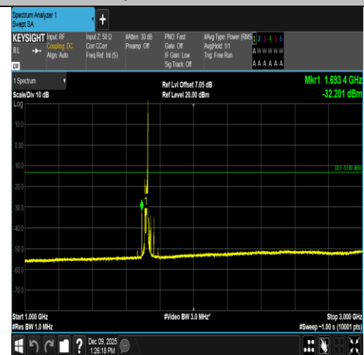
Band4-20MHz-16QAM-20050-1RB#99-1000~3000-PASS
