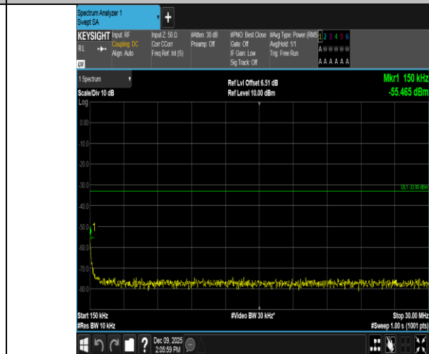
Band4-20MHz-QPSK-20300-100RB#0-0.15~30-PASS
