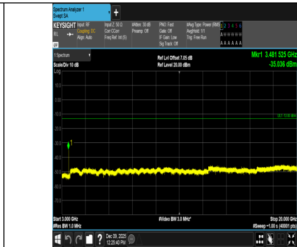
Band4-15MHz-16QAM-20325-1RB#0-3000~20000-PASS
