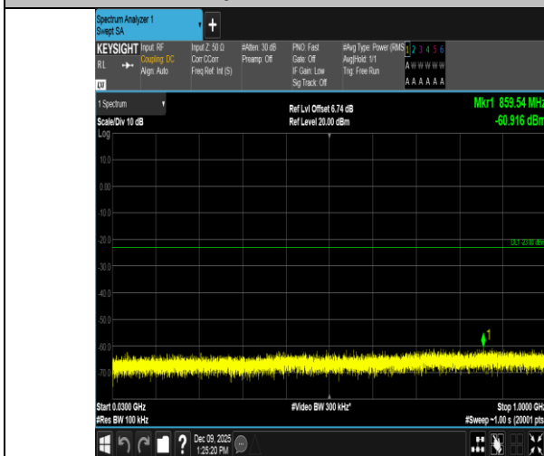
Band4-20MHz-16QAM-20050-1RB#99-30~1000-PASS
