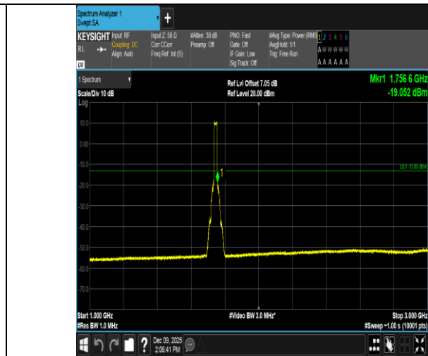
Band4-20MHz-QPSK-20300-100RB#0-1000~3000-PASS
