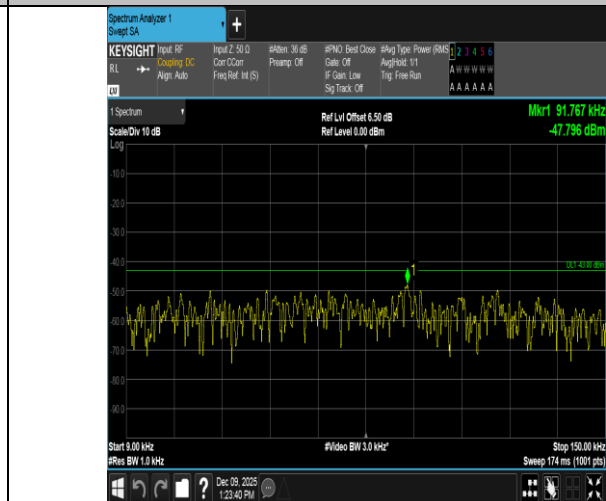
Band4-20MHz-QPSK-20050-1RB#99-0.009~0.15-PASS
