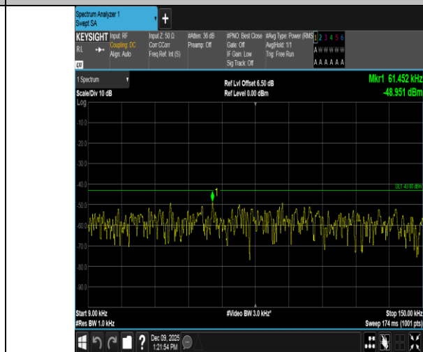
Band4-20MHz-16QAM-20050-1RB#0-0.009~0.15-PASS
