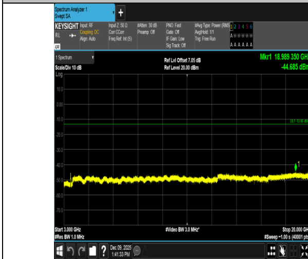
Band4-20MHz-QPSK-20175-100RB#0-3000~20000-PASS
