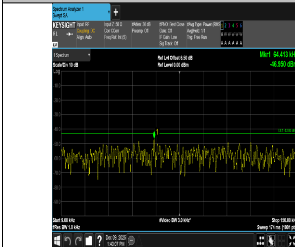
Band4-20MHz-QPSK-20175-100RB#0-0.009~0.15-PASS
