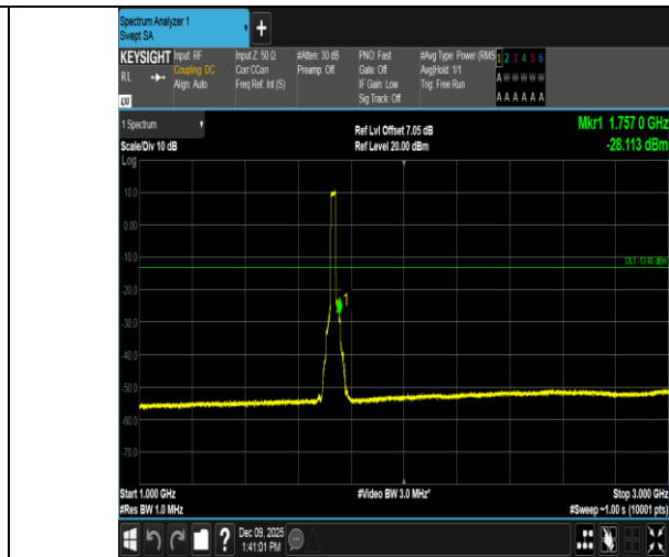
Band4-20MHz-QPSK-20175-100RB#0-1000~3000-PASS
