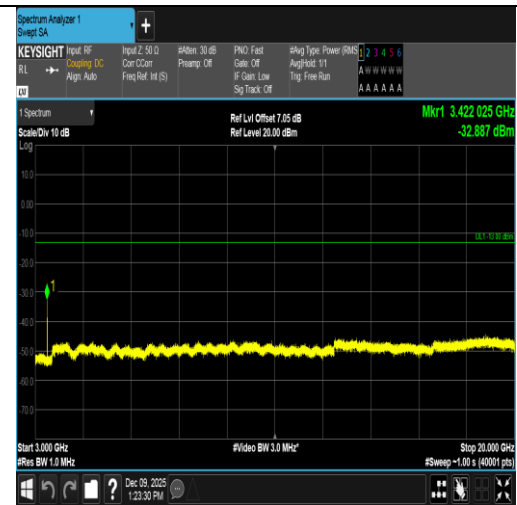
Band4-20MHz-16QAM-20050-1RB#0-3000~20000-PASS
