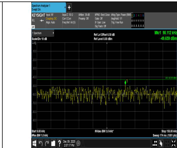
Band4-20MHz-16QAM-20300-100RB#0-0.009~0.15-PASS
