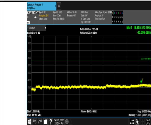
Band4-20MHz-16QAM-20300-100RB#0-3000~20000-PASS
