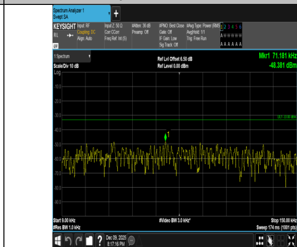
Band5-3MHz-16QAM-20635-15RB#0-0.009~0.15-PASS
