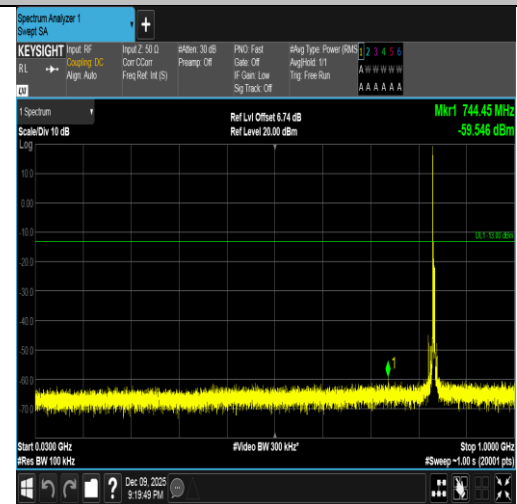
Band5-5MHz-16QAM-20525-1RB#0-30~1000-PASS
