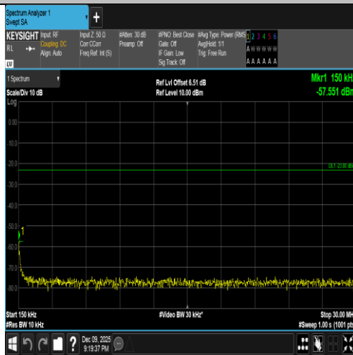
Band5-5MHz-16QAM-20525-1RB#0-0.15~30-PASS
