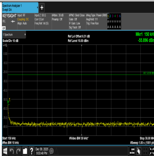
Band5-5MHz-16QAM-20425-1RB#0-0.15~30-PASS
