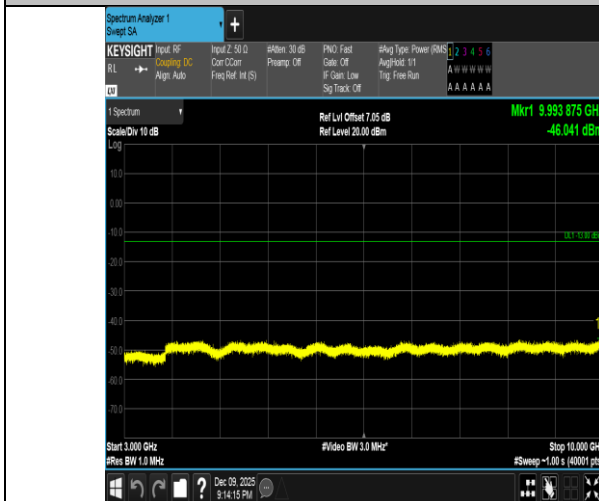
Band5-5MHz-16QAM-20425-1RB#24-3000~10000-PASS
