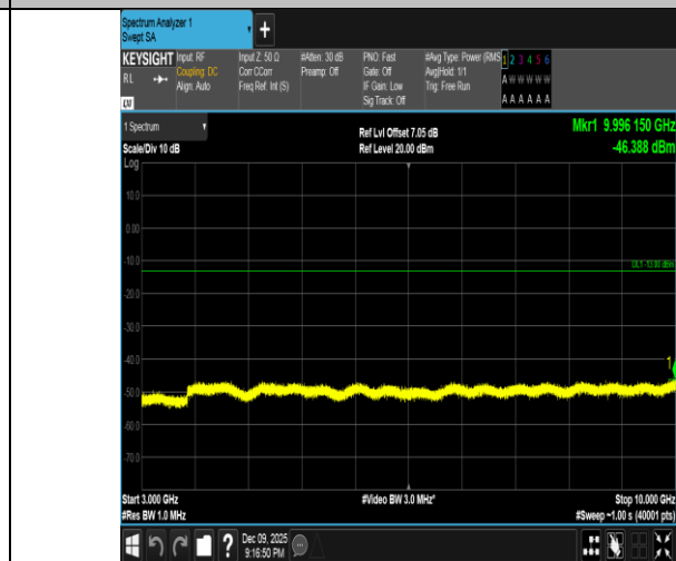
Band5-5MHz-16QAM-20425-25RB#0-3000~10000-PASS
