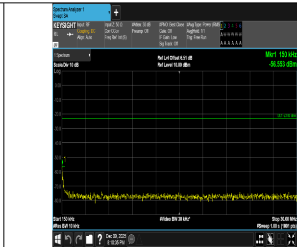
Band5-3MHz-16QAM-20635-1RB#14-0.15~30-PASS
