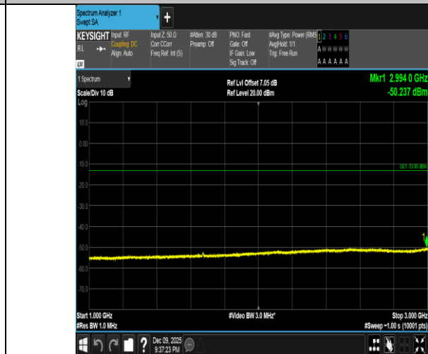
Band5-5MHz-QPSK-20525-25RB#0-1000~3000-PASS
