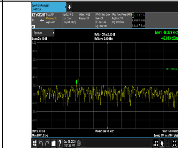
Band5-5MHz-QPSK-20525-1RB#24-0.009~0.15-PASS
