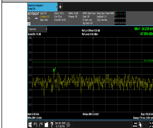
Band5-5MHz-QPSK-20525-1RB#0-0.009~0.15-PASS
