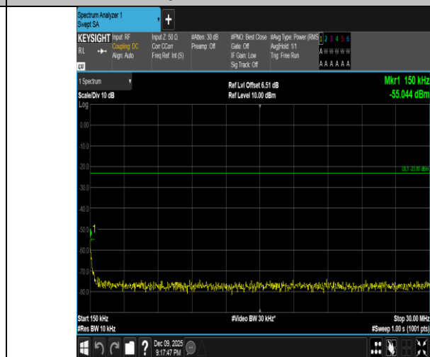
Band5-5MHz-QPSK-20525-1RB#0-0.15~30-PASS
