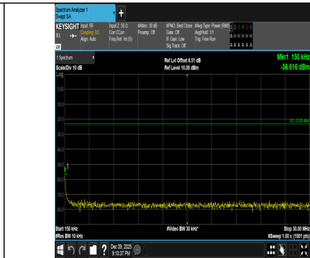
Band5-5MHz-16QAM-20425-1RB#24-0.15~30-PASS
