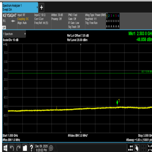
Band5-5MHz-16QAM-20525-1RB#0-1000~3000-PASS
