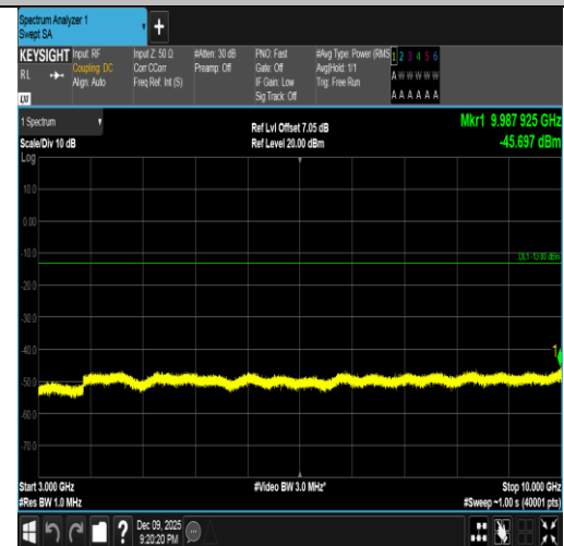
Band5-5MHz-16QAM-20525-1RB#0-3000~10000-PASS
