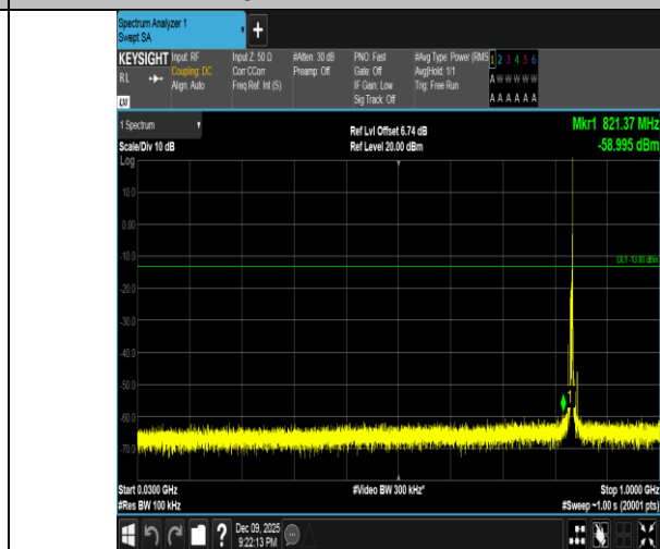
Band5-5MHz-QPSK-20525-1RB#24-30~1000-PASS
