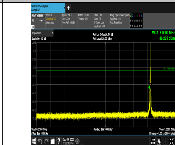
Band5-5MHz-QPSK-20425-1RB#24-30~1000-PASS
