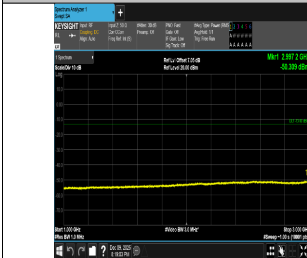
Band5-3MHz-16QAM-20635-15RB#0-1000~3000-PASS
