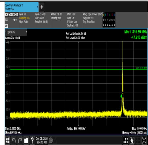
Band5-5MHz-16QAM-20425-1RB#0-30~1000-PASS
