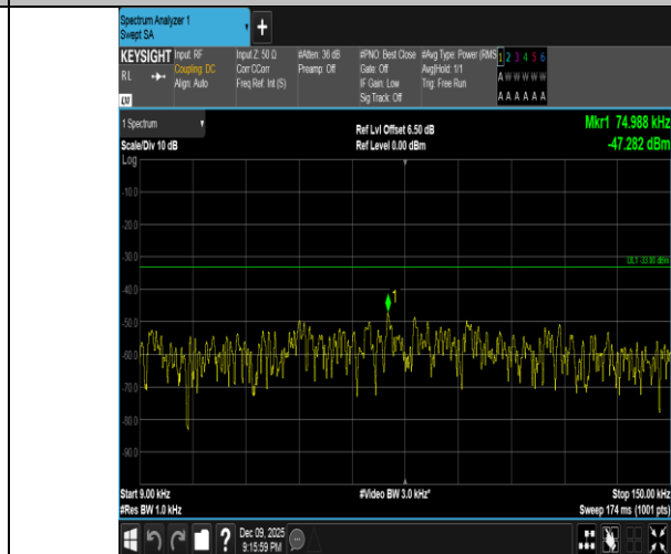
Band5-5MHz-16QAM-20425-25RB#0-0.009~0.15-PASS
