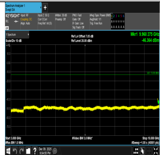
Band5-5MHz-16QAM-20425-1RB#0-3000~10000-PASS
