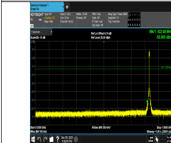
Band5-5MHz-QPSK-20525-25RB#0-30~1000-PASS
