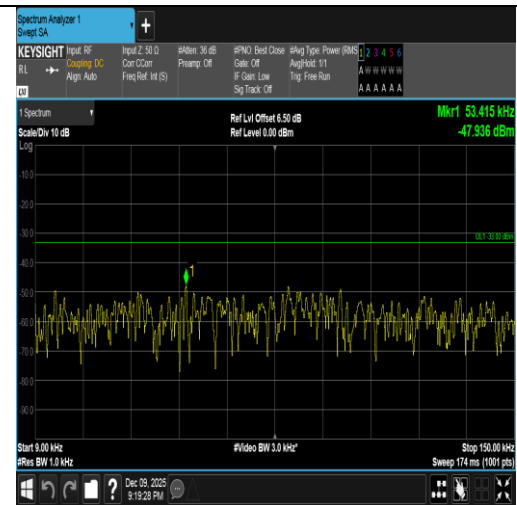
Band5-5MHz-16QAM-20525-1RB#0-0.009~0.15-PASS
