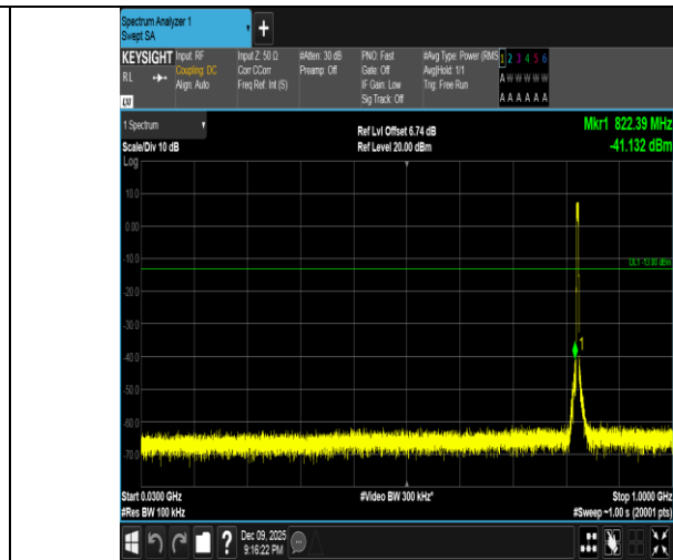
Band5-5MHz-16QAM-20425-25RB#0-30~1000-PASS
