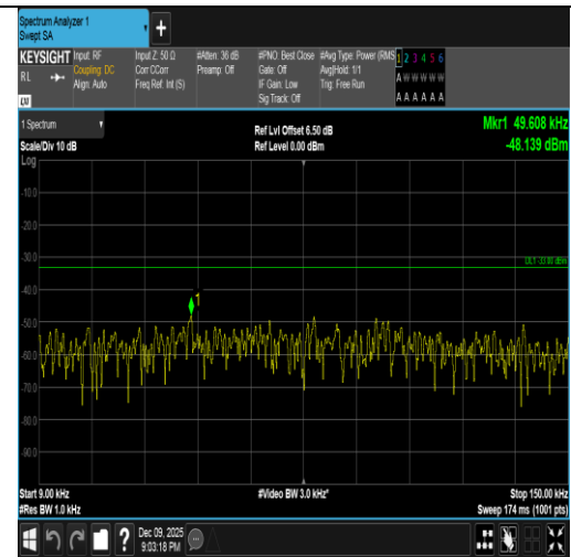
Band5-5MHz-16QAM-20425-1RB#0-0.009~0.15-PASS
