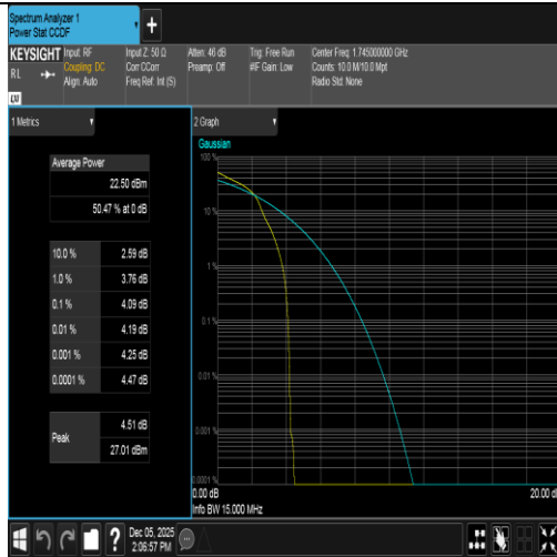
Band66-15MHz-16QAM-132322-1RB#0-PASS
