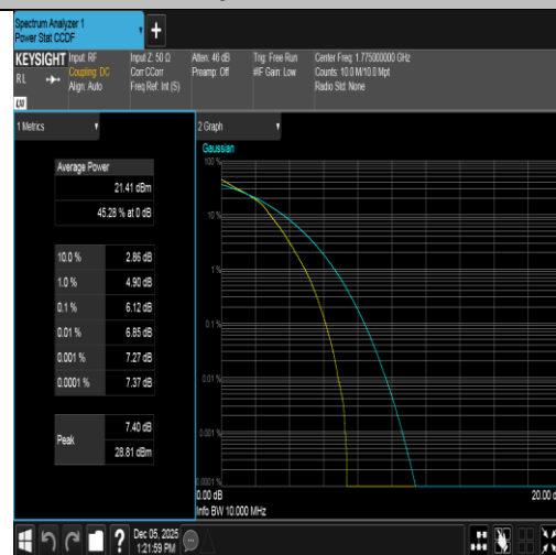
Band66-10MHz-16QAM-132622-50RB#0-PASS
