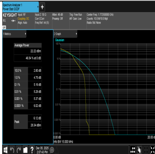
Band66-15MHz-16QAM-132597-1RB#0-PASS
