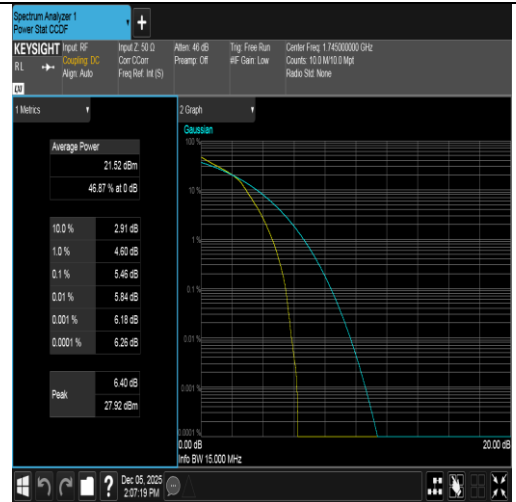
Band66-15MHz-16QAM-132322-75RB#0-PASS
