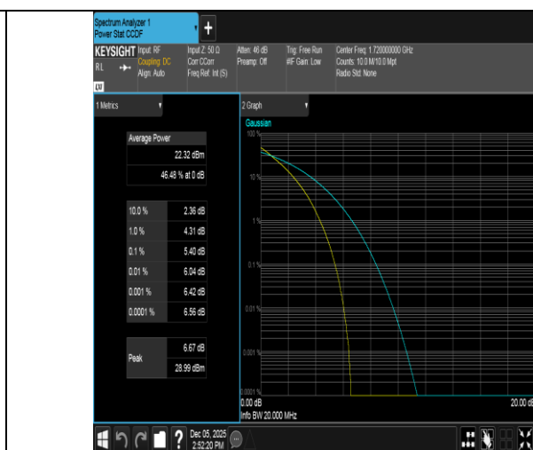
Band66-20MHz-QPSK-132072-100RB#0-PASS
