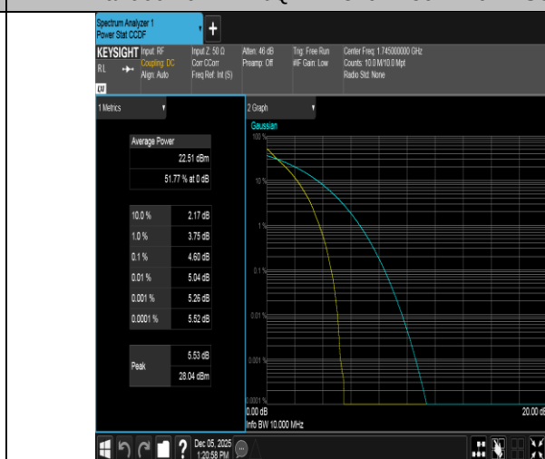
Band66-10MHz-QPSK-132322-50RB#0-PASS
