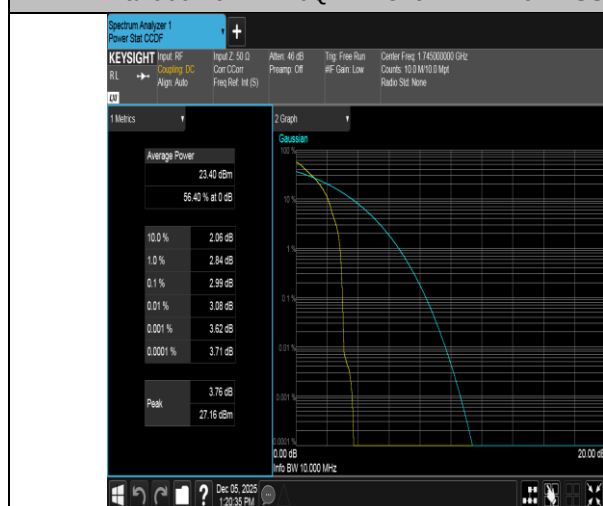
Band66-10MHz-QPSK-132322-1RB#0-PASS
