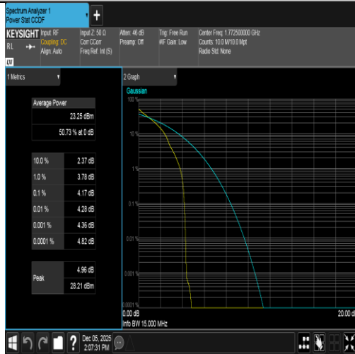
Band66-15MHz-QPSK-132597-1RB#0-PASS
