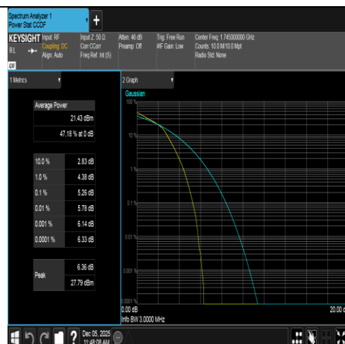
Band66-3MHz-16QAM-132322-15RB#0-PASS
