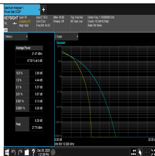
Band66-10MHz-16QAM-132322-50RB#0-PASS
