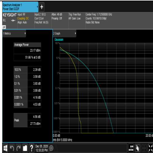
Band66-5MHz-QPSK-131997-1RB#0-PASS
