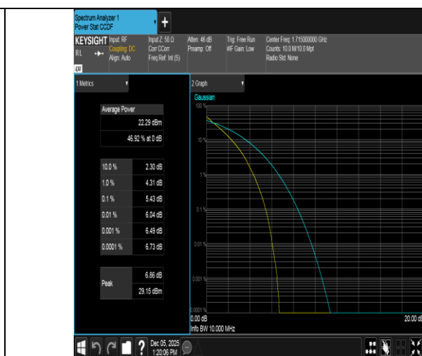
Band66-10MHz-QPSK-132022-50RB#0-PASS
