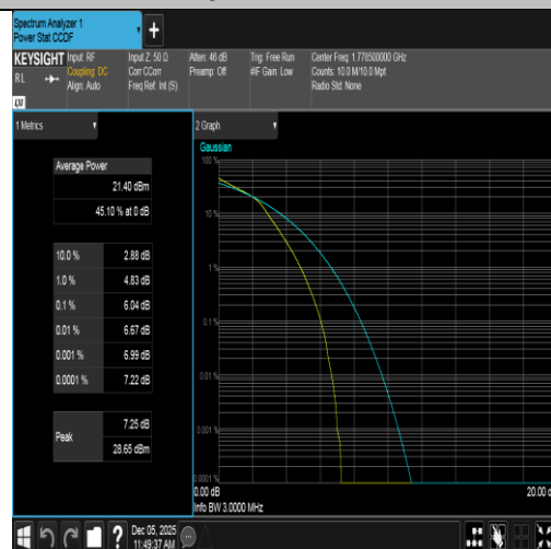
Band66-3MHz-16QAM-132657-15RB#0-PASS
