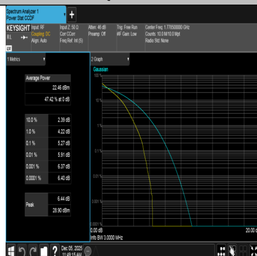
Band66-3MHz-QPSK-132657-15RB#0-PASS
