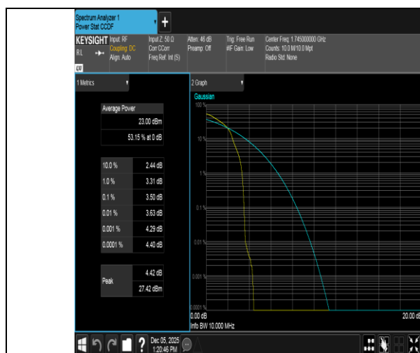
Band66-10MHz-16QAM-132322-1RB#0-PASS
