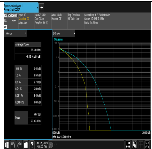
Band66-15MHz-QPSK-132047-75RB#0-PASS
