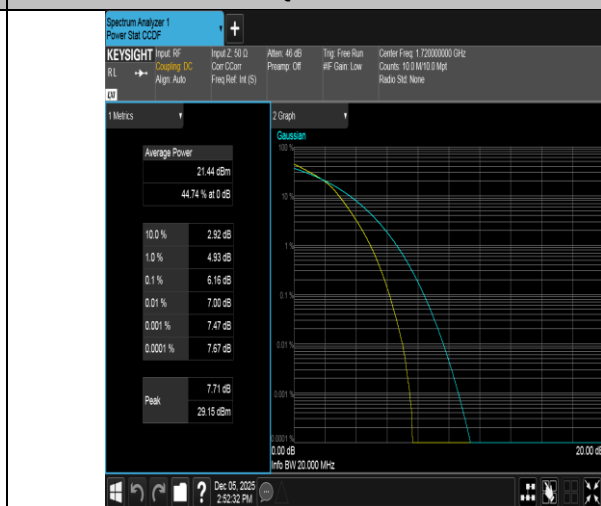
Band66-20MHz-16QAM-132072-100RB#0-PASS
