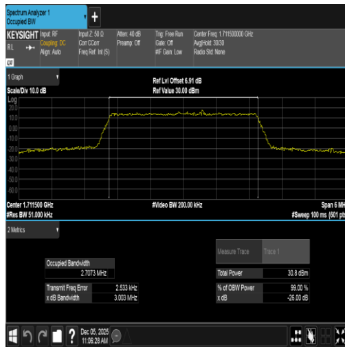
Band66-3MHz-QPSK-131987-15RB#0-PASS
