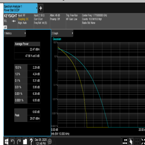
Band66-10MHz-QPSK-132622-50RB#0-PASS
