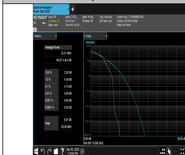
Band66-10MHz-16QAM-132022-1RB#0-PASS
