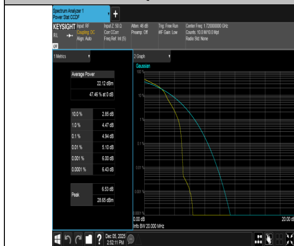
Band66-20MHz-16QAM-132072-1RB#0-PASS
