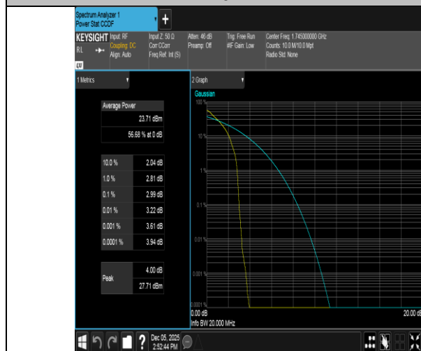
Band66-20MHz-QPSK-132322-1RB#0-PASS
