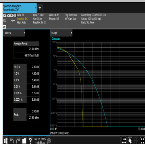
Band66-3MHz-16QAM-132657-1RB#0-PASS
