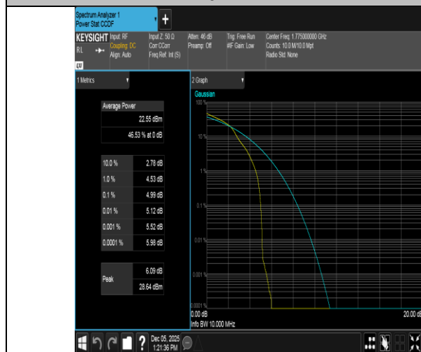
Band66-10MHz-16QAM-132622-1RB#0-PASS
