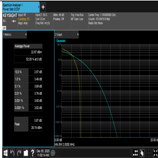
Band66-1.4MHz-16QAM-132322-1RB#0-PASS
