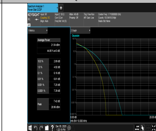
Band66-10MHz-16QAM-132022-50RB#0-PASS
