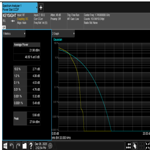
Band66-20MHz-16QAM-132322-1RB#0-PASS
