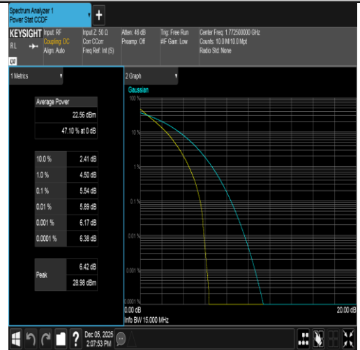
Band66-15MHz-QPSK-132597-75RB#0-PASS
