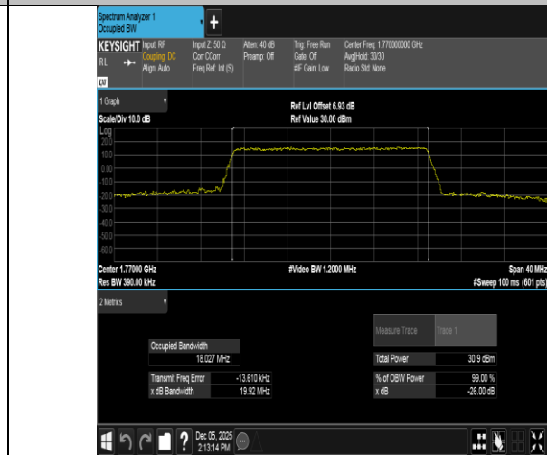
Band66-20MHz-16QAM-132572-100RB#0-PASS
