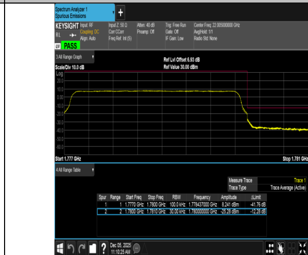
Band66-3MHz-16QAM-132657-15RB#0-PASS
