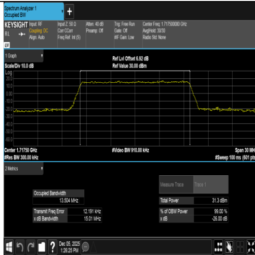
Band66-15MHz-QPSK-132047-75RB#0-PASS
