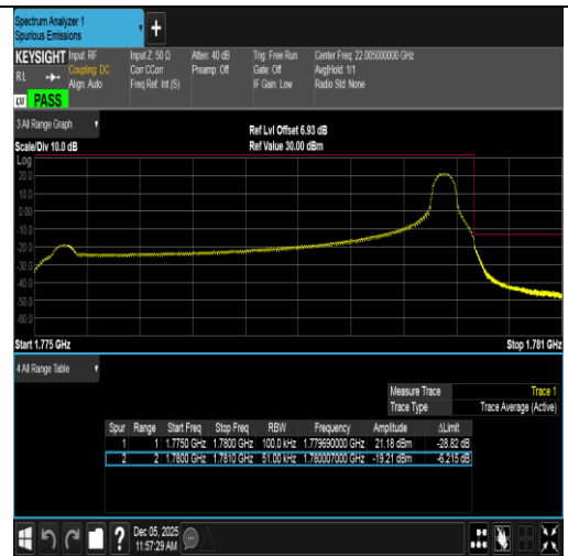
Band66-5MHz-QPSK-132647-1RB#24-PASS
