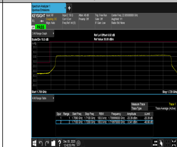
Band66-10MHz-16QAM-132022-50RB#0-PASS
