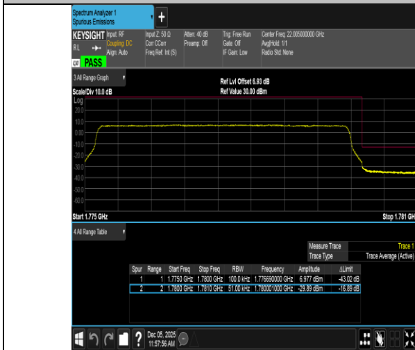
Band66-5MHz-QPSK-132647-25RB#0-PASS
