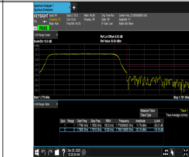
Band66-1.4MHz-16QAM-132665-6RB#0-PASS
