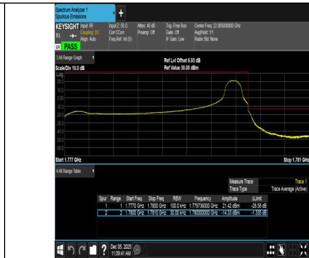
Band66-3MHz-QPSK-132657-1RB#14-PASS
