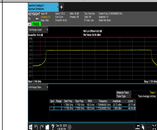
Band66-15MHz-16QAM-132047-75RB#0-PASS
