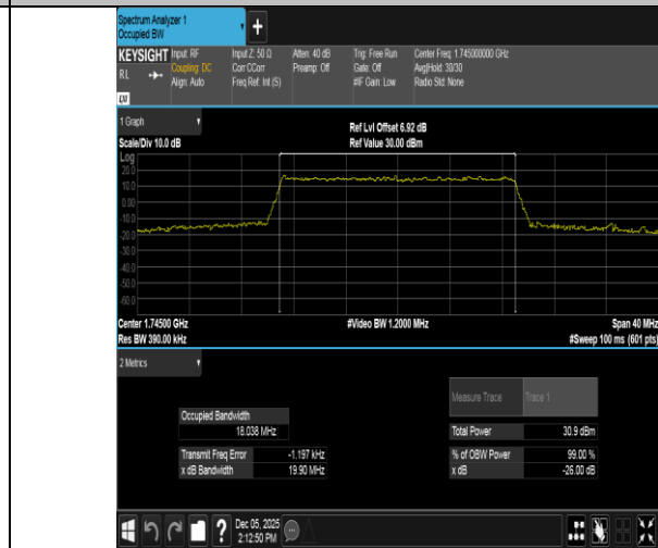
Band66-20MHz-16QAM-132322-100RB#0-PASS
