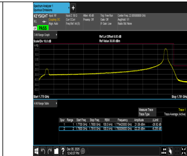
Band66-10MHz-QPSK-132622-1RB#49-PASS
