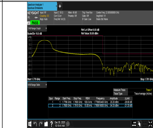
Band66-1.4MHz-16QAM-132665-1RB#0-PASS
