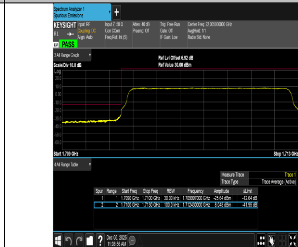
Band66-3MHz-16QAM-131987-15RB#0-PASS
