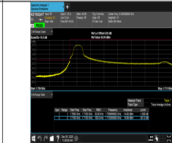
Band66-3MHz-16QAM-131987-1RB#0-PASS
