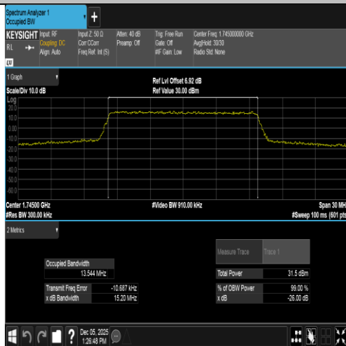
Band66-15MHz-QPSK-132322-75RB#0-PASS
