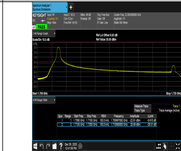
Band66-10MHz-16QAM-132022-1RB#0-PASS
