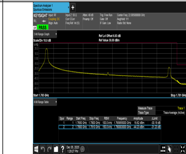
Band66-15MHz-16QAM-132597-1RB#0-PASS
