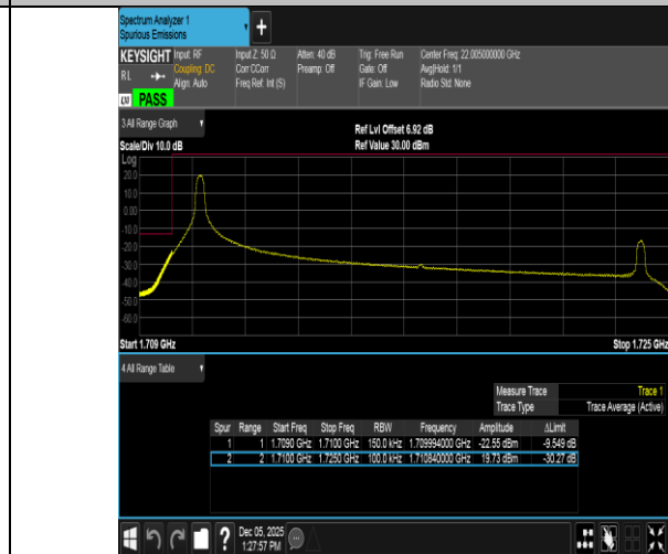
Band66-15MHz-16QAM-132047-1RB#0-PASS
