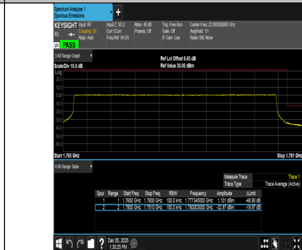
Band66-15MHz-16QAM-132597-75RB#0-PASS
