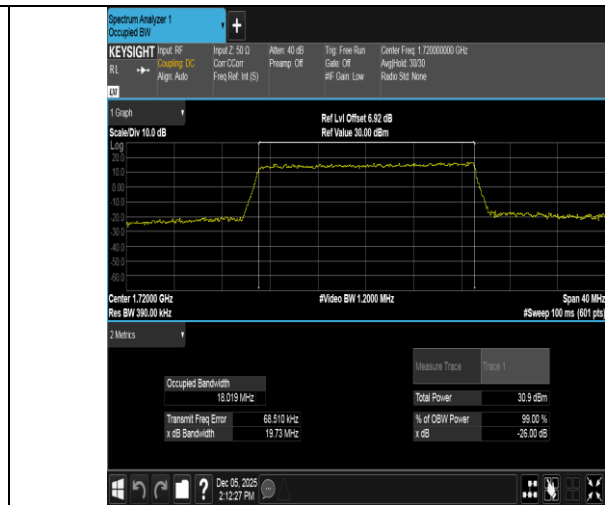
Band66-20MHz-16QAM-132072-100RB#0-PASS
