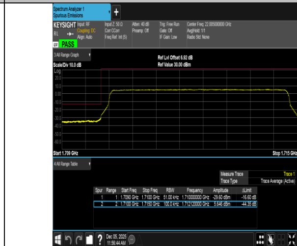
Band66-5MHz-16QAM-131997-25RB#0-PASS
