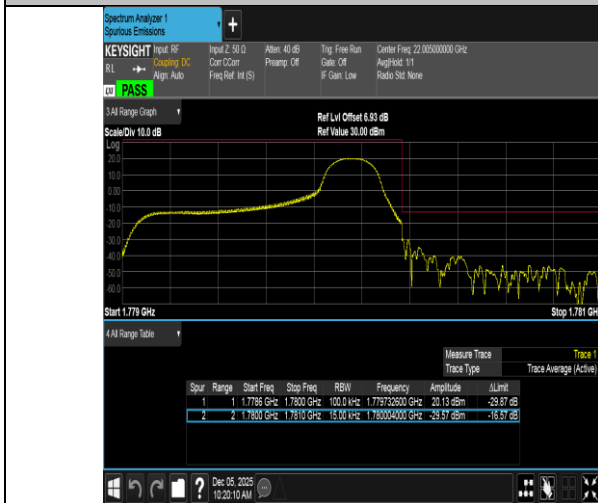
Band66-1.4MHz-16QAM-132665-1RB#5-PASS
