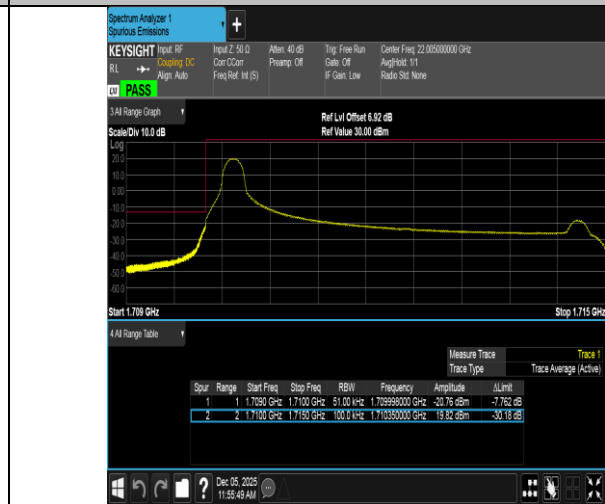
Band66-5MHz-16QAM-131997-1RB#0-PASS
