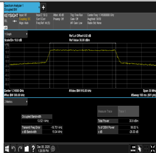
Band66-15MHz-16QAM-132322-75RB#0-PASS
