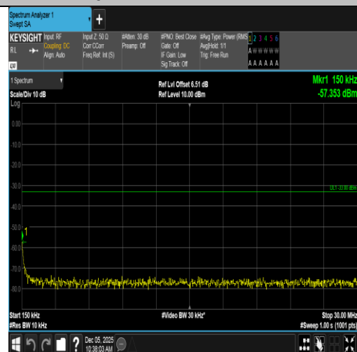
Band66-1.4MHz-QPSK-132665-6RB#0-0.15~30-PASS
