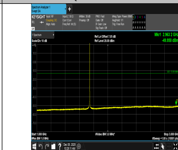
Band66-1.4MHz-QPSK-132322-1RB#0-1000~3000-PASS
