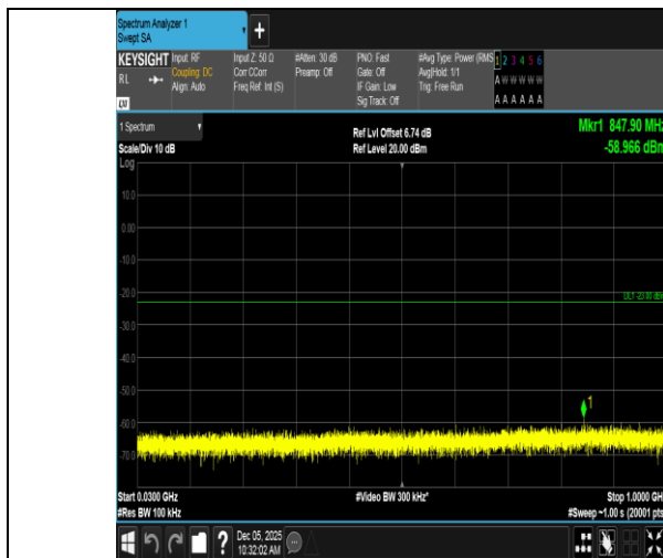
Band66-1.4MHz-QPSK-132322-6RB#0-30~1000-PASS
