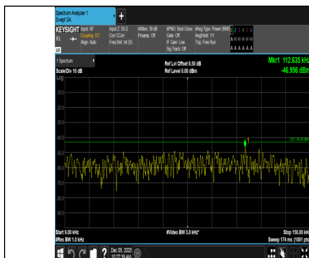
Band66-1.4MHz-QPSK-132322-1RB#0-0.009~0.15-PASS
