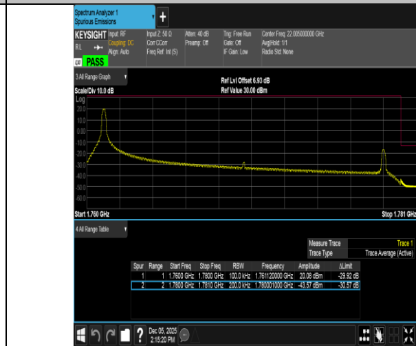
Band66-20MHz-16QAM-132572-1RB#0-PASS
