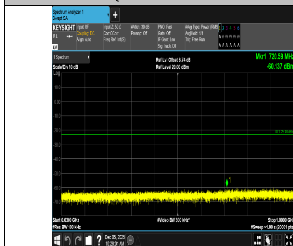
Band66-1.4MHz-QPSK-132322-1RB#0-30~1000-PASS
