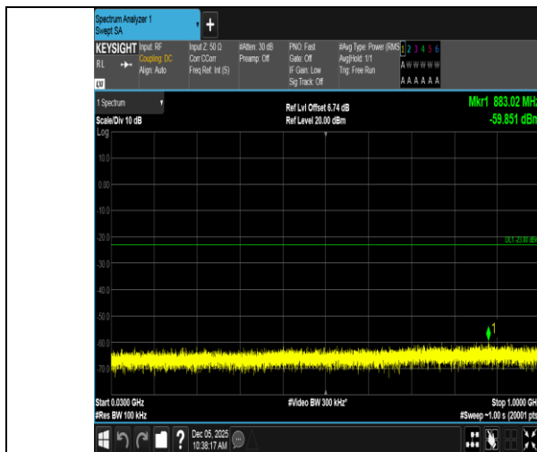
Band66-1.4MHz-QPSK-132665-6RB#0-30~1000-PASS
