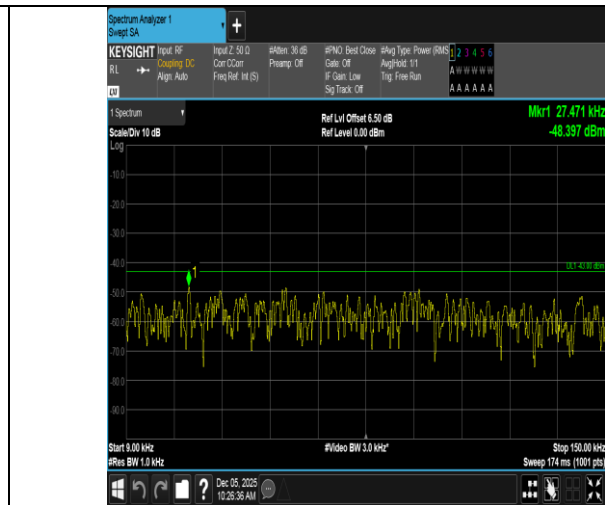
Band66-1.4MHz-16QAM-131979-6RB#0-0.009~0.15-PASS
