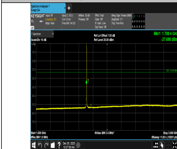
Band66-1.4MHz-16QAM-131979-6RB#0-1000~3000-PASS
