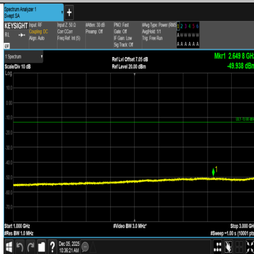
Band66-1.4MHz-QPSK-132665-1RB#5-1000~3000-PASS
