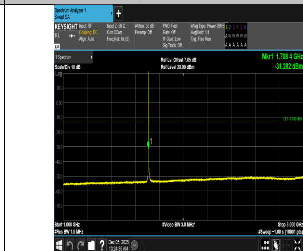
Band66-1.4MHz-16QAM-131979-1RB#5-1000~3000-PASS
