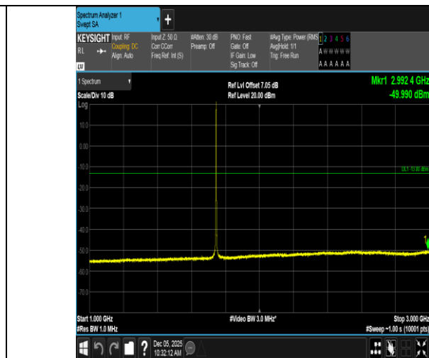
Band66-1.4MHz-QPSK-132322-6RB#0-1000~3000-PASS
