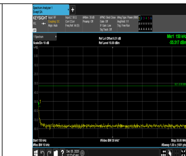
Band66-1.4MHz-QPSK-132322-1RB#0-0.15~30-PASS
