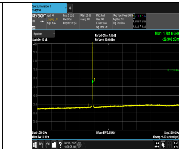
Band66-1.4MHz-QPSK-132665-6RB#0-1000~3000-PASS
