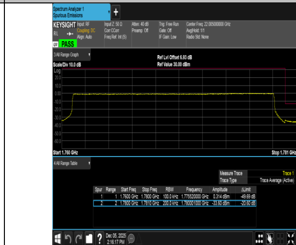
Band66-20MHz-16QAM-132572-100RB#0-PASS
