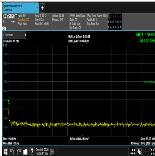
Band66-1.4MHz-QPSK-132665-1RB#5-0.15~30-PASS
