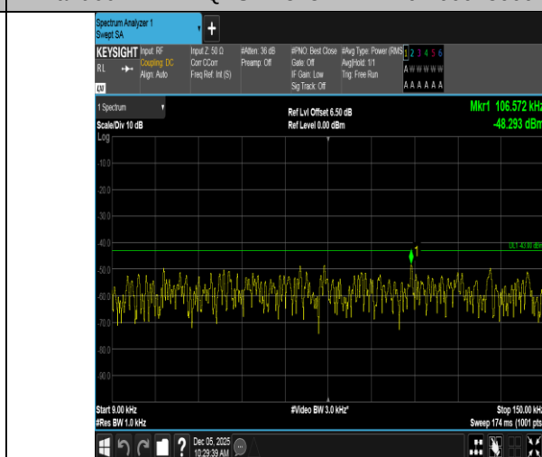
Band66-1.4MHz-QPSK-132322-1RB#5-0.009~0.15-PASS
