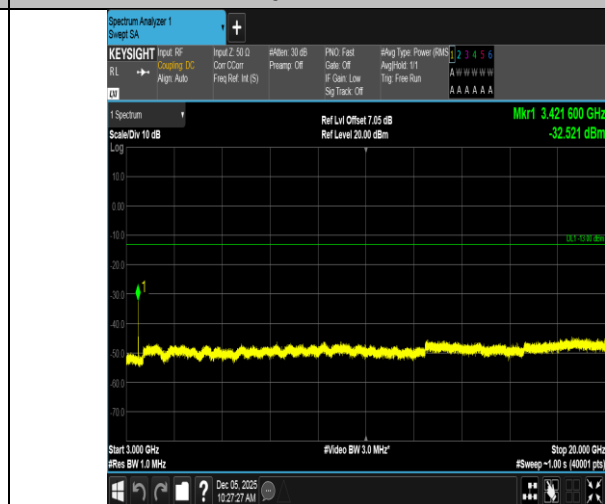
Band66-1.4MHz-16QAM-131979-6RB#0-3000~20000-PASS
