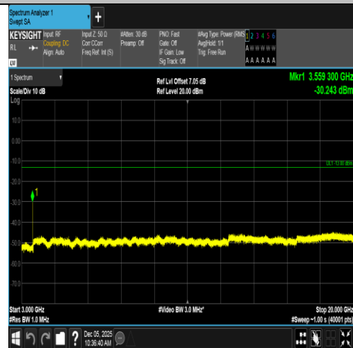
Band66-1.4MHz-QPSK-132665-1RB#5-3000~20000-PASS
