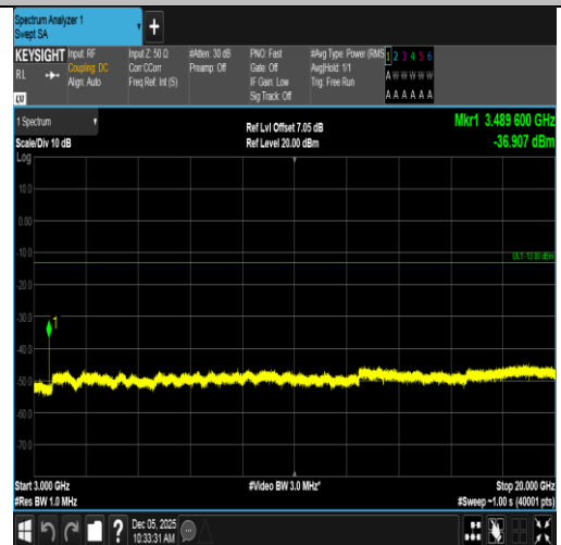
Band66-1.4MHz-16QAM-132322-6RB#0-3000~20000-PASS
