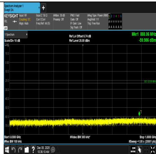
Band66-1.4MHz-QPSK-132665-1RB#5-30~1000-PASS
