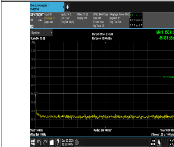
Band66-10MHz-16QAM-132322-50RB#0-0.15~30-PASS
