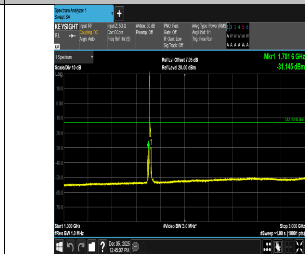
Band66-10MHz-QPSK-132022-1RB#0-1000~3000-PASS
