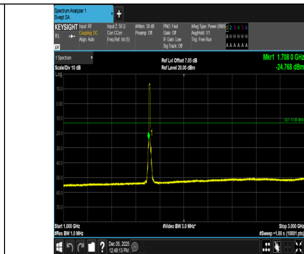
Band66-10MHz-QPSK-132022-50RB#0-1000~3000-PASS
