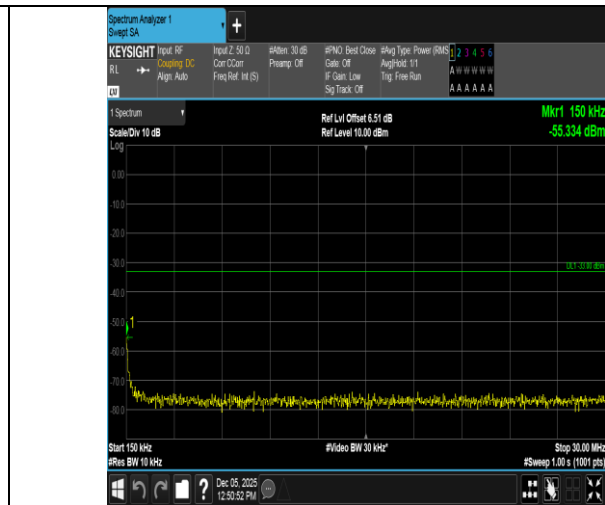
Band66-10MHz-QPSK-132322-1RB#0-0.15~30-PASS
