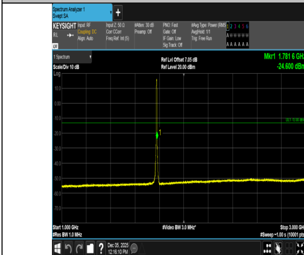
Band66-5MHz-16QAM-132647-25RB#0-1000~3000-PASS
