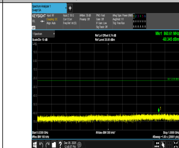
Band66-10MHz-16QAM-132022-1RB#0-30~1000-PASS
