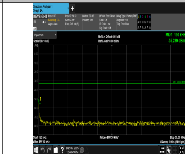
Band66-10MHz-QPSK-132022-50RB#0-0.15~30-PASS
