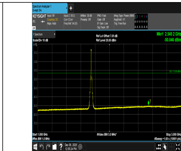
Band66-10MHz-QPSK-132322-50RB#0-1000~3000-PASS
