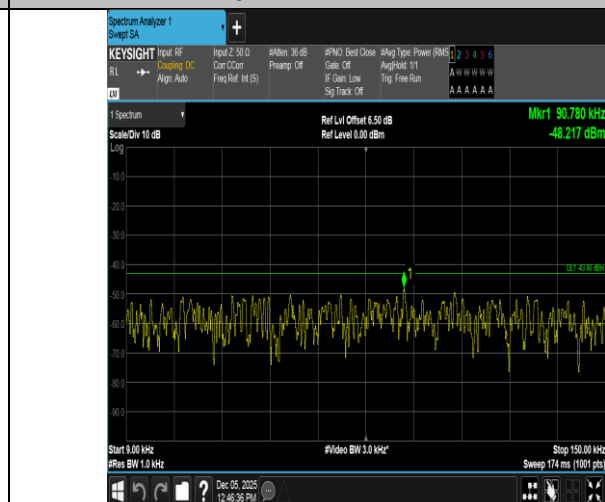
Band66-10MHz-QPSK-132022-1RB#49-0.009~0.15-PASS
