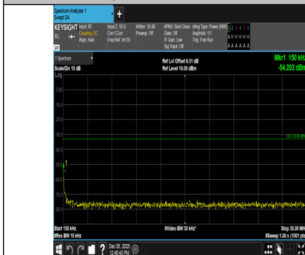
Band66-10MHz-16QAM-132022-1RB#0-0.15~30-PASS
