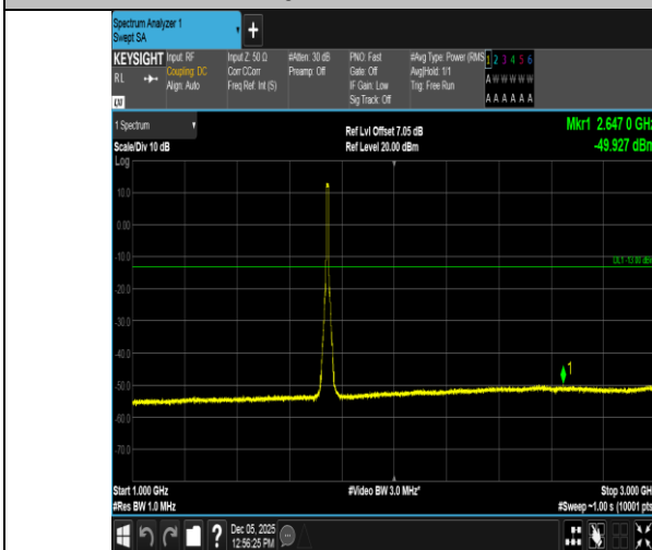
Band66-10MHz-16QAM-132322-50RB#0-1000~3000-PASS
