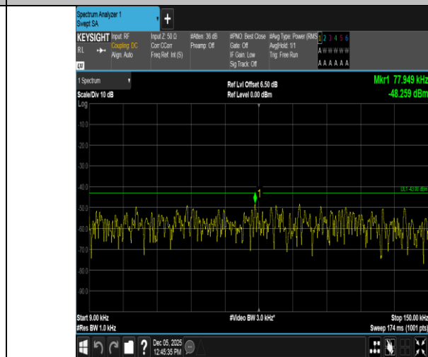
Band66-10MHz-16QAM-132022-1RB#0-0.009~0.15-PASS
