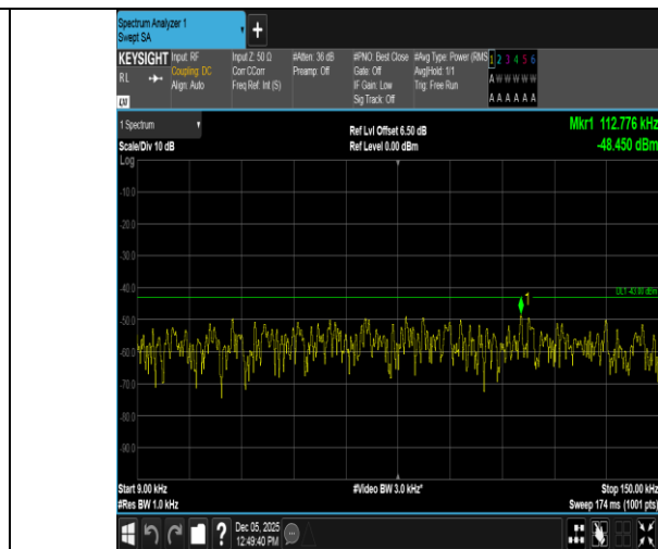
Band66-10MHz-16QAM-132022-50RB#0-0.009~0.15-PASS
