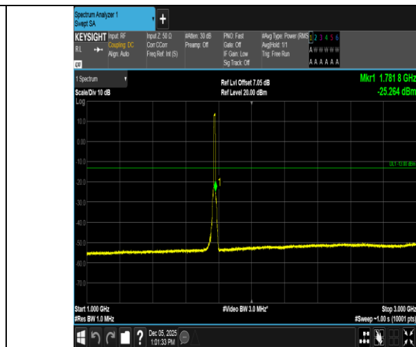
Band66-10MHz-QPSK-132622-50RB#0-1000~3000-PASS
