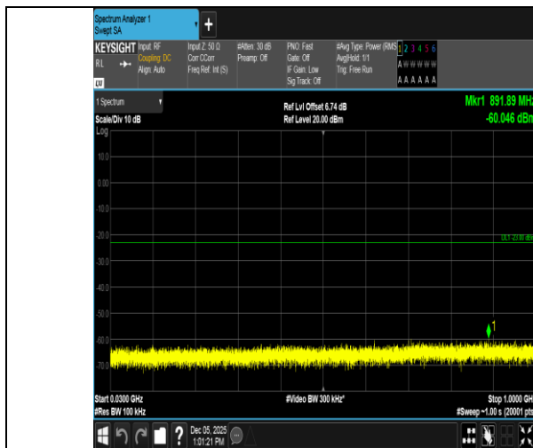
Band66-10MHz-QPSK-132622-50RB#0-30~1000-PASS
