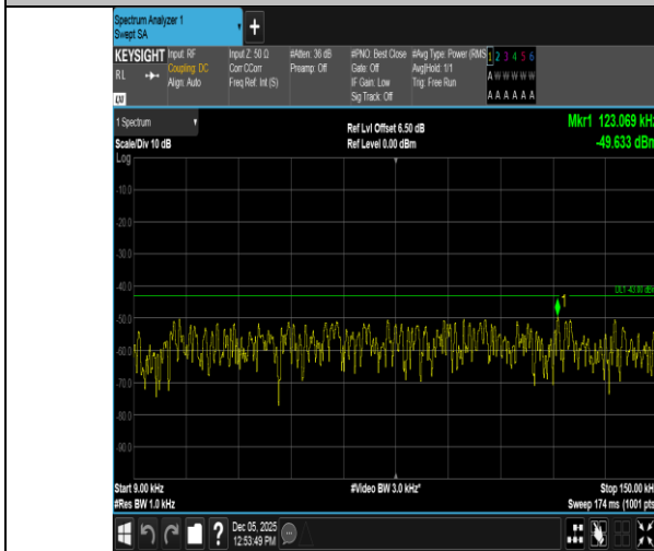
Band66-10MHz-16QAM-132322-1RB#49-0.009~0.15-PASS
