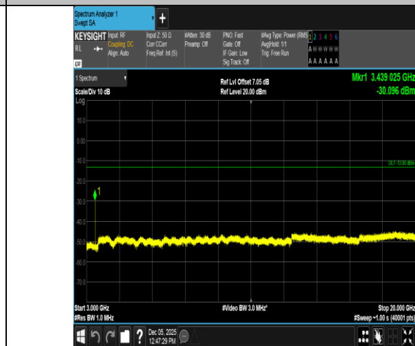
Band66-10MHz-QPSK-132022-1RB#49-3000~20000-PASS
