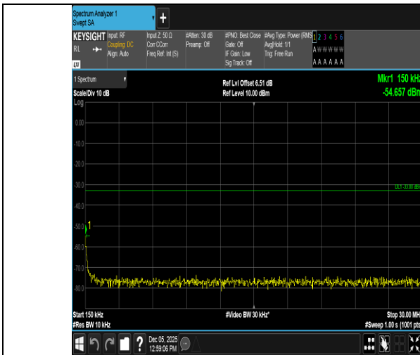
Band66-10MHz-QPSK-132622-1RB#49-0.15~30-PASS
