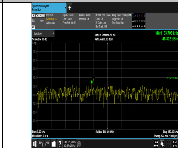
Band66-10MHz-16QAM-132622-1RB#0-0.009~0.15-PASS
