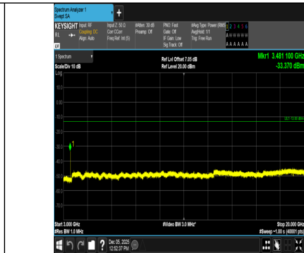
Band66-10MHz-16QAM-132322-1RB#0-3000~20000-PASS
