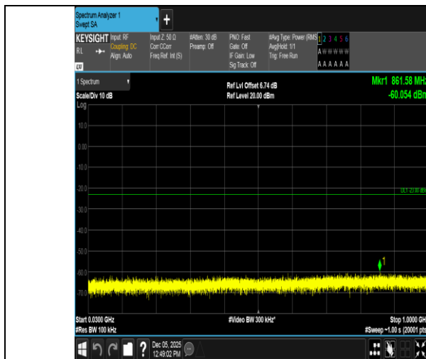
Band66-10MHz-QPSK-132022-50RB#0-30~1000-PASS
