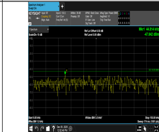
Band66-10MHz-QPSK-132322-1RB#49-0.009~0.15-PASS
