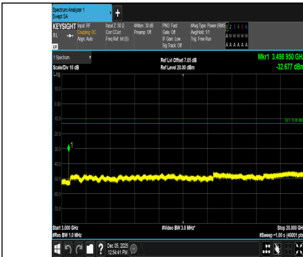
Band66-10MHz-16QAM-132322-1RB#49-3000~20000-PASS
