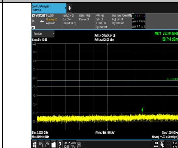
Band66-10MHz-16QAM-132622-1RB#0-30~1000-PASS
