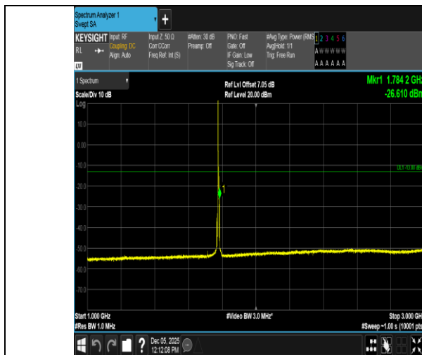
Band66-5MHz-16QAM-132647-1RB#0-1000~3000-PASS
