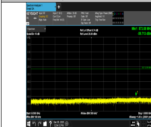
Band66-10MHz-16QAM-132322-1RB#49-30~1000-PASS
