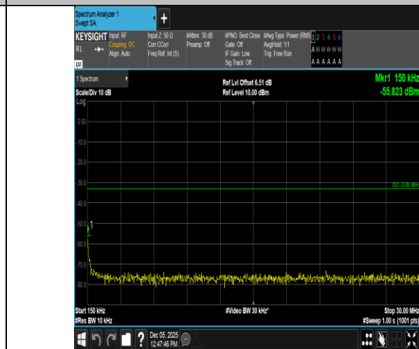
Band66-10MHz-16QAM-132022-1RB#49-0.15~30-PASS
