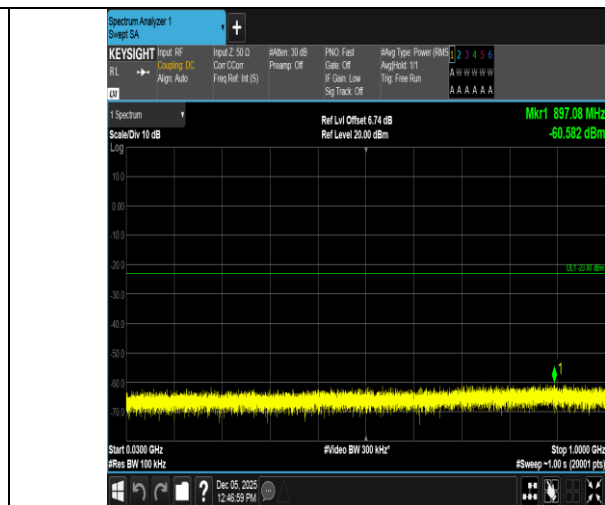
Band66-10MHz-QPSK-132022-1RB#49-30~1000-PASS
