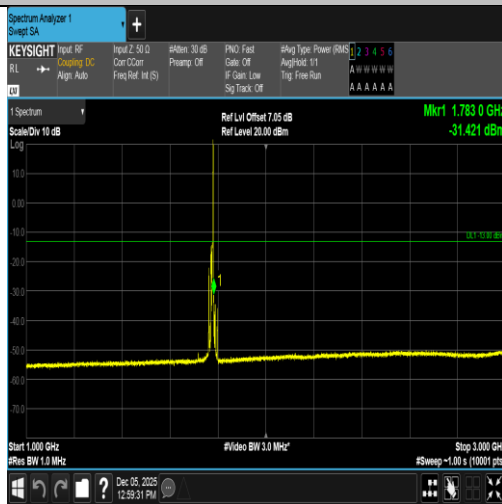
Band66-10MHz-QPSK-132622-1RB#49-1000~3000-PASS
