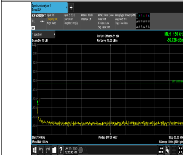
Band66-5MHz-16QAM-132647-25RB#0-0.15~30-PASS
