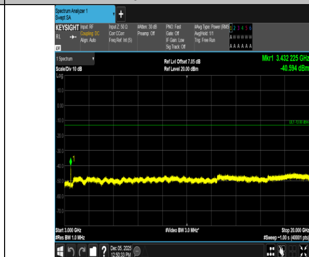
Band66-10MHz-16QAM-132022-50RB#0-3000~20000-PASS
