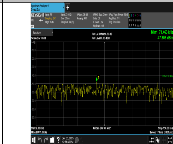
Band66-10MHz-16QAM-132322-1RB#0-0.009~0.15-PASS
