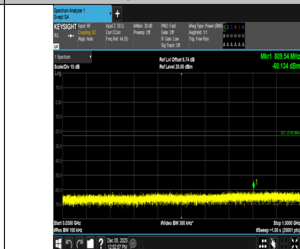
Band66-10MHz-16QAM-132322-1RB#0-30~1000-PASS
