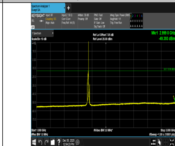
Band66-10MHz-16QAM-132322-1RB#49-1000~3000-PASS
