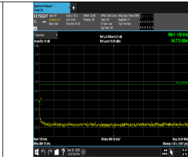
Band66-10MHz-QPSK-132622-1RB#0-0.15~30-PASS
