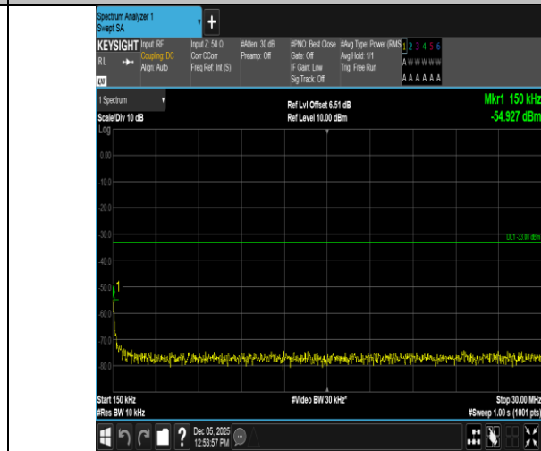
Band66-10MHz-16QAM-132322-1RB#49-0.15~30-PASS
