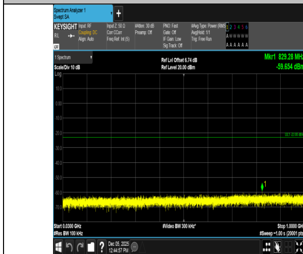
Band66-10MHz-QPSK-132022-1RB#0-30~1000-PASS
