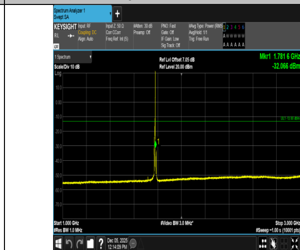
Band66-5MHz-16QAM-132647-1RB#24-1000~3000-PASS
