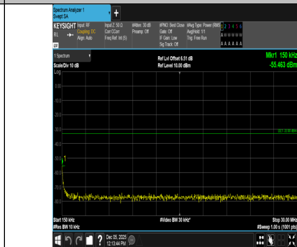
Band66-5MHz-16QAM-132647-1RB#24-0.15~30-PASS
