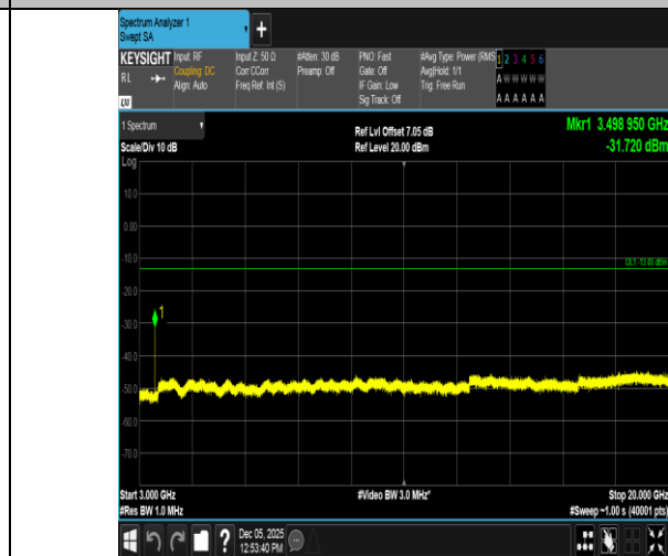
Band66-10MHz-QPSK-132322-1RB#49-3000~20000-PASS
