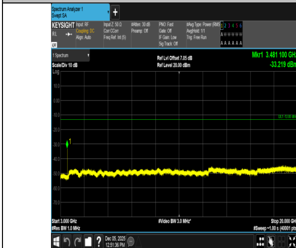
Band66-10MHz-QPSK-132322-1RB#0-3000~20000-PASS
