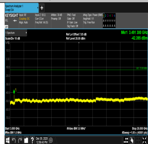
Band66-10MHz-16QAM-132322-50RB#0-3000~20000-PASS
