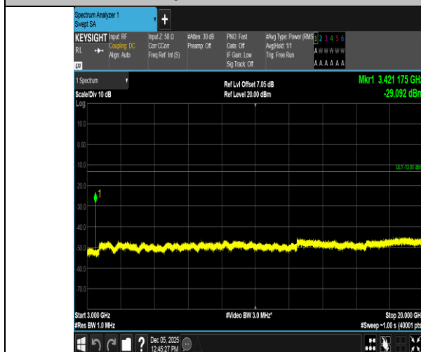
Band66-10MHz-QPSK-132022-1RB#0-3000~20000-PASS
