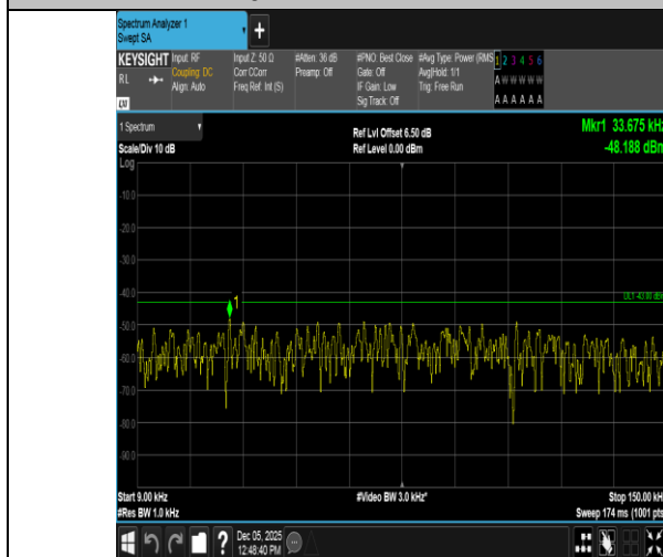
Band66-10MHz-QPSK-132022-50RB#0-0.009~0.15-PASS
