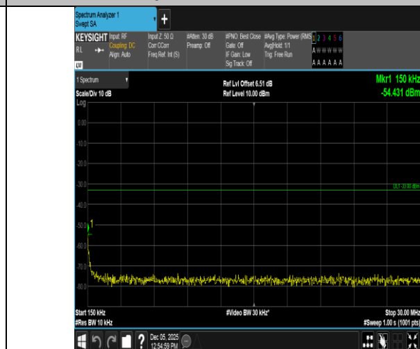
Band66-10MHz-QPSK-132322-50RB#0-0.15~30-PASS
