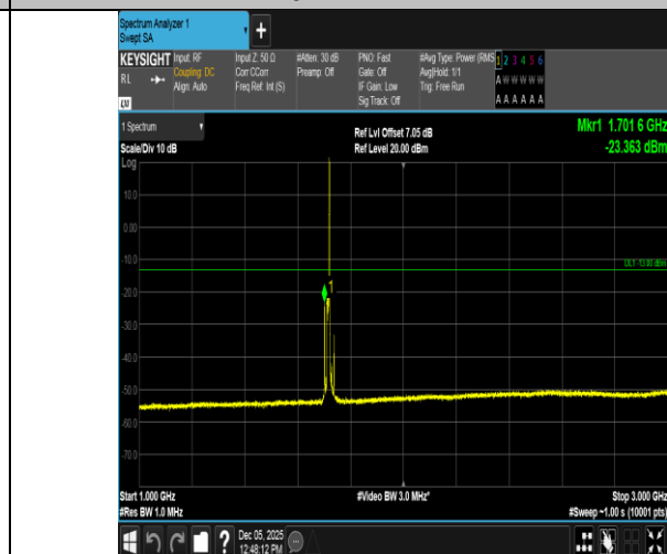
Band66-10MHz-16QAM-132022-1RB#49-1000~3000-PASS
