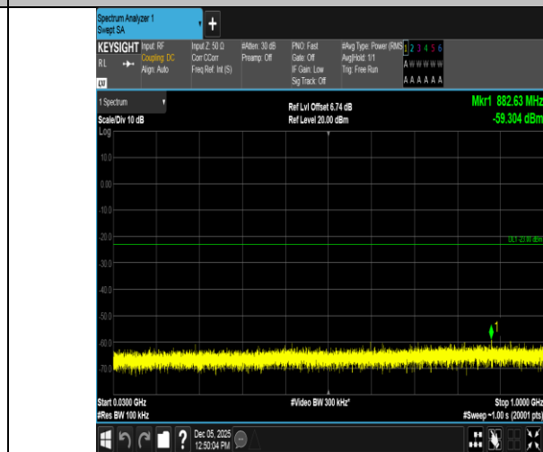
Band66-10MHz-16QAM-132022-50RB#0-30~1000-PASS
