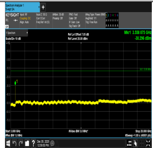
Band66-10MHz-QPSK-132622-1RB#49-3000~20000-PASS
