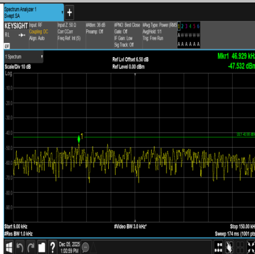
Band66-10MHz-QPSK-132622-50RB#0-0.009~0.15-PASS
