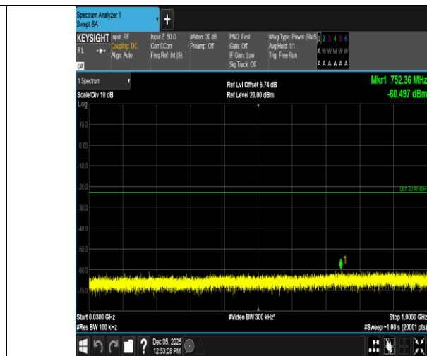
Band66-10MHz-QPSK-132322-1RB#49-30~1000-PASS
