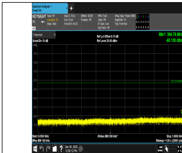
Band66-10MHz-QPSK-132322-50RB#0-30~1000-PASS
