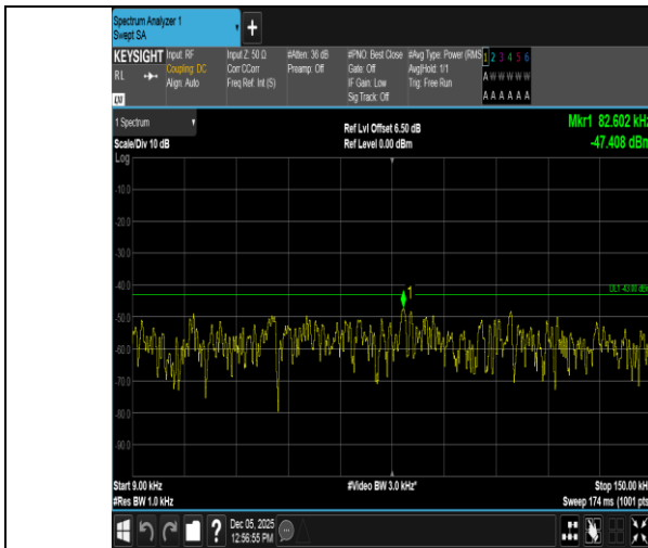
Band66-10MHz-QPSK-132622-1RB#0-0.009~0.15-PASS
