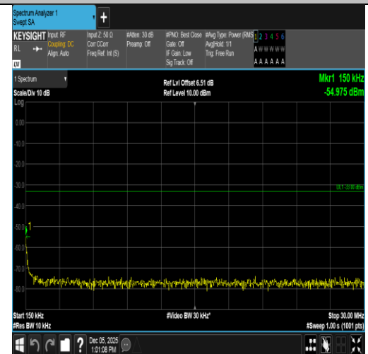
Band66-10MHz-QPSK-132622-50RB#0-0.15~30-PASS
