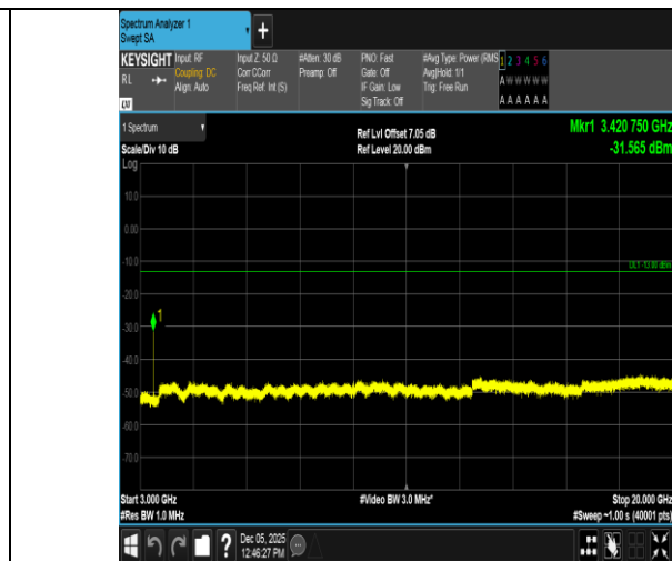
Band66-10MHz-16QAM-132022-1RB#0-3000~20000-PASS
