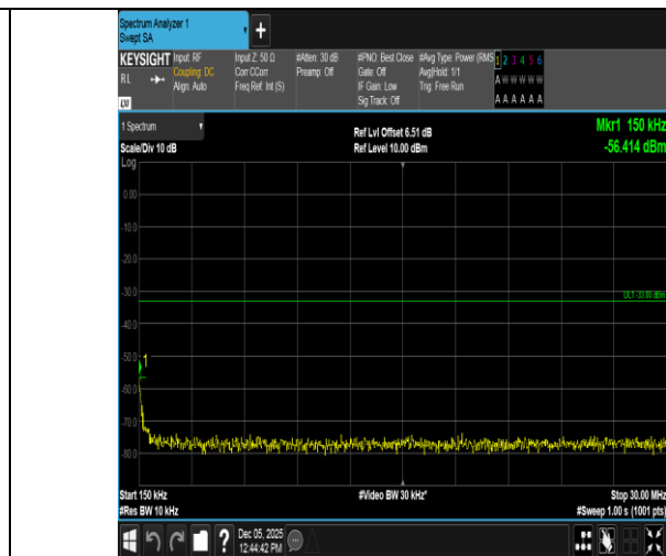
Band66-10MHz-QPSK-132022-1RB#0-0.15~30-PASS
