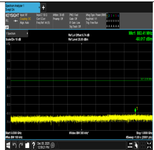
Band66-10MHz-QPSK-132622-1RB#49-30~1000-PASS
