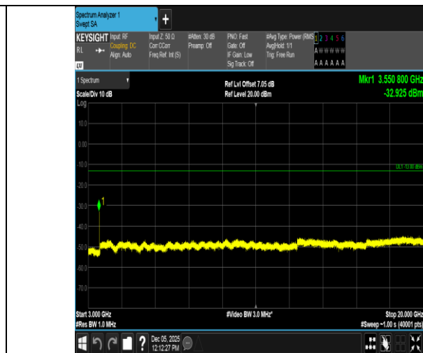
Band66-5MHz-16QAM-132647-1RB#0-3000~20000-PASS
