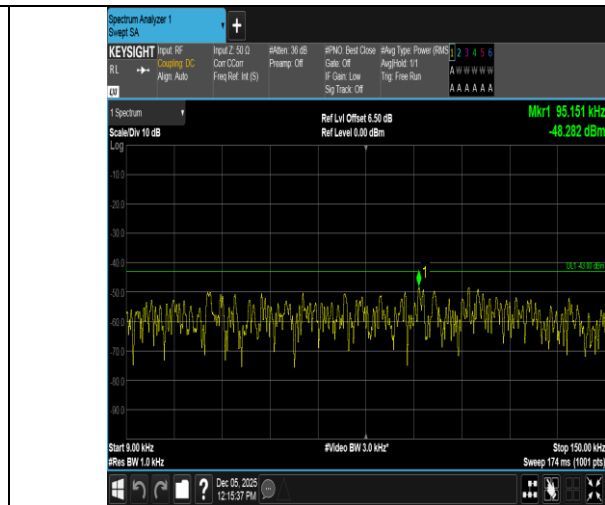
Band66-5MHz-16QAM-132647-25RB#0-0.009~0.15-PASS
