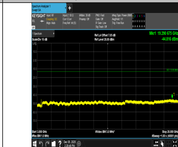
Band66-20MHz-16QAM-132322-100RB#0-3000~20000-PASS
