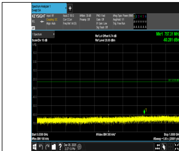
Band66-20MHz-QPSK-132322-100RB#0-30~1000-PASS
