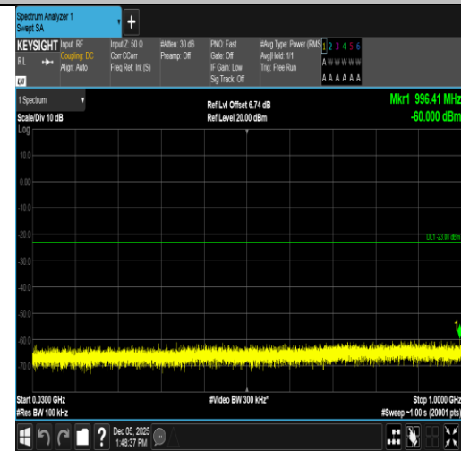
Band66-15MHz-16QAM-132597-75RB#0-30~1000-PASS
