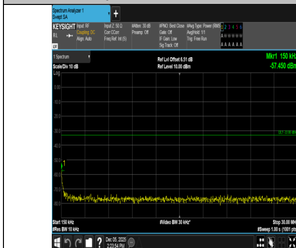
Band66-20MHz-16QAM-132322-1RB#0-0.15~30-PASS
