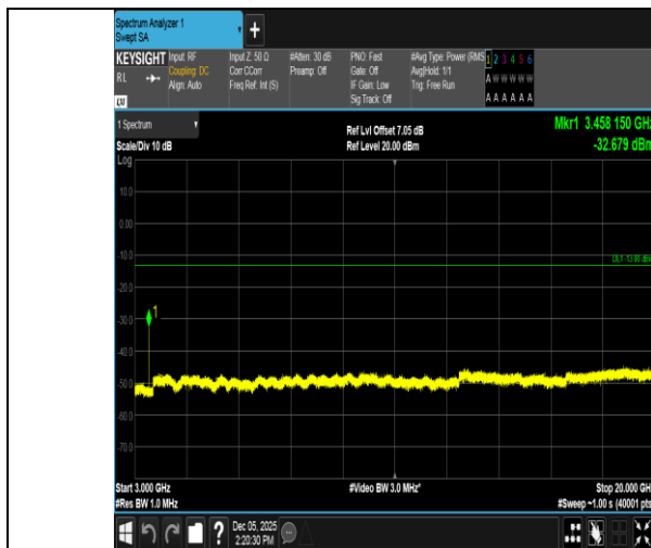
Band66-20MHz-16QAM-132072-1RB#99-3000~20000-PASS
