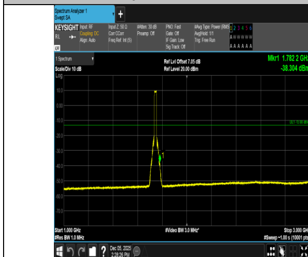
Band66-20MHz-16QAM-132322-100RB#0-1000~3000-PASS
