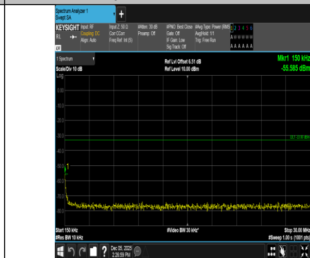
Band66-20MHz-QPSK-132322-100RB#0-0.15~30-PASS
