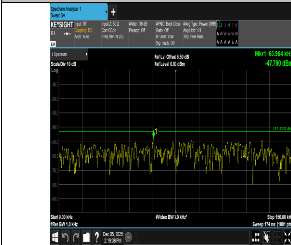
Band66-20MHz-16QAM-132072-1RB#99-0.009~0.15-PASS
