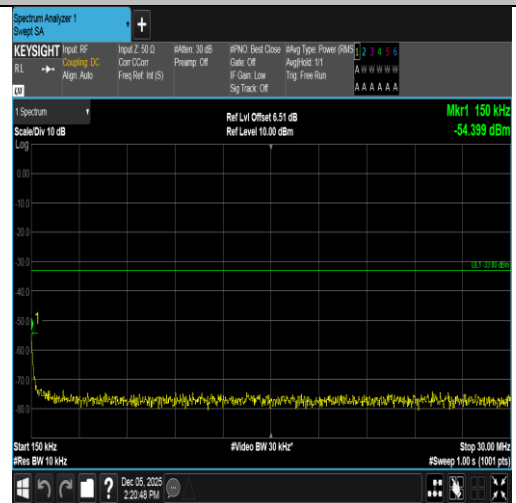
Band66-20MHz-QPSK-132072-100RB#0-0.15~30-PASS
