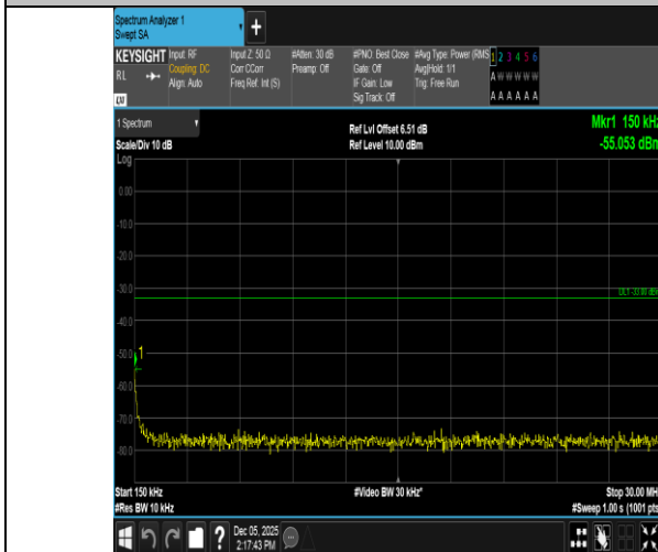
Band66-20MHz-16QAM-132072-1RB#0-0.15~30-PASS
