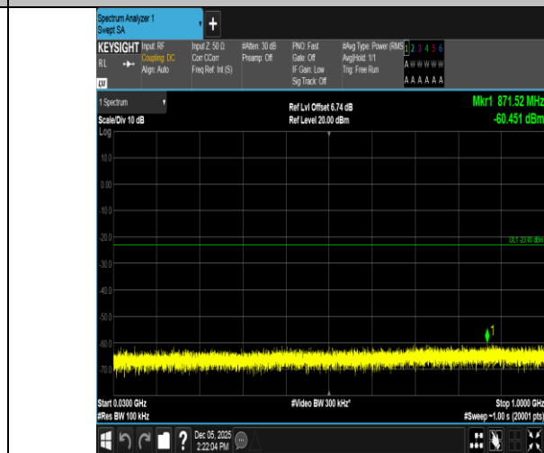
Band66-20MHz-16QAM-132072-100RB#0-30~1000-PASS
