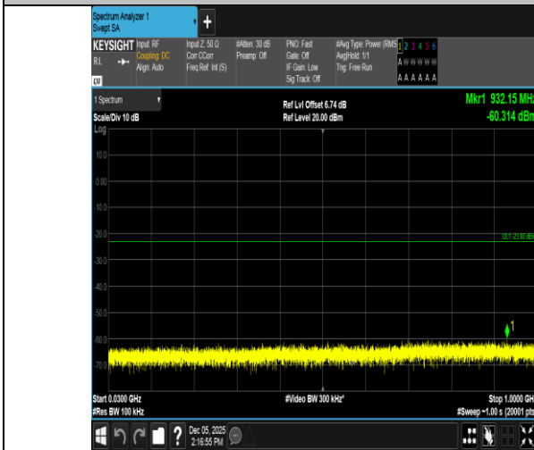
Band66-20MHz-QPSK-132072-1RB#0-30~1000-PASS
