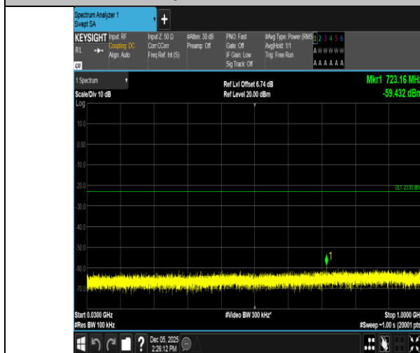
Band66-20MHz-16QAM-132322-1RB#99-30~1000-PASS
