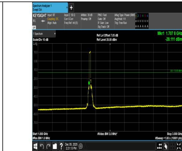
Band66-20MHz-QPSK-132072-100RB#0-1000~3000-PASS
