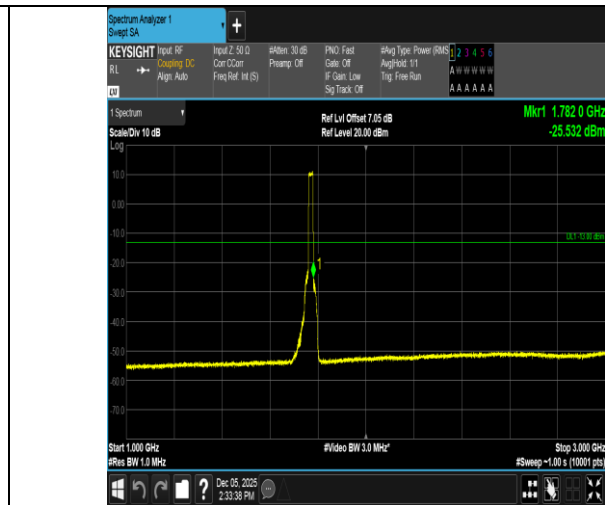
Band66-20MHz-QPSK-132572-100RB#0-1000~3000-PASS
