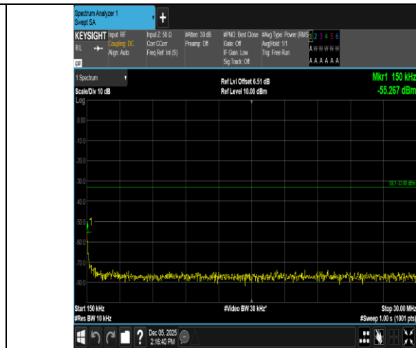
Band66-20MHz-QPSK-132072-1RB#0-0.15~30-PASS
