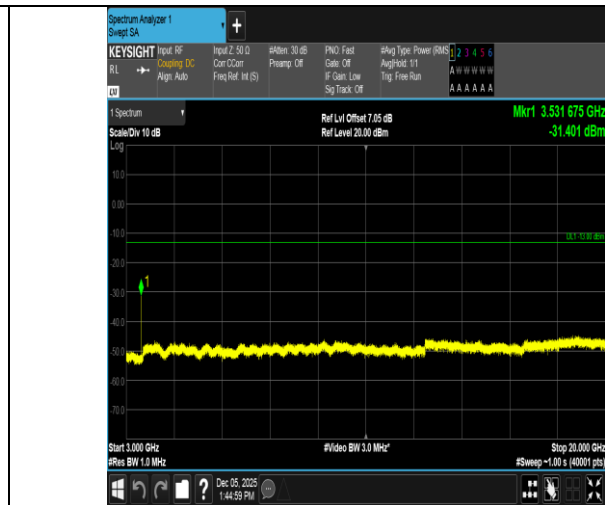
Band66-15MHz-16QAM-132597-1RB#0-3000~20000-PASS
