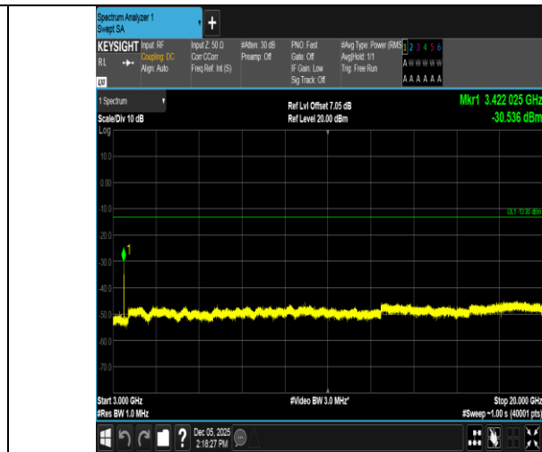
Band66-20MHz-16QAM-132072-1RB#0-3000~20000-PASS
