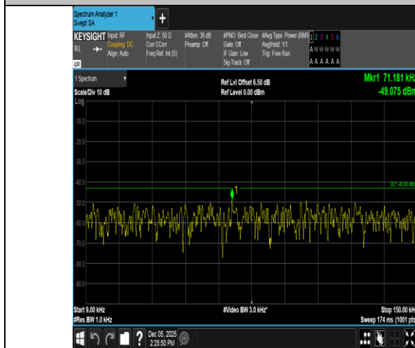
Band66-20MHz-16QAM-132322-1RB#99-0.009~0.15-PASS
