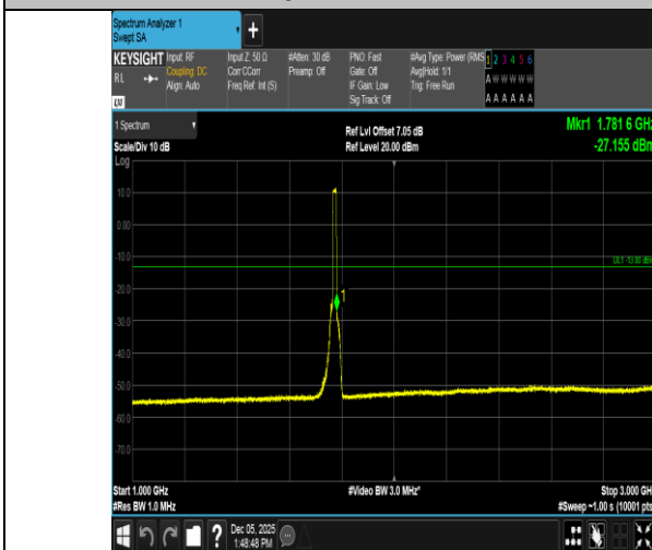
Band66-15MHz-16QAM-132597-75RB#0-1000~3000-PASS
