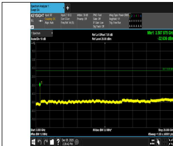
Band66-20MHz-16QAM-132322-1RB#99-3000~20000-PASS
