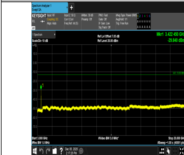
Band66-20MHz-QPSK-132072-1RB#0-3000~20000-PASS
