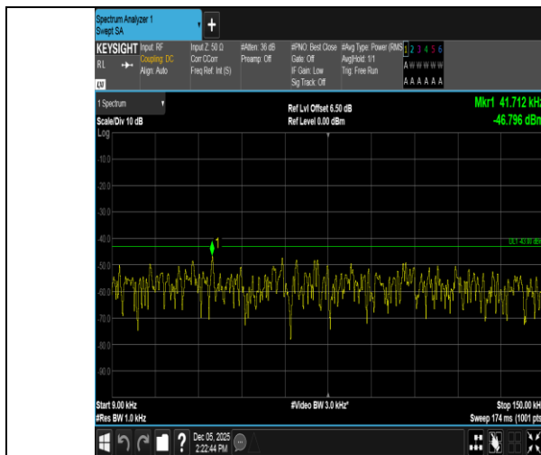
Band66-20MHz-QPSK-132322-1RB#0-0.009~0.15-PASS
