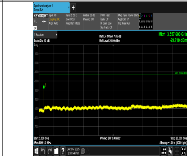
Band66-20MHz-QPSK-132572-1RB#99-3000~20000-PASS
