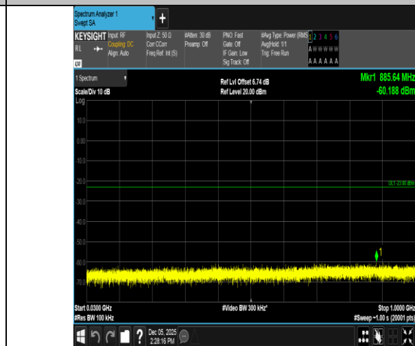
Band66-20MHz-16QAM-132322-100RB#0-30~1000-PASS
