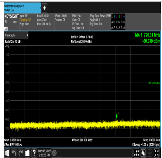
Band66-20MHz-QPSK-132072-1RB#99-30~1000-PASS
