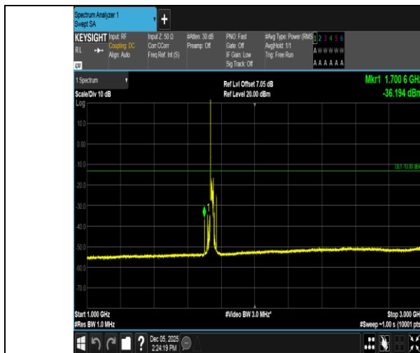
Band66-20MHz-16QAM-132322-1RB#0-1000~3000-PASS
