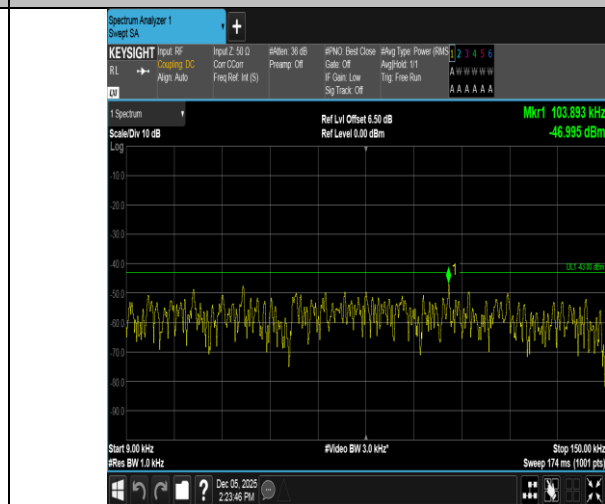
Band66-20MHz-16QAM-132322-1RB#0-0.009~0.15-PASS
