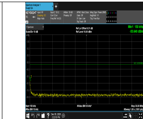
Band66-20MHz-QPSK-132322-1RB#0-0.15~30-PASS
