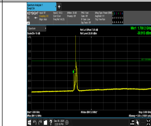
Band66-20MHz-QPSK-132322-1RB#0-1000~3000-PASS
