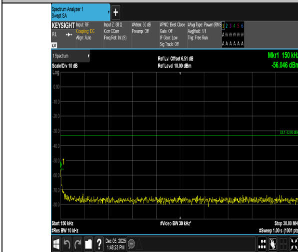
Band66-15MHz-16QAM-132597-75RB#0-0.15~30-PASS
