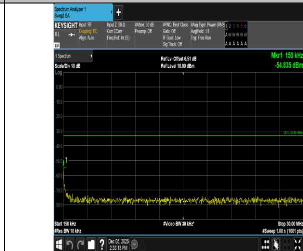
Band66-20MHz-QPSK-132572-100RB#0-0.15~30-PASS
