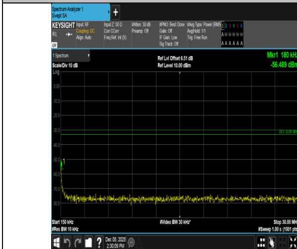
Band66-20MHz-16QAM-132572-1RB#0-0.15~30-PASS
