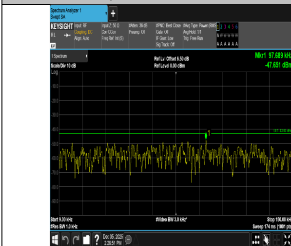
Band66-20MHz-QPSK-132322-100RB#0-0.009~0.15-PASS
