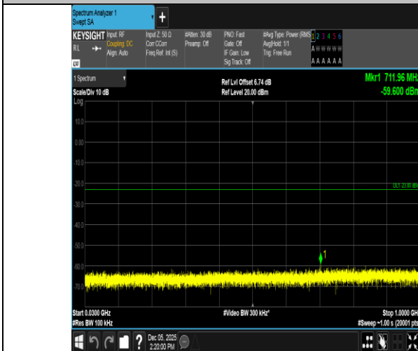
Band66-20MHz-16QAM-132072-1RB#99-30~1000-PASS
