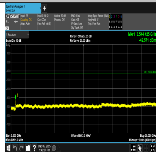
Band66-15MHz-16QAM-132597-75RB#0-3000~20000-PASS
