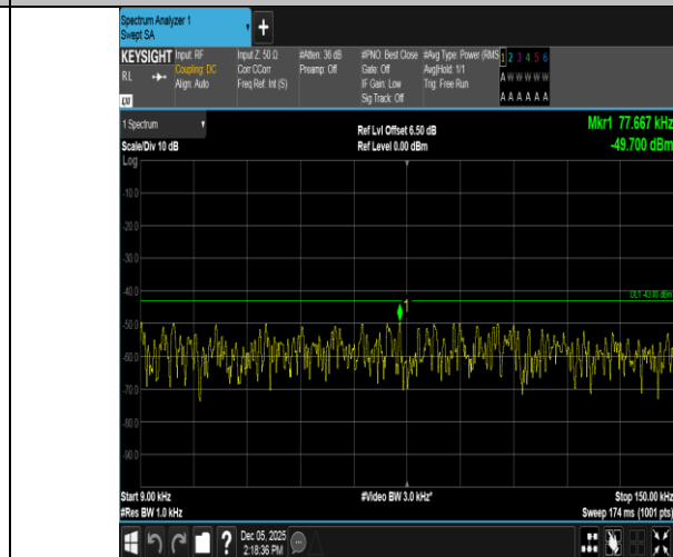
Band66-20MHz-QPSK-132072-1RB#99-0.009~0.15-PASS
