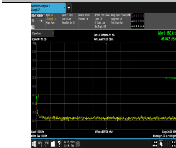
Band66-20MHz-16QAM-132072-100RB#0-0.15~30-PASS
