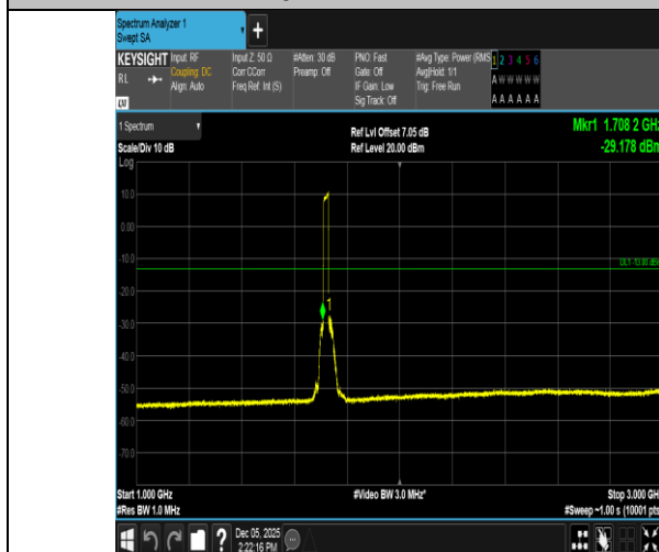
Band66-20MHz-16QAM-132072-100RB#0-1000~3000-PASS
