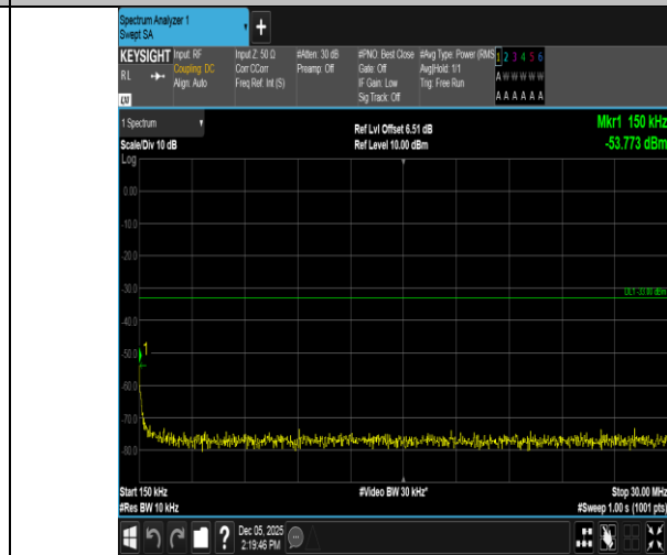
Band66-20MHz-16QAM-132072-1RB#99-0.15~30-PASS
