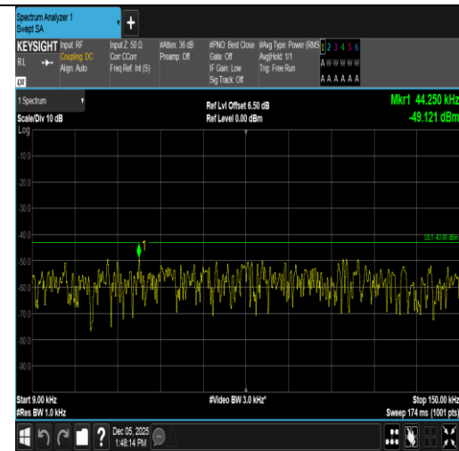
Band66-15MHz-16QAM-132597-75RB#0-0.009~0.15-PASS
