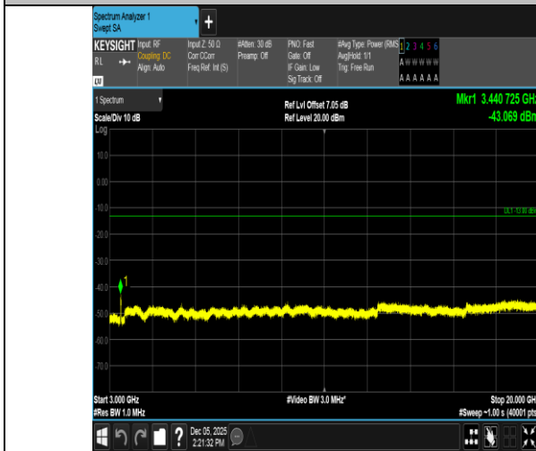
Band66-20MHz-QPSK-132072-100RB#0-3000~20000-PASS
