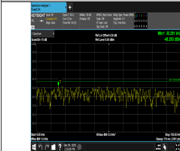
Band66-20MHz-QPSK-132572-100RB#0-0.009~0.15-PASS
