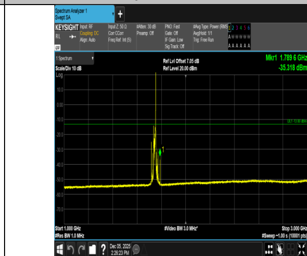
Band66-20MHz-16QAM-132322-1RB#99-1000~3000-PASS
