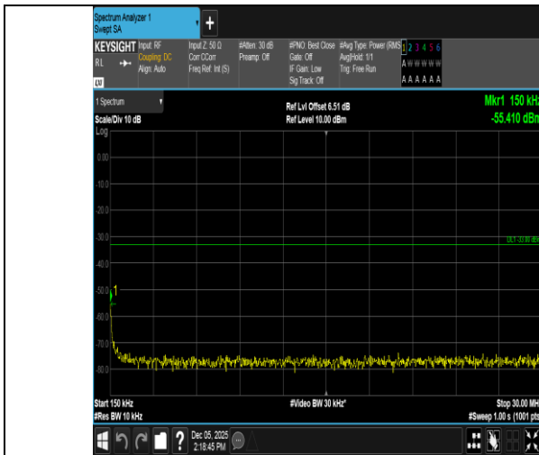
Band66-20MHz-QPSK-132072-1RB#99-0.15~30-PASS
