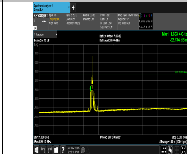
Band66-20MHz-16QAM-132072-1RB#99-1000~3000-PASS
