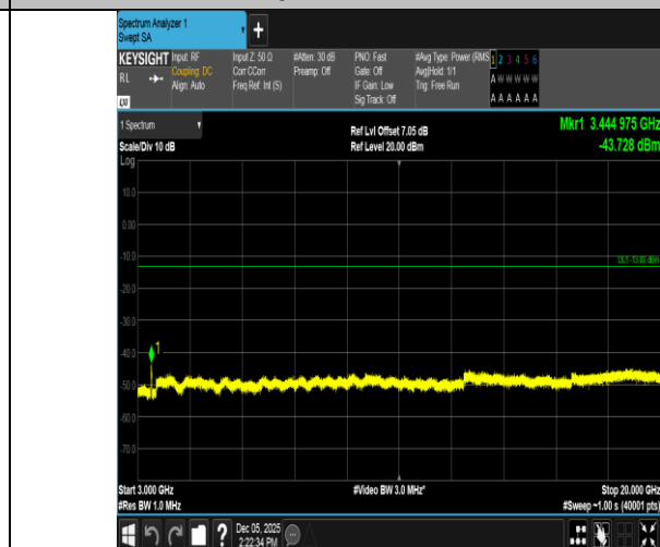
Band66-20MHz-16QAM-132072-100RB#0-3000~20000-PASS
