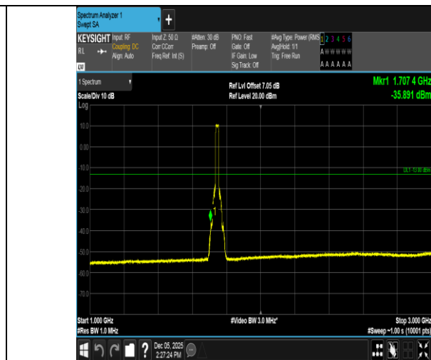
Band66-20MHz-QPSK-132322-100RB#0-1000~3000-PASS
