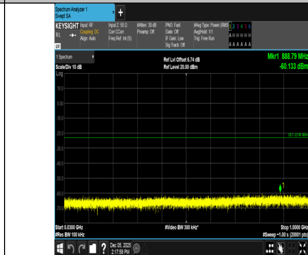
Band66-20MHz-16QAM-132072-1RB#0-30~1000-PASS
