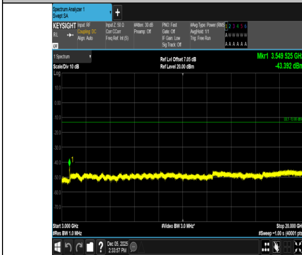
Band66-20MHz-QPSK-132572-100RB#0-3000~20000-PASS
