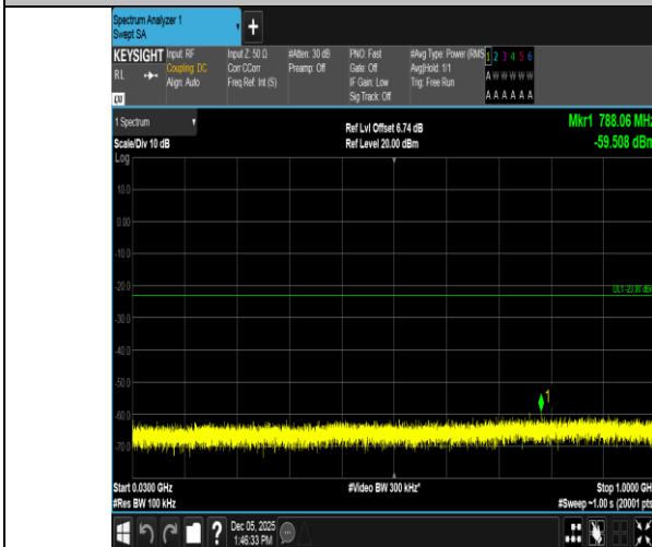
Band66-15MHz-16QAM-132597-1RB#74-30~1000-PASS
