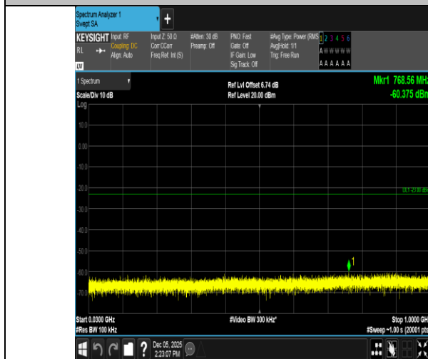
Band66-20MHz-QPSK-132322-1RB#0-30~1000-PASS
