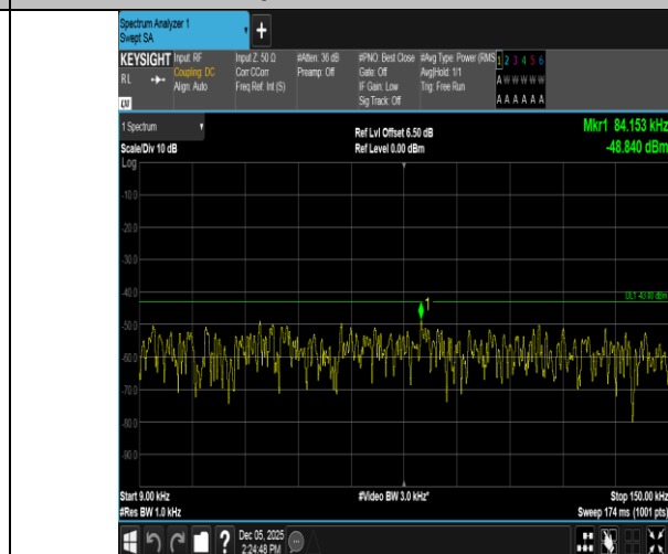
Band66-20MHz-QPSK-132322-1RB#99-0.009~0.15-PASS
