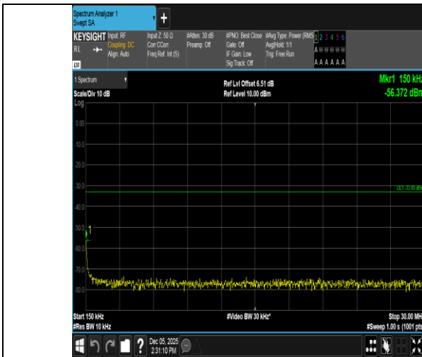
Band66-20MHz-QPSK-132572-1RB#99-0.15~30-PASS
