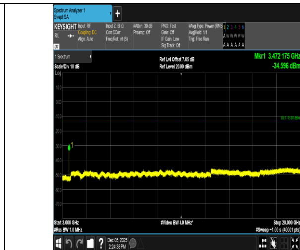
Band66-20MHz-16QAM-132322-1RB#0-3000~20000-PASS
