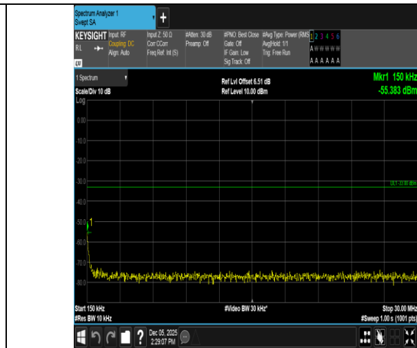
Band66-20MHz-QPSK-132572-1RB#0-0.15~30-PASS
