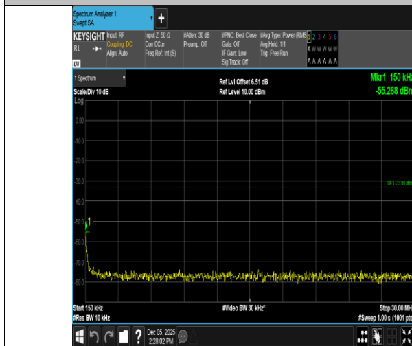
Band66-20MHz-16QAM-132322-100RB#0-0.15~30-PASS
