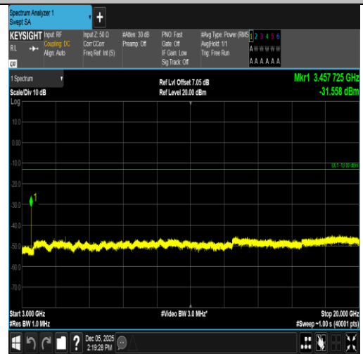
Band66-20MHz-QPSK-132072-1RB#99-3000~20000-PASS
