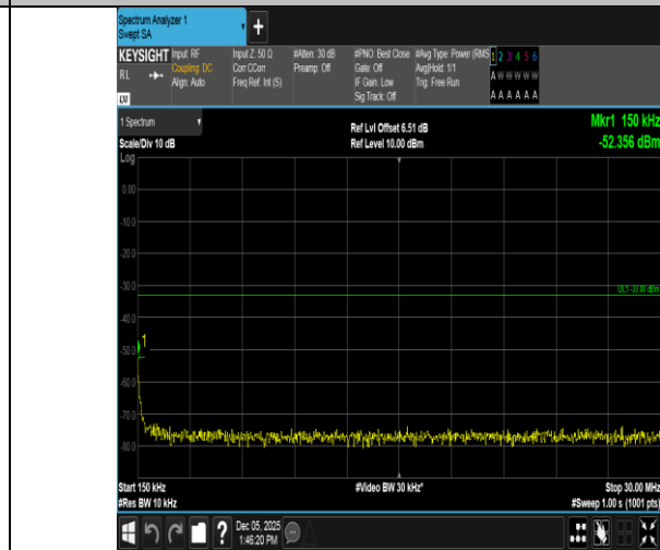
Band66-15MHz-16QAM-132597-1RB#74-0.15~30-PASS
