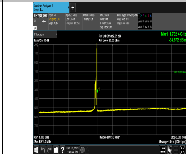
Band66-15MHz-16QAM-132597-1RB#74-1000~3000-PASS
