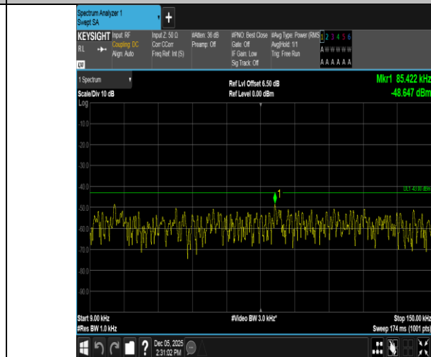
Band66-20MHz-QPSK-132572-1RB#99-0.009~0.15-PASS
