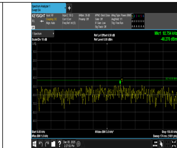
Band66-20MHz-16QAM-132322-100RB#0-0.009~0.15-PASS
