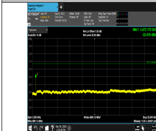
Band66-20MHz-QPSK-132322-1RB#0-3000~20000-PASS
