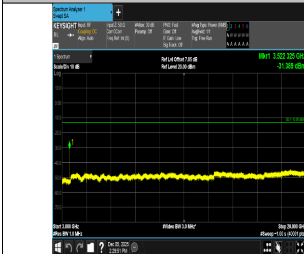
Band66-20MHz-QPSK-132572-1RB#0-3000~20000-PASS
