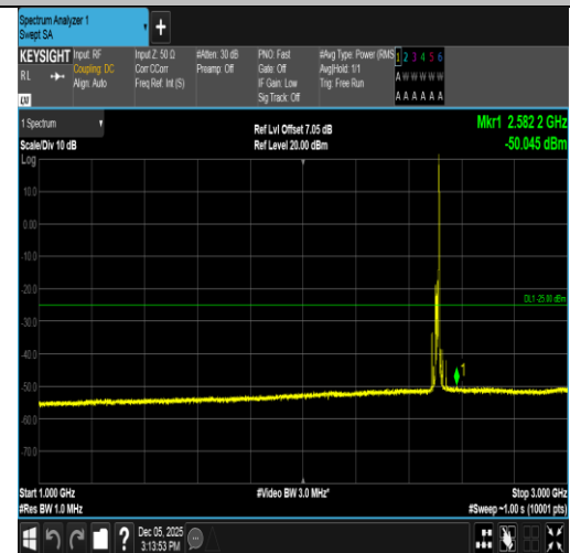
Band7-15MHz-QPSK-20825-1RB#74-1000~3000-PASS
