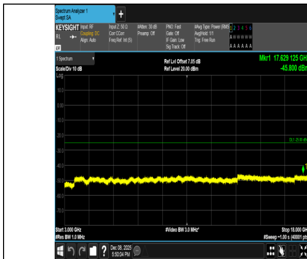
Band7-10MHz-16QAM-21100-1RB#0-3000~18000-PASS
