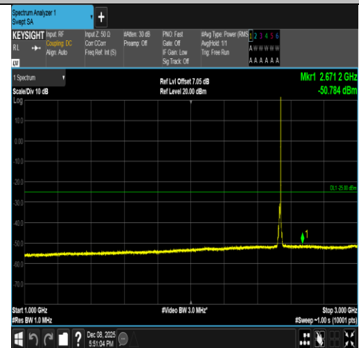
Band7-10MHz-QPSK-21100-1RB#49-1000~3000-PASS
