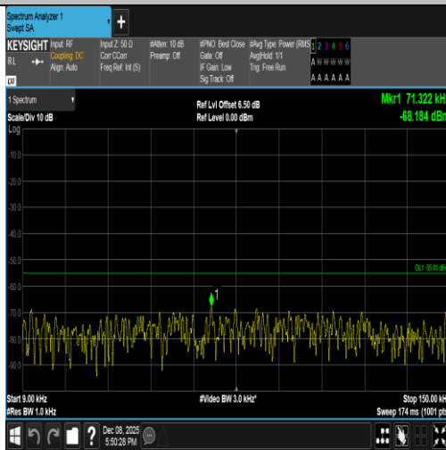
Band7-10MHz-QPSK-21100-1RB#49-0.009~0.15-PASS
