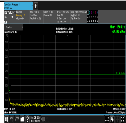
Band7-10MHz-QPSK-21100-1RB#0-0.15~30-PASS
