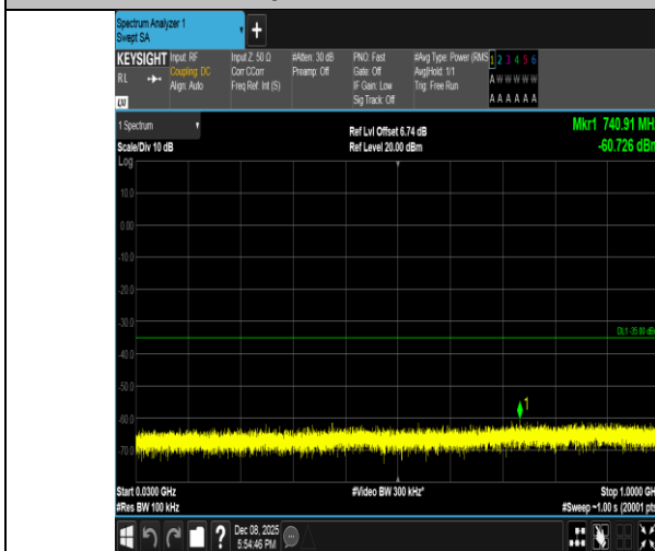
Band7-10MHz-16QAM-21100-50RB#0-30~1000-PASS
