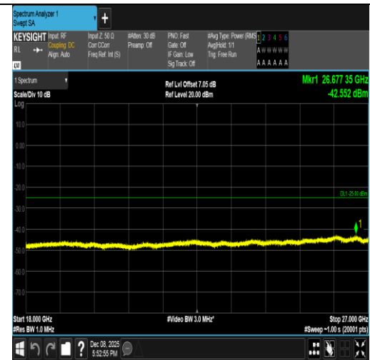
Band7-10MHz-16QAM-21100-1RB#49-18000~27000-PASS
