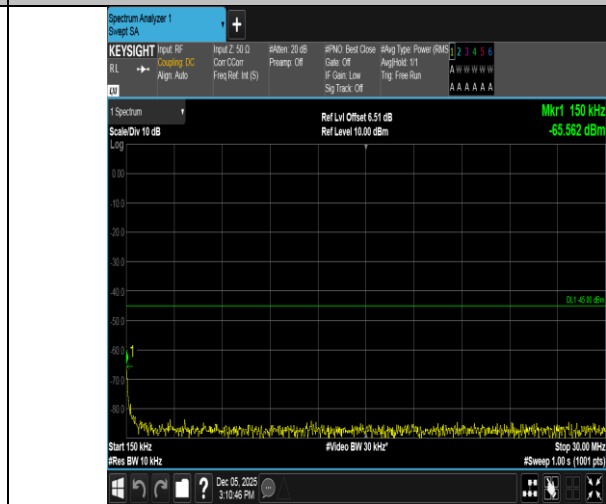
Band7-15MHz-QPSK-20825-1RB#0-0.15~30-PASS
