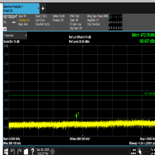
Band7-10MHz-QPSK-21100-50RB#0-30~1000-PASS
