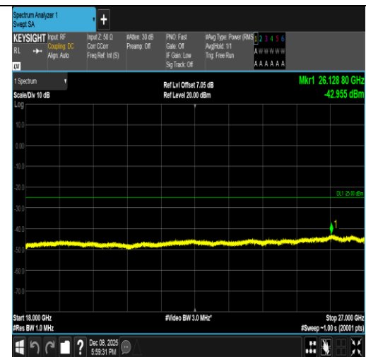
Band7-10MHz-QPSK-21400-1RB#49-18000~27000-PASS
