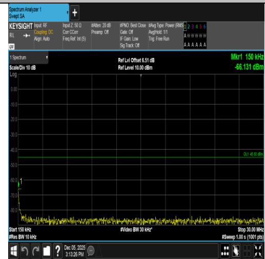
Band7-15MHz-QPSK-20825-1RB#74-0.15~30-PASS
