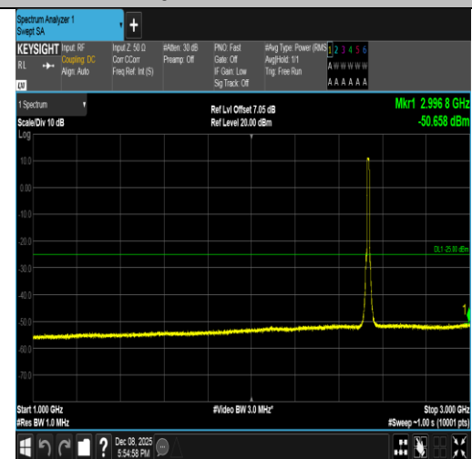
Band7-10MHz-16QAM-21100-50RB#0-1000~3000-PASS
