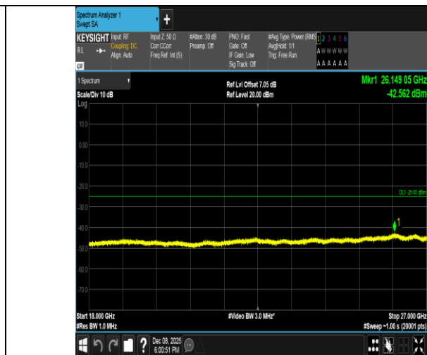
Band7-10MHz-16QAM-21400-1RB#49-18000~27000-PASS
