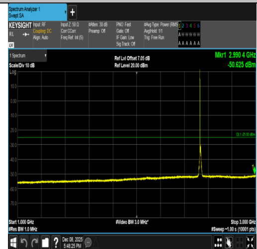
Band7-10MHz-QPSK-21100-1RB#0-1000~3000-PASS
