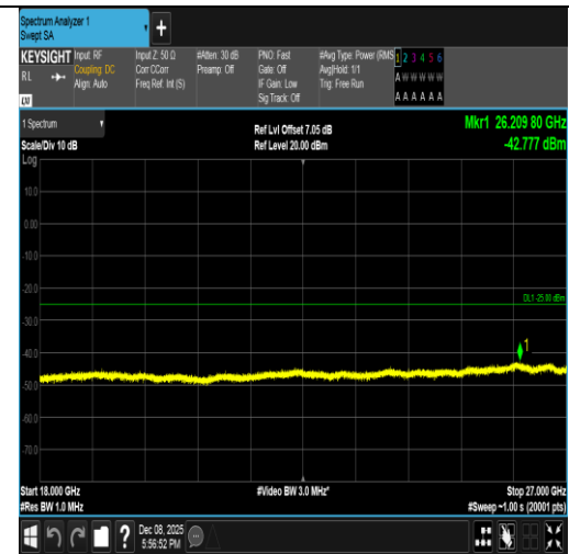
Band7-10MHz-QPSK-21400-1RB#0-18000~27000-PASS
