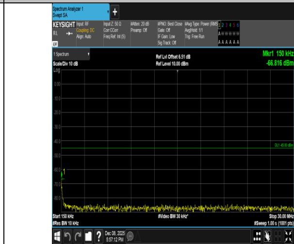
Band7-10MHz-16QAM-21400-1RB#0-0.15~30-PASS
