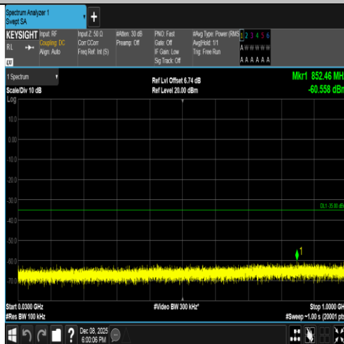
Band7-10MHz-16QAM-21400-1RB#49-30~1000-PASS
