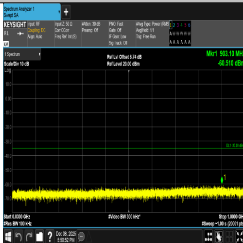
Band7-10MHz-QPSK-21100-1RB#49-30~1000-PASS
