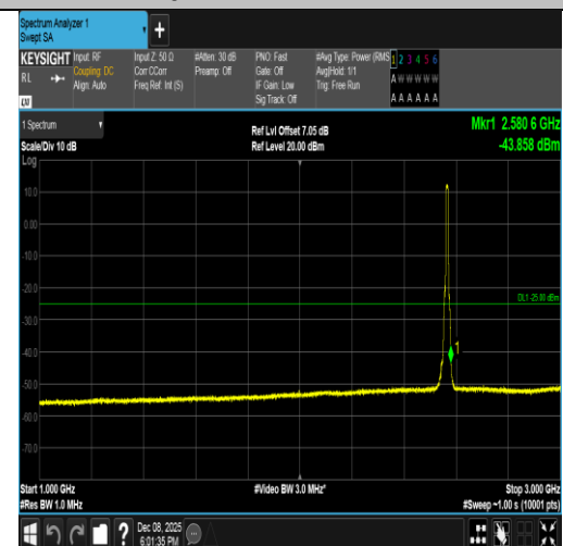
Band7-10MHz-QPSK-21400-50RB#0-1000~3000-PASS
