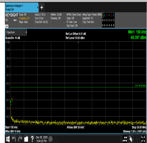
Band7-10MHz-16QAM-21100-50RB#0-0.15~30-PASS
