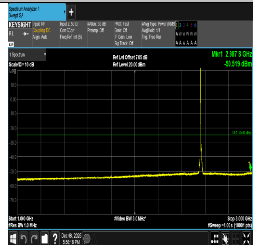
Band7-10MHz-QPSK-21400-1RB#0-1000~3000-PASS
