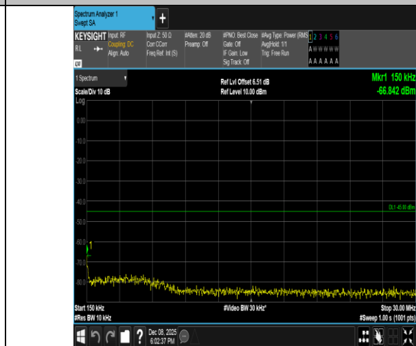
Band7-10MHz-16QAM-21400-50RB#0-0.15~30-PASS
