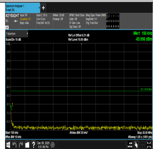
Band7-10MHz-16QAM-21100-1RB#49-0.15~30-PASS
