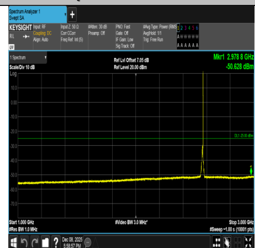
Band7-10MHz-QPSK-21400-1RB#49-1000~3000-PASS
