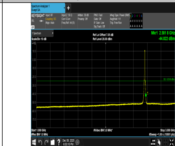
Band7-10MHz-16QAM-21400-50RB#0-1000~3000-PASS
