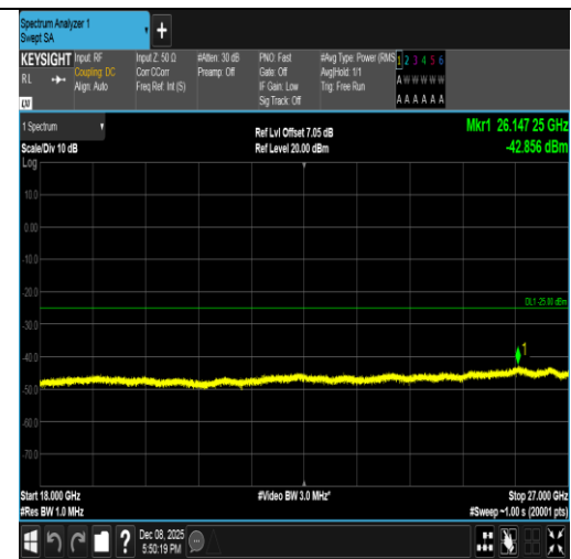
Band7-10MHz-16QAM-21100-1RB#0-18000~27000-PASS
