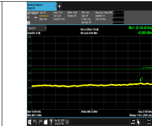
Band7-10MHz-16QAM-21400-50RB#0-18000~27000-PASS
