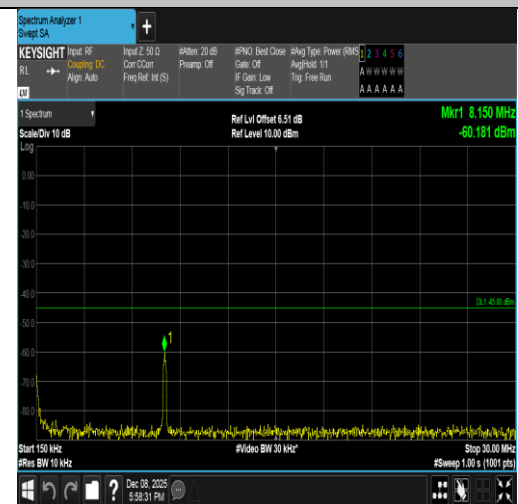
Band7-10MHz-QPSK-21400-1RB#49-0.15~30-PASS
