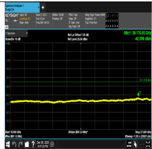
Band7-10MHz-16QAM-20800-50RB#0-18000~27000-PASS
