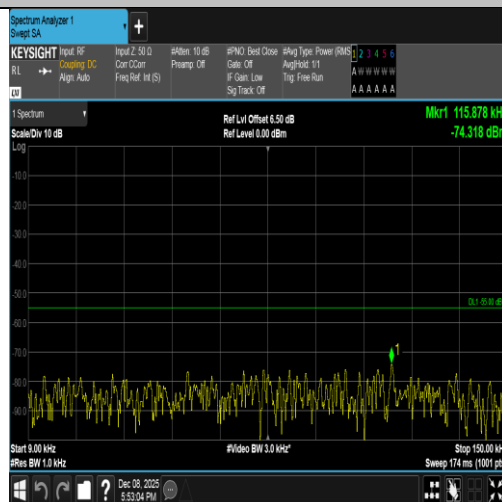
Band7-10MHz-QPSK-21100-50RB#0-0.009~0.15-PASS
