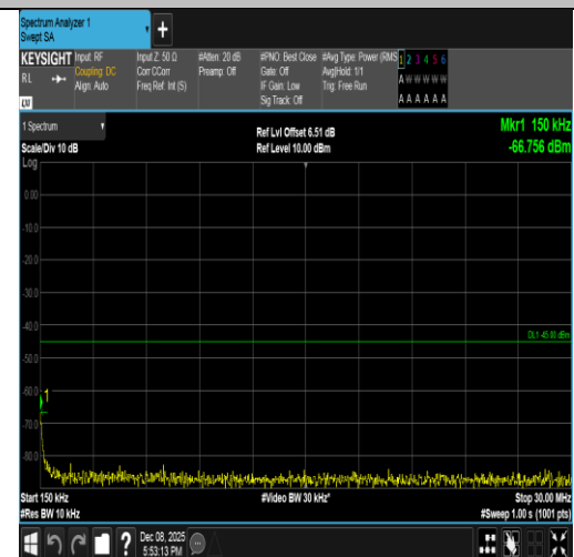
Band7-10MHz-QPSK-21100-50RB#0-0.15~30-PASS
