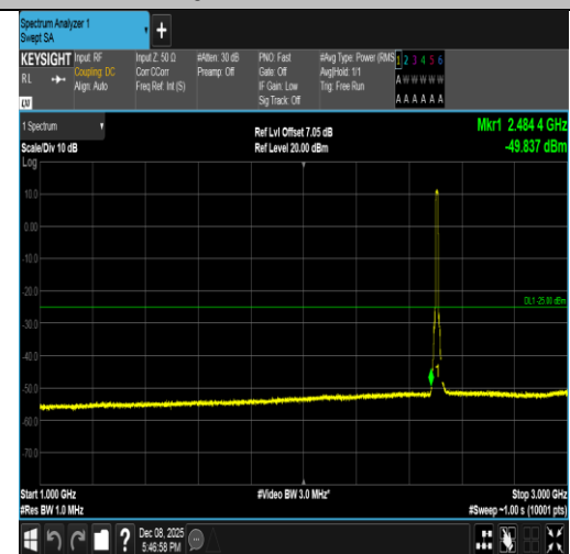
Band7-10MHz-16QAM-20800-50RB#0-1000~3000-PASS
