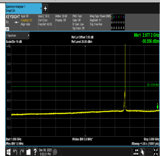
Band7-10MHz-16QAM-21100-1RB#49-1000~3000-PASS
