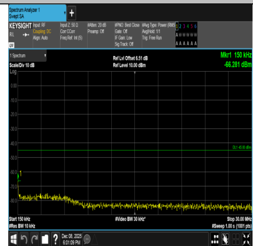
Band7-10MHz-QPSK-21400-50RB#0-0.15~30-PASS
