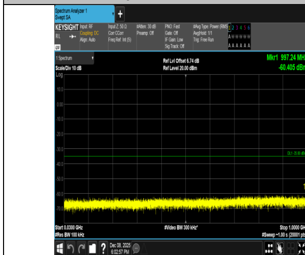
Band7-10MHz-16QAM-21400-50RB#0-30~1000-PASS
