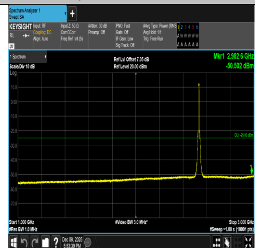
Band7-10MHz-QPSK-21100-50RB#0-1000~3000-PASS
