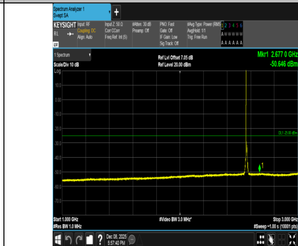
Band7-10MHz-16QAM-21400-1RB#0-1000~3000-PASS
