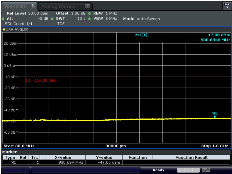
Test_Graph_band66_1772.5MHz_15M_QPSK_75RB#LOW_30M_1G_TX
