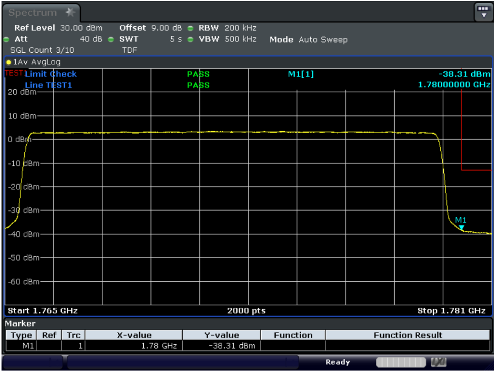
Test_Graph_band66_1772.5MHz_15M_QPSK_1RB#HIGH_Band edge
