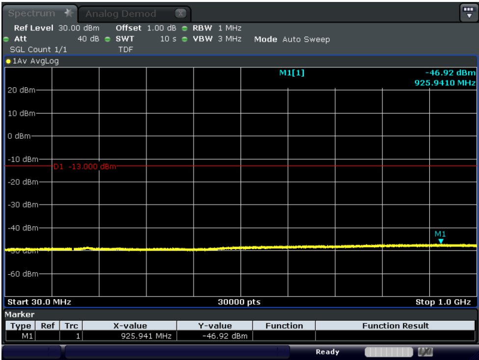
Test_Graph_band66_1710.7MHz_1.4M_QPSK_6RB#LOW_30M_1G_TX
