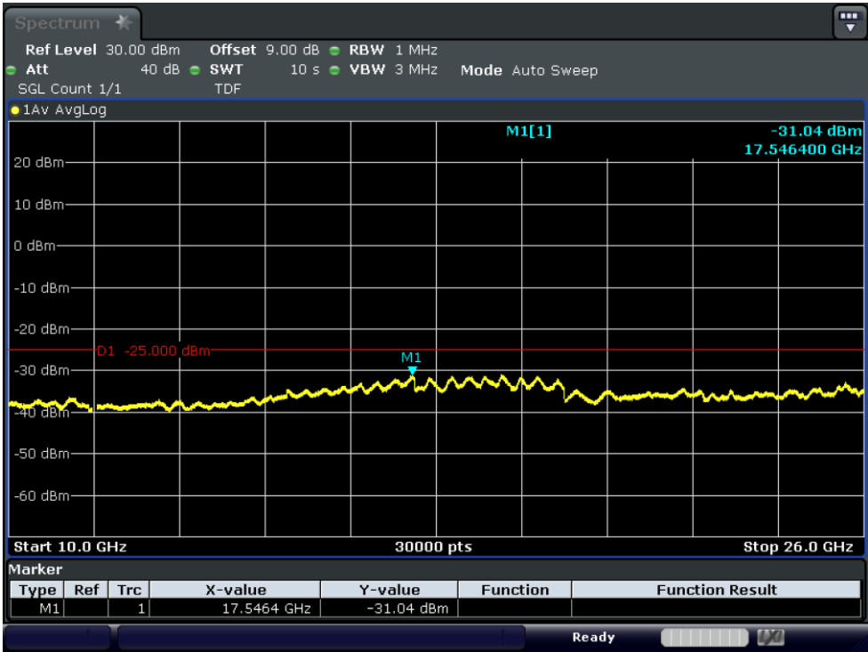
Test_Graph_band7_2507.5MHz_15M_QPSK_75RB#LOW_10G_26.0G_TX
