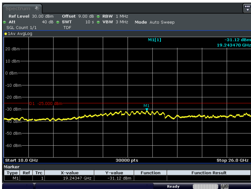
Test_Graph_band7_2562.5MHz_15M_QPSK_75RB#LOW_10G_26.0G_TX
