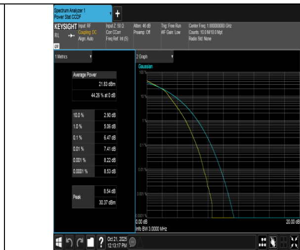
Band2-3MHz-16QAM-18900-15RB#0-PASS
