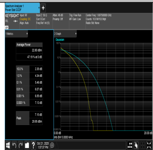
Band2-5MHz-QPSK-19175-25RB#0-PASS
