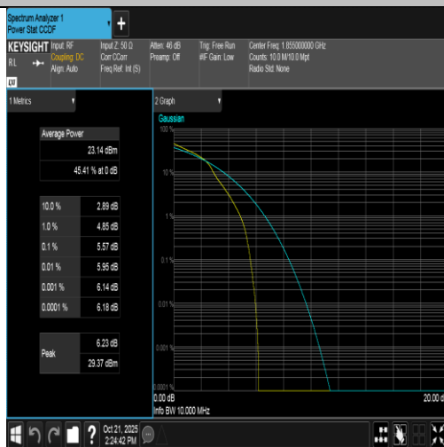
Band2-10MHz-16QAM-18650-1RB#0-PASS
