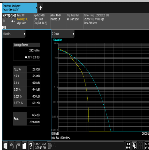
Band2-15MHz-16QAM-18675-1RB#0-PASS
