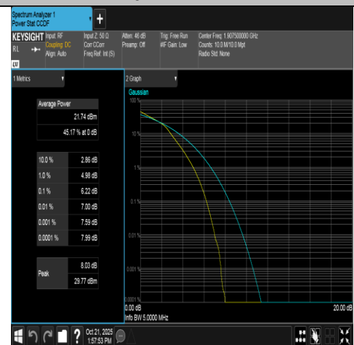
Band2-5MHz-16QAM-19175-25RB#0-PASS
