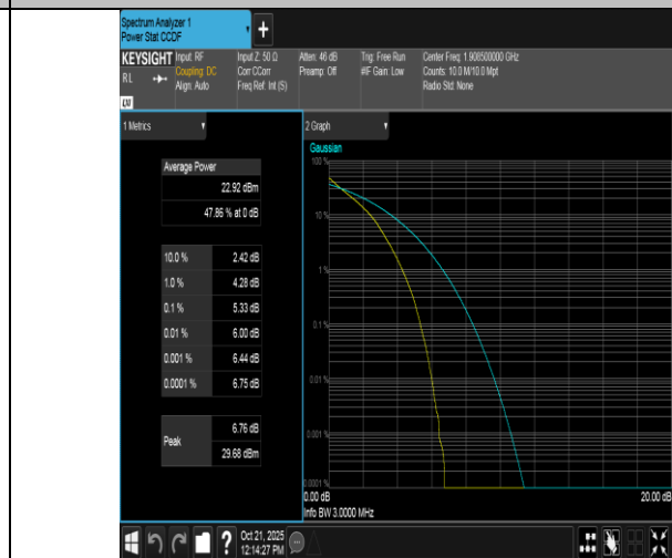
Band2-3MHz-QPSK-19185-15RB#0-PASS
