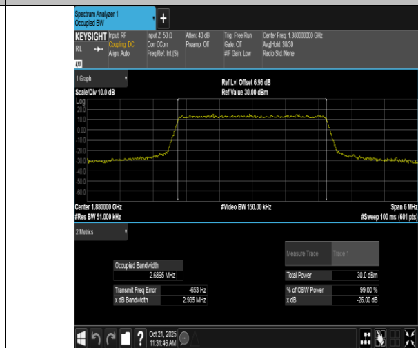
Band2-3MHz-16QAM-18900-15RB#0-PASS
