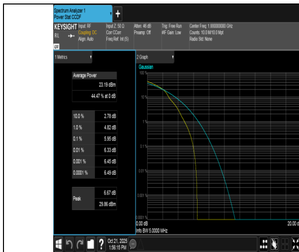
Band2-5MHz-16QAM-18900-1RB#0-PASS
