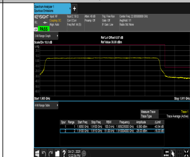
Band2-5MHz-16QAM-19175-25RB#0-PASS
