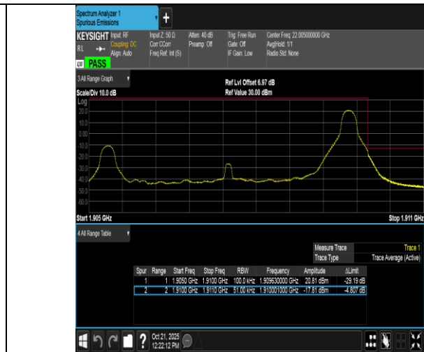
Band2-5MHz-QPSK-19175-1RB#24-PASS
