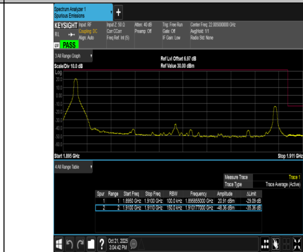
Band2-15MHz-16QAM-19125-1RB#0-PASS
