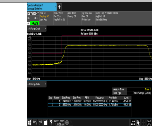
Band2-3MHz-16QAM-18615-15RB#0-PASS
