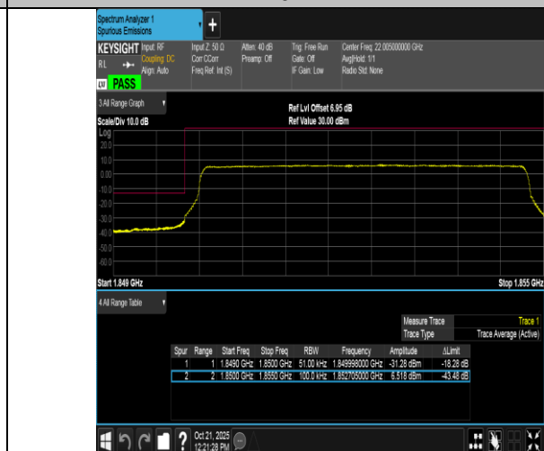
Band2-5MHz-16QAM-18625-25RB#0-PASS
