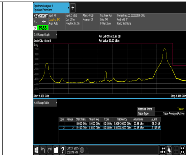
Band2-10MHz-QPSK-19150-1RB#49-PASS
