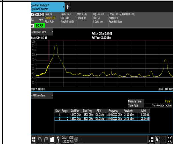
Band2-10MHz-16QAM-18650-1RB#0-PASS
