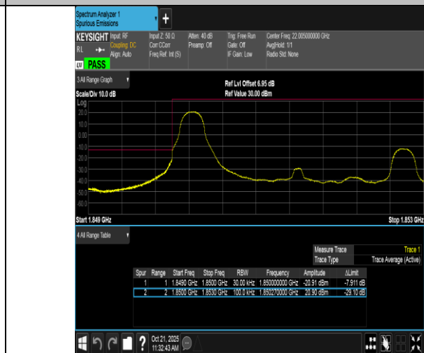
Band2-3MHz-16QAM-18615-1RB#0-PASS
