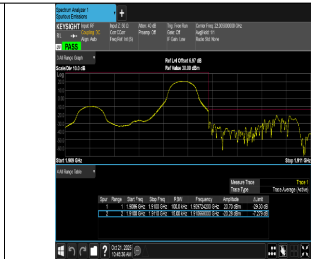
Band2-1.4MHz-QPSK-19193-1RB#5-PASS
