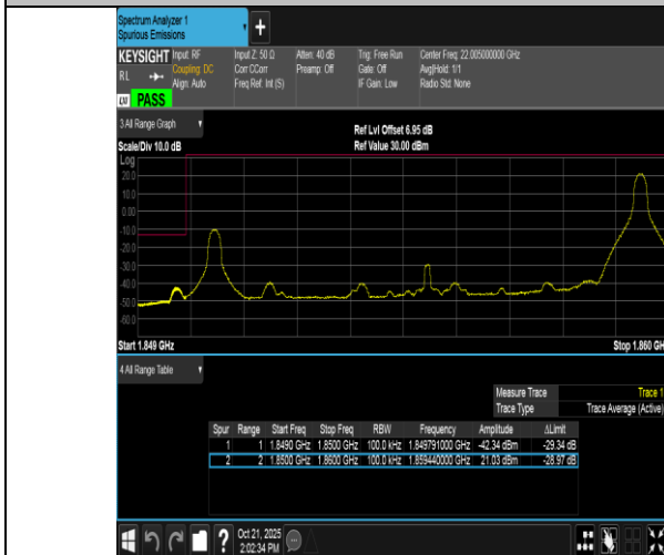
Band2-10MHz-16QAM-18650-1RB#49-PASS
