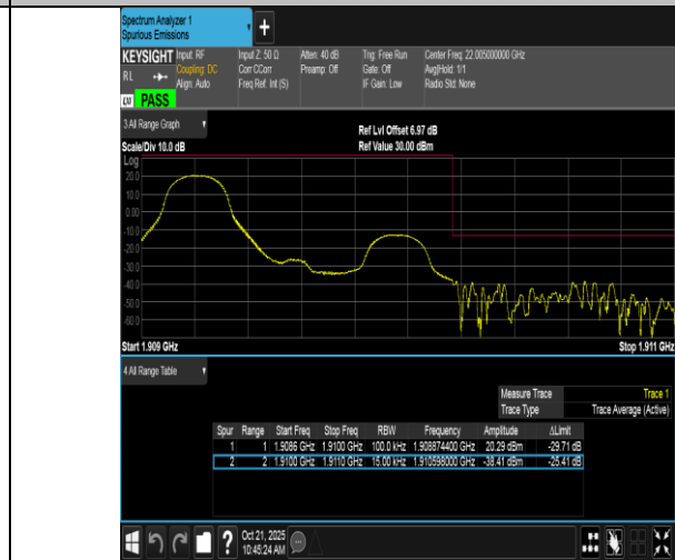
Band2-1.4MHz-16QAM-19193-1RB#0-PASS
