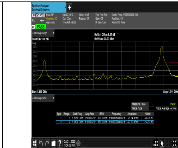
Band2-15MHz-QPSK-19125-1RB#74-PASS
