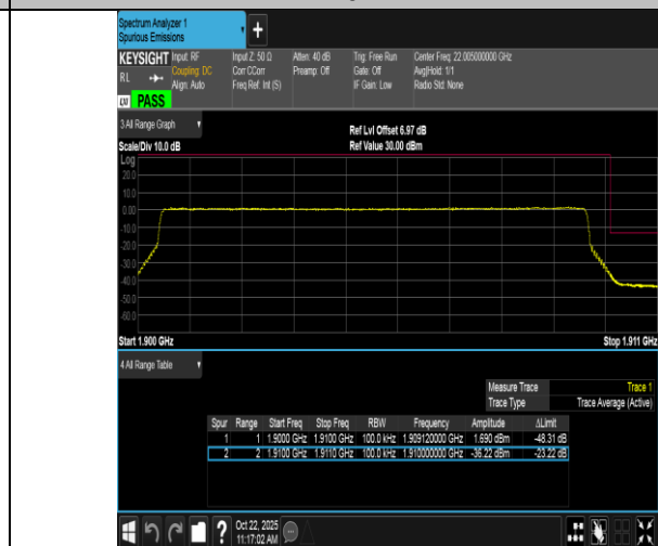
Band2-10MHz-16QAM-19150-50RB#0-PASS
