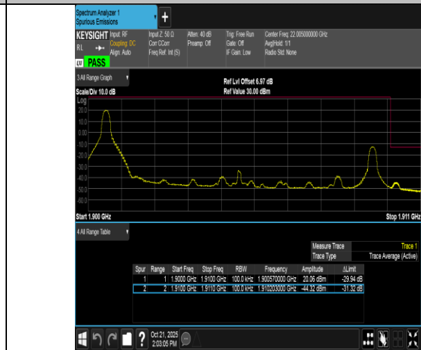
Band2-10MHz-16QAM-19150-1RB#0-PASS
