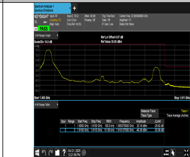
Band2-5MHz-16QAM-19175-1RB#0-PASS
