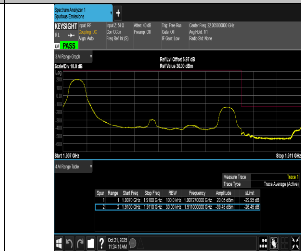
Band2-3MHz-16QAM-19185-1RB#0-PASS
