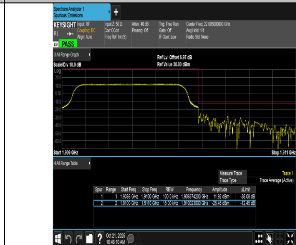
Band2-1.4MHz-16QAM-19193-6RB#0-PASS
