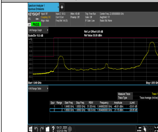
Band2-5MHz-16QAM-18625-1RB#24-PASS
