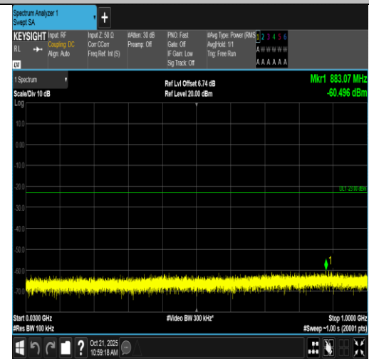
Band2-1.4MHz-16QAM-18900-6RB#0-30~1000-PASS
