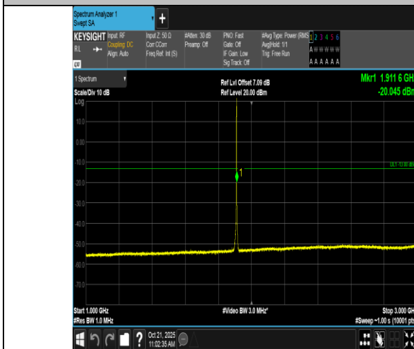
Band2-1.4MHz-QPSK-19193-1RB#5-1000~3000-PASS
