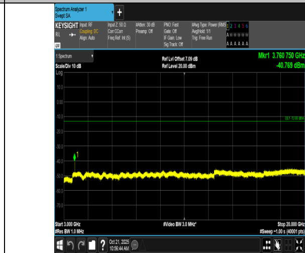
Band2-1.4MHz-QPSK-18900-1RB#5-3000~20000-PASS
