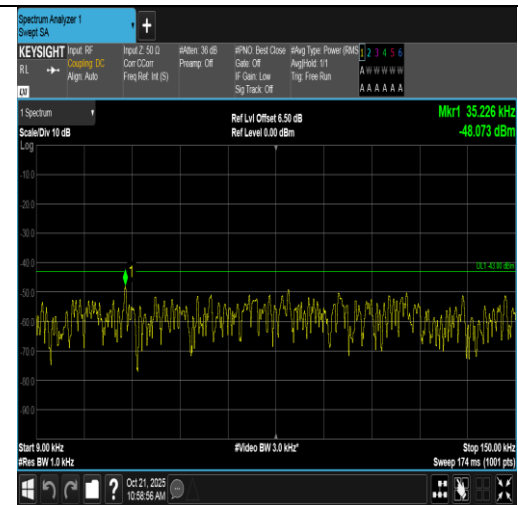
Band2-1.4MHz-16QAM-18900-6RB#0-0.009~0.15-PASS
