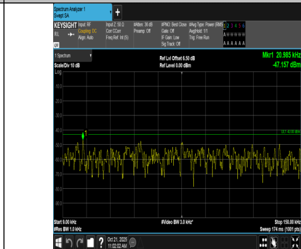
Band2-1.4MHz-QPSK-19193-1RB#5-0.009~0.15-PASS
