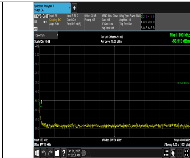
Band2-1.4MHz-QPSK-19193-1RB#0-0.15~30-PASS
