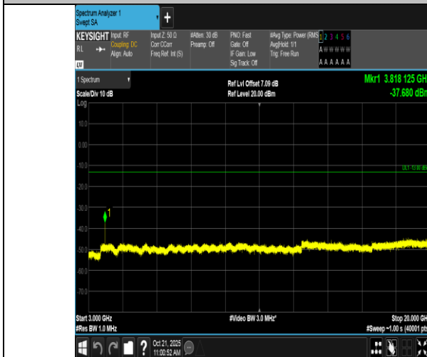
Band2-1.4MHz-QPSK-19193-1RB#0-3000~20000-PASS
