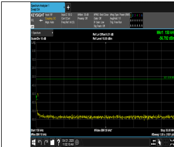
Band2-1.4MHz-QPSK-19193-1RB#5-0.15~30-PASS
