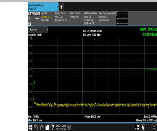
Band2-1.4MHz-16QAM-18900-1RB#5-0.15~30-PASS
