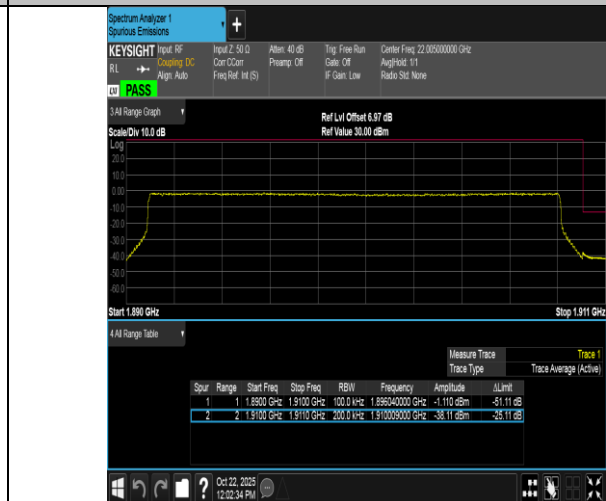
Band2-20MHz-16QAM-19100-100RB#0-PASS
