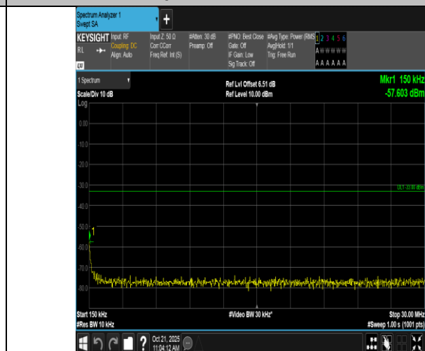
Band2-1.4MHz-QPSK-19193-6RB#0-0.15~30-PASS
