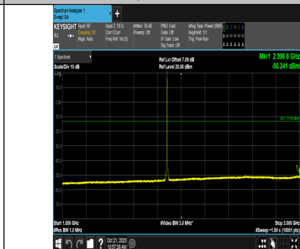
Band2-1.4MHz-16QAM-18900-1RB#5-1000~3000-PASS
