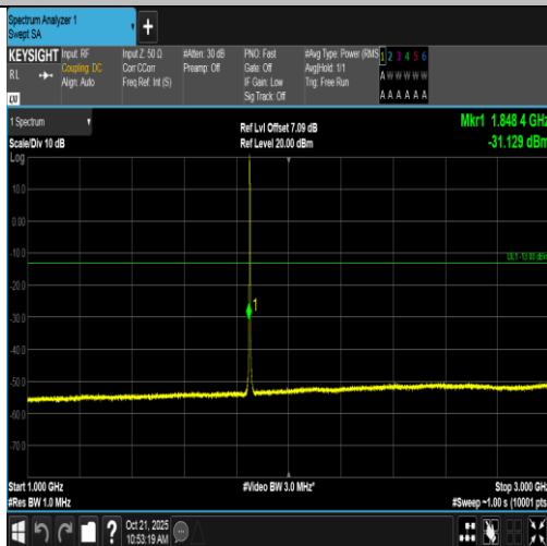
Band2-1.4MHz-16QAM-18607-6RB#0-1000~3000-PASS
