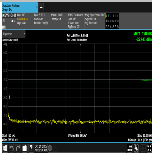
Band2-1.4MHz-16QAM-18607-6RB#0-0.15~30-PASS
