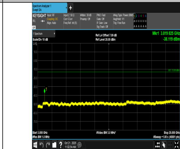
Band2-1.4MHz-QPSK-19193-1RB#5-3000~20000-PASS
