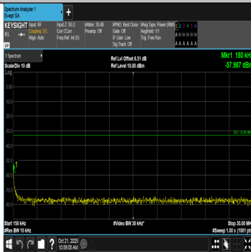
Band2-1.4MHz-16QAM-18900-6RB#0-0.15~30-PASS
