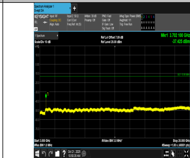
Band2-1.4MHz-QPSK-18607-1RB#5-3000~20000-PASS
