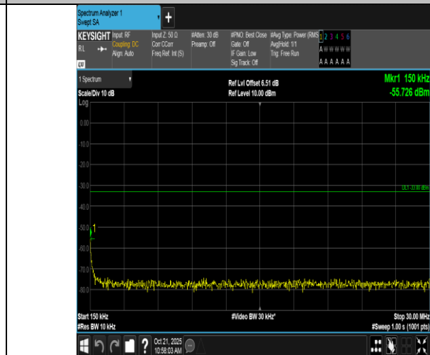
Band2-1.4MHz-QPSK-18900-6RB#0-0.15~30-PASS
