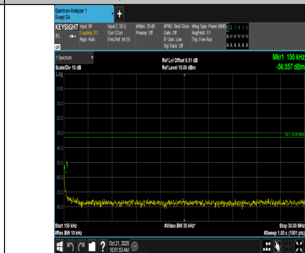
Band2-1.4MHz-QPSK-18607-6RB#0-0.15~30-PASS
