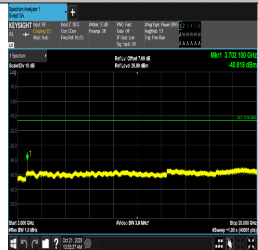
Band2-1.4MHz-16QAM-18607-6RB#0-3000~20000-PASS
