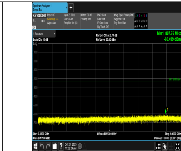
Band2-1.4MHz-QPSK-19193-1RB#5-30~1000-PASS
