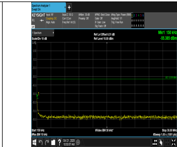
Band2-1.4MHz-QPSK-18900-1RB#0-0.15~30-PASS
