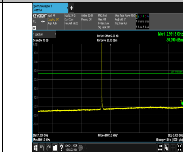
Band2-1.4MHz-QPSK-18900-1RB#0-1000~3000-PASS
