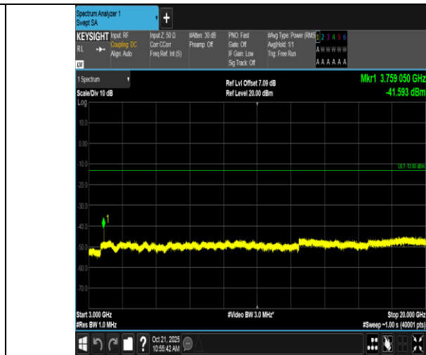
Band2-1.4MHz-16QAM-18900-1RB#0-3000~20000-PASS
