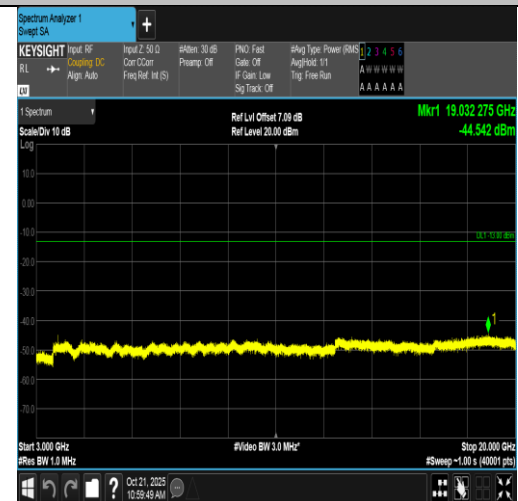
Band2-1.4MHz-16QAM-18900-6RB#0-3000~20000-PASS
