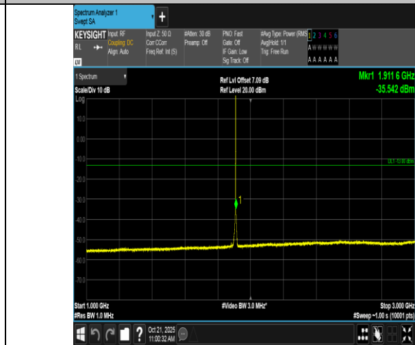
Band2-1.4MHz-QPSK-19193-1RB#0-1000~3000-PASS
