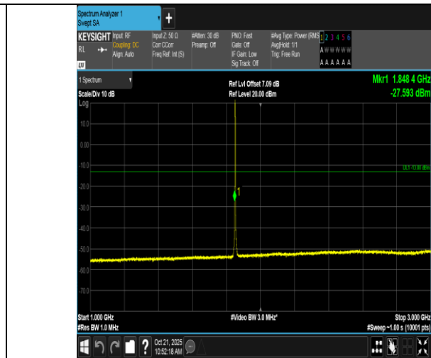
Band2-1.4MHz-QPSK-18607-6RB#0-1000~3000-PASS
