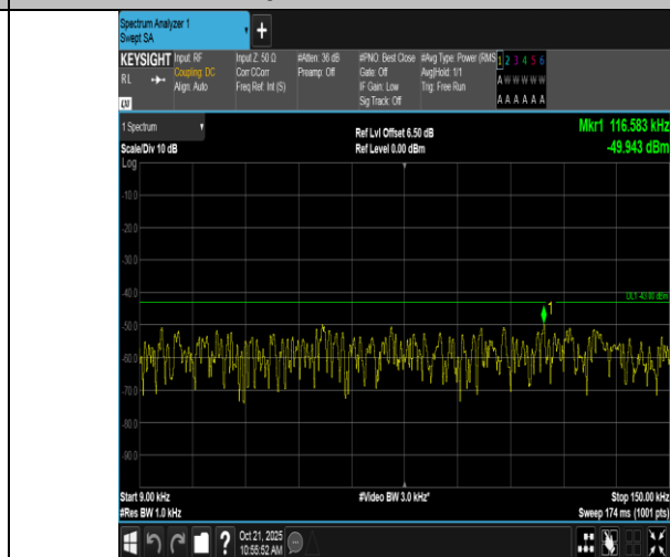
Band2-1.4MHz-QPSK-18900-1RB#5-0.009~0.15-PASS
