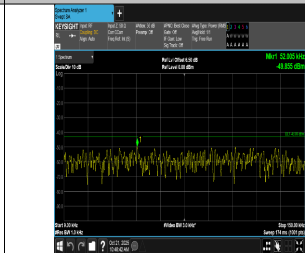
Band2-1.4MHz-16QAM-18607-1RB#0-0.009~0.15-PASS
