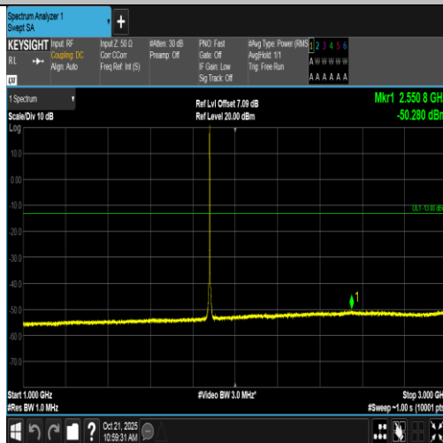
Band2-1.4MHz-16QAM-18900-6RB#0-1000~3000-PASS
