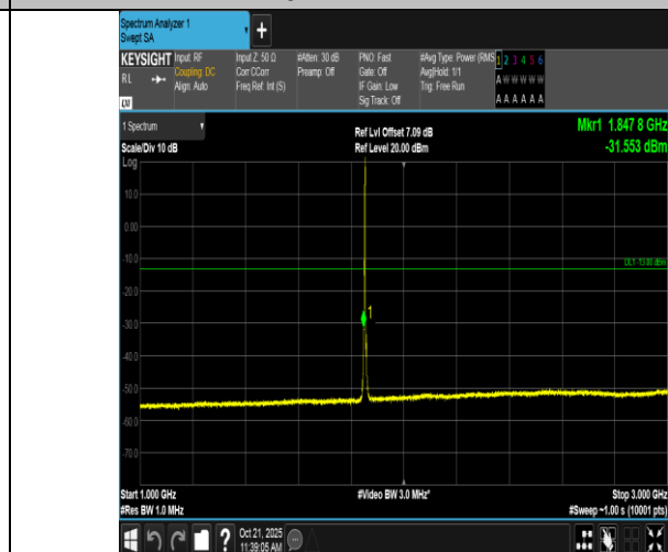
Band2-3MHz-16QAM-18615-1RB#14-1000~3000-PASS
