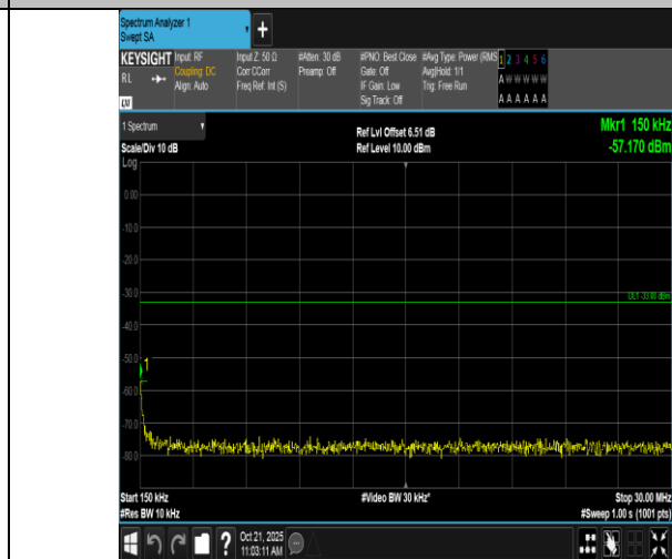
Band2-1.4MHz-16QAM-19193-1RB#5-0.15~30-PASS
