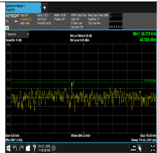
Band2-3MHz-16QAM-18615-15RB#0-0.009~0.15-PASS
