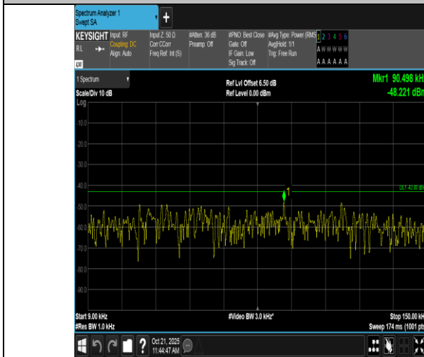
Band2-3MHz-16QAM-18900-1RB#14-0.009~0.15-PASS
