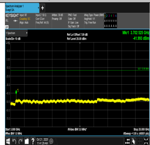
Band2-3MHz-16QAM-18615-15RB#0-3000~20000-PASS
