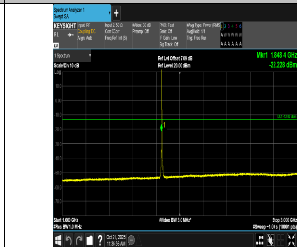
Band2-3MHz-QPSK-18615-1RB#0-1000~3000-PASS
