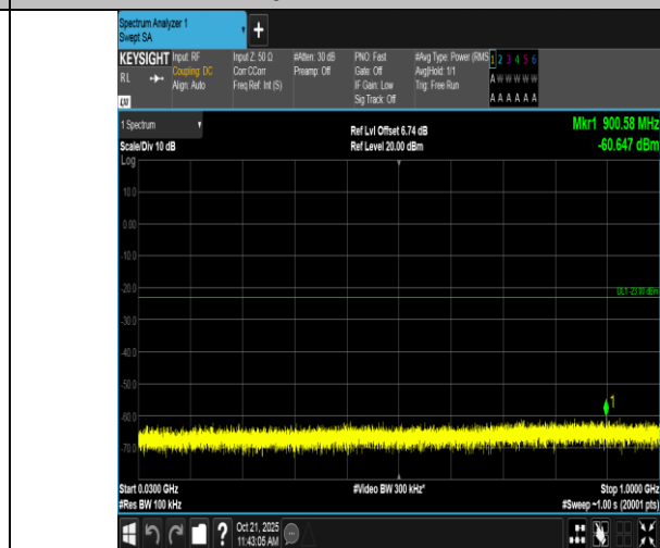
Band2-3MHz-16QAM-18900-1RB#0-30~1000-PASS
