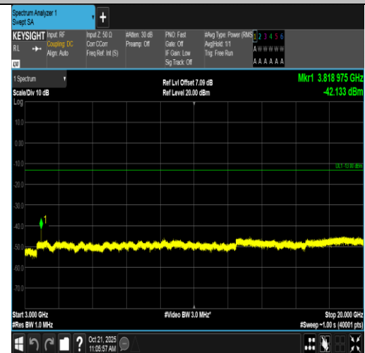
Band2-1.4MHz-16QAM-19193-6RB#0-3000~20000-PASS
