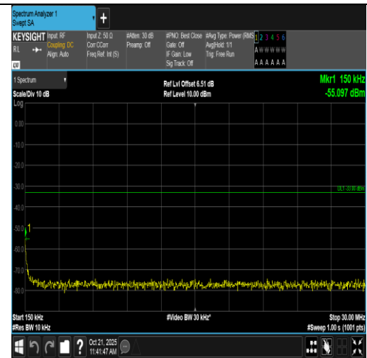
Band2-3MHz-QPSK-18900-1RB#0-0.15~30-PASS
