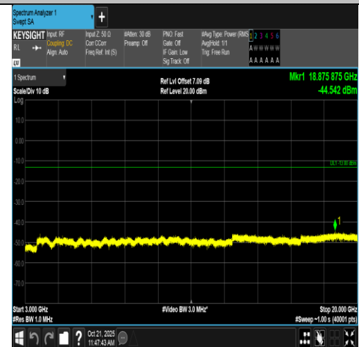
Band2-3MHz-16QAM-18900-15RB#0-3000~20000-PASS
