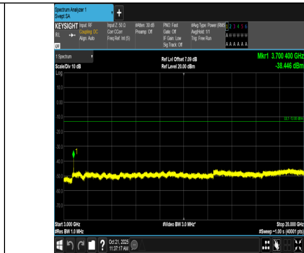
Band2-3MHz-16QAM-18615-1RB#0-3000~20000-PASS
