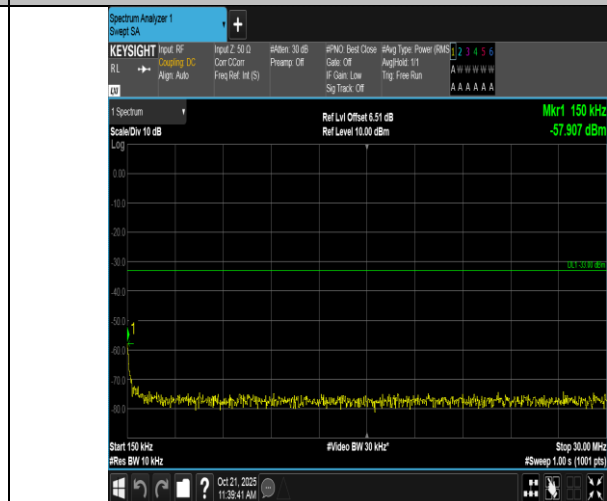
Band2-3MHz-QPSK-18615-15RB#0-0.15~30-PASS
