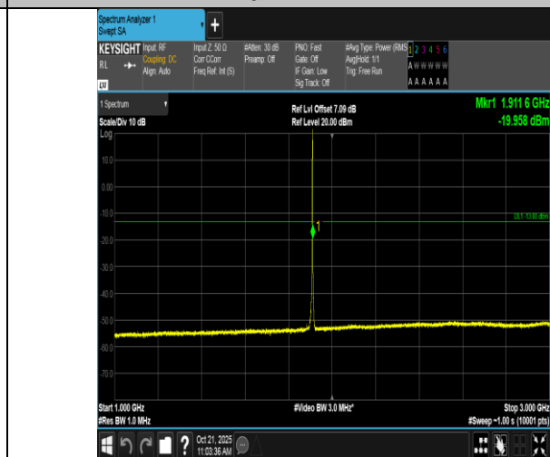
Band2-1.4MHz-16QAM-19193-1RB#5-1000~3000-PASS
