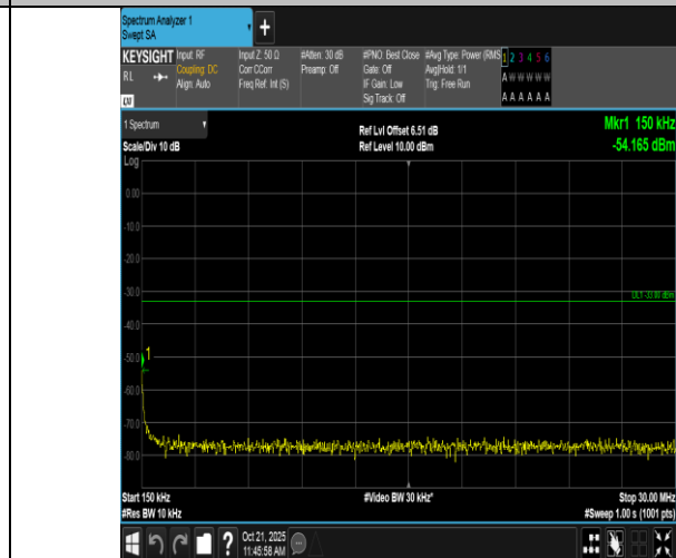
Band2-3MHz-QPSK-18900-15RB#0-0.15~30-PASS
