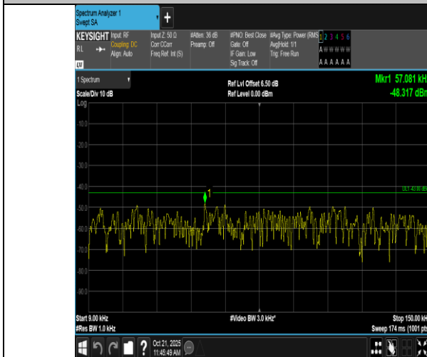
Band2-3MHz-QPSK-18900-15RB#0-0.009~0.15-PASS
