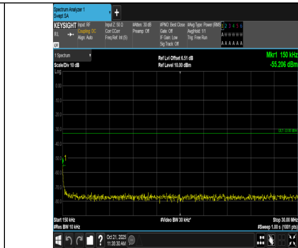
Band2-3MHz-QPSK-18615-1RB#0-0.15~30-PASS
