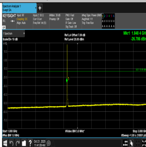
Band2-3MHz-16QAM-18615-15RB#0-1000~3000-PASS
