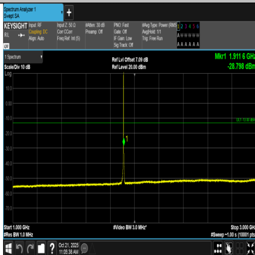
Band2-1.4MHz-16QAM-19193-6RB#0-1000~3000-PASS
