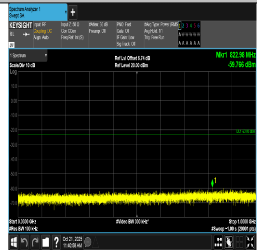
Band2-3MHz-16QAM-18615-15RB#0-30~1000-PASS
