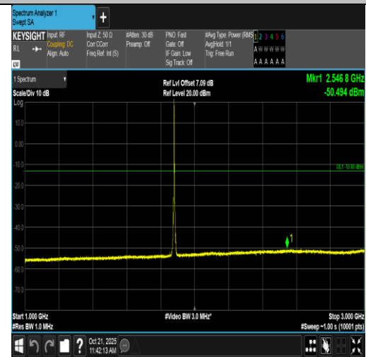
Band2-3MHz-QPSK-18900-1RB#0-1000~3000-PASS
