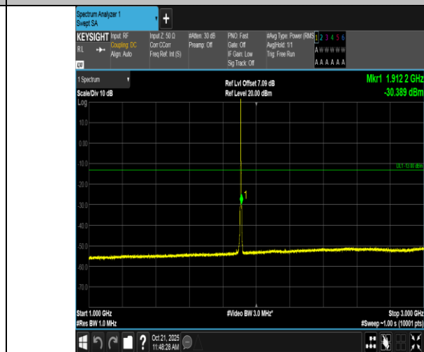
Band2-3MHz-QPSK-19185-1RB#0-1000~3000-PASS
