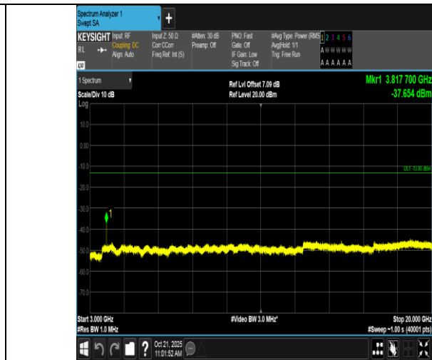
Band2-1.4MHz-16QAM-19193-1RB#0-3000~20000-PASS
