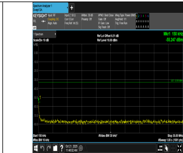
Band2-3MHz-QPSK-19185-1RB#0-0.15~30-PASS
