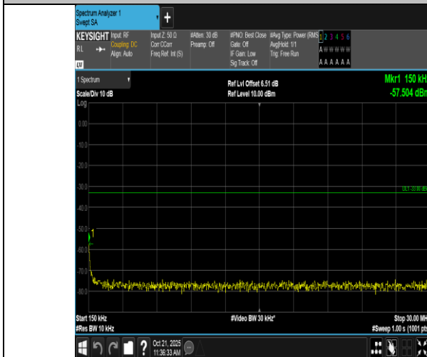
Band2-3MHz-16QAM-18615-1RB#0-0.15~30-PASS
