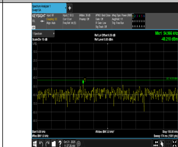
Band2-3MHz-QPSK-18615-1RB#14-0.009~0.15-PASS
