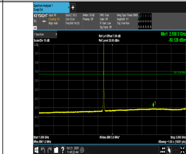
Band2-3MHz-16QAM-18900-1RB#14-1000~3000-PASS
