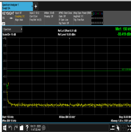
Band2-3MHz-16QAM-18900-15RB#0-0.15~30-PASS
