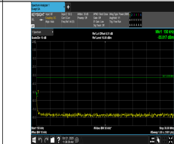
Band2-3MHz-16QAM-18615-1RB#14-0.15~30-PASS
