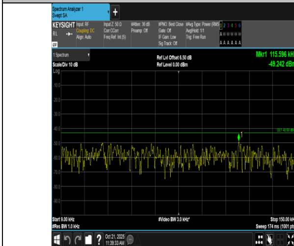
Band2-3MHz-QPSK-18615-15RB#0-0.009~0.15-PASS
