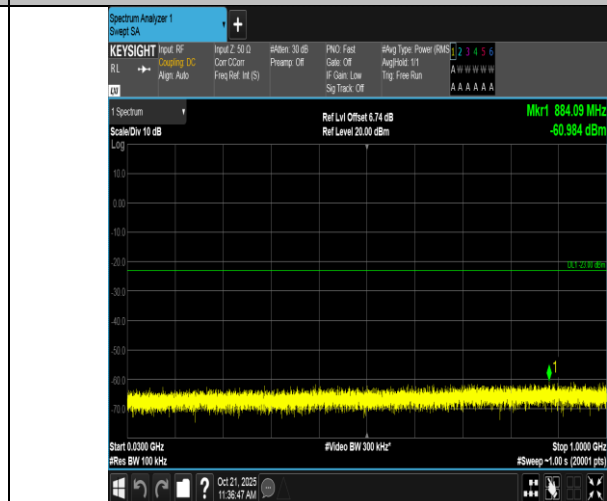
Band2-3MHz-16QAM-18615-1RB#0-30~1000-PASS
