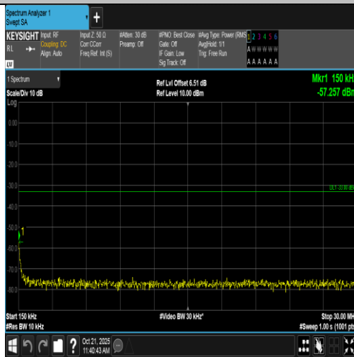
Band2-3MHz-16QAM-18615-15RB#0-0.15~30-PASS
