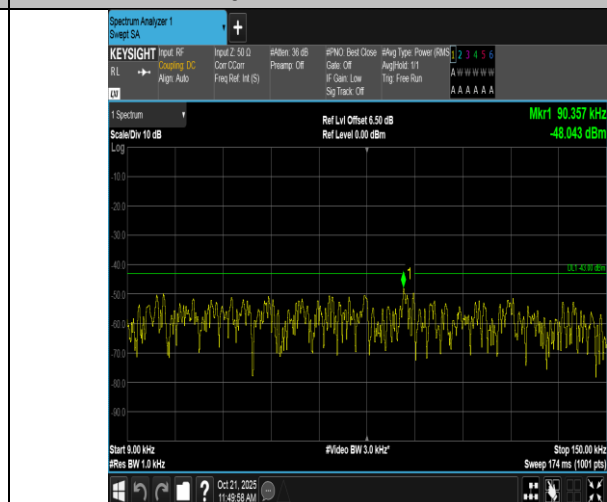
Band2-3MHz-QPSK-19185-1RB#14-0.009~0.15-PASS
