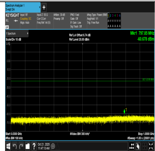
Band2-3MHz-16QAM-18900-15RB#0-30~1000-PASS
