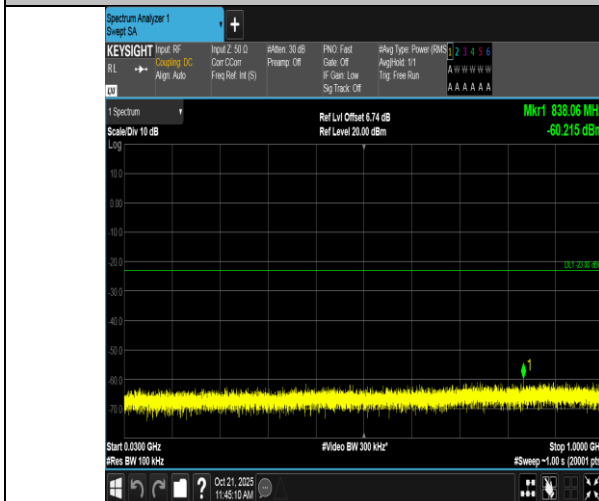
Band2-3MHz-16QAM-18900-1RB#14-30~1000-PASS
