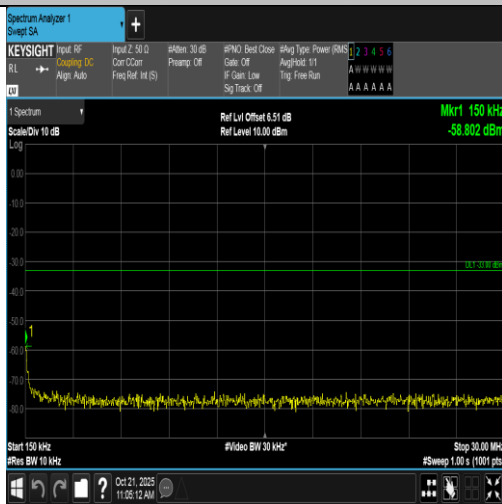
Band2-1.4MHz-16QAM-19193-6RB#0-0.15~30-PASS
