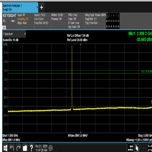
Band2-3MHz-16QAM-18900-15RB#0-1000~3000-PASS
