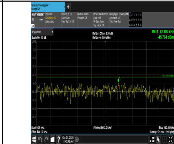
Band2-3MHz-16QAM-18900-1RB#0-0.009~0.15-PASS
