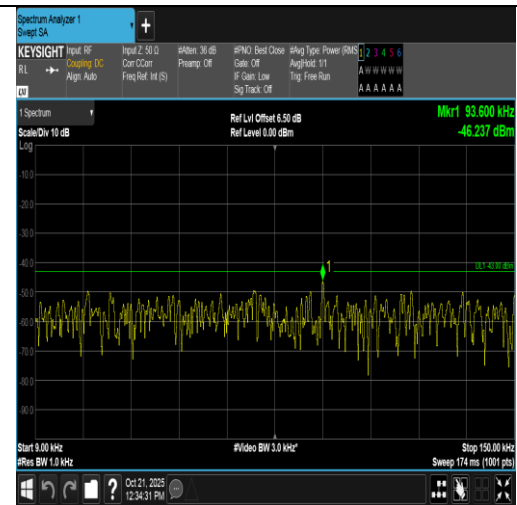
Band2-5MHz-16QAM-18900-25RB#0-0.009~0.15-PASS
