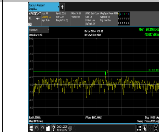
Band2-5MHz-16QAM-18900-1RB#0-0.009~0.15-PASS
