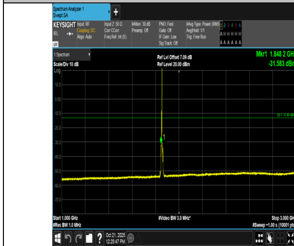
Band2-5MHz-QPSK-18625-1RB#24-1000~3000-PASS
