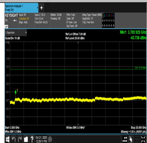
Band2-5MHz-16QAM-18625-25RB#0-3000~20000-PASS
