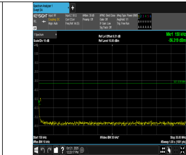
Band2-5MHz-QPSK-18625-1RB#0-0.15~30-PASS
