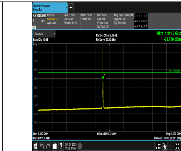
Band2-3MHz-QPSK-19185-15RB#0-1000~3000-PASS
