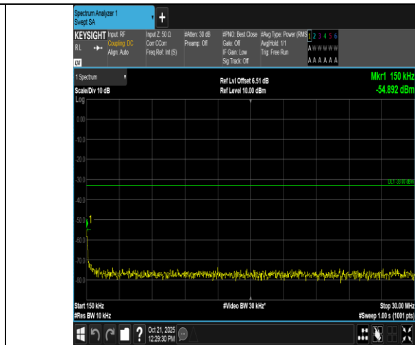
Band2-5MHz-QPSK-18900-1RB#0-0.15~30-PASS
