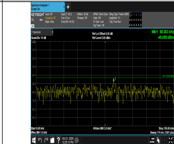
Band2-5MHz-QPSK-18625-1RB#24-0.009~0.15-PASS
