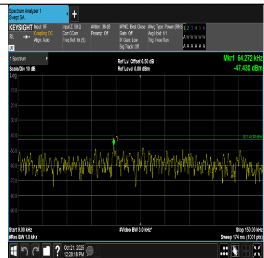
Band2-5MHz-16QAM-18625-25RB#0-0.009~0.15-PASS
