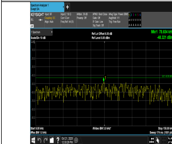
Band2-5MHz-QPSK-18900-25RB#0-0.009~0.15-PASS
