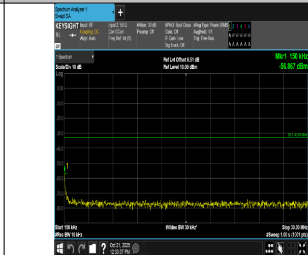
Band2-5MHz-QPSK-18900-25RB#0-0.15~30-PASS
