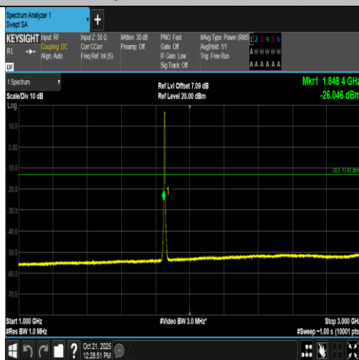
Band2-5MHz-16QAM-18625-25RB#0-1000~3000-PASS
