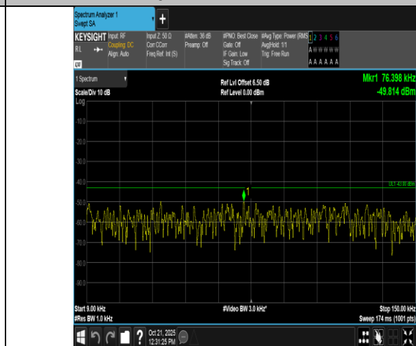
Band2-5MHz-QPSK-18900-1RB#24-0.009~0.15-PASS
