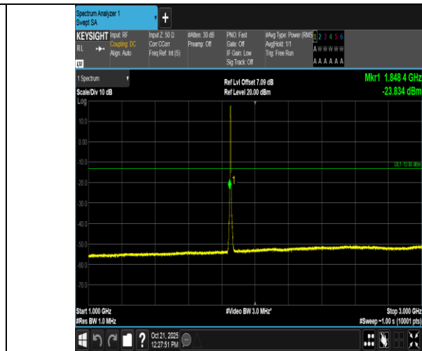
Band2-5MHz-QPSK-18625-25RB#0-1000~3000-PASS
