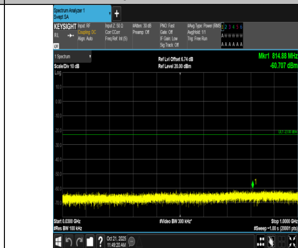
Band2-3MHz-16QAM-19185-1RB#0-30~1000-PASS
