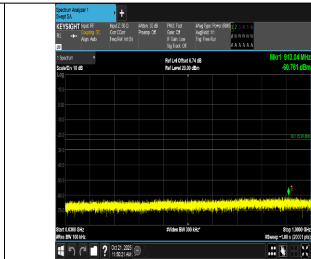
Band2-3MHz-QPSK-19185-1RB#14-30~1000-PASS
