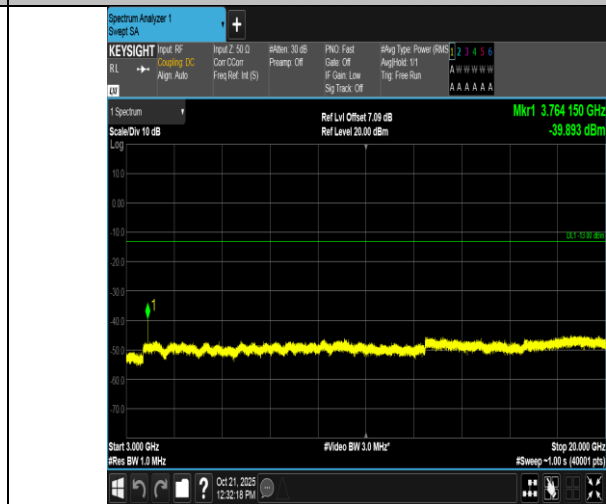
Band2-5MHz-QPSK-18900-1RB#24-3000~20000-PASS
