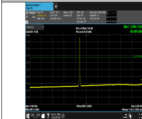
Band2-5MHz-16QAM-18900-25RB#0-1000~3000-PASS
