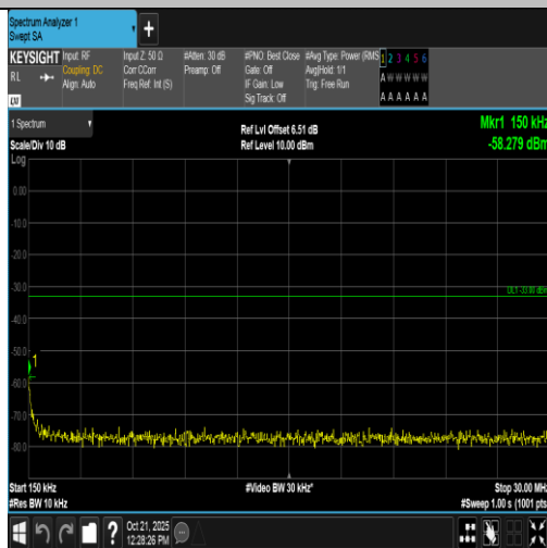
Band2-5MHz-16QAM-18625-25RB#0-0.15~30-PASS
