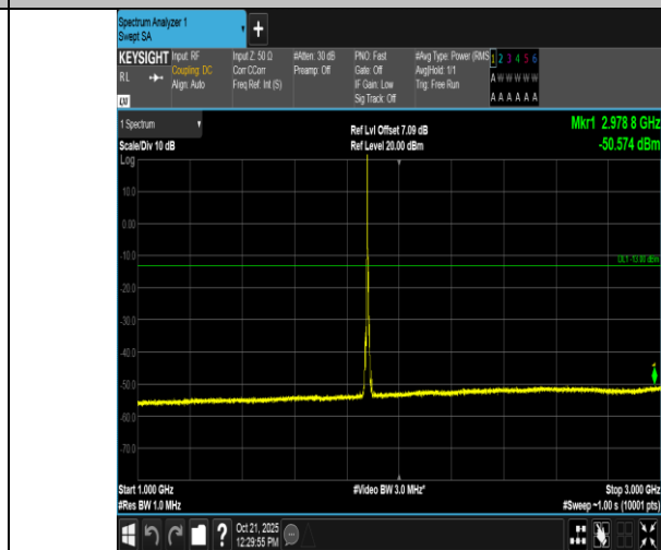
Band2-5MHz-QPSK-18900-1RB#0-1000~3000-PASS
