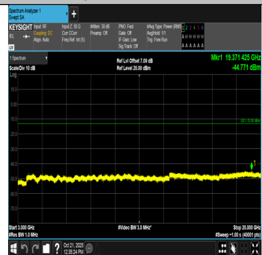
Band2-5MHz-16QAM-18900-25RB#0-3000~20000-PASS
