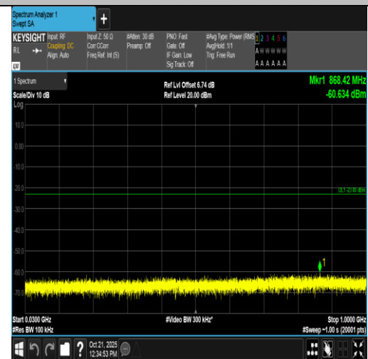
Band2-5MHz-16QAM-18900-25RB#0-30~1000-PASS
