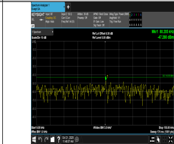
Band2-3MHz-16QAM-19185-1RB#0-0.009~0.15-PASS
