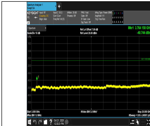
Band2-5MHz-16QAM-18900-1RB#24-3000~20000-PASS
