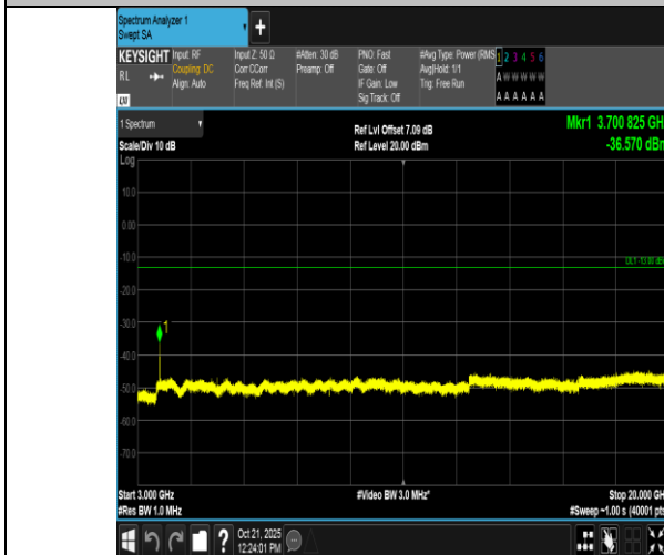
Band2-5MHz-QPSK-18625-1RB#0-3000~20000-PASS
