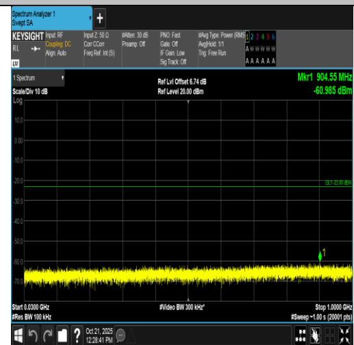
Band2-5MHz-16QAM-18625-25RB#0-30~1000-PASS
