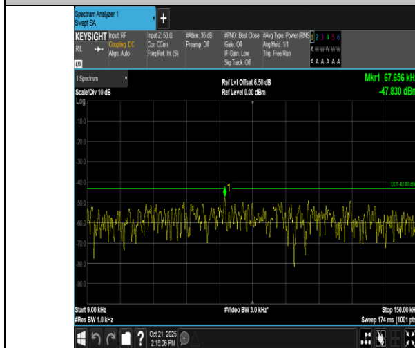
Band2-10MHz-16QAM-19150-1RB#49-0.009~0.15-PASS
