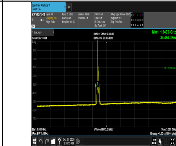
Band2-15MHz-QPSK-18900-1RB#0-1000~3000-PASS
