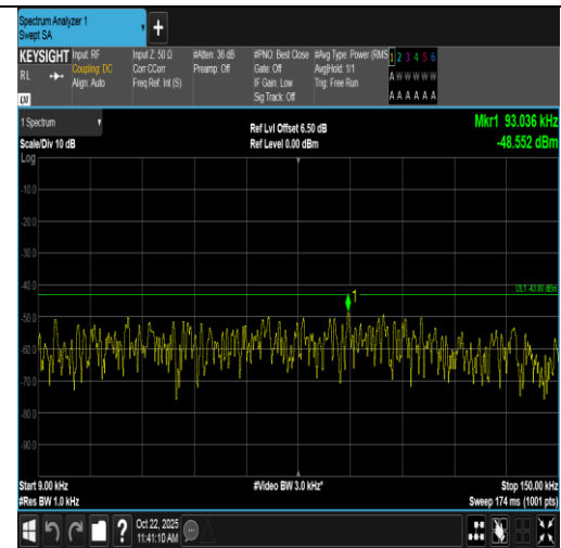
Band2-15MHz-16QAM-18675-75RB#0-0.009~0.15-PASS
