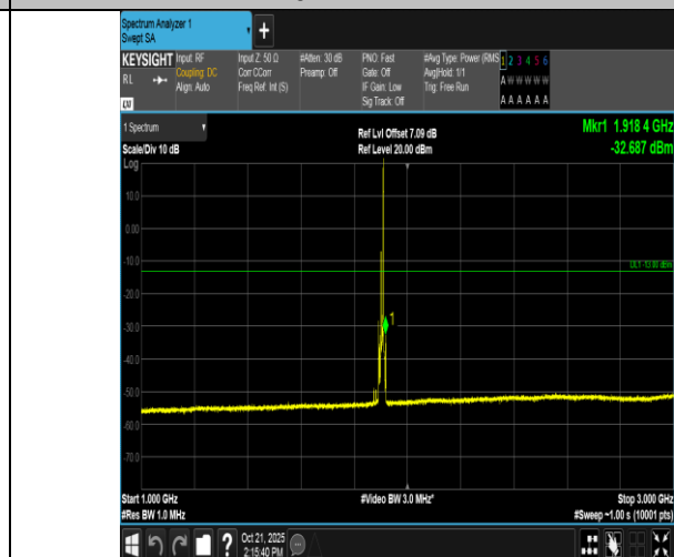
Band2-10MHz-16QAM-19150-1RB#49-1000~3000-PASS
