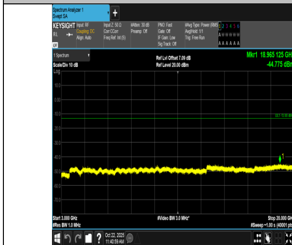
Band2-15MHz-QPSK-18675-75RB#0-3000~20000-PASS
