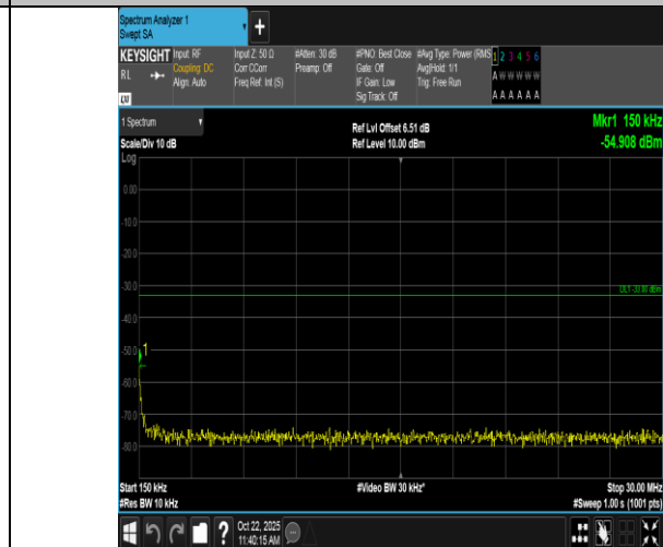
Band2-15MHz-QPSK-18675-75RB#0-0.15~30-PASS
