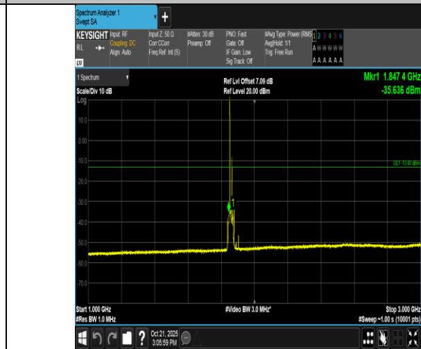
Band2-15MHz-QPSK-18675-1RB#0-1000~3000-PASS
