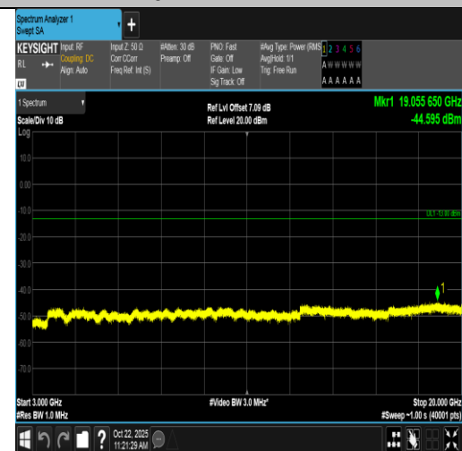
Band2-10MHz-16QAM-18900-50RB#0-3000~20000-PASS
