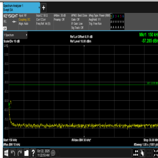
Band2-10MHz-16QAM-19150-50RB#0-0.15~30-PASS
