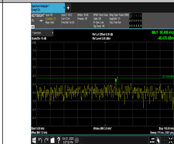
Band2-15MHz-QPSK-18675-1RB#74-0.009~0.15-PASS
