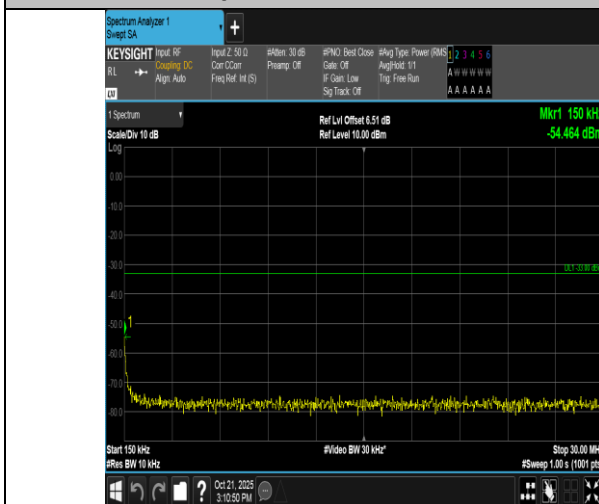
Band2-15MHz-16QAM-18900-1RB#0-0.15~30-PASS
