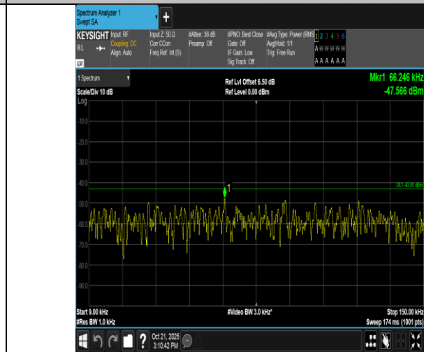
Band2-15MHz-16QAM-18900-1RB#0-0.009~0.15-PASS
