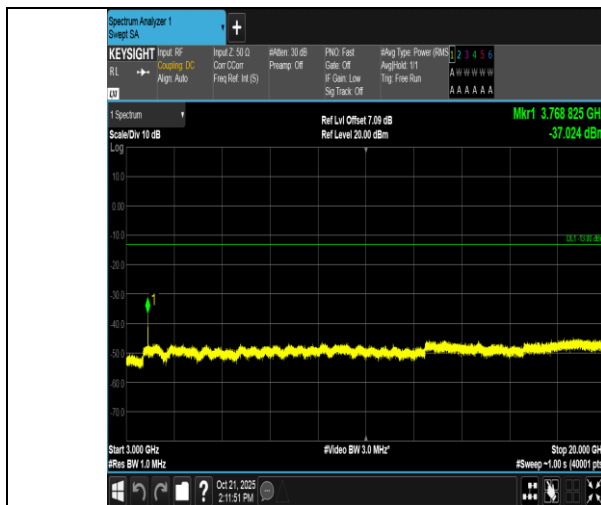
Band2-10MHz-16QAM-18900-1RB#49-3000~20000-PASS
