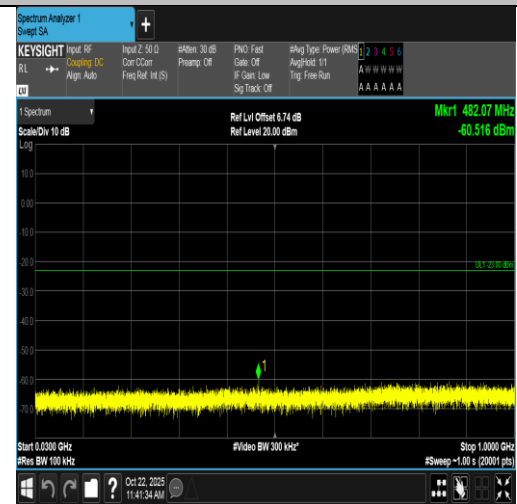
Band2-15MHz-16QAM-18675-75RB#0-30~1000-PASS
