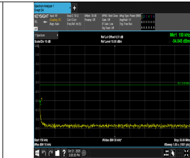
Band2-15MHz-QPSK-18675-1RB#0-0.15~30-PASS
