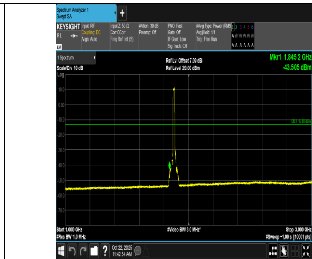
Band2-15MHz-QPSK-18900-75RB#0-1000~3000-PASS
