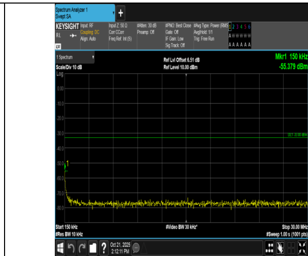
Band2-10MHz-QPSK-19150-1RB#0-0.15~30-PASS
