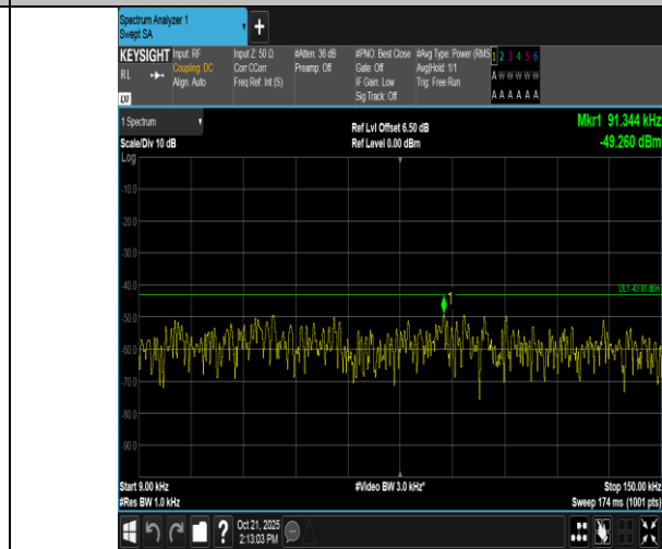
Band2-10MHz-16QAM-19150-1RB#0-0.009~0.15-PASS
