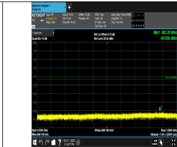
Band2-10MHz-QPSK-19150-1RB#49-30~1000-PASS
