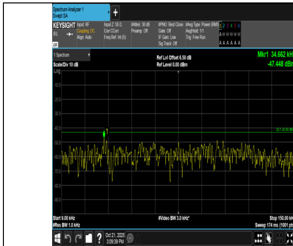
Band2-15MHz-QPSK-18900-1RB#0-0.009~0.15-PASS
