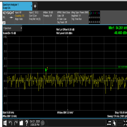
Band2-15MHz-16QAM-18675-1RB#74-0.009~0.15-PASS
