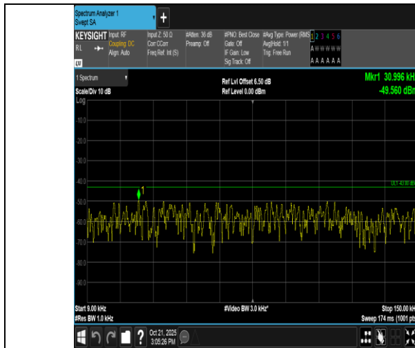
Band2-15MHz-QPSK-18675-1RB#0-0.009~0.15-PASS
