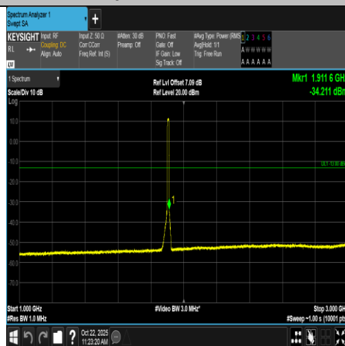
Band2-10MHz-16QAM-19150-50RB#0-1000~3000-PASS
