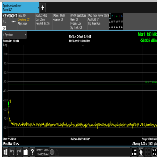
Band2-15MHz-16QAM-18675-75RB#0-0.15~30-PASS
