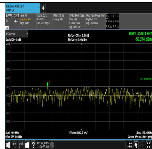
Band2-10MHz-16QAM-18900-50RB#0-0.009~0.15-PASS
