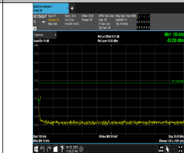
Band2-15MHz-QPSK-18900-75RB#0-0.15~30-PASS
