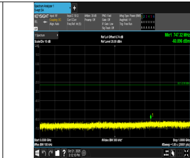
Band2-15MHz-QPSK-18900-1RB#74-30~1000-PASS
