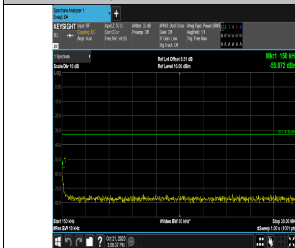
Band2-15MHz-16QAM-18675-1RB#0-0.15~30-PASS
