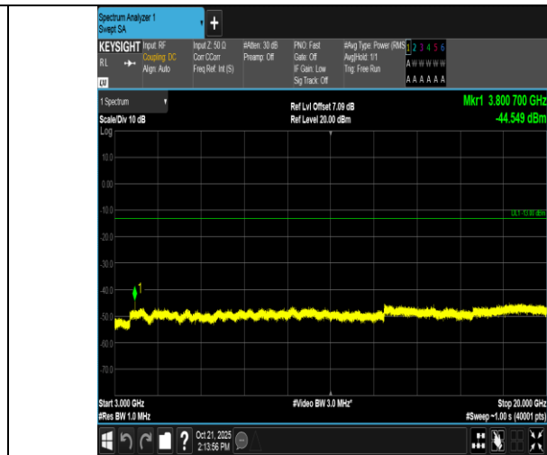
Band2-10MHz-16QAM-19150-1RB#0-3000~20000-PASS
