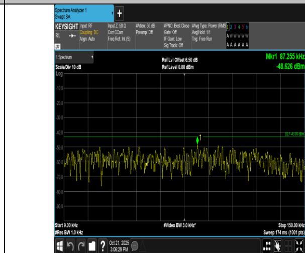
Band2-15MHz-16QAM-18675-1RB#0-0.009~0.15-PASS
