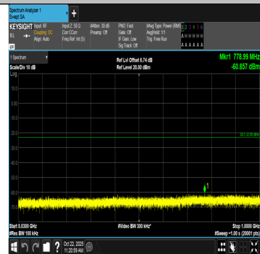
Band2-10MHz-16QAM-18900-50RB#0-30~1000-PASS
