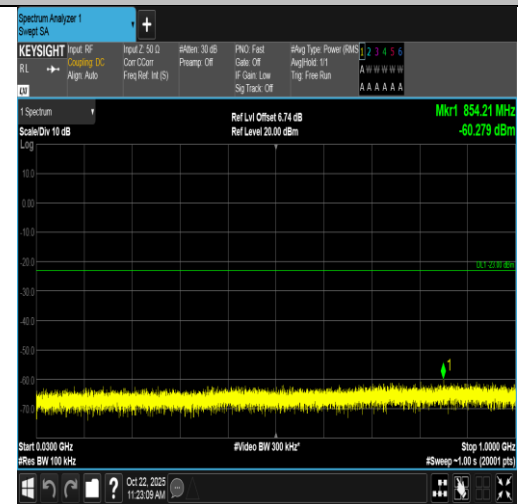
Band2-10MHz-16QAM-19150-50RB#0-30~1000-PASS
