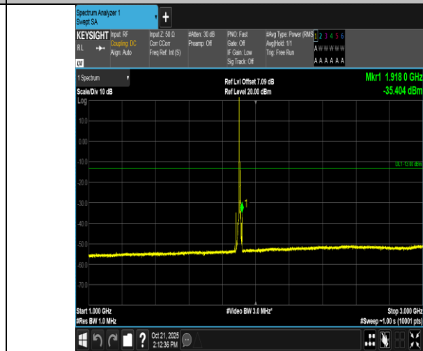
Band2-10MHz-QPSK-19150-1RB#0-1000~3000-PASS
