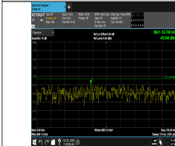
Band2-15MHz-QPSK-18675-75RB#0-0.009~0.15-PASS
