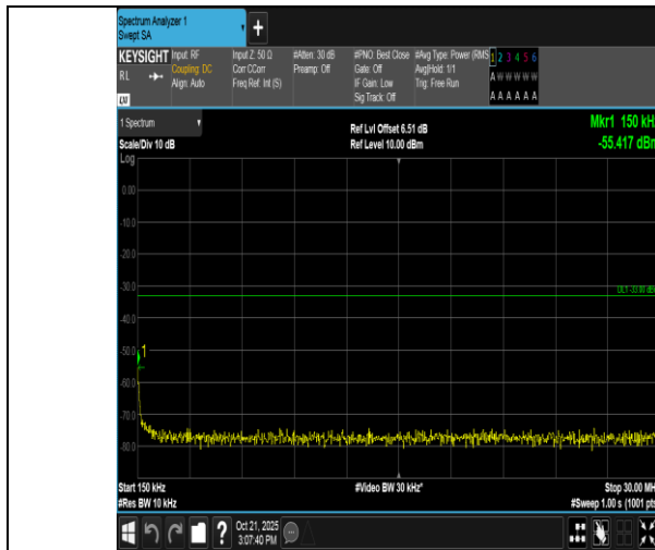
Band2-15MHz-QPSK-18675-1RB#74-0.15~30-PASS
