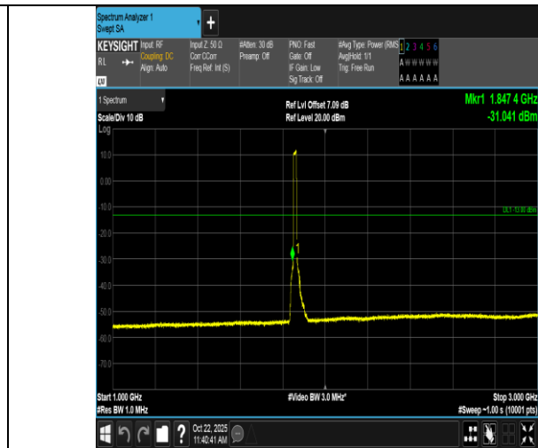
Band2-15MHz-QPSK-18675-75RB#0-1000~3000-PASS
