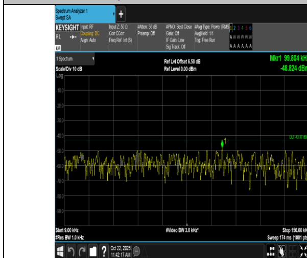
Band2-15MHz-QPSK-18900-75RB#0-0.009~0.15-PASS
