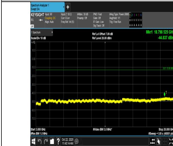
Band2-15MHz-QPSK-18900-75RB#0-3000~20000-PASS
