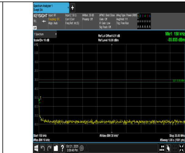
Band2-15MHz-QPSK-18900-1RB#0-0.15~30-PASS
