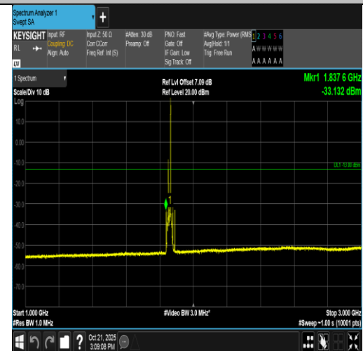
Band2-15MHz-16QAM-18675-1RB#74-1000~3000-PASS
