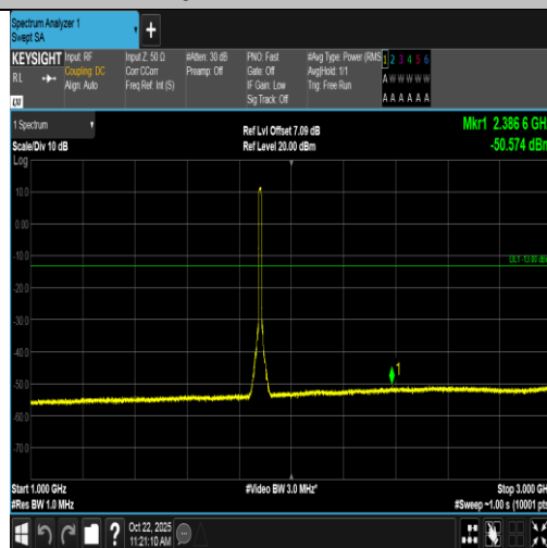
Band2-10MHz-16QAM-18900-50RB#0-1000~3000-PASS
