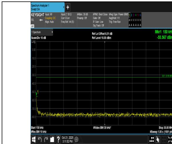
Band2-15MHz-QPSK-18900-1RB#74-0.15~30-PASS
