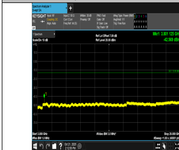
Band2-10MHz-QPSK-19150-1RB#0-3000~20000-PASS
