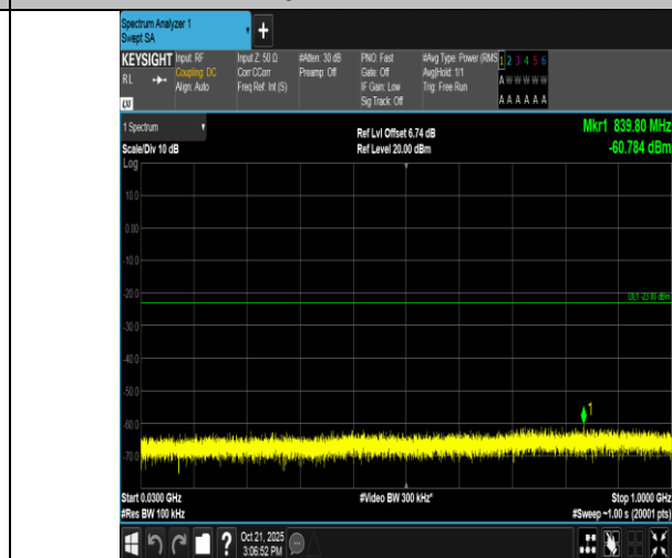
Band2-15MHz-16QAM-18675-1RB#0-30~1000-PASS
