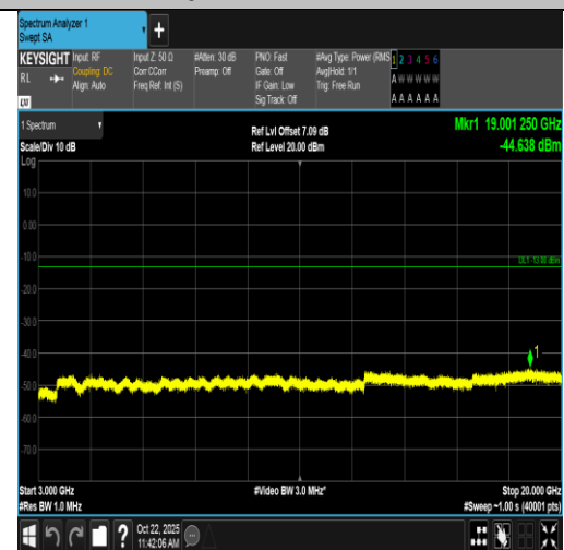
Band2-15MHz-16QAM-18675-75RB#0-3000~20000-PASS
