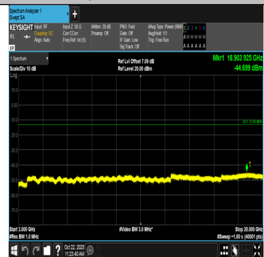
Band2-10MHz-16QAM-19150-50RB#0-3000~20000-PASS
