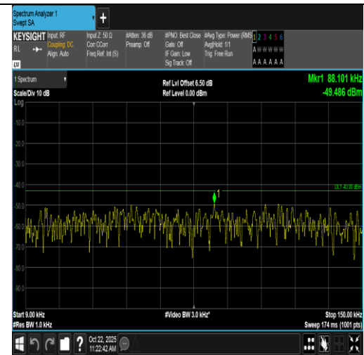
Band2-10MHz-16QAM-19150-50RB#0-0.009~0.15-PASS
