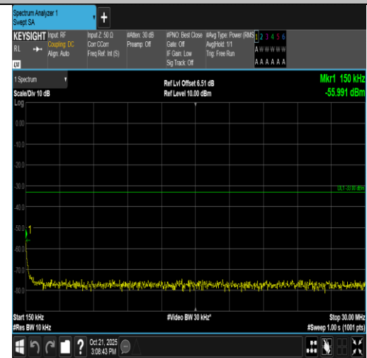
Band2-15MHz-16QAM-18675-1RB#74-0.15~30-PASS
