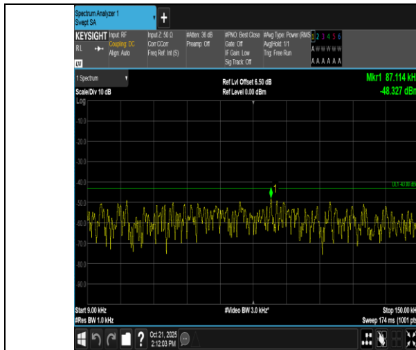
Band2-10MHz-QPSK-19150-1RB#0-0.009~0.15-PASS
