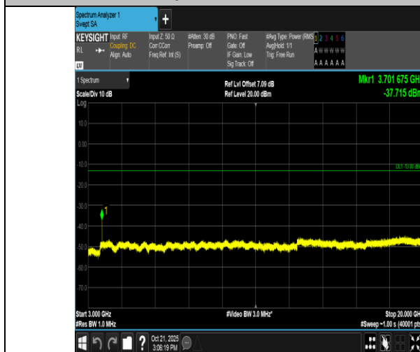
Band2-15MHz-QPSK-18675-1RB#0-3000~20000-PASS
