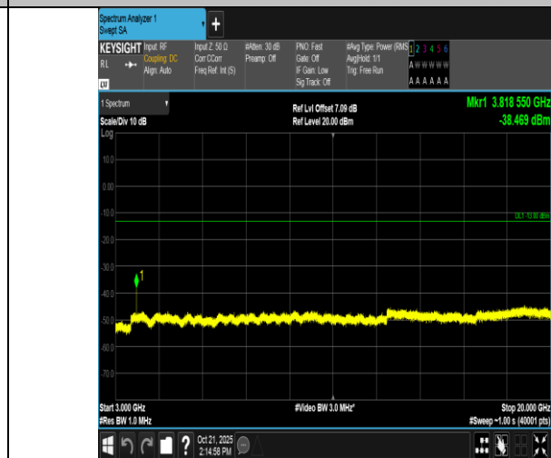
Band2-10MHz-QPSK-19150-1RB#49-3000~20000-PASS
