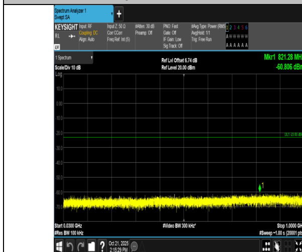
Band2-10MHz-16QAM-19150-1RB#49-30~1000-PASS
