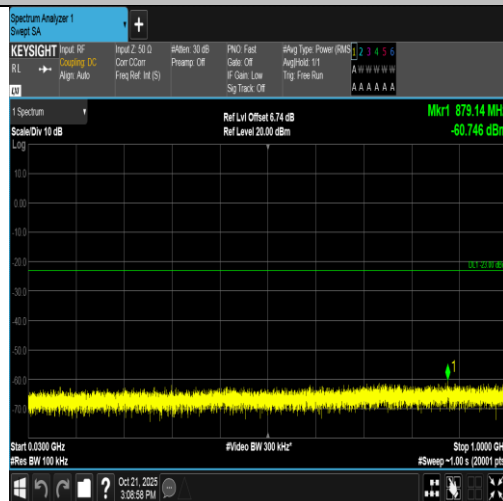
Band2-15MHz-16QAM-18675-1RB#74-30~1000-PASS
