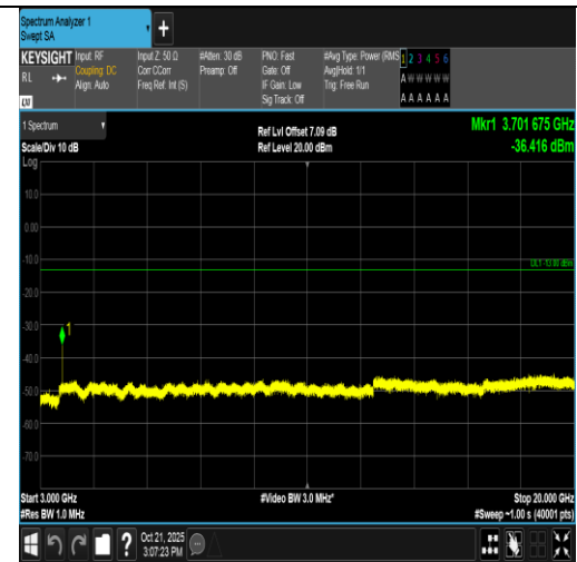
Band2-15MHz-16QAM-18675-1RB#0-3000~20000-PASS
