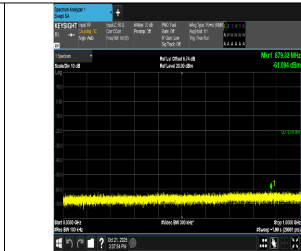
Band2-15MHz-QPSK-18675-1RB#74-30~1000-PASS
