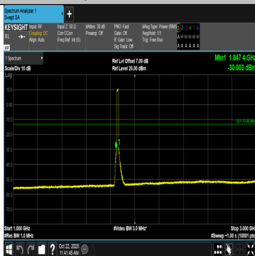
Band2-15MHz-16QAM-18675-75RB#0-1000~3000-PASS
