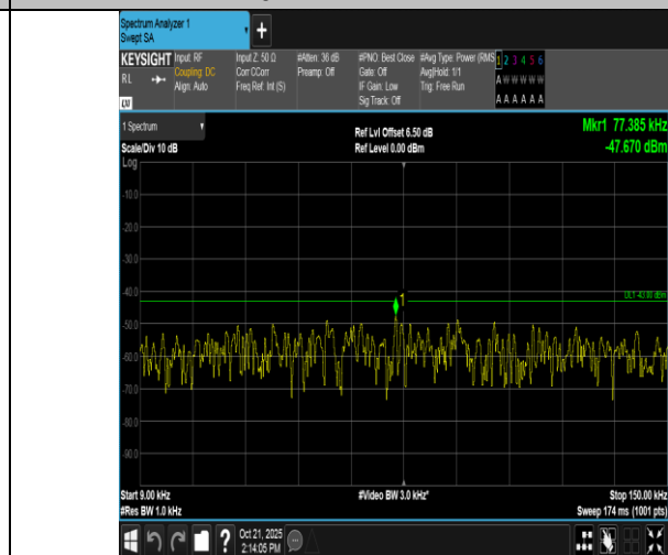
Band2-10MHz-QPSK-19150-1RB#49-0.009~0.15-PASS
