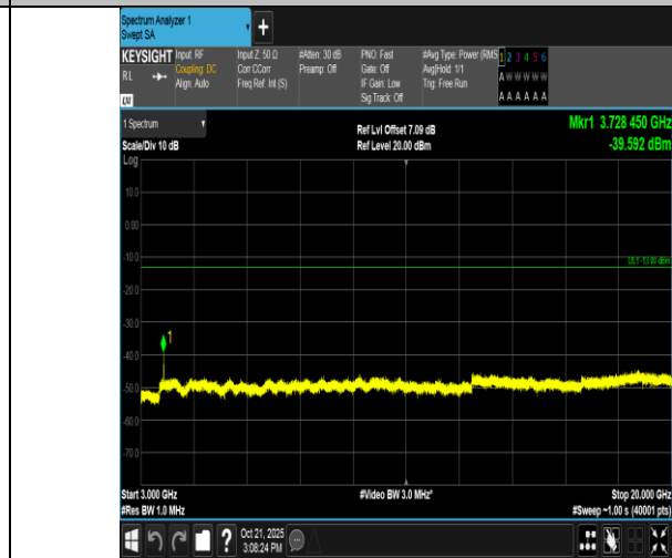
Band2-15MHz-QPSK-18675-1RB#74-3000~20000-PASS
