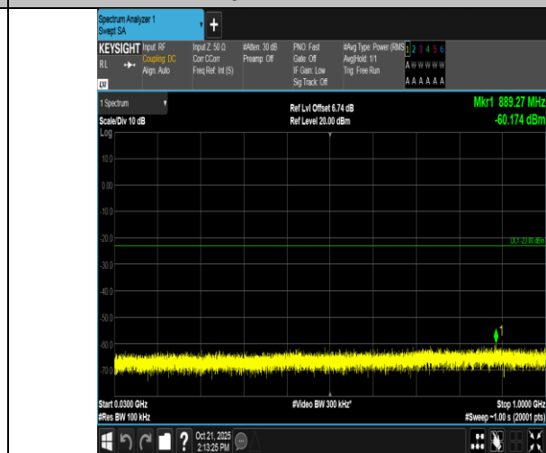
Band2-10MHz-16QAM-19150-1RB#0-30~1000-PASS
