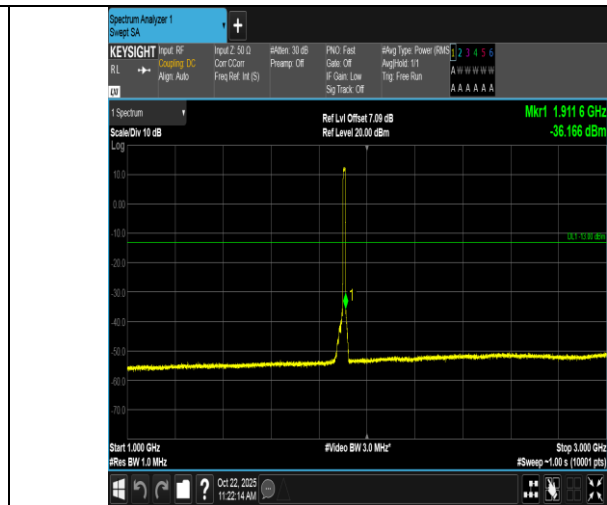
Band2-10MHz-QPSK-19150-50RB#0-1000~3000-PASS
