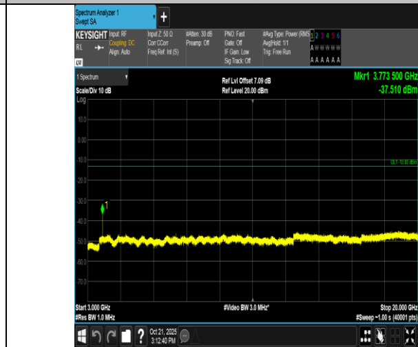
Band2-15MHz-QPSK-18900-1RB#74-3000~20000-PASS
