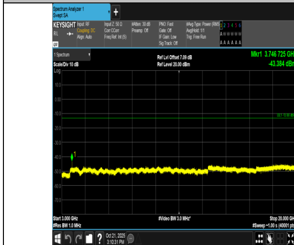
Band2-15MHz-QPSK-18900-1RB#0-3000~20000-PASS
