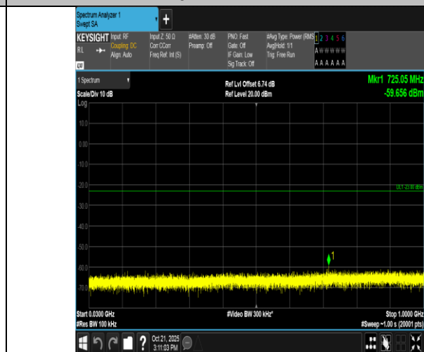
Band2-15MHz-16QAM-18900-1RB#0-30~1000-PASS
