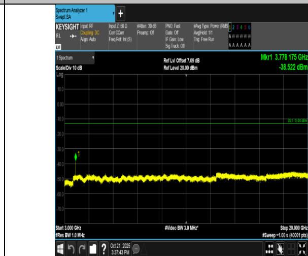
Band2-20MHz-QPSK-18900-1RB#99-3000~20000-PASS
