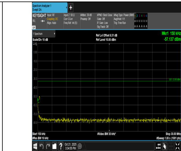
Band2-20MHz-QPSK-18900-1RB#0-0.15~30-PASS
