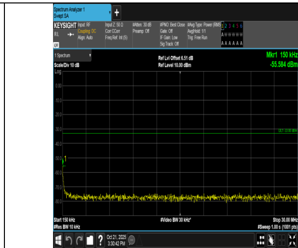
Band2-20MHz-QPSK-18700-1RB#0-0.15~30-PASS
