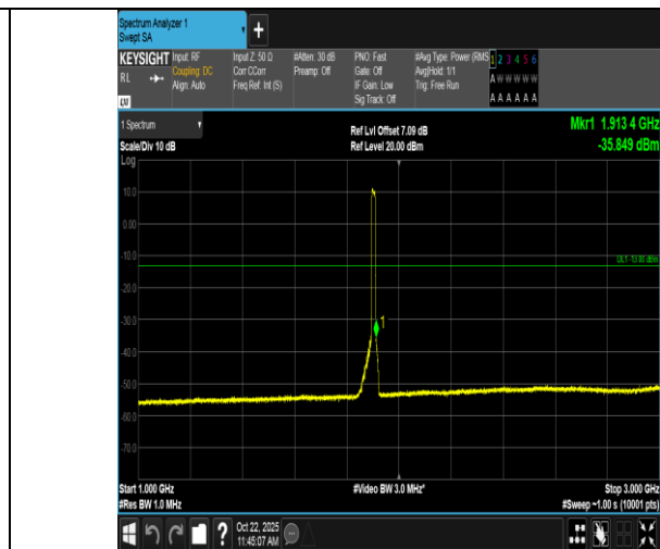
Band2-15MHz-QPSK-19125-75RB#0-1000~3000-PASS
