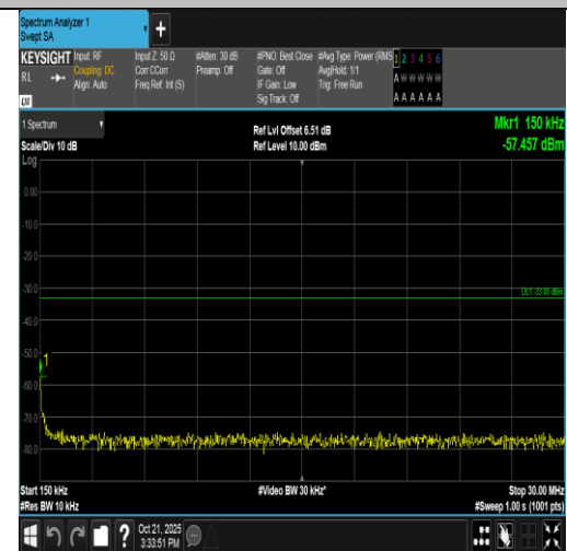
Band2-20MHz-16QAM-18700-1RB#99-0.15~30-PASS
