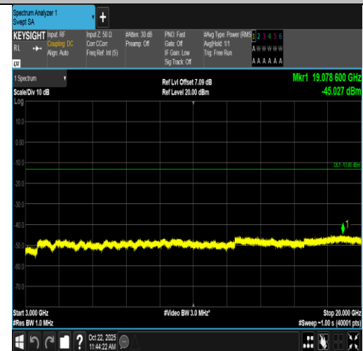
Band2-15MHz-16QAM-18900-75RB#0-3000~20000-PASS
