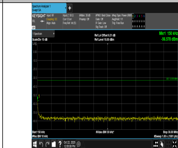
Band2-20MHz-QPSK-18900-100RB#0-0.15~30-PASS
