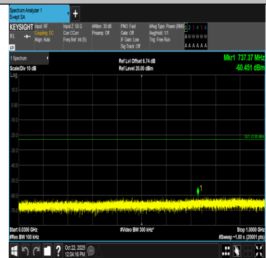
Band2-20MHz-16QAM-18700-100RB#0-30~1000-PASS
