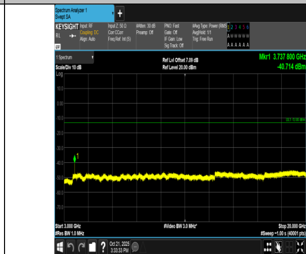
Band2-20MHz-QPSK-18700-1RB#99-3000~20000-PASS
