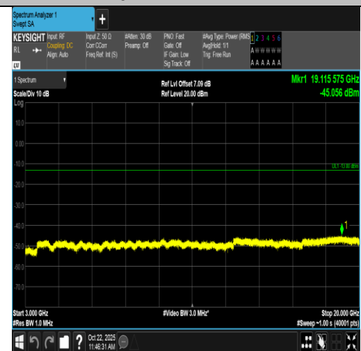
Band2-15MHz-16QAM-19125-75RB#0-3000~20000-PASS
