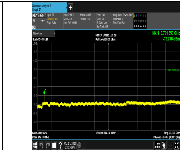
Band2-15MHz-16QAM-19125-1RB#0-3000~20000-PASS
