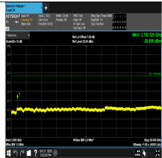
Band2-20MHz-16QAM-18700-1RB#0-3000~20000-PASS
