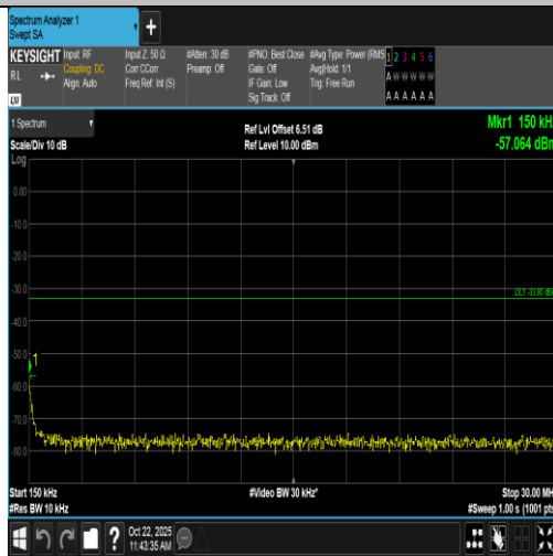
Band2-15MHz-16QAM-18900-75RB#0-0.15~30-PASS
