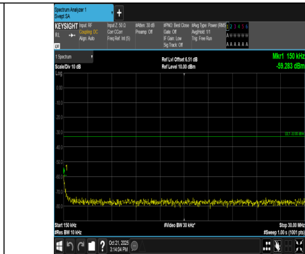
Band2-15MHz-QPSK-19125-1RB#0-0.15~30-PASS
