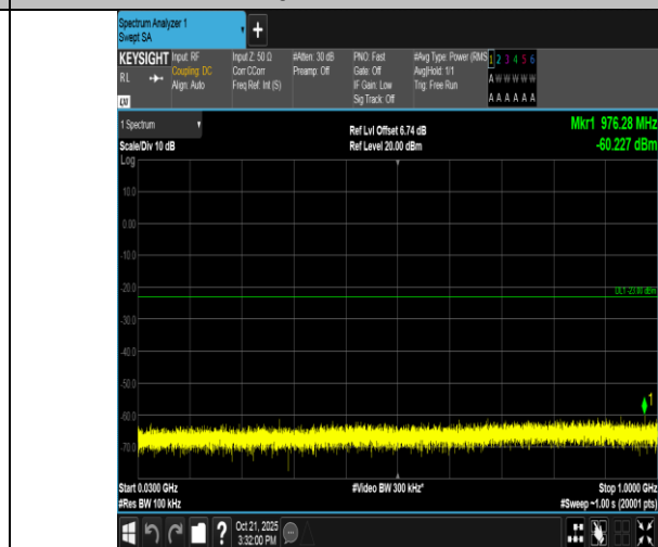
Band2-20MHz-16QAM-18700-1RB#0-30~1000-PASS
