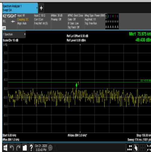
Band2-20MHz-16QAM-18700-1RB#99-0.009~0.15-PASS
