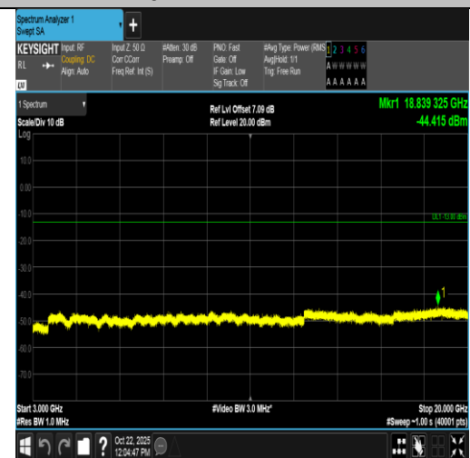
Band2-20MHz-16QAM-18700-100RB#0-3000~20000-PASS
