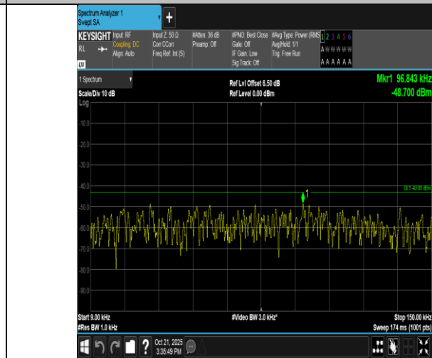
Band2-20MHz-16QAM-18900-1RB#0-0.009~0.15-PASS
