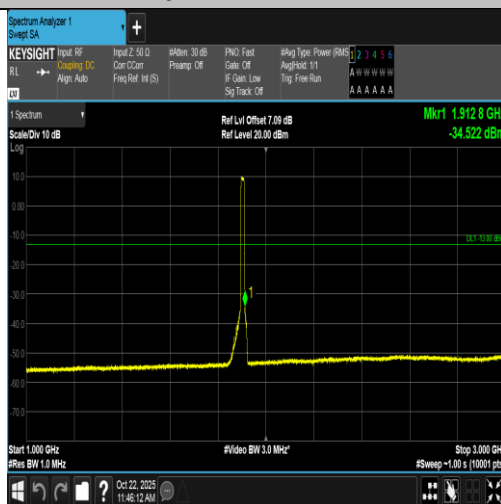
Band2-15MHz-16QAM-19125-75RB#0-1000~3000-PASS
