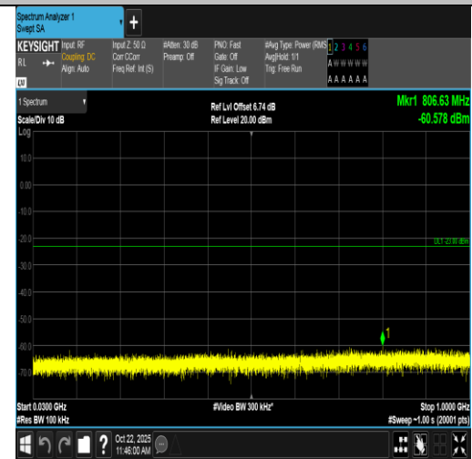
Band2-15MHz-16QAM-19125-75RB#0-30~1000-PASS
