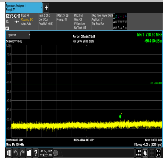
Band2-15MHz-16QAM-18900-75RB#0-30~1000-PASS
