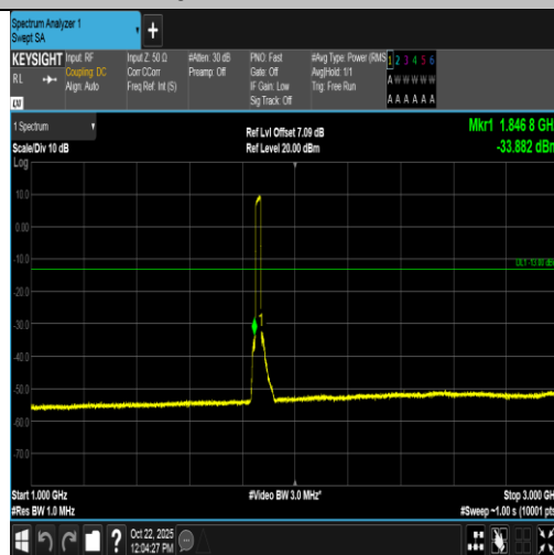
Band2-20MHz-16QAM-18700-100RB#0-1000~3000-PASS
