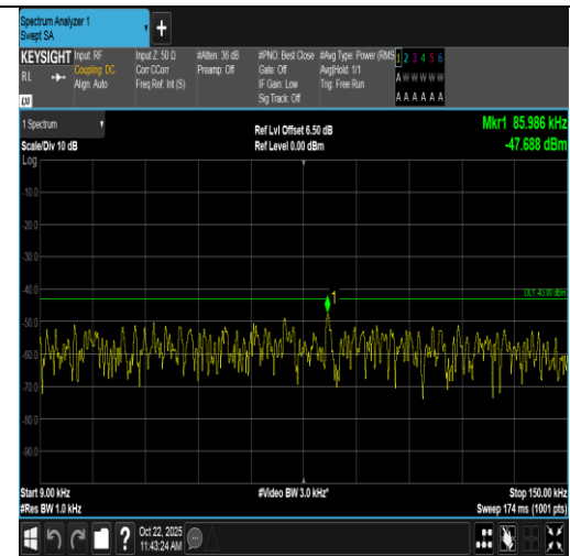
Band2-15MHz-16QAM-18900-75RB#0-0.009~0.15-PASS
