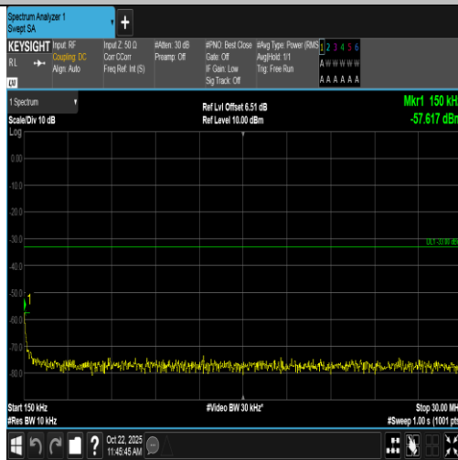
Band2-15MHz-16QAM-19125-75RB#0-0.15~30-PASS
