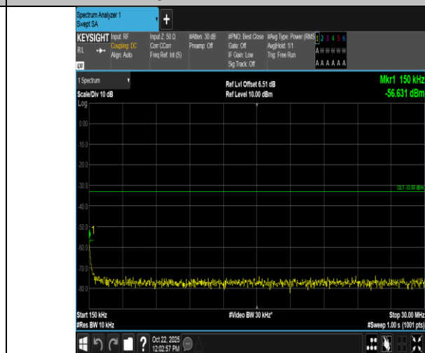
Band2-20MHz-QPSK-18700-100RB#0-0.15~30-PASS
