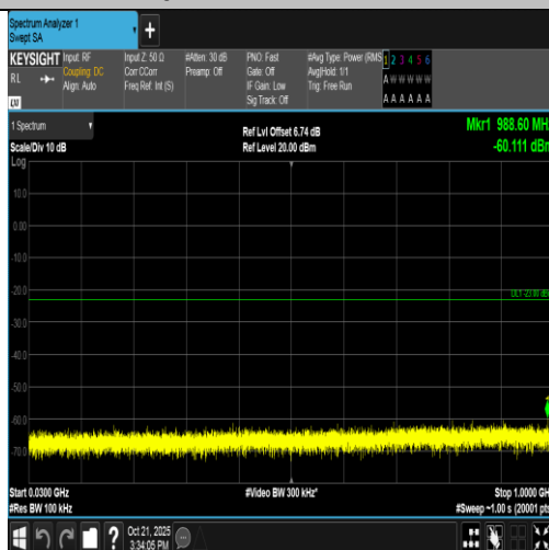
Band2-20MHz-16QAM-18700-1RB#99-30~1000-PASS
