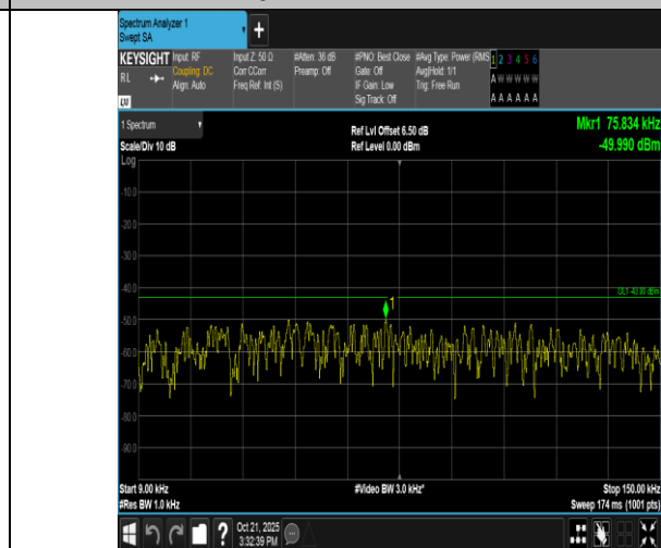
Band2-20MHz-QPSK-18700-1RB#99-0.009~0.15-PASS
