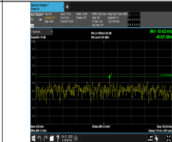
Band2-15MHz-QPSK-19125-1RB#74-0.009~0.15-PASS
