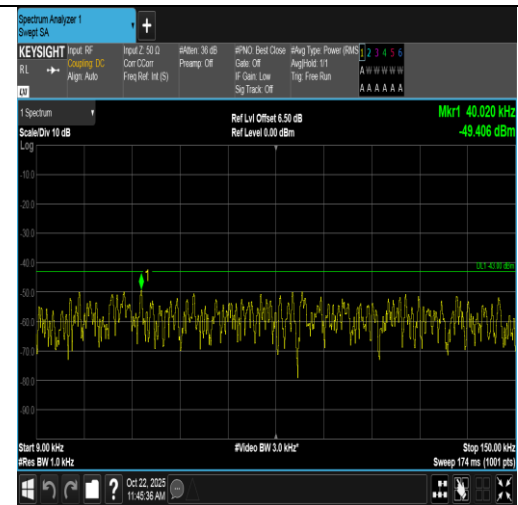
Band2-15MHz-16QAM-19125-75RB#0-0.009~0.15-PASS
