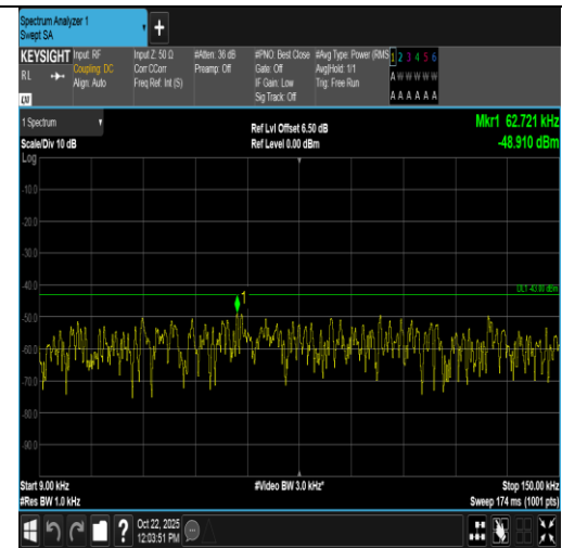
Band2-20MHz-16QAM-18700-100RB#0-0.009~0.15-PASS
