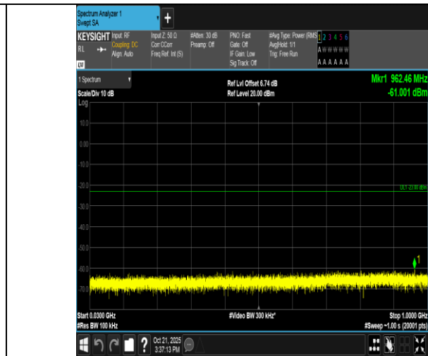
Band2-20MHz-QPSK-18900-1RB#99-30~1000-PASS
