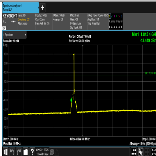
Band2-15MHz-16QAM-18900-75RB#0-1000~3000-PASS
