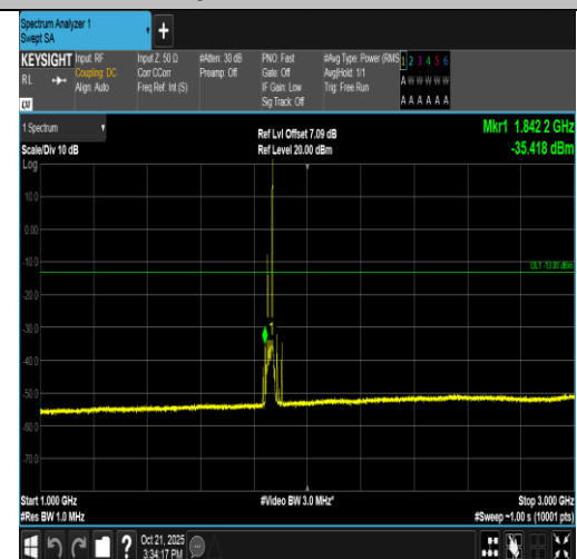
Band2-20MHz-16QAM-18700-1RB#99-1000~3000-PASS
