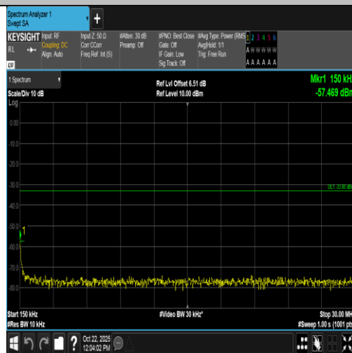
Band2-20MHz-16QAM-18700-100RB#0-0.15~30-PASS
