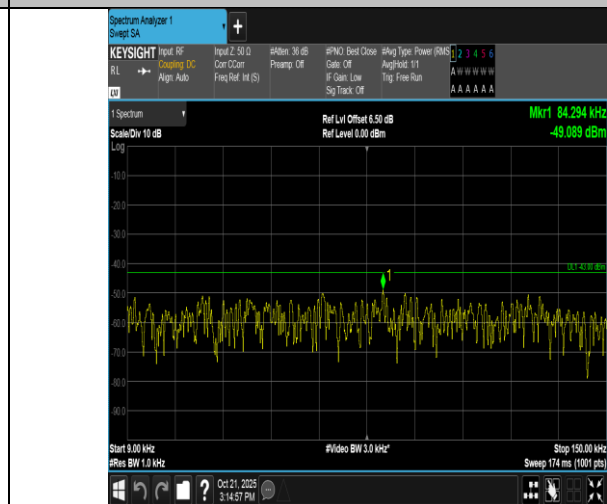
Band2-15MHz-16QAM-19125-1RB#0-0.009~0.15-PASS
