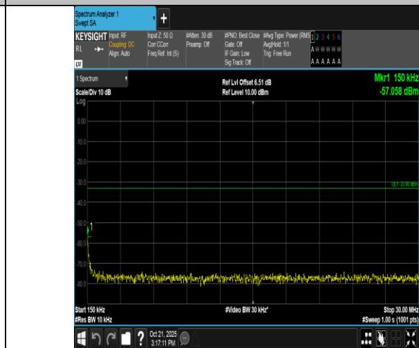
Band2-15MHz-16QAM-19125-1RB#74-0.15~30-PASS
