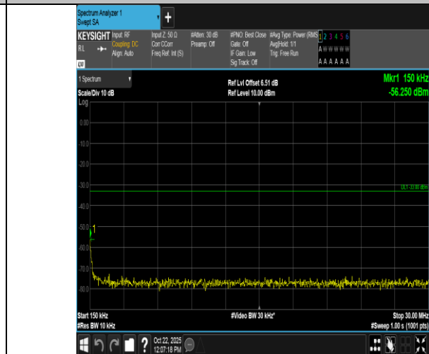
Band2-20MHz-QPSK-19100-100RB#0-0.15~30-PASS
