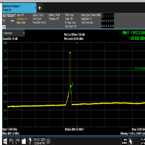
Band2-20MHz-16QAM-19100-100RB#0-1000~3000-PASS
