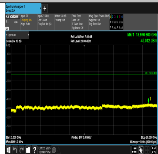
Band2-20MHz-16QAM-19100-100RB#0-3000~20000-PASS
