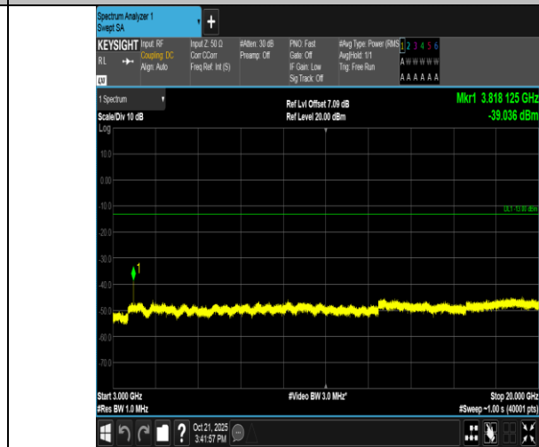
Band2-20MHz-QPSK-19100-1RB#99-3000~20000-PASS
