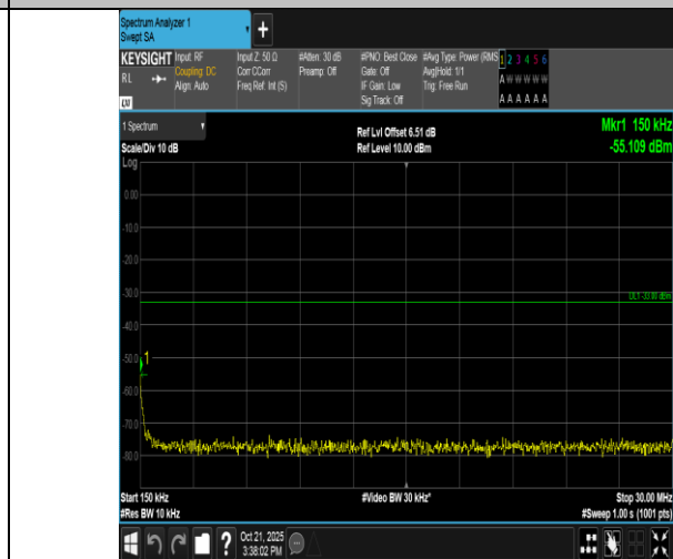
Band2-20MHz-16QAM-18900-1RB#99-0.15~30-PASS
