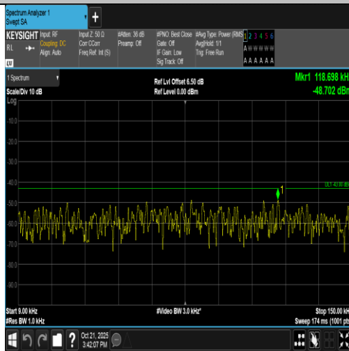
Band2-20MHz-16QAM-19100-1RB#99-0.009~0.15-PASS
