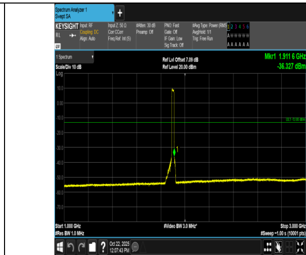
Band2-20MHz-QPSK-19100-100RB#0-1000~3000-PASS
