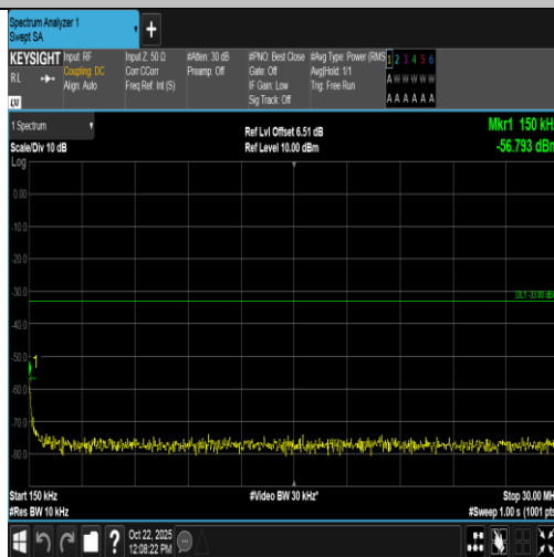
Band2-20MHz-16QAM-19100-100RB#0-0.15~30-PASS
