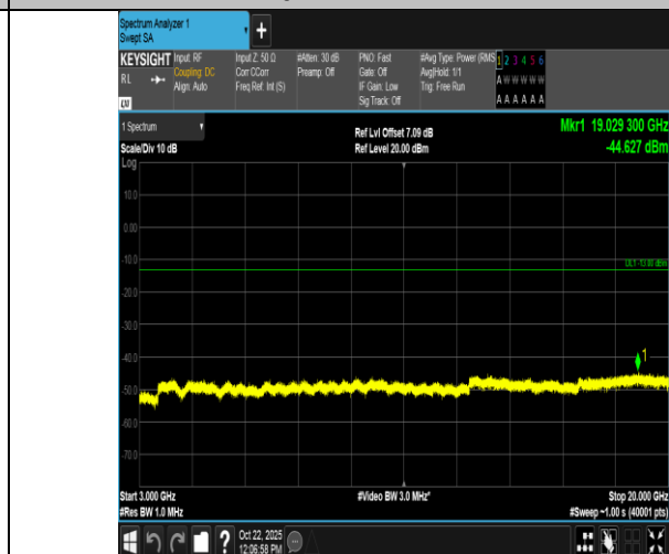
Band2-20MHz-16QAM-18900-100RB#0-3000~20000-PASS
