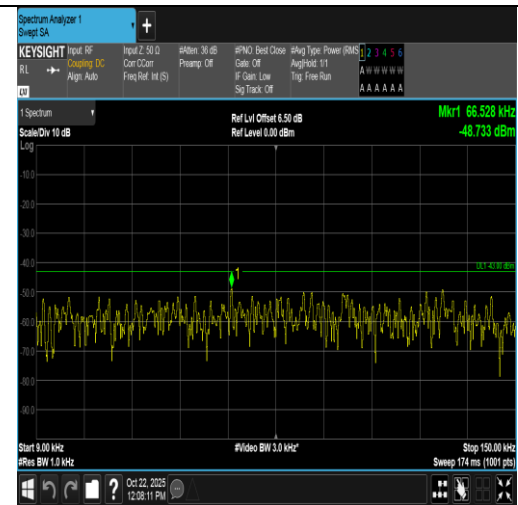
Band2-20MHz-16QAM-19100-100RB#0-0.009~0.15-PASS
