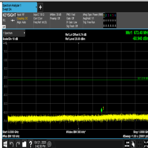
Band2-20MHz-16QAM-19100-1RB#99-30~1000-PASS
