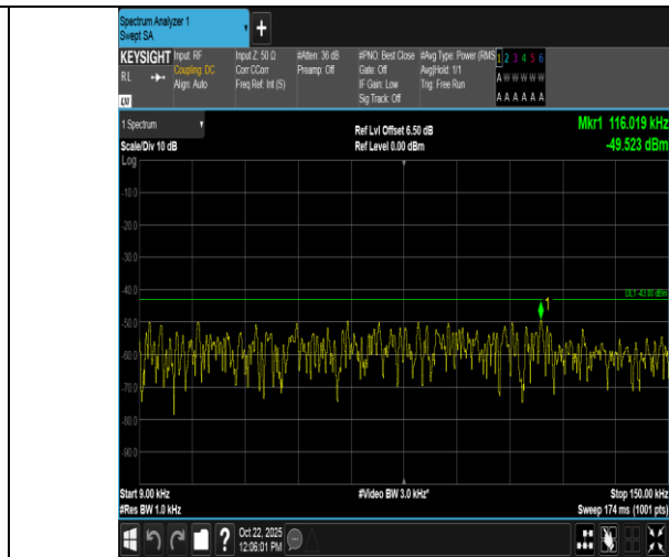
Band2-20MHz-16QAM-18900-100RB#0-0.009~0.15-PASS
