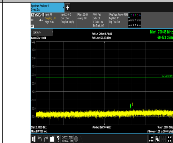
Band2-20MHz-16QAM-18900-100RB#0-30~1000-PASS
