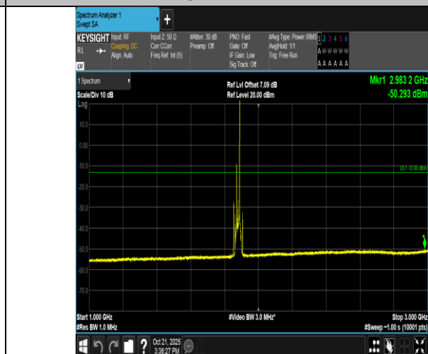
Band2-20MHz-16QAM-18900-1RB#99-1000~3000-PASS
