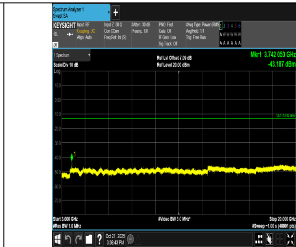
Band2-20MHz-16QAM-18900-1RB#0-3000~20000-PASS
