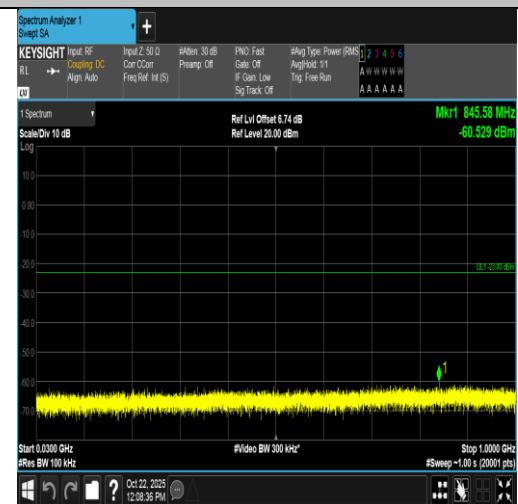
Band2-20MHz-16QAM-19100-100RB#0-30~1000-PASS
