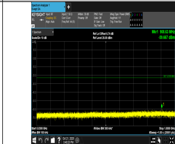
Band2-20MHz-16QAM-19100-1RB#0-30~1000-PASS
