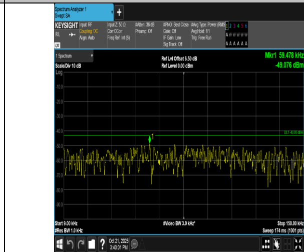
Band2-20MHz-16QAM-19100-1RB#0-0.009~0.15-PASS
