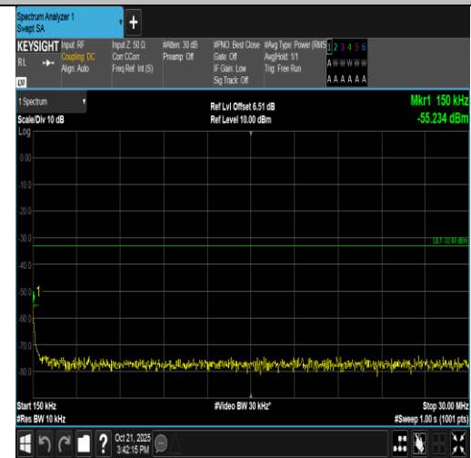
Band2-20MHz-16QAM-19100-1RB#99-0.15~30-PASS
