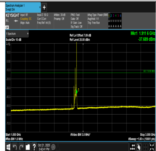
Band2-20MHz-16QAM-19100-1RB#99-1000~3000-PASS
