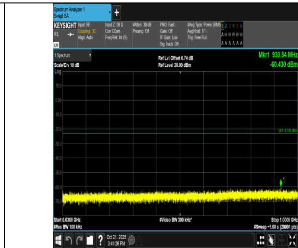
Band2-20MHz-QPSK-19100-1RB#99-30~1000-PASS
