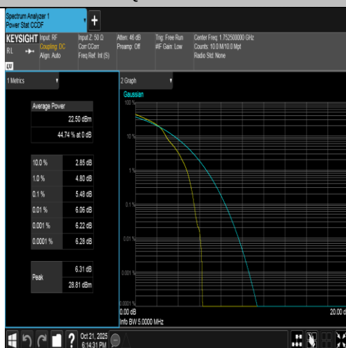
Band4-5MHz-16QAM-20375-1RB#0-PASS
