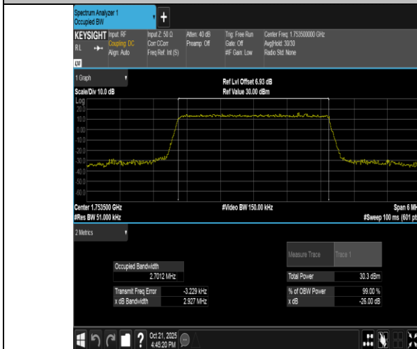
Band4-3MHz-QPSK-20385-15RB#0-PASS
