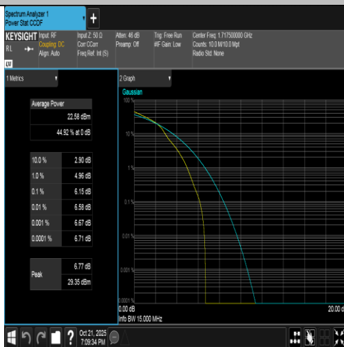
Band4-15MHz-16QAM-20025-1RB#0-PASS
