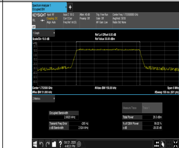
Band4-3MHz-16QAM-20385-15RB#0-PASS
