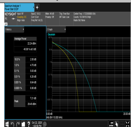
Band4-15MHz-QPSK-20175-75RB#0-PASS
