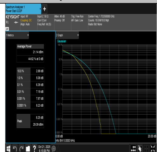
Band4-5MHz-16QAM-20375-25RB#0-PASS
