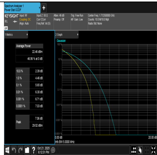
Band4-5MHz-QPSK-19975-25RB#0-PASS
