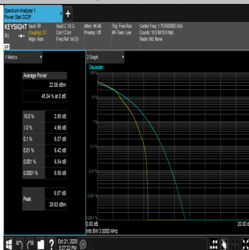
Band4-3MHz-16QAM-20385-1RB#0-PASS
