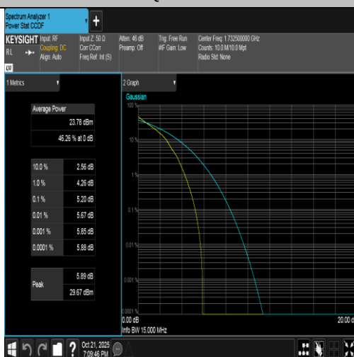
Band4-15MHz-QPSK-20175-1RB#0-PASS
