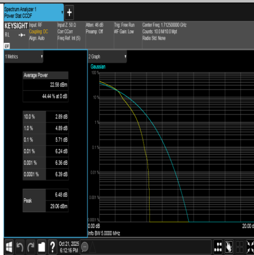
Band4-5MHz-16QAM-19975-1RB#0-PASS
