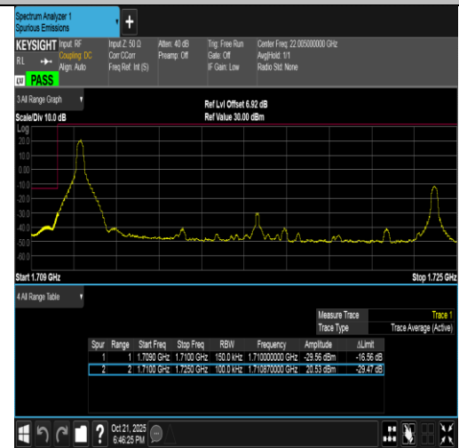
Band4-15MHz-16QAM-20025-1RB#0-PASS
