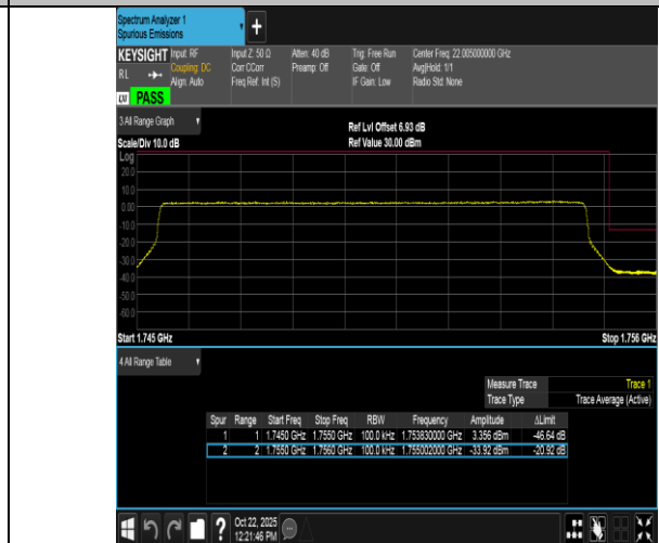
Band4-10MHz-16QAM-20350-50RB#0-PASS
