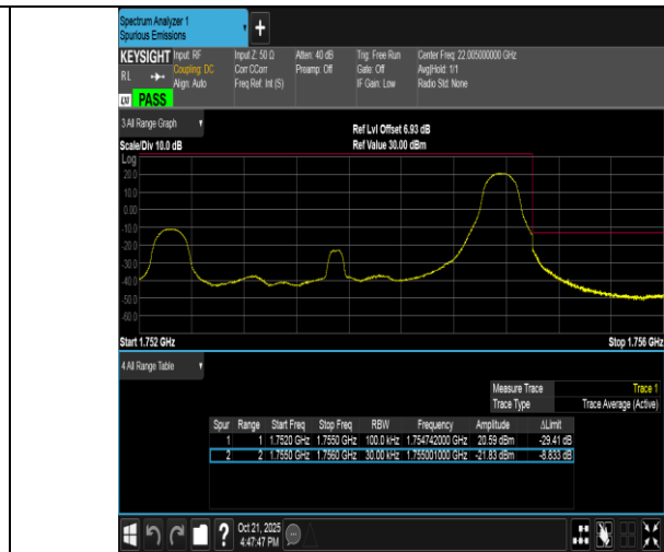
Band4-3MHz-QPSK-20385-1RB#14-PASS
