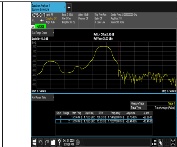
Band4-1.4MHz-QPSK-20393-1RB#5-PASS
