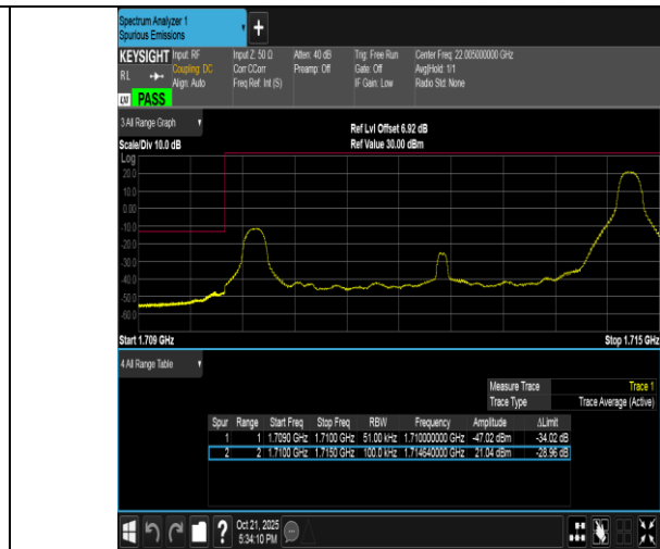
Band4-5MHz-QPSK-19975-1RB#24-PASS
