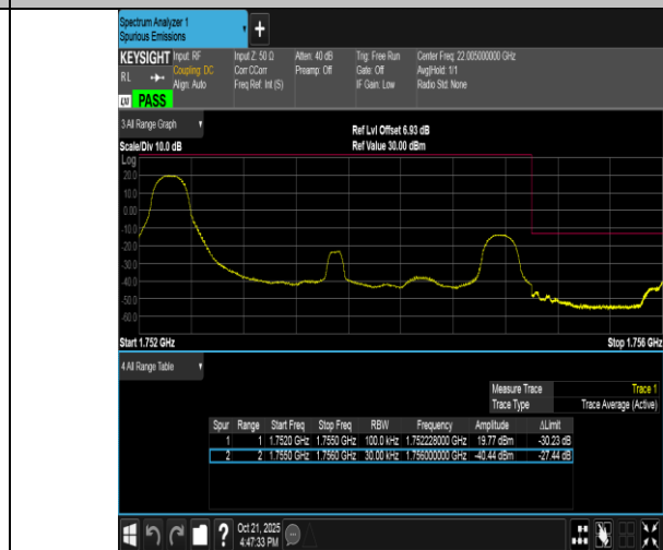
Band4-3MHz-16QAM-20385-1RB#0-PASS
