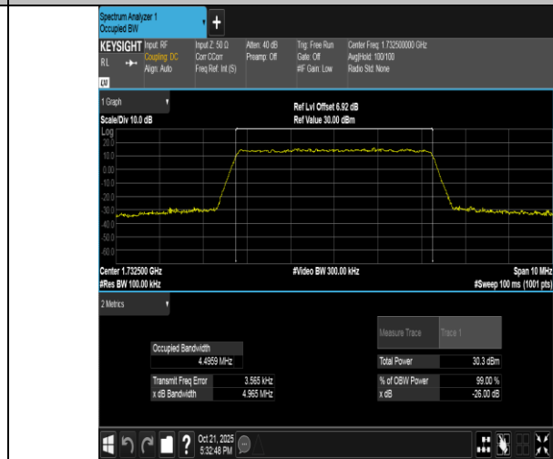
Band4-5MHz-16QAM-20175-25RB#0-PASS
