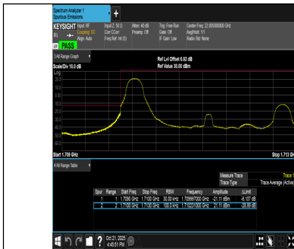
Band4-3MHz-QPSK-19965-1RB#0-PASS
