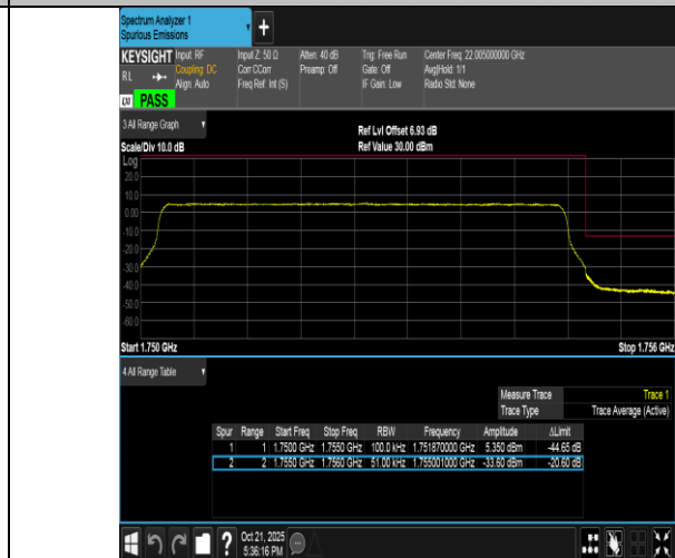
Band4-5MHz-16QAM-20375-25RB#0-PASS
