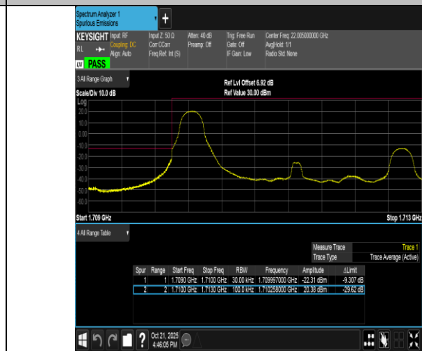
Band4-3MHz-16QAM-19965-1RB#0-PASS
