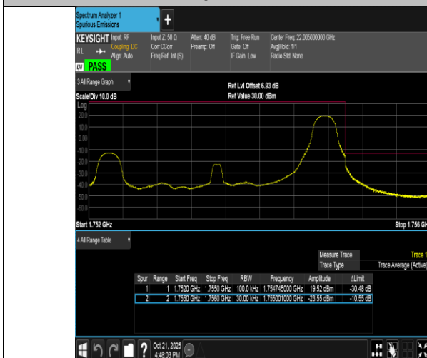
Band4-3MHz-16QAM-20385-1RB#14-PASS
