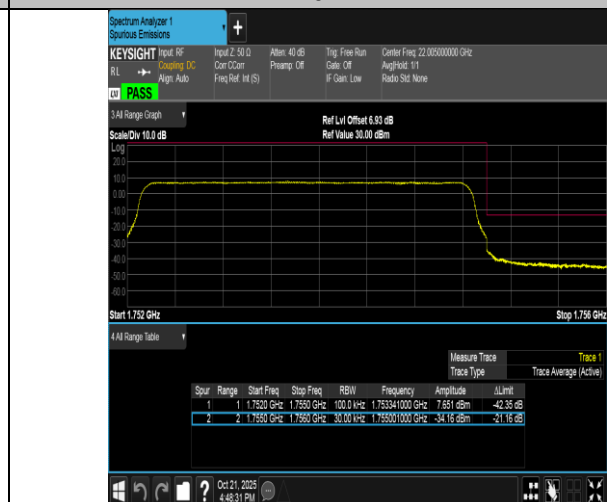
Band4-3MHz-16QAM-20385-15RB#0-PASS
