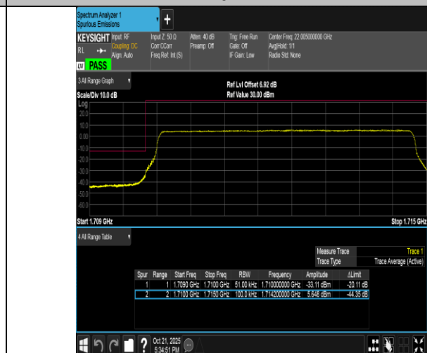
Band4-5MHz-16QAM-19975-25RB#0-PASS
