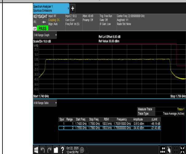
Band4-15MHz-16QAM-20325-75RB#0-PASS
