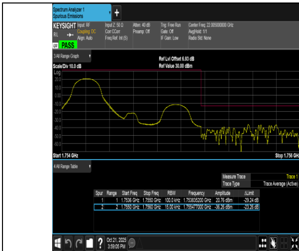
Band4-1.4MHz-QPSK-20393-1RB#0-PASS
