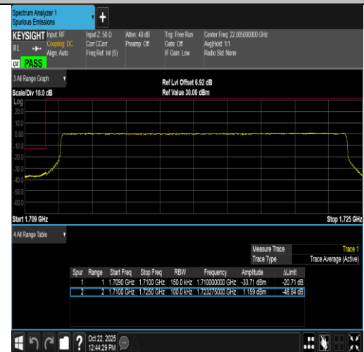
Band4-15MHz-16QAM-20025-75RB#0-PASS
