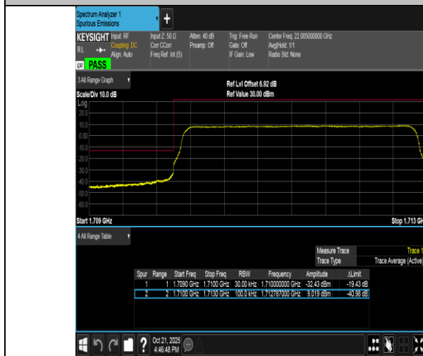
Band4-3MHz-QPSK-19965-15RB#0-PASS
