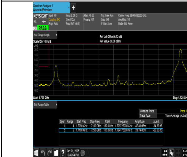
Band4-15MHz-16QAM-20025-1RB#74-PASS
