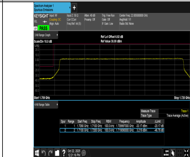
Band4-10MHz-16QAM-20000-50RB#0-PASS
