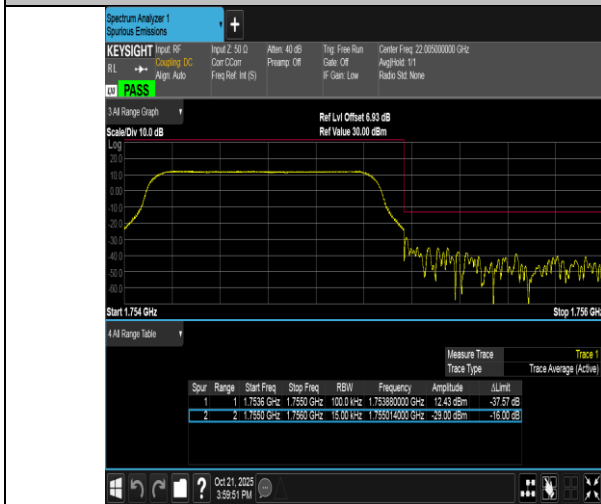
Band4-1.4MHz-QPSK-20393-6RB#0-PASS
