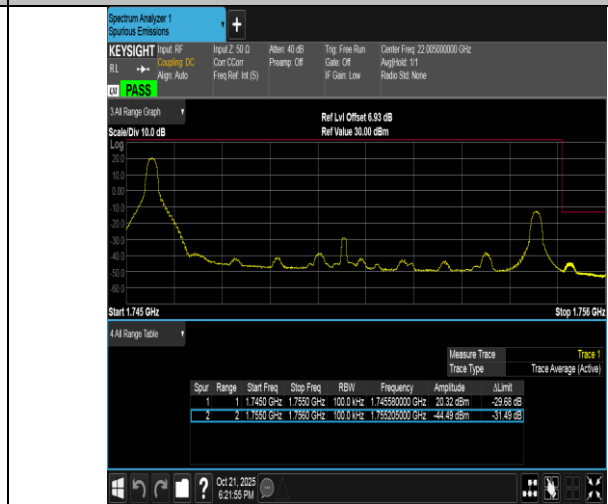
Band4-10MHz-16QAM-20350-1RB#0-PASS
