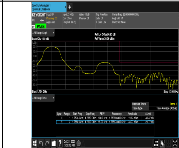
Band4-1.4MHz-16QAM-20393-1RB#0-PASS
