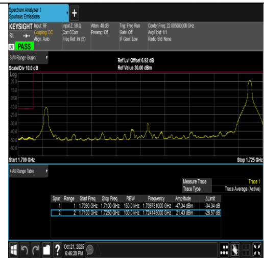
Band4-15MHz-QPSK-20025-1RB#74-PASS
