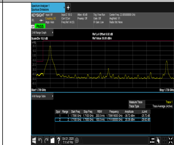
Band4-20MHz-16QAM-20050-1RB#0-PASS
