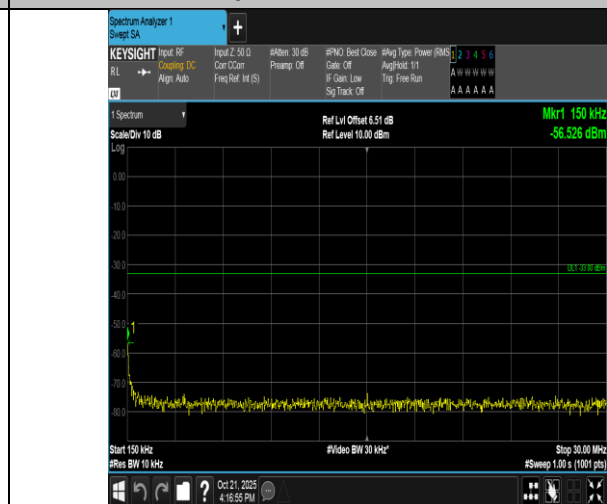
Band4-1.4MHz-QPSK-20393-6RB#0-0.15~30-PASS
