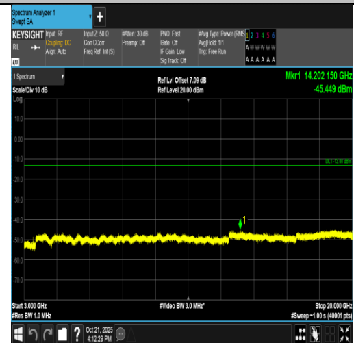
Band4-1.4MHz-16QAM-20175-6RB#0-3000~20000-PASS
