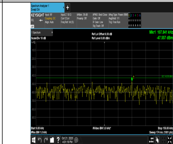
Band4-1.4MHz-16QAM-19957-1RB#0-0.009~0.15-PASS
