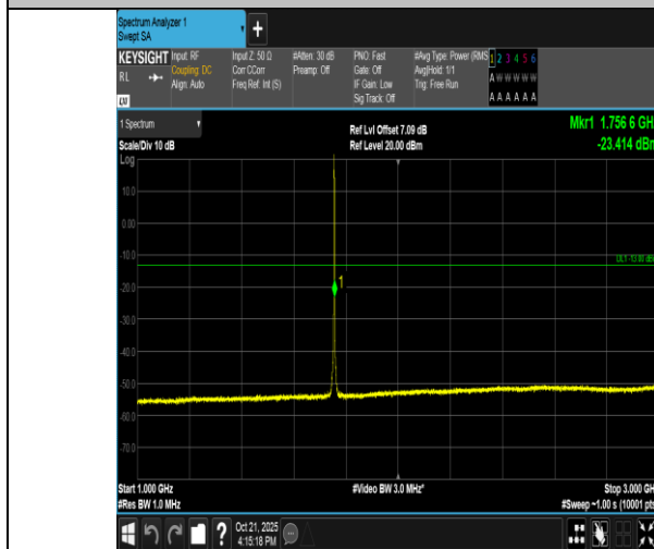
Band4-1.4MHz-QPSK-20393-1RB#5-1000~3000-PASS
