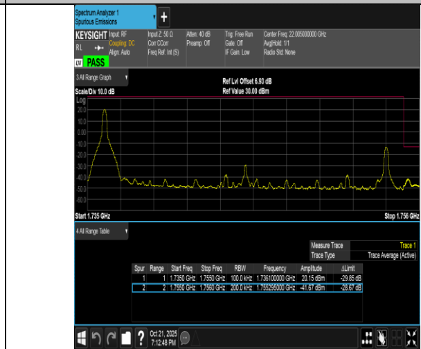
Band4-20MHz-16QAM-20300-1RB#0-PASS
