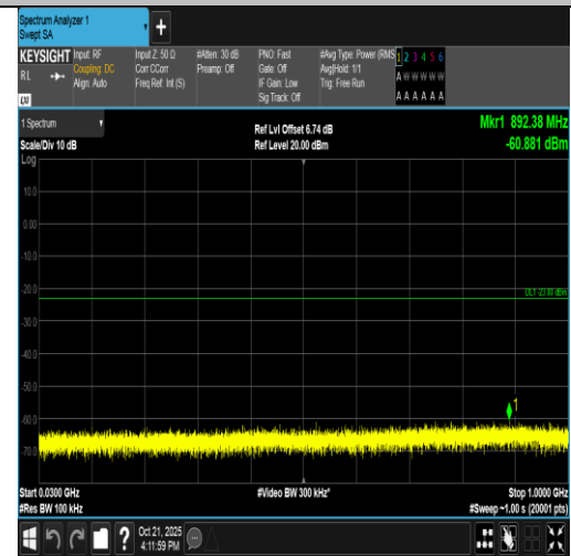
Band4-1.4MHz-16QAM-20175-6RB#0-30~1000-PASS
