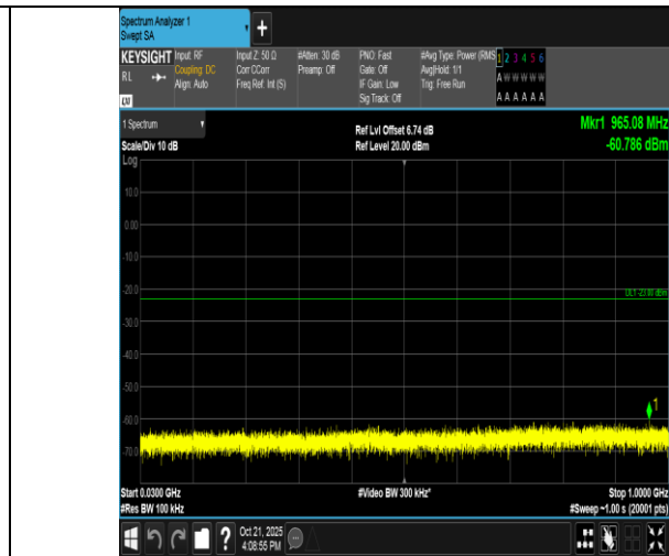
Band4-1.4MHz-QPSK-20175-1RB#5-30~1000-PASS
