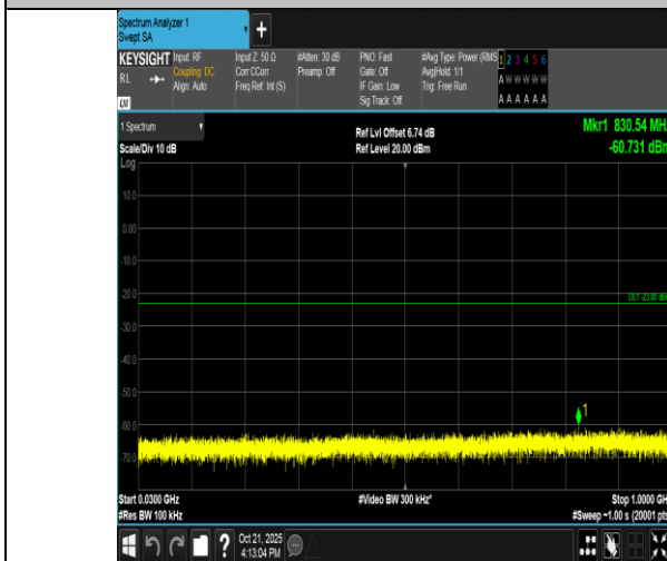
Band4-1.4MHz-QPSK-20393-1RB#0-30~1000-PASS
