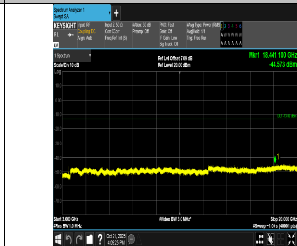
Band4-1.4MHz-QPSK-20175-1RB#5-3000~20000-PASS
