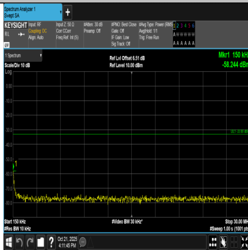
Band4-1.4MHz-16QAM-20175-6RB#0-0.15~30-PASS
