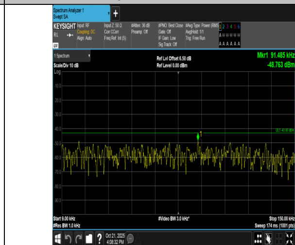
Band4-1.4MHz-QPSK-20175-1RB#5-0.009~0.15-PASS
