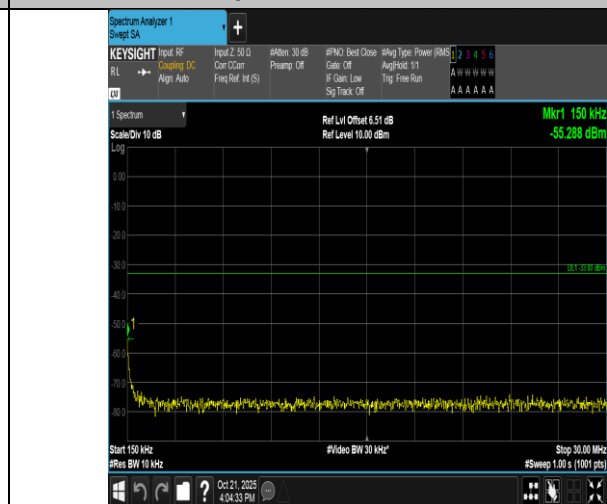
Band4-1.4MHz-QPSK-19957-6RB#0-0.15~30-PASS
