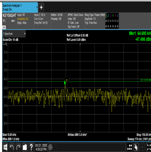
Band4-1.4MHz-16QAM-19957-1RB#5-0.009~0.15-PASS
