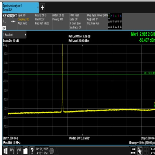
Band4-1.4MHz-16QAM-20175-6RB#0-1000~3000-PASS
