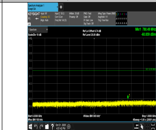
Band4-1.4MHz-16QAM-19957-1RB#0-30~1000-PASS
