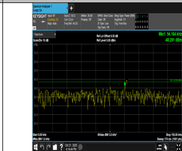
Band4-1.4MHz-QPSK-20393-1RB#5-0.009~0.15-PASS
