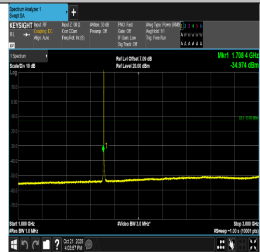
Band4-1.4MHz-16QAM-19957-1RB#5-1000~3000-PASS
