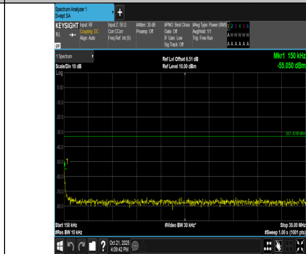
Band4-1.4MHz-16QAM-20175-1RB#5-0.15~30-PASS
