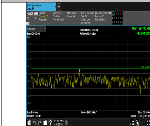
Band4-1.4MHz-QPSK-19957-6RB#0-0.009~0.15-PASS
