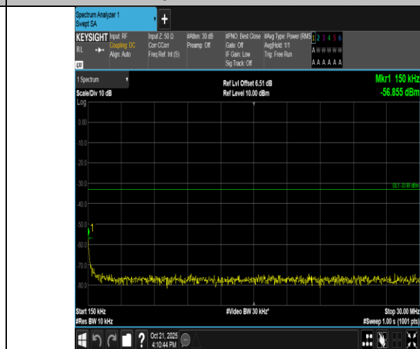
Band4-1.4MHz-QPSK-20175-6RB#0-0.15~30-PASS
