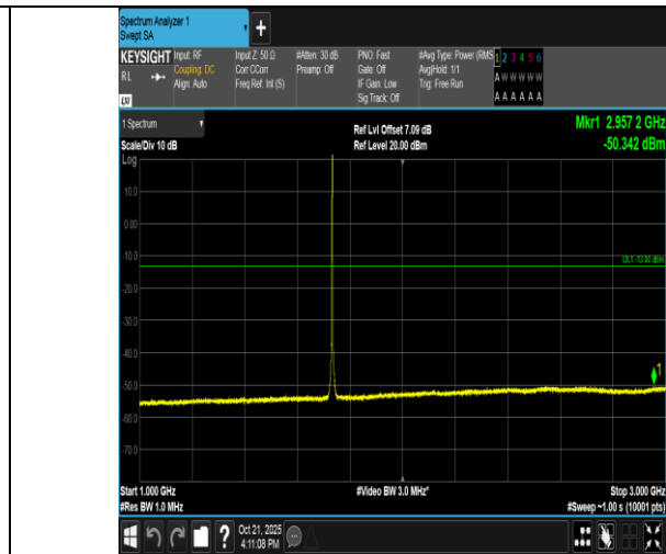
Band4-1.4MHz-QPSK-20175-6RB#0-1000~3000-PASS
