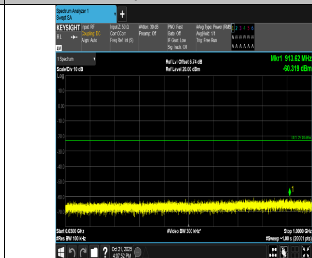
Band4-1.4MHz-16QAM-20175-1RB#0-30~1000-PASS
