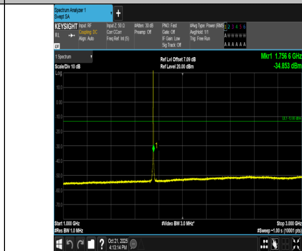
Band4-1.4MHz-QPSK-20393-1RB#0-1000~3000-PASS
