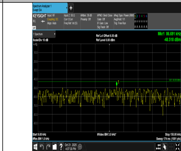
Band4-1.4MHz-16QAM-20175-1RB#0-0.009~0.15-PASS
