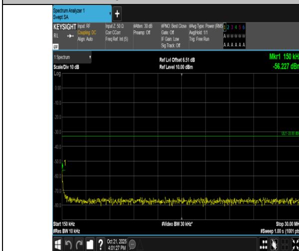
Band4-1.4MHz-16QAM-19957-1RB#0-0.15~30-PASS
