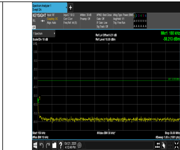
Band4-1.4MHz-QPSK-20393-1RB#0-0.15~30-PASS
