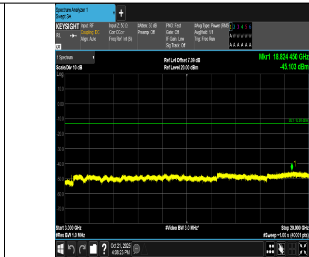
Band4-1.4MHz-16QAM-20175-1RB#0-3000~20000-PASS
