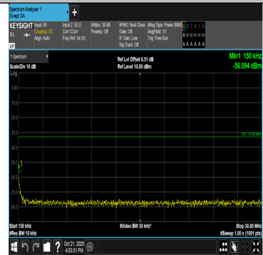
Band4-1.4MHz-16QAM-19957-1RB#5-0.15~30-PASS
