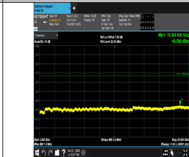
Band4-1.4MHz-QPSK-20393-1RB#5-3000~20000-PASS
