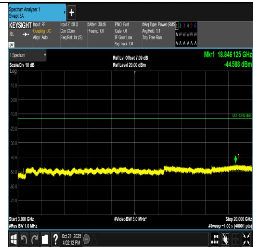
Band4-1.4MHz-16QAM-19957-1RB#0-3000~20000-PASS
