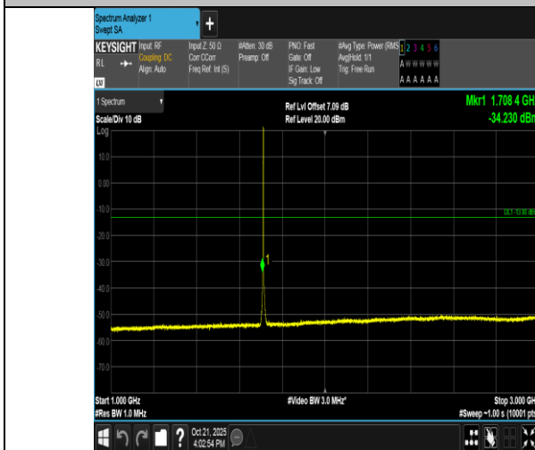
Band4-1.4MHz-QPSK-19957-1RB#5-1000~3000-PASS
