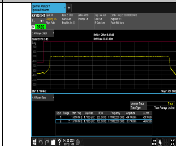
Band4-20MHz-16QAM-20050-100RB#0-PASS
