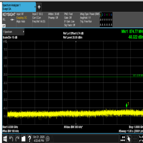
Band4-1.4MHz-16QAM-19957-1RB#5-30~1000-PASS
