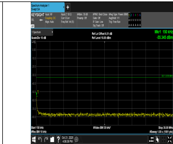
Band4-1.4MHz-QPSK-20175-1RB#0-0.15~30-PASS
