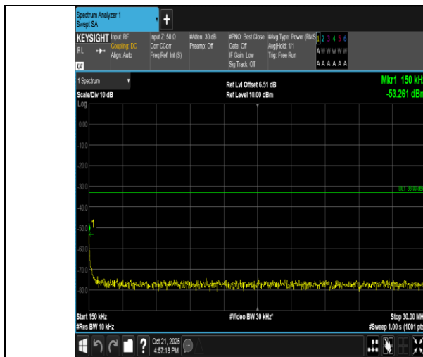
Band4-3MHz-QPSK-20175-1RB#14-0.15~30-PASS
