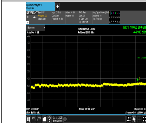
Band4-3MHz-QPSK-20175-15RB#0-3000~20000-PASS
