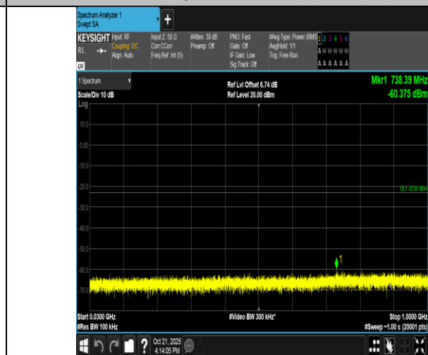
Band4-1.4MHz-16QAM-20393-1RB#0-30~1000-PASS
