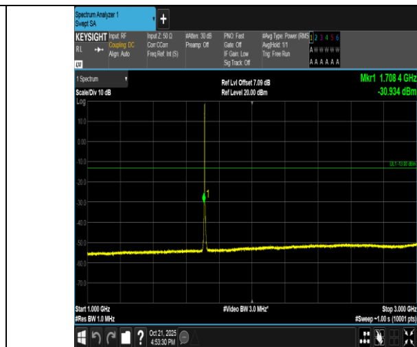
Band4-3MHz-QPSK-19965-15RB#0-1000~3000-PASS
