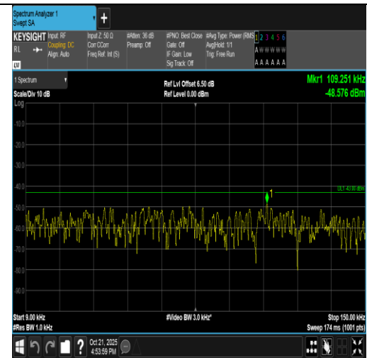
Band4-3MHz-16QAM-19965-15RB#0-0.009~0.15-PASS
