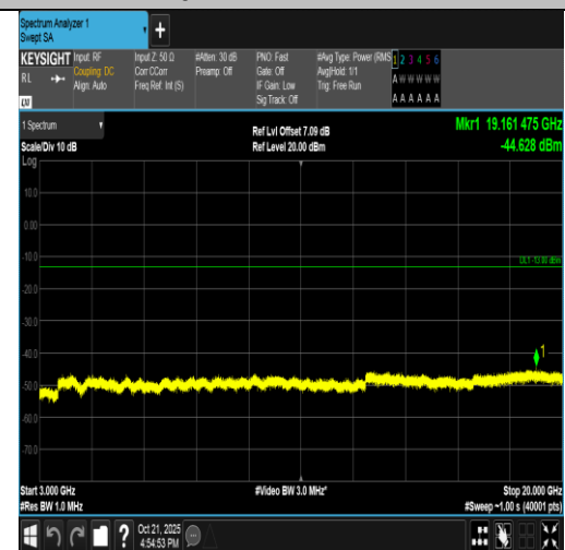
Band4-3MHz-16QAM-19965-15RB#0-3000~20000-PASS
