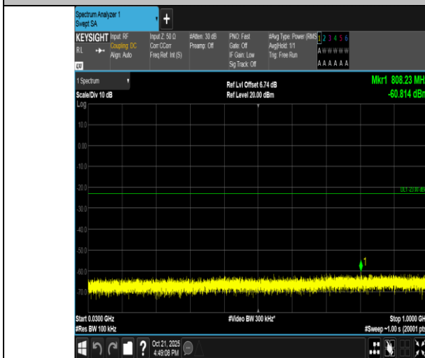
Band4-3MHz-QPSK-19965-1RB#0-30~1000-PASS
