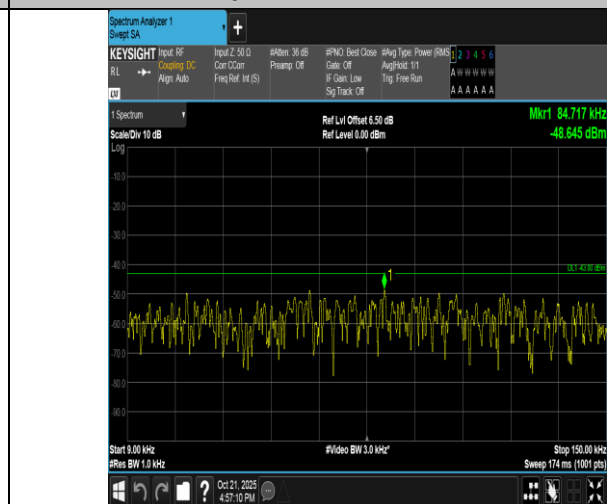
Band4-3MHz-QPSK-20175-1RB#14-0.009~0.15-PASS
