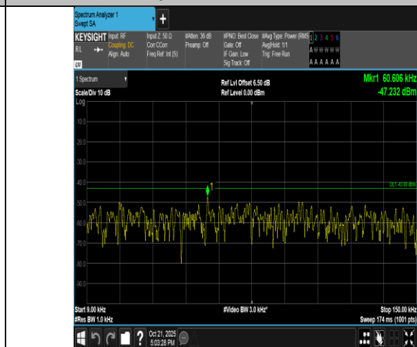
Band4-3MHz-QPSK-20385-1RB#14-0.009~0.15-PASS
