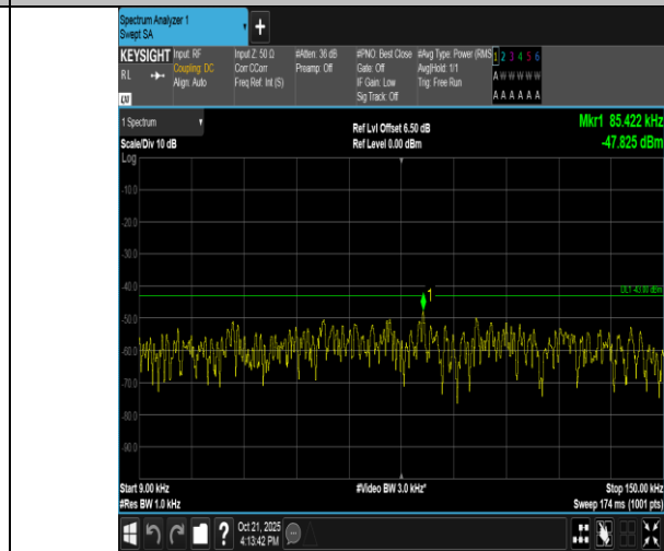
Band4-1.4MHz-16QAM-20393-1RB#0-0.009~0.15-PASS
