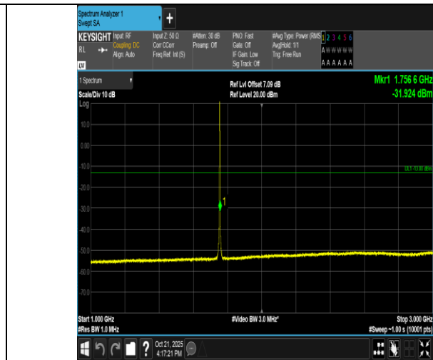
Band4-1.4MHz-QPSK-20393-6RB#0-1000~3000-PASS
