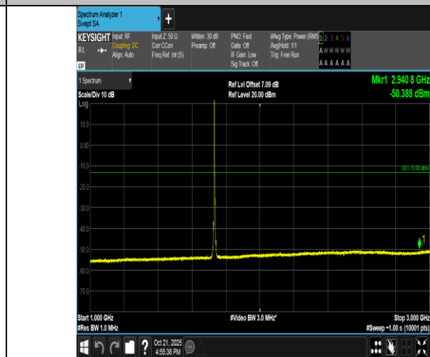
Band4-3MHz-QPSK-20175-1RB#0-1000~3000-PASS
