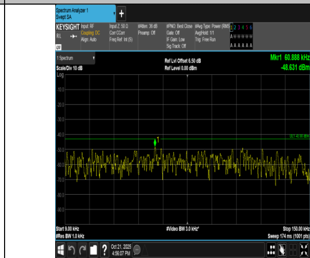
Band4-3MHz-16QAM-20175-1RB#0-0.009~0.15-PASS
