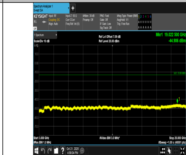
Band4-3MHz-QPSK-20175-1RB#14-3000~20000-PASS
