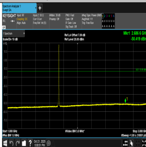
Band4-3MHz-16QAM-20175-15RB#0-1000~3000-PASS
