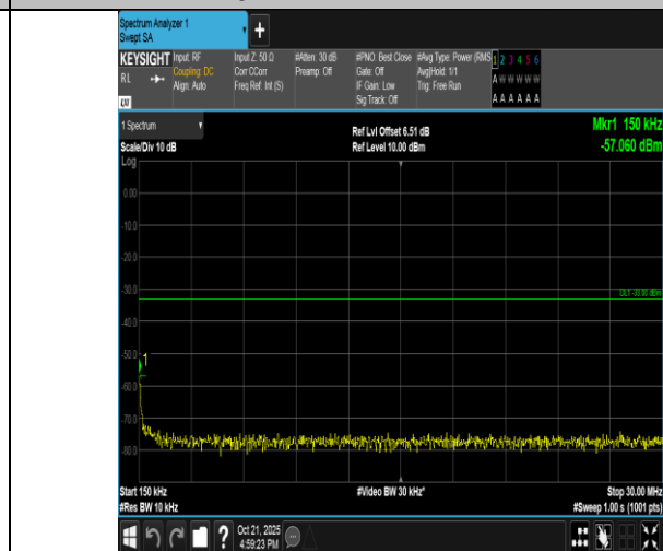
Band4-3MHz-QPSK-20175-15RB#0-0.15~30-PASS
