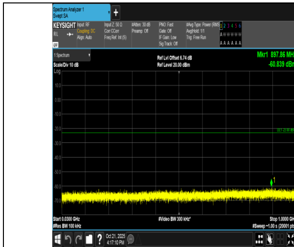
Band4-1.4MHz-QPSK-20393-6RB#0-30~1000-PASS
