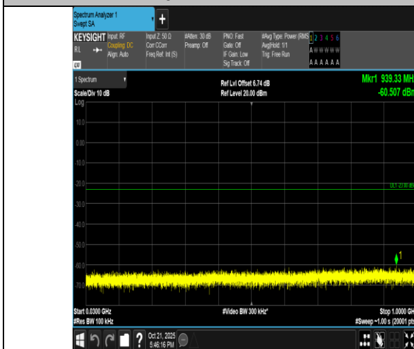
Band4-5MHz-16QAM-20175-1RB#24-30~1000-PASS
