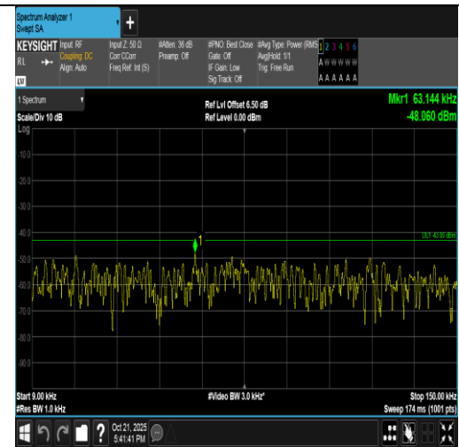
Band4-5MHz-16QAM-19975-25RB#0-0.009~0.15-PASS
