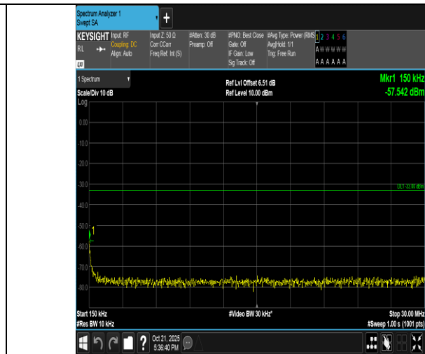
Band4-5MHz-QPSK-19975-1RB#0-0.15~30-PASS
