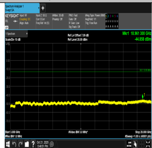
Band4-5MHz-16QAM-20175-25RB#0-3000~20000-PASS
