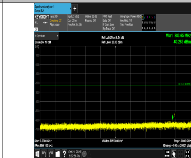
Band4-5MHz-16QAM-19975-1RB#0-30~1000-PASS
