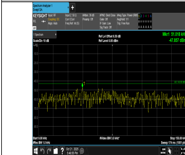
Band4-5MHz-QPSK-20175-25RB#0-0.009~0.15-PASS
