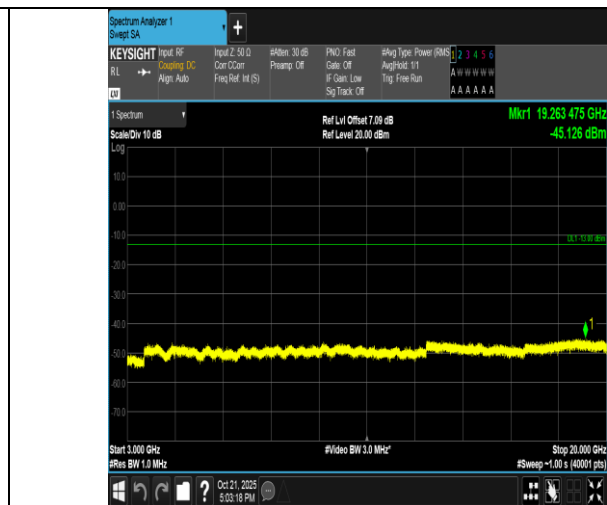
Band4-3MHz-16QAM-20385-1RB#0-3000~20000-PASS
