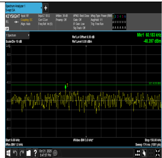
Band4-5MHz-16QAM-20175-25RB#0-0.009~0.15-PASS
