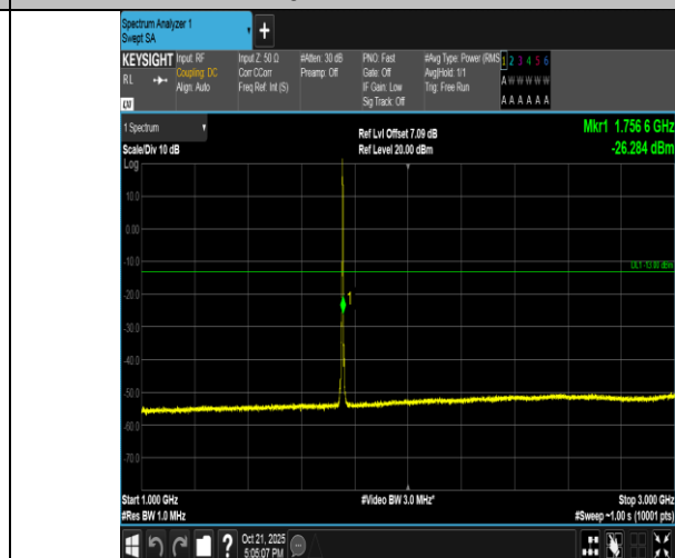
Band4-3MHz-16QAM-20385-1RB#14-1000~3000-PASS
