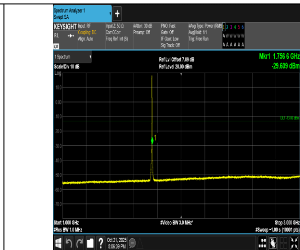
Band4-3MHz-QPSK-20385-15RB#0-1000~3000-PASS
