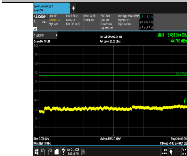
Band4-3MHz-QPSK-20385-15RB#0-3000~20000-PASS
