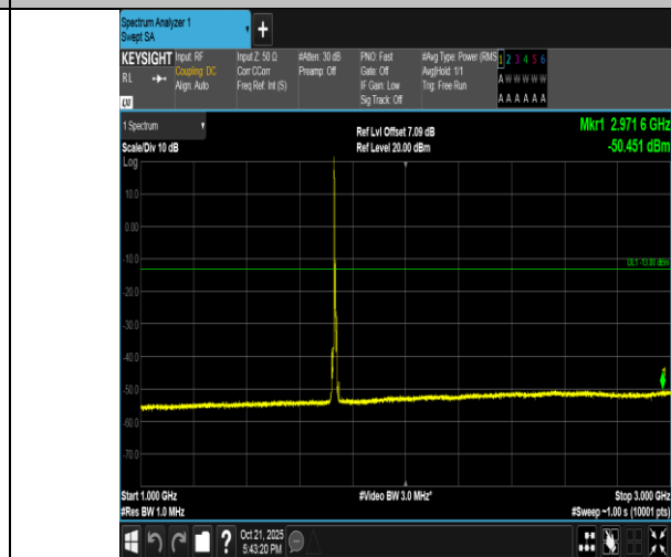
Band4-5MHz-QPSK-20175-1RB#0-1000~3000-PASS
