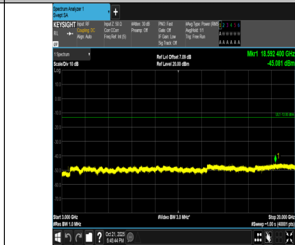
Band4-5MHz-QPSK-20175-1RB#24-3000~20000-PASS
