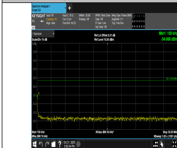
Band4-3MHz-16QAM-20385-1RB#0-0.15~30-PASS
