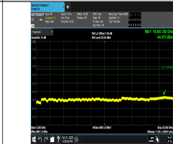
Band4-5MHz-QPSK-19975-1RB#24-3000~20000-PASS
