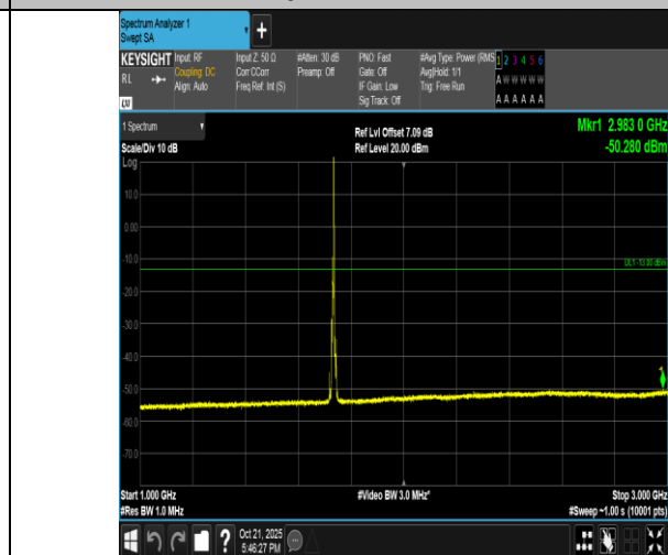
Band4-5MHz-16QAM-20175-1RB#24-1000~3000-PASS
