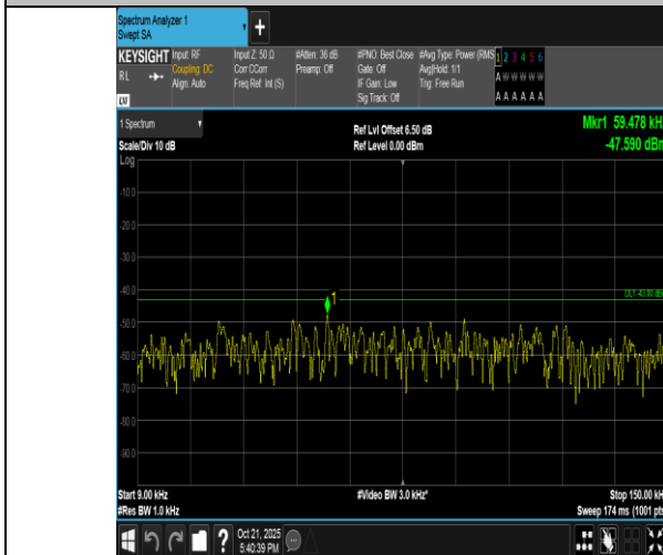
Band4-5MHz-QPSK-19975-25RB#0-0.009~0.15-PASS
