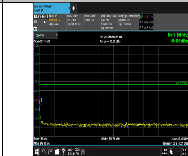
Band4-3MHz-16QAM-20385-1RB#14-0.15~30-PASS
