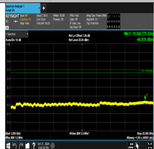
Band4-5MHz-16QAM-19975-25RB#0-3000~20000-PASS
