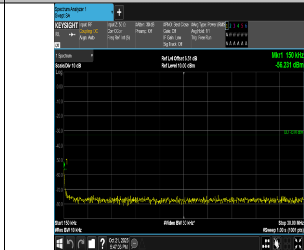
Band4-5MHz-QPSK-20175-25RB#0-0.15~30-PASS
