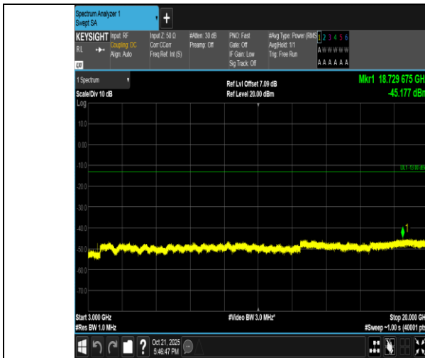
Band4-5MHz-16QAM-20175-1RB#24-3000~20000-PASS
