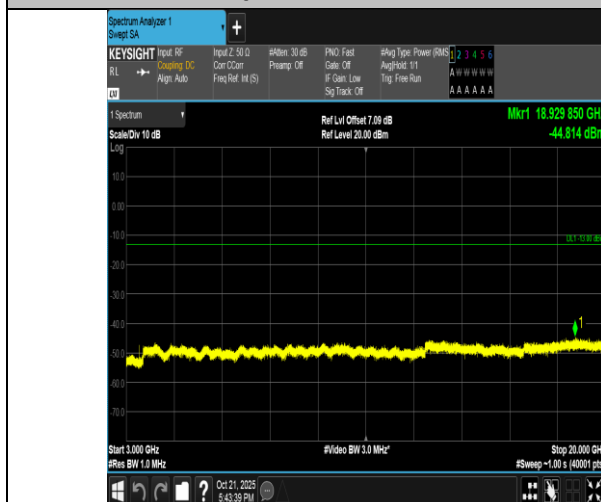
Band4-5MHz-QPSK-20175-1RB#0-3000~20000-PASS
