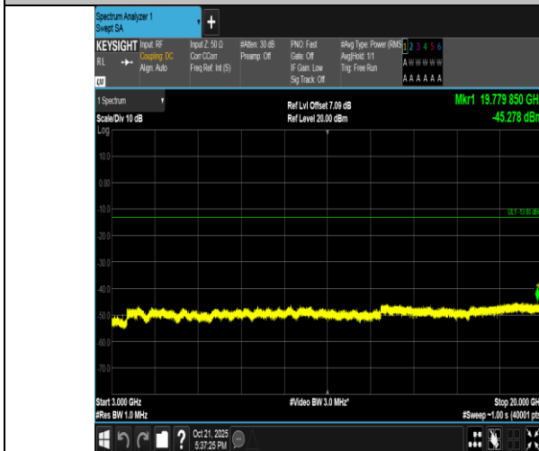
Band4-5MHz-QPSK-19975-1RB#0-3000~20000-PASS
