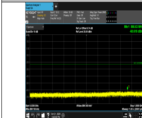
Band4-5MHz-16QAM-19975-1RB#24-30~1000-PASS
