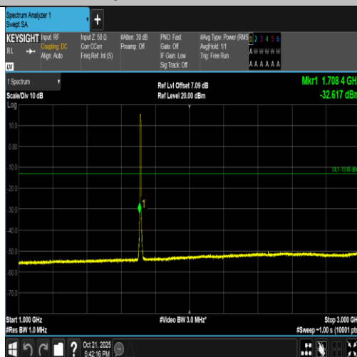
Band4-5MHz-16QAM-19975-25RB#0-1000~3000-PASS
