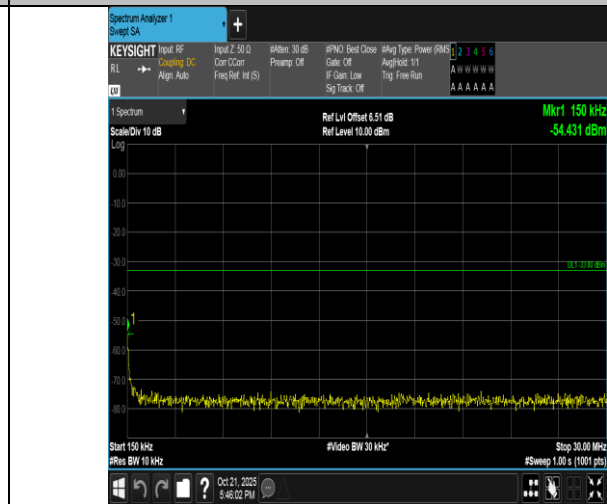
Band4-5MHz-16QAM-20175-1RB#24-0.15~30-PASS
