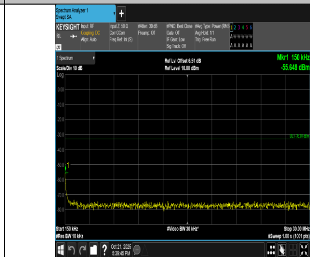
Band4-5MHz-16QAM-19975-1RB#24-0.15~30-PASS
