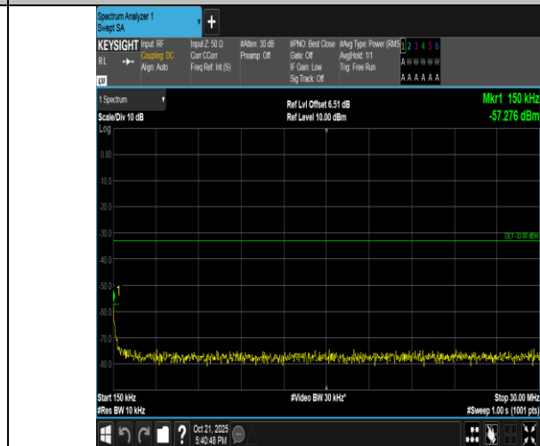
Band4-5MHz-QPSK-19975-25RB#0-0.15~30-PASS
