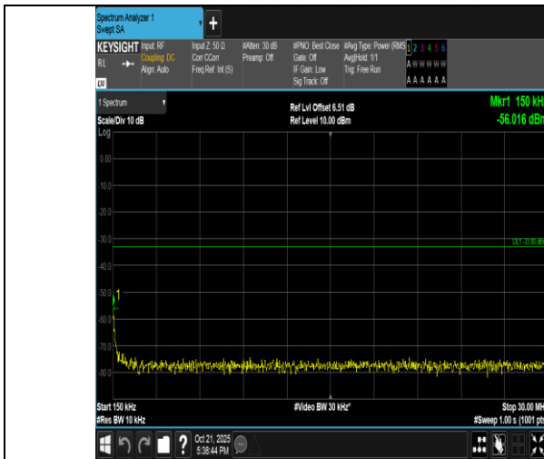
Band4-5MHz-QPSK-19975-1RB#24-0.15~30-PASS
