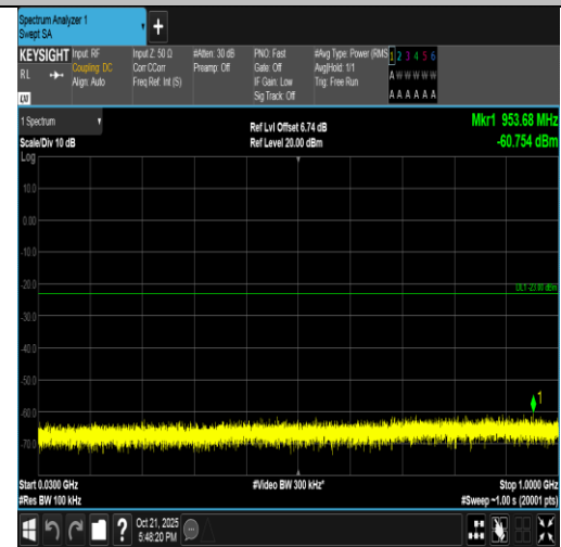
Band4-5MHz-16QAM-20175-25RB#0-30~1000-PASS
