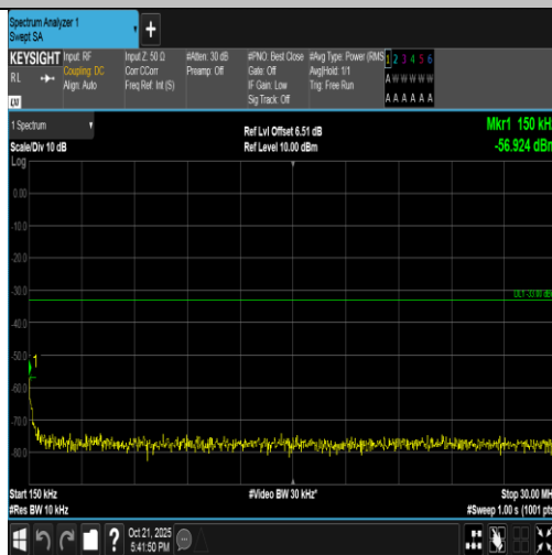
Band4-5MHz-16QAM-19975-25RB#0-0.15~30-PASS
