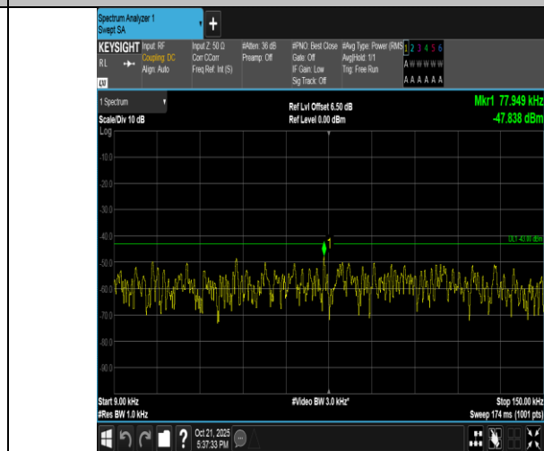
Band4-5MHz-16QAM-19975-1RB#0-0.009~0.15-PASS
