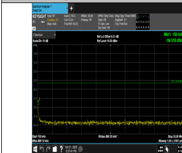
Band4-5MHz-16QAM-19975-1RB#0-0.15~30-PASS
