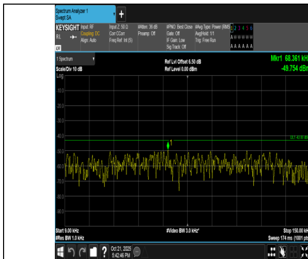
Band4-5MHz-QPSK-20175-1RB#0-0.009~0.15-PASS
