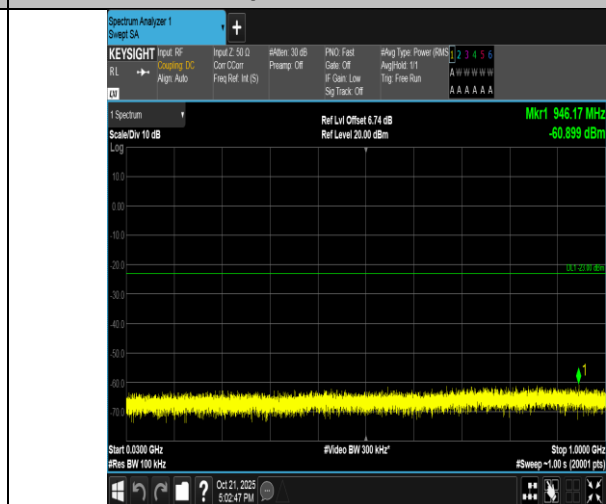
Band4-3MHz-16QAM-20385-1RB#0-30~1000-PASS
