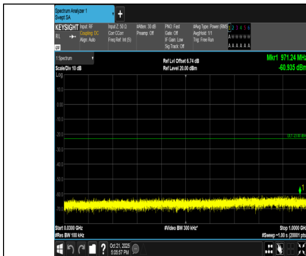
Band4-3MHz-QPSK-20385-15RB#0-30~1000-PASS
