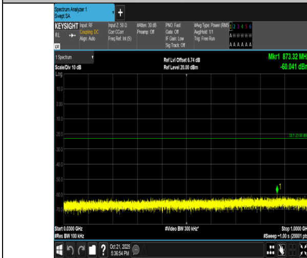
Band4-5MHz-QPSK-19975-1RB#0-30~1000-PASS
