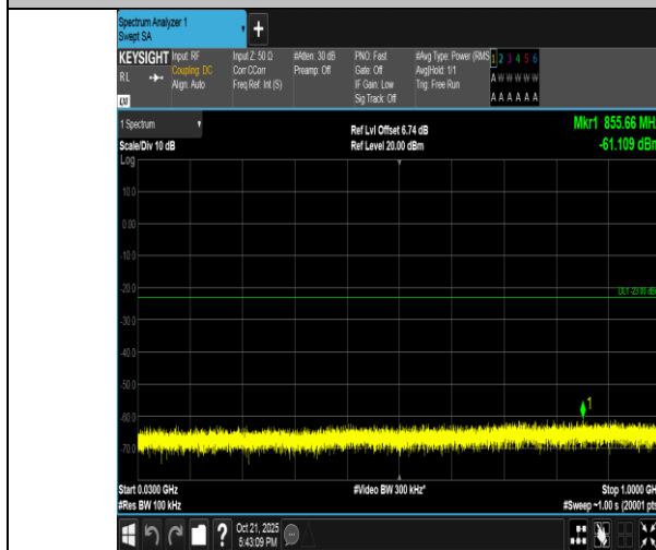
Band4-5MHz-QPSK-20175-1RB#0-30~1000-PASS
