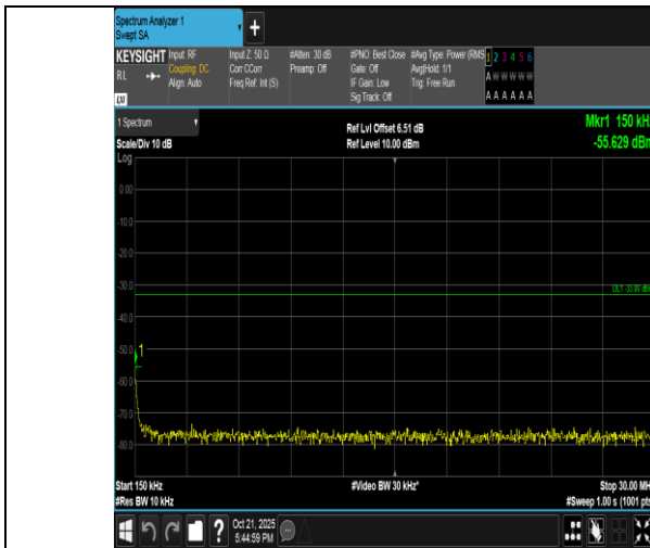
Band4-5MHz-QPSK-20175-1RB#24-0.15~30-PASS
