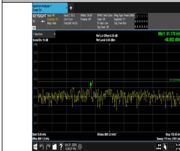
Band4-5MHz-16QAM-19975-1RB#24-0.009~0.15-PASS
