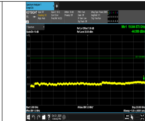
Band4-5MHz-16QAM-20175-1RB#0-3000~20000-PASS
