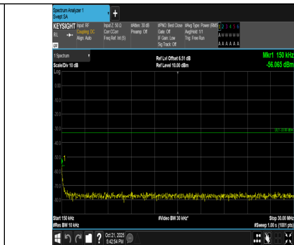
Band4-5MHz-QPSK-20175-1RB#0-0.15~30-PASS
