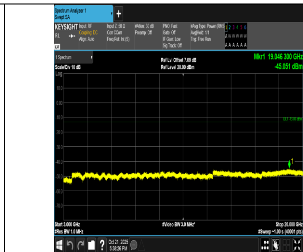
Band4-5MHz-16QAM-19975-1RB#0-3000~20000-PASS
