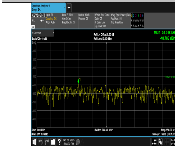
Band4-3MHz-16QAM-20385-1RB#14-0.009~0.15-PASS
