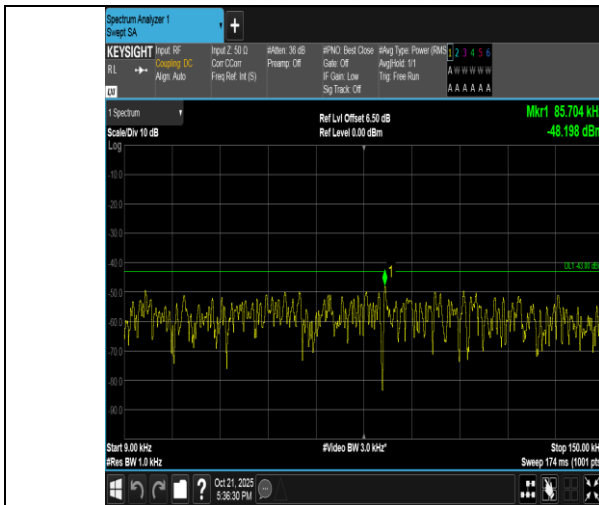
Band4-5MHz-QPSK-19975-1RB#0-0.009~0.15-PASS
