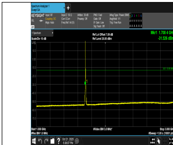
Band4-5MHz-16QAM-19975-1RB#0-1000~3000-PASS
