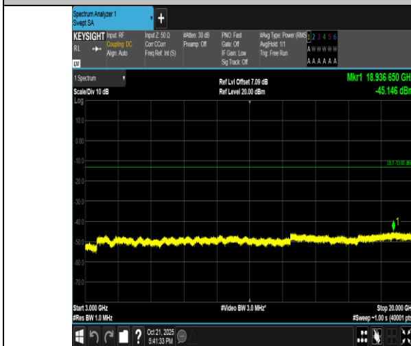
Band4-5MHz-QPSK-19975-25RB#0-3000~20000-PASS
