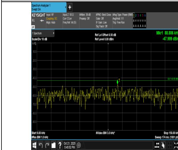
Band4-5MHz-16QAM-20175-1RB#24-0.009~0.15-PASS
