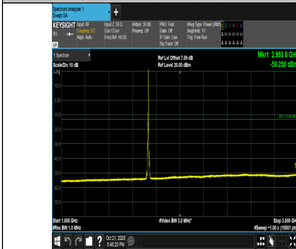
Band4-5MHz-QPSK-20175-1RB#24-1000~3000-PASS
