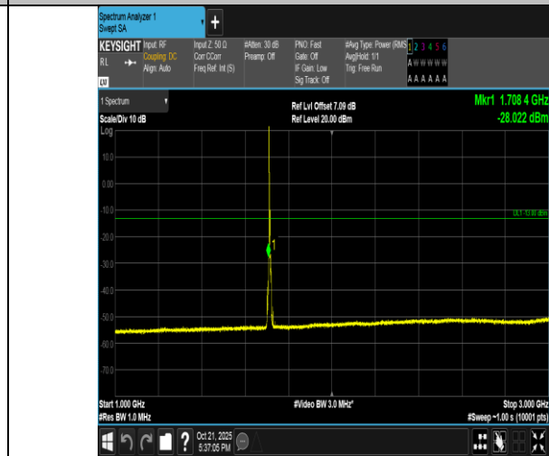
Band4-5MHz-QPSK-19975-1RB#0-1000~3000-PASS
