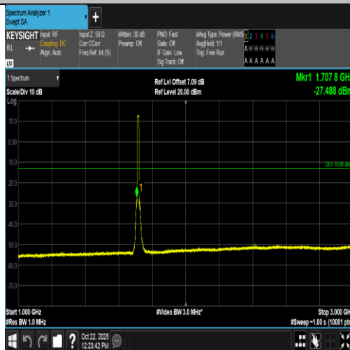
Band4-10MHz-16QAM-20000-50RB#0-1000~3000-PASS
