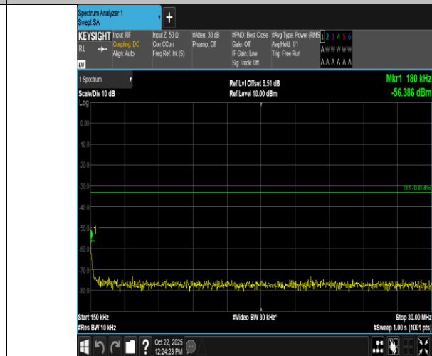
Band4-10MHz-QPSK-20175-50RB#0-0.15~30-PASS
