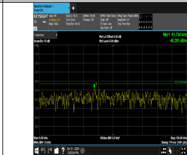
Band4-5MHz-16QAM-20375-1RB#0-0.009~0.15-PASS
