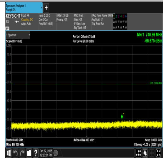
Band4-10MHz-16QAM-20000-50RB#0-30~1000-PASS
