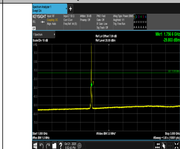
Band4-5MHz-16QAM-20375-1RB#24-1000~3000-PASS
