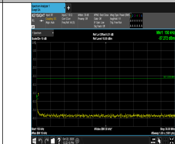
Band4-10MHz-QPSK-20000-50RB#0-0.15~30-PASS
