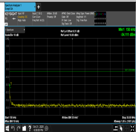
Band4-10MHz-16QAM-20175-1RB#49-0.15~30-PASS
