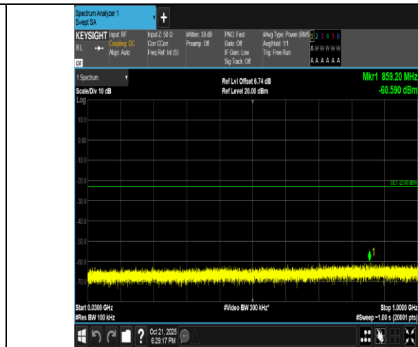
Band4-10MHz-QPSK-20175-1RB#49-30~1000-PASS
