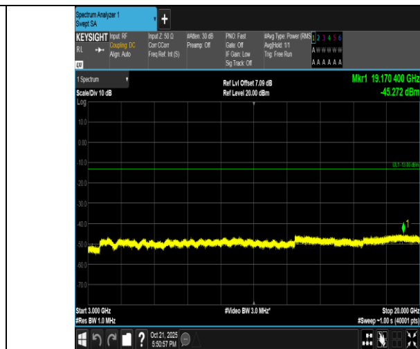
Band4-5MHz-16QAM-20375-1RB#0-3000~20000-PASS
