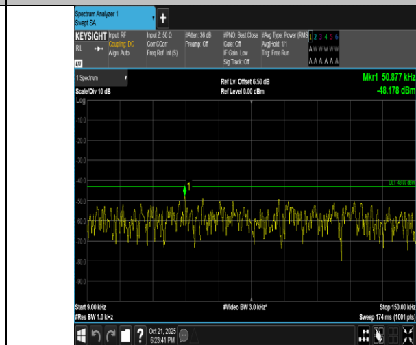
Band4-10MHz-16QAM-20000-1RB#0-0.009~0.15-PASS
