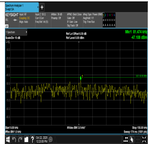
Band4-10MHz-16QAM-20000-50RB#0-0.009~0.15-PASS
