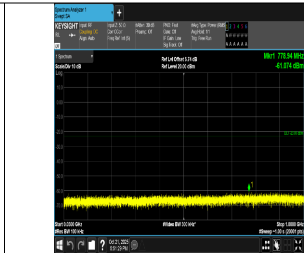
Band4-5MHz-QPSK-20375-1RB#24-30~1000-PASS
