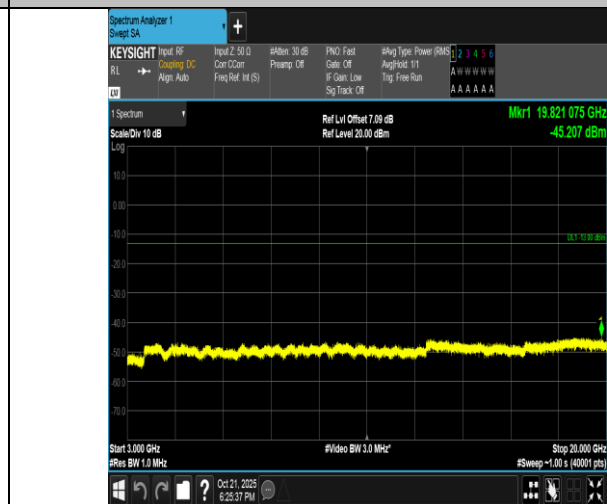
Band4-10MHz-QPSK-20000-1RB#49-3000~20000-PASS
