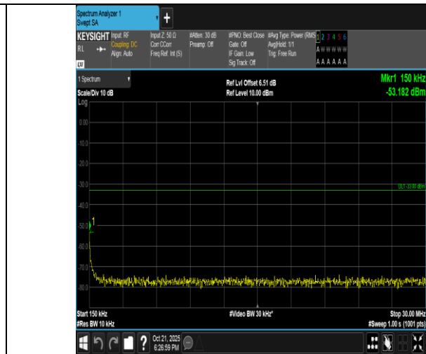
Band4-10MHz-QPSK-20175-1RB#0-0.15~30-PASS
