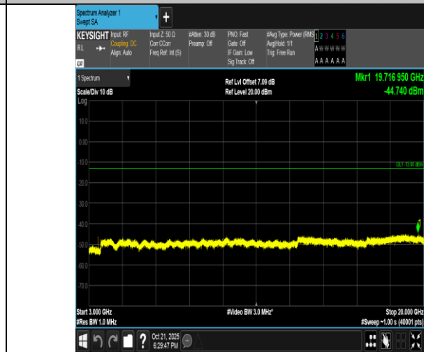
Band4-10MHz-QPSK-20175-1RB#49-3000~20000-PASS
