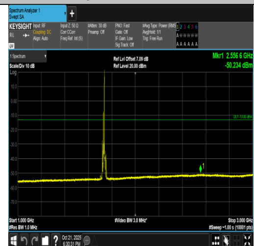
Band4-10MHz-16QAM-20175-1RB#49-1000~3000-PASS
