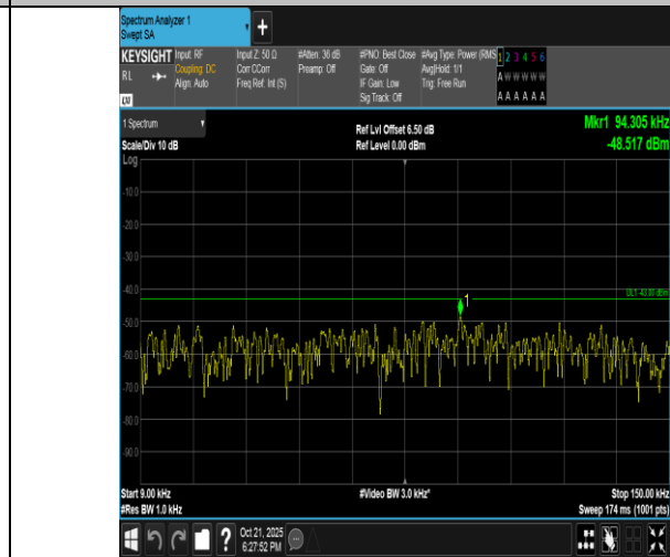
Band4-10MHz-16QAM-20175-1RB#0-0.009~0.15-PASS
