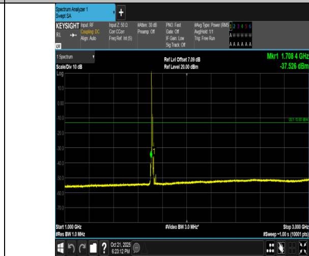
Band4-10MHz-QPSK-20000-1RB#0-1000~3000-PASS
