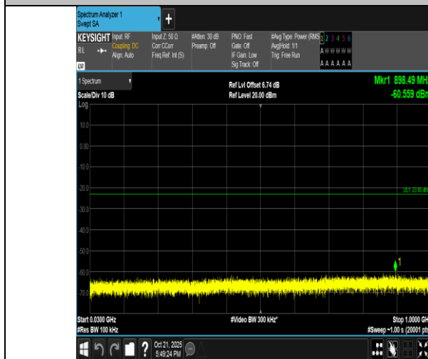
Band4-5MHz-QPSK-20375-1RB#0-30~1000-PASS
