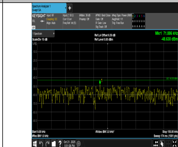
Band4-5MHz-QPSK-20375-1RB#24-0.009~0.15-PASS
