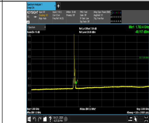
Band4-10MHz-QPSK-20175-1RB#0-1000~3000-PASS
