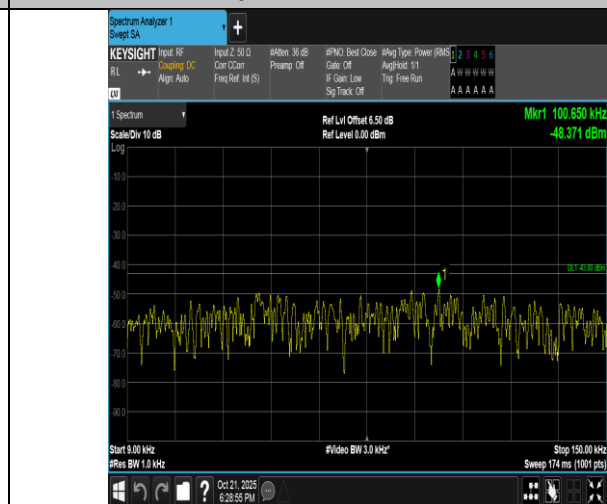
Band4-10MHz-QPSK-20175-1RB#49-0.009~0.15-PASS
