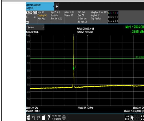
Band4-5MHz-QPSK-20375-1RB#24-1000~3000-PASS
