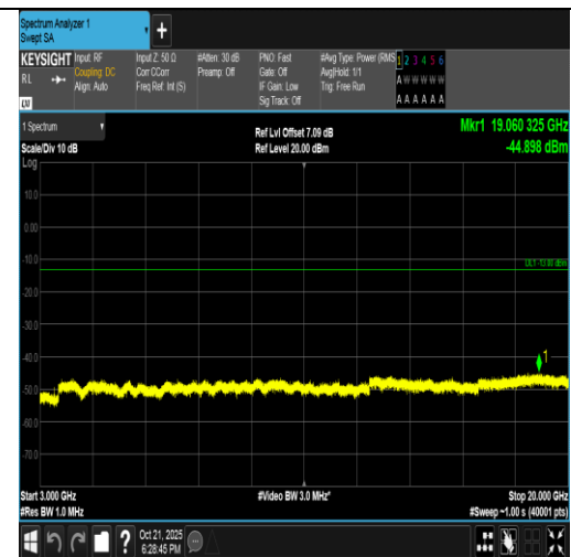
Band4-10MHz-16QAM-20175-1RB#0-3000~20000-PASS
