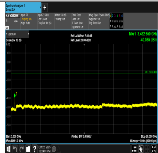
Band4-10MHz-16QAM-20000-50RB#0-3000~20000-PASS
