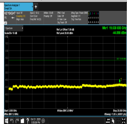
Band4-5MHz-16QAM-20375-25RB#0-3000~20000-PASS
