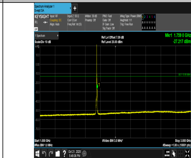
Band4-5MHz-QPSK-20375-1RB#0-1000~3000-PASS
