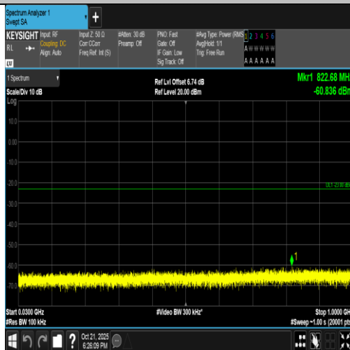
Band4-10MHz-16QAM-20000-1RB#49-30~1000-PASS
