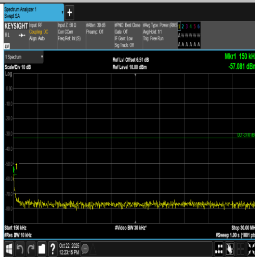
Band4-10MHz-16QAM-20000-50RB#0-0.15~30-PASS
