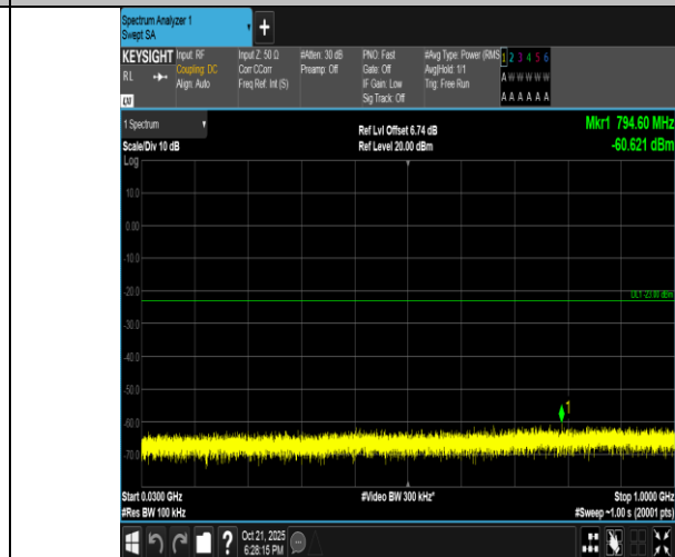
Band4-10MHz-16QAM-20175-1RB#0-30~1000-PASS
