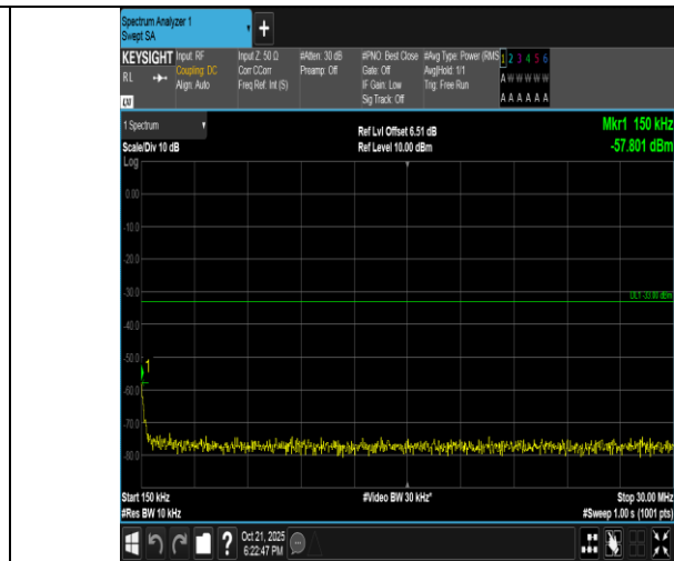
Band4-10MHz-QPSK-20000-1RB#0-0.15~30-PASS
