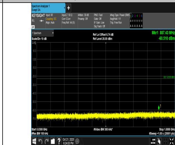
Band4-10MHz-16QAM-20000-1RB#0-30~1000-PASS
