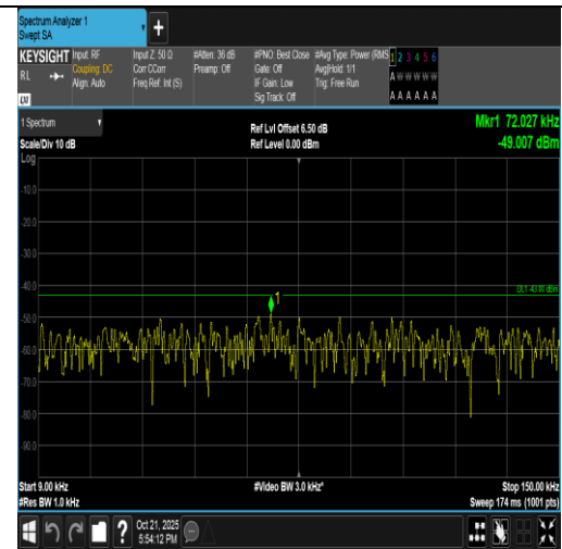
Band4-5MHz-16QAM-20375-25RB#0-0.009~0.15-PASS
