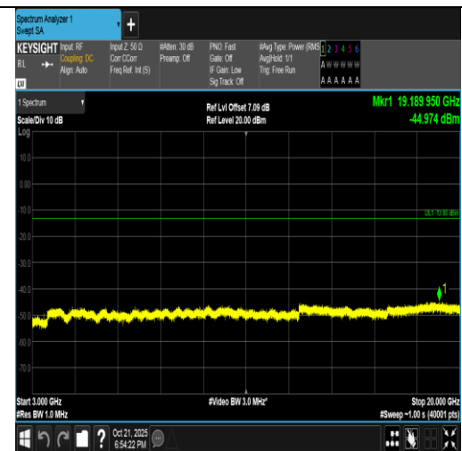
Band4-15MHz-16QAM-20175-1RB#0-3000~20000-PASS
