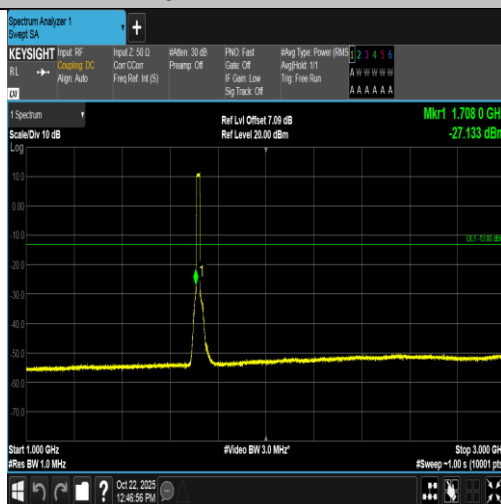
Band4-15MHz-16QAM-20025-75RB#0-1000~3000-PASS
