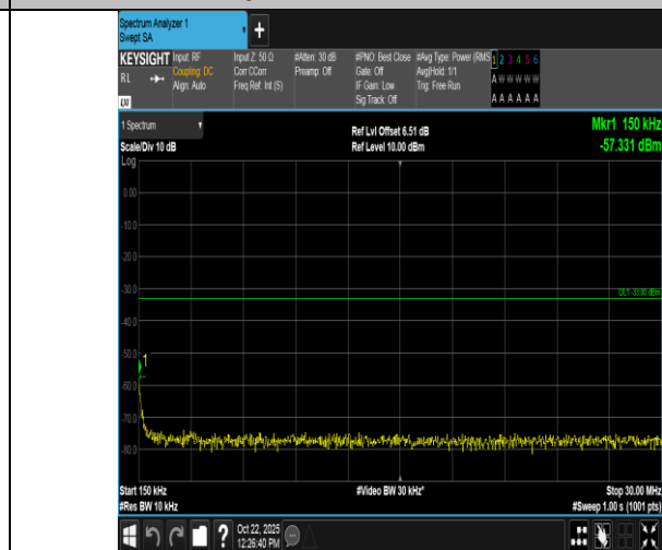
Band4-10MHz-QPSK-20350-50RB#0-0.15~30-PASS
