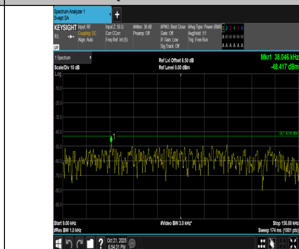
Band4-15MHz-QPSK-20175-1RB#74-0.009~0.15-PASS
