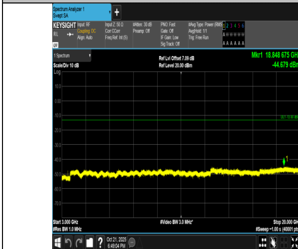
Band4-15MHz-QPSK-20025-1RB#0-3000~20000-PASS
