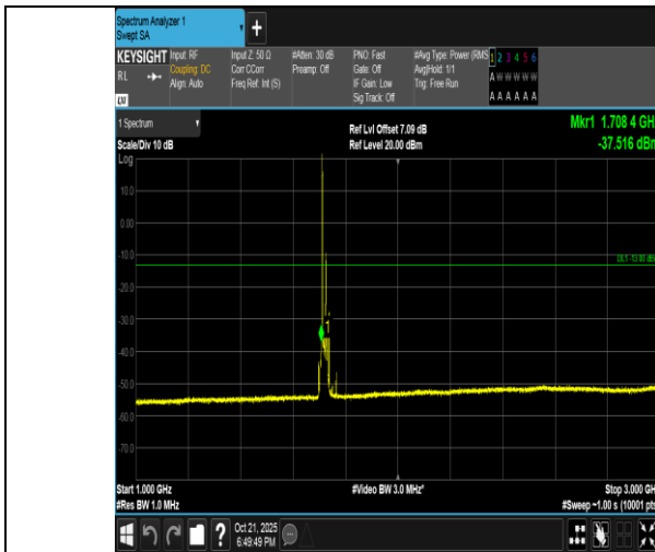
Band4-15MHz-16QAM-20025-1RB#0-1000~3000-PASS
