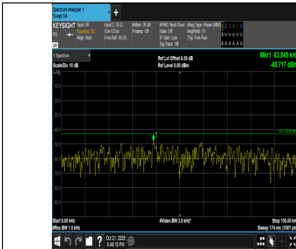
Band4-15MHz-QPSK-20025-1RB#0-0.009~0.15-PASS
