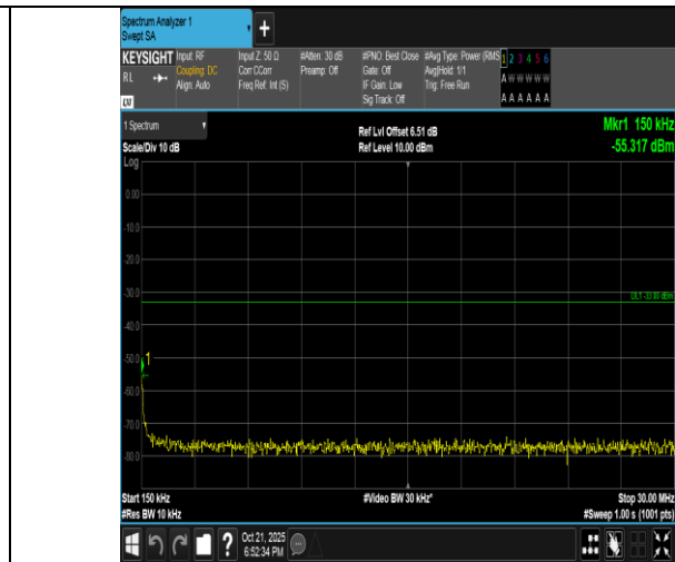
Band4-15MHz-QPSK-20175-1RB#0-0.15~30-PASS
