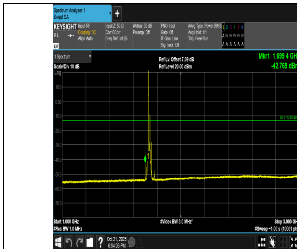
Band4-15MHz-16QAM-20175-1RB#0-1000~3000-PASS
