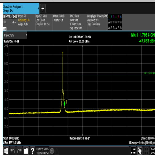
Band4-10MHz-16QAM-20175-50RB#0-1000~3000-PASS
