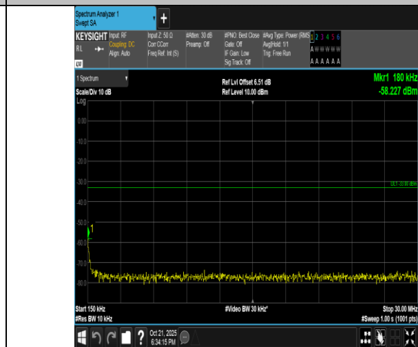
Band4-10MHz-16QAM-20350-1RB#49-0.15~30-PASS
