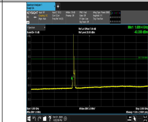
Band4-15MHz-QPSK-20175-1RB#0-1000~3000-PASS
