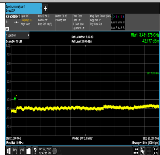
Band4-15MHz-16QAM-20025-75RB#0-3000~20000-PASS
