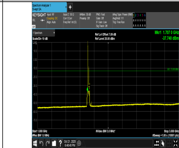
Band4-15MHz-QPSK-20025-1RB#0-1000~3000-PASS
