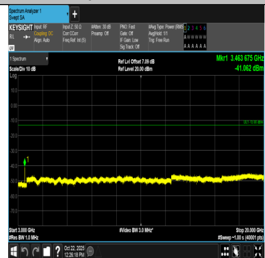
Band4-10MHz-16QAM-20175-50RB#0-3000~20000-PASS
