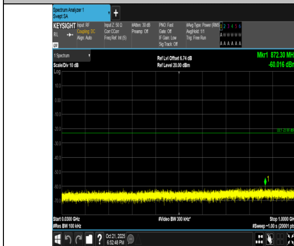
Band4-15MHz-QPSK-20175-1RB#0-30~1000-PASS
