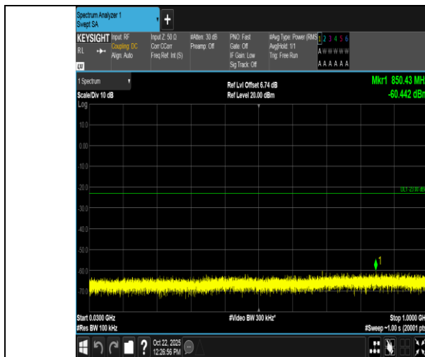
Band4-10MHz-QPSK-20350-50RB#0-30~1000-PASS
