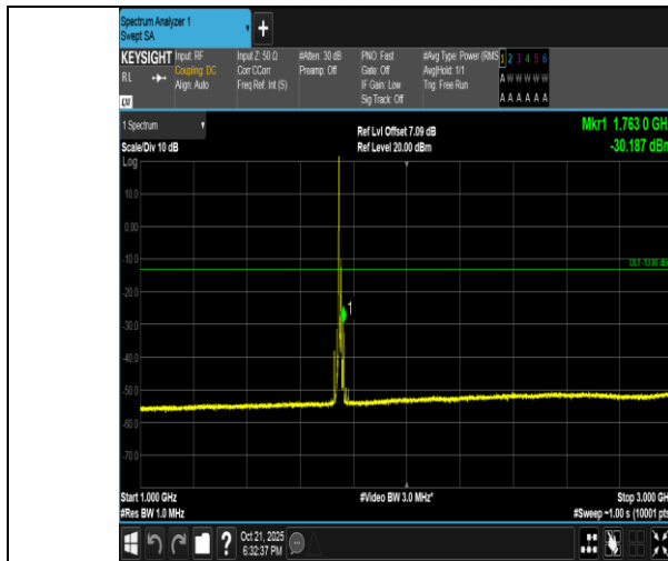
Band4-10MHz-16QAM-20350-1RB#0-1000~3000-PASS
