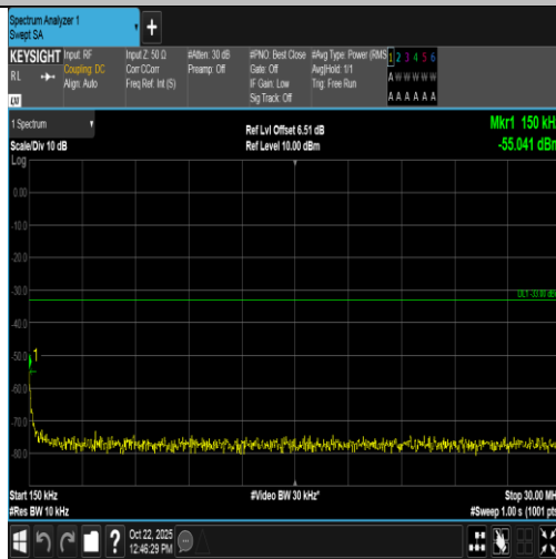
Band4-15MHz-16QAM-20025-75RB#0-0.15~30-PASS
