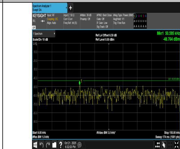
Band4-10MHz-16QAM-20350-1RB#0-0.009~0.15-PASS
