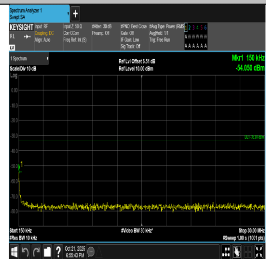
Band4-15MHz-16QAM-20175-1RB#74-0.15~30-PASS
