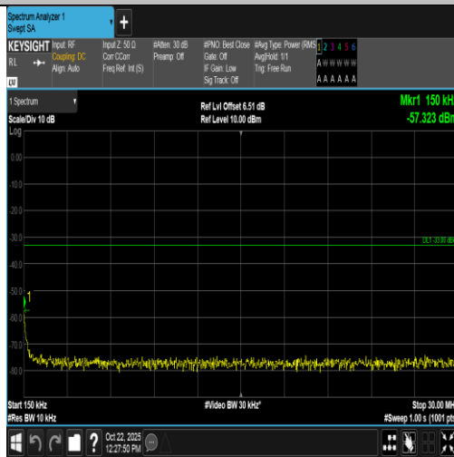
Band4-10MHz-16QAM-20350-50RB#0-0.15~30-PASS
