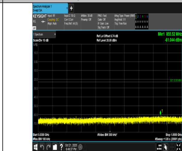
Band4-15MHz-16QAM-2025-1RB#0-30~1000-PASS
