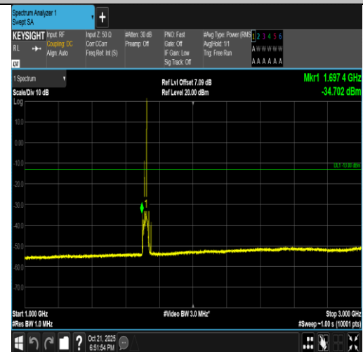
Band4-15MHz-16QAM-20025-1RB#74-1000~3000-PASS
