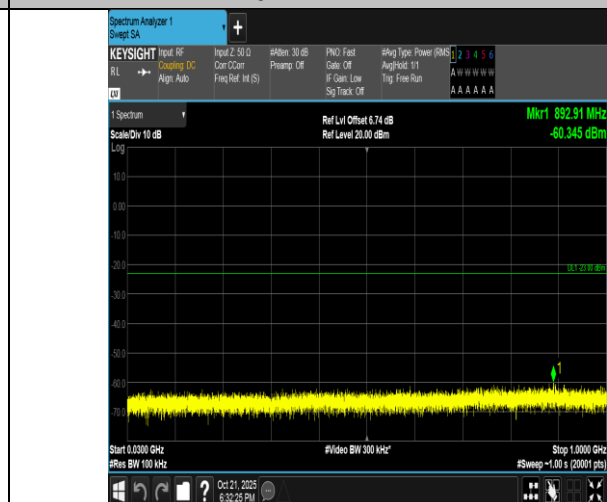
Band4-10MHz-16QAM-20350-1RB#0-30~1000-PASS
