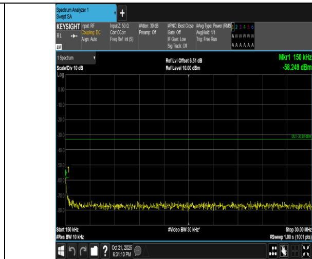
Band4-10MHz-QPSK-20350-1RB#0-0.15~30-PASS
