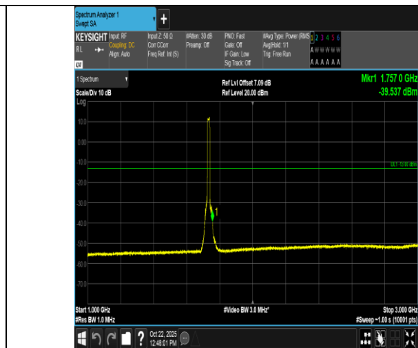
Band4-15MHz-QPSK-20175-75RB#0-1000~3000-PASS
