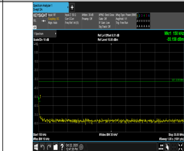
Band4-15MHz-QPSK-20175-75RB#0-0.15~30-PASS
