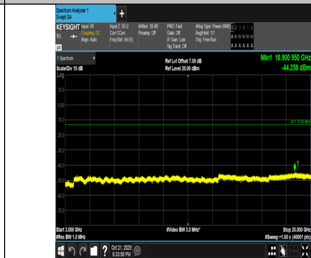
Band4-10MHz-QPSK-20350-1RB#49-3000~20000-PASS
