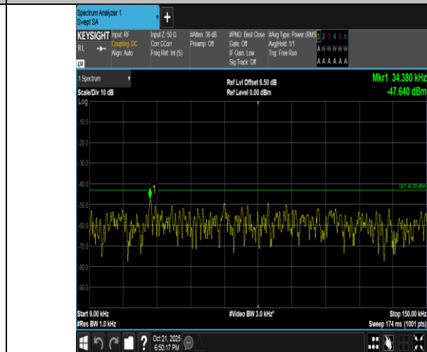
Band4-15MHz-QPSK-20025-1RB#74-0.009~0.15-PASS
