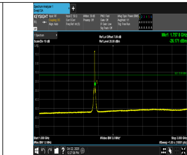
Band4-10MHz-QPSK-20350-50RB#0-1000~3000-PASS
