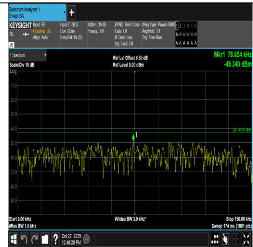
Band4-15MHz-16QAM-20025-75RB#0-0.009~0.15-PASS
