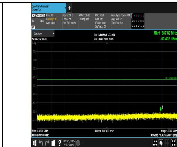
Band4-15MHz-QPSK-2025-1RB#74-30~1000-PASS
