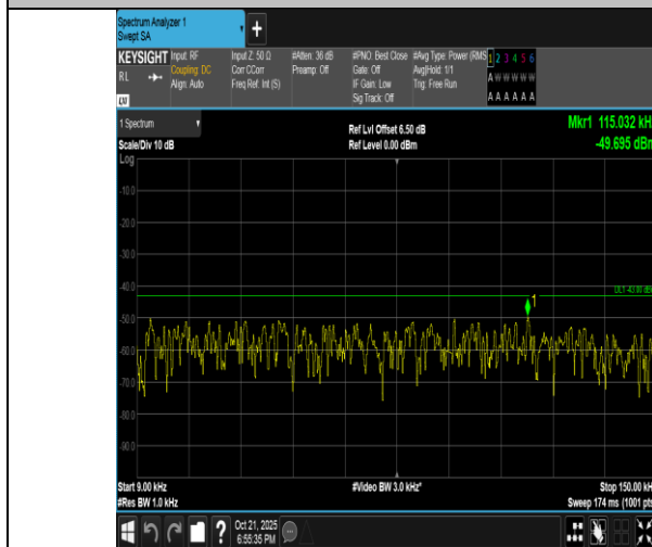
Band4-15MHz-16QAM-20175-1RB#74-0.009~0.15-PASS
