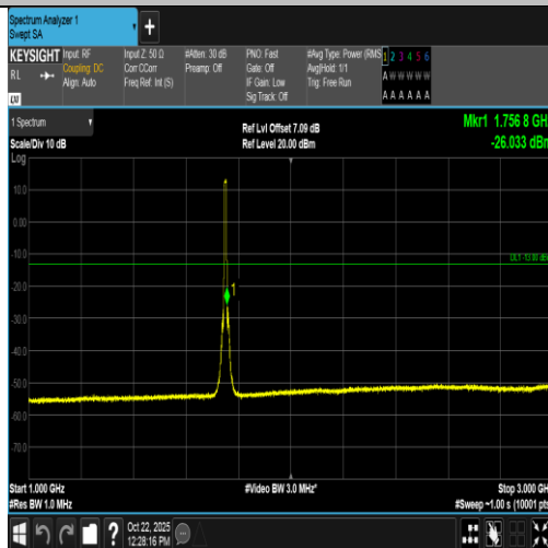
Band4-10MHz-16QAM-20350-50RB#0-1000~3000-PASS
