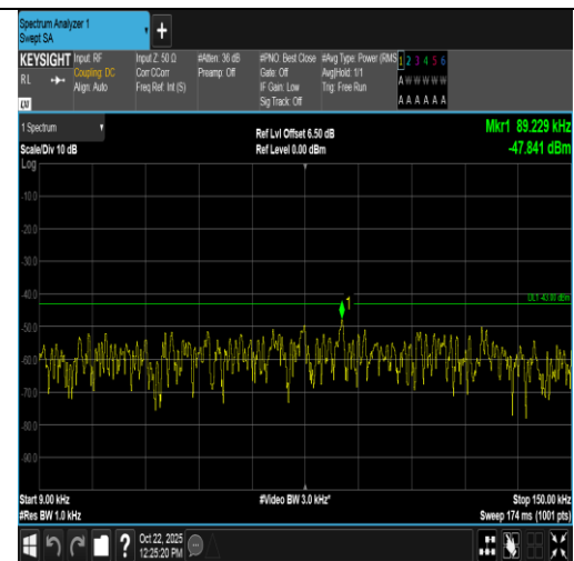
Band4-10MHz-16QAM-20175-50RB#0-0.009~0.15-PASS
