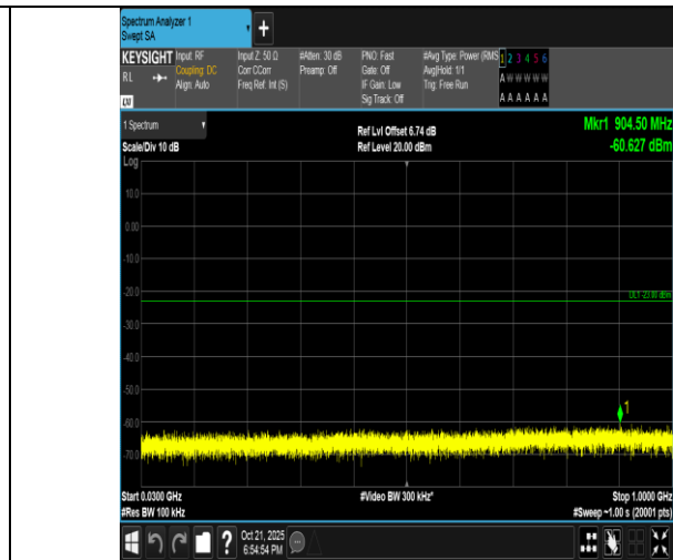
Band4-15MHz-QPSK-20175-1RB#74-30~1000-PASS
