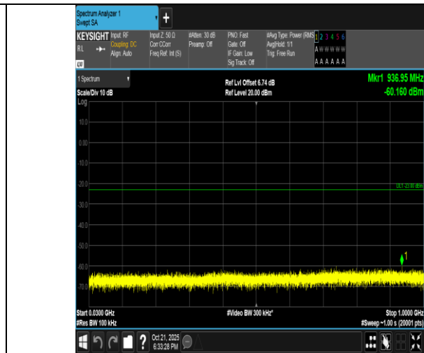
Band4-10MHz-QPSK-20350-1RB#49-30~1000-PASS
