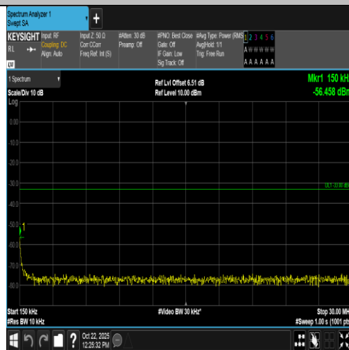
Band4-10MHz-16QAM-20175-50RB#0-0.15~30-PASS
