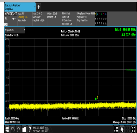
Band4-10MHz-16QAM-20175-50RB#0-30~1000-PASS
