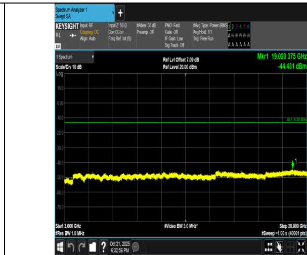
Band4-10MHz-16QAM-20350-1RB#0-3000~20000-PASS
