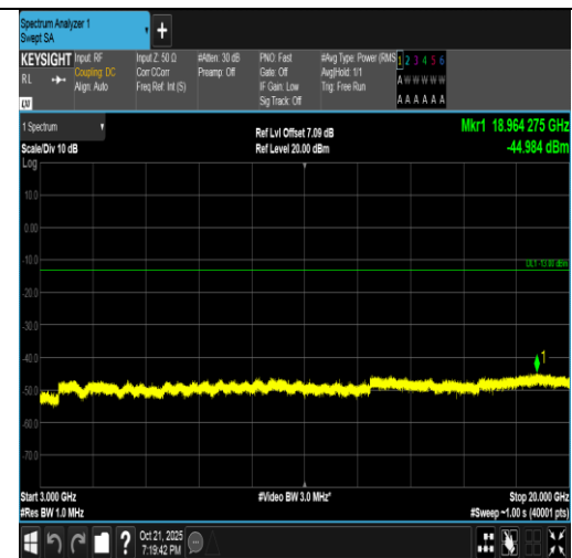
Band4-20MHz-16QAM-20175-1RB#0-3000~20000-PASS
