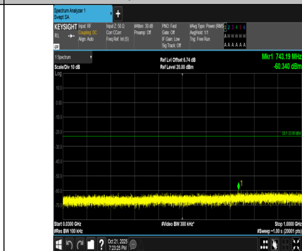
Band4-20MHz-16QAM-20300-1RB#0-30~1000-PASS
