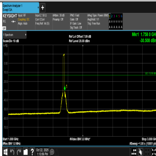
Band4-20MHz-16QAM-20300-100RB#0-1000~3000-PASS
