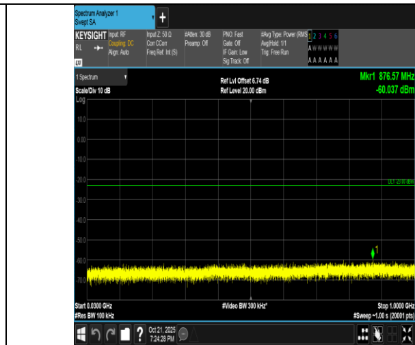
Band4-20MHz-QPSK-20300-1RB#99-30~1000-PASS
