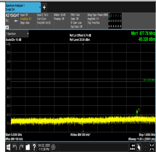
Band4-20MHz-16QAM-20175-100RB#0-30~1000-PASS
