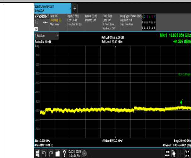
Band4-20MHz-QPSK-20300-1RB#99-3000~20000-PASS
