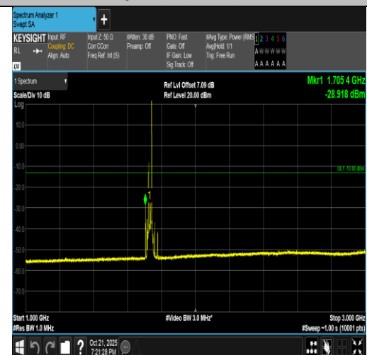
Band4-20MHz-16QAM-20175-1RB#99-1000~3000-PASS
