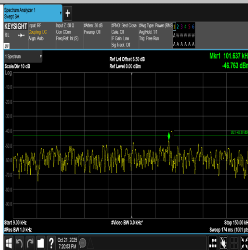
Band4-20MHz-16QAM-20175-1RB#99-0.009~0.15-PASS
