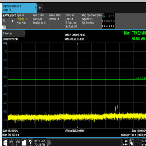
Band4-20MHz-16QAM-20175-1RB#99-30~1000-PASS
