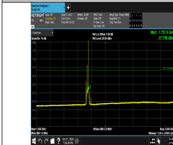
Band4-20MHz-QPSK-20300-1RB#99-1000~3000-PASS
