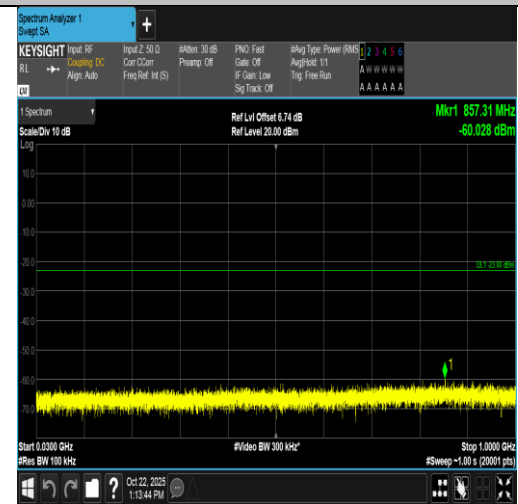
Band4-20MHz-16QAM-20300-100RB#0-30~1000-PASS
