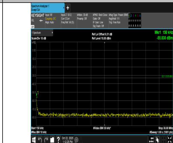
Band4-20MHz-QPSK-20300-100RB#0-0.15~30-PASS
