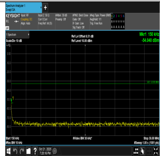
Band4-20MHz-16QAM-20300-1RB#99-0.15~30-PASS
