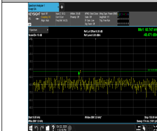
Band4-20MHz-QPSK-20300-100RB#0-0.009~0.15-PASS
