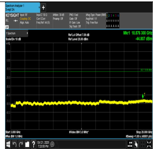
Band4-20MHz-16QAM-20300-1RB#0-3000~20000-PASS
