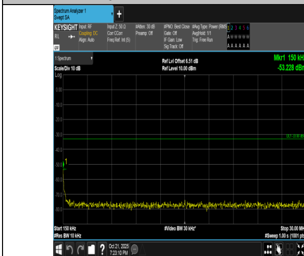
Band4-20MHz-16QAM-20300-1RB#0-0.15~30-PASS
