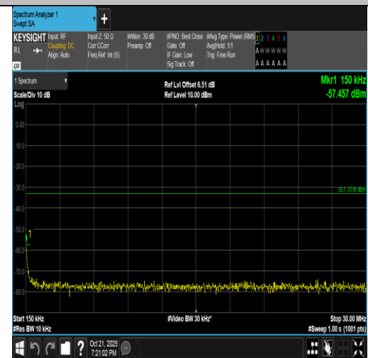
Band4-20MHz-16QAM-20175-1RB#99-0.15~30-PASS
