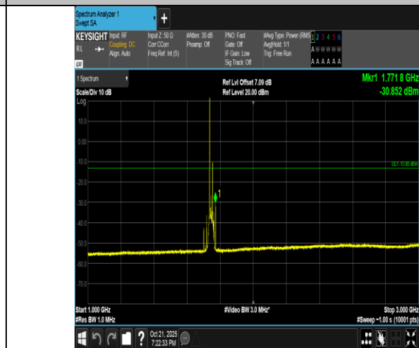
Band4-20MHz-QPSK-20300-1RB#0-1000~3000-PASS
