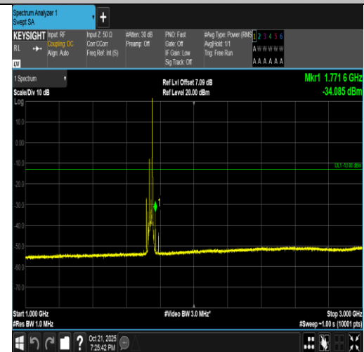
Band4-20MHz-16QAM-20300-1RB#99-1000~3000-PASS
