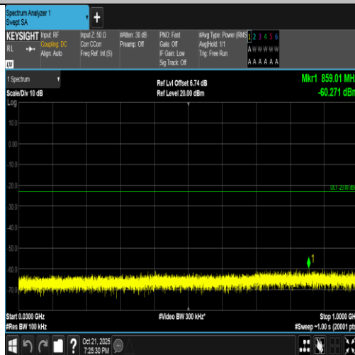
Band4-20MHz-16QAM-20300-1RB#99-30~1000-PASS
