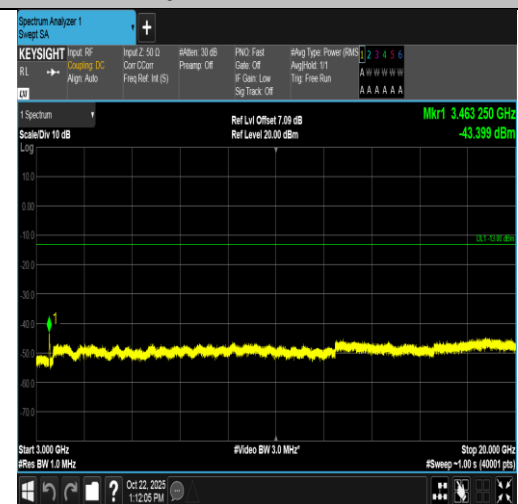
Band4-20MHz-16QAM-20175-100RB#0-3000~20000-PASS
