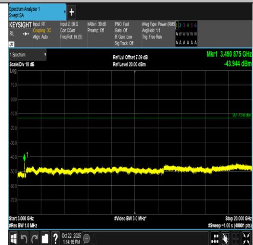
Band4-20MHz-16QAM-20300-100RB#0-3000~20000-PASS
