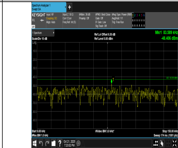
Band4-20MHz-16QAM-20300-1RB#0-0.009~0.15-PASS
