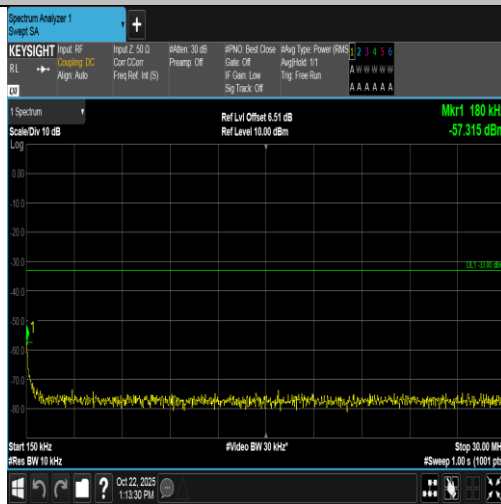
Band4-20MHz-16QAM-20300-100RB#0-0.15~30-PASS
