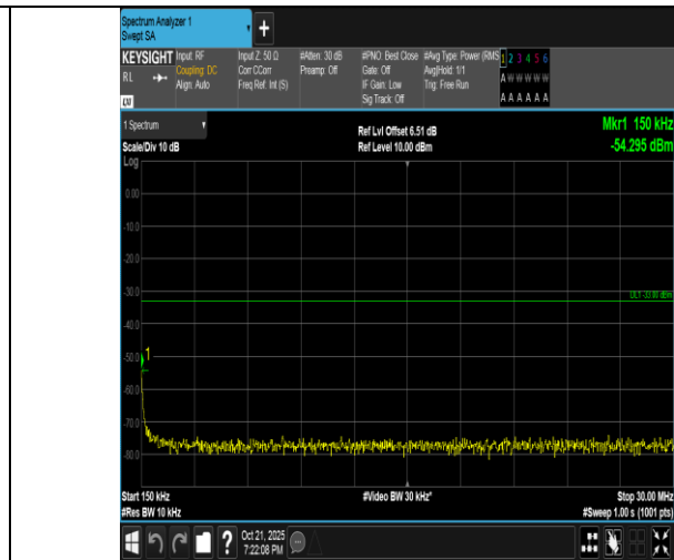
Band4-20MHz-QPSK-20300-1RB#0-0.15~30-PASS
