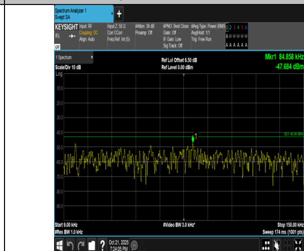
Band4-20MHz-QPSK-20300-1RB#99-0.009~0.15-PASS
