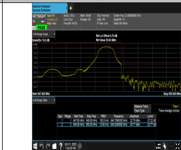
Band5-1.4MHz-QPSK-20643-1RB#5-PASS
