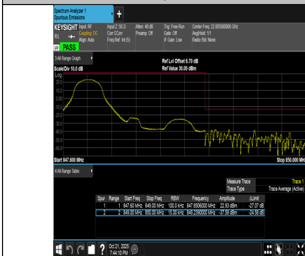
Band5-1.4MHz-QPSK-20643-1RB#0-PASS
