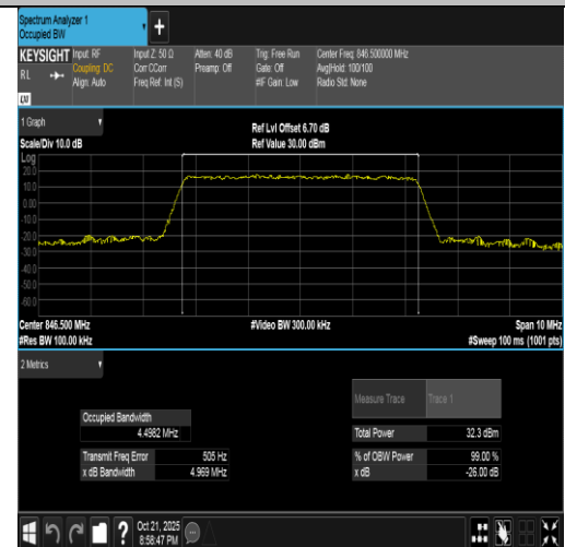
Band5-5MHz-16QAM-20625-25RB#0-PASS
