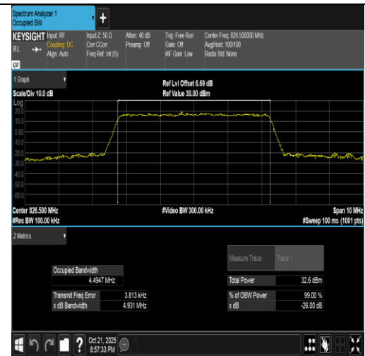
Band5-5MHz-16QAM-20425-25RB#0-PASS
