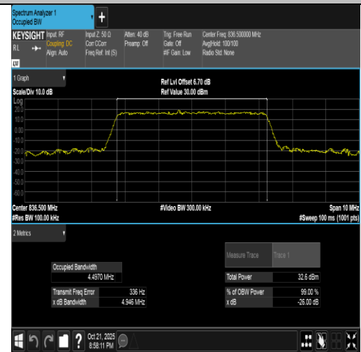
Band5-5MHz-16QAM-20525-25RB#0-PASS
