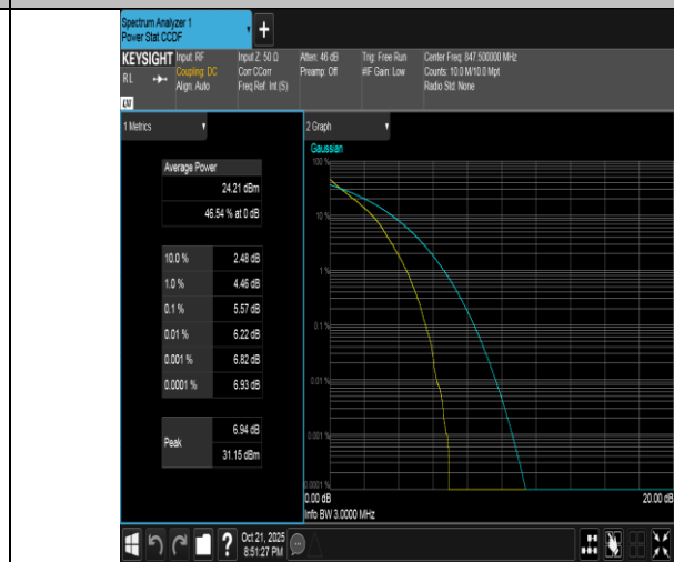
Band5-3MHz-QPSK-20635-15RB#0-PASS
