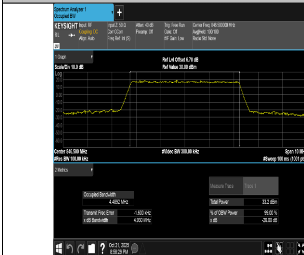
Band5-5MHz-QPSK-20625-25RB#0-PASS
