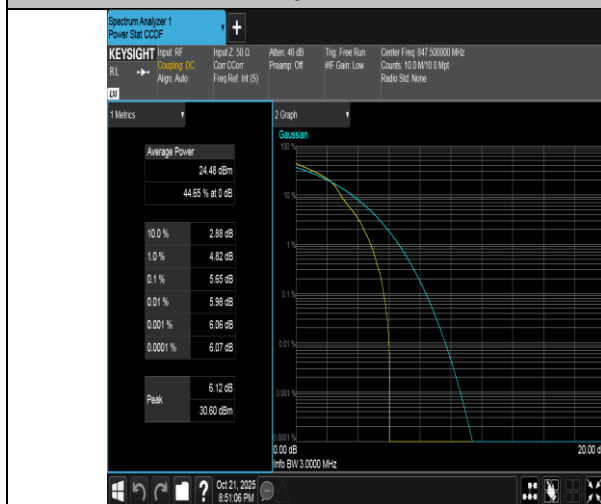
Band5-3MHz-16QAM-20635-1RB#0-PASS
