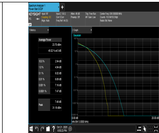
Band5-3MHz-16QAM-20525-15RB#0-PASS
