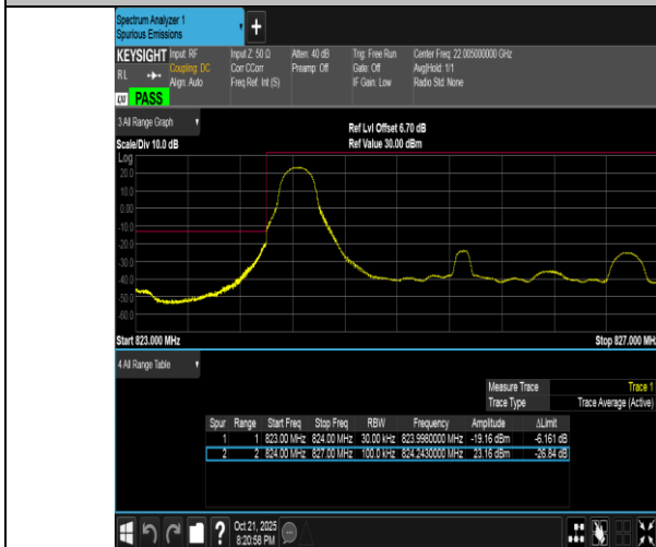
Band5-3MHz-QPSK-20415-1RB#0-PASS
