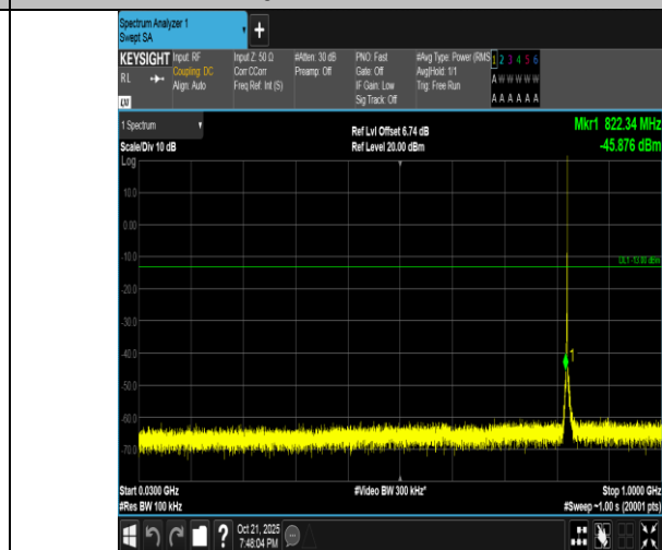
Band5-1.4MHz-QPSK-20407-1RB#5-30~1000-PASS
