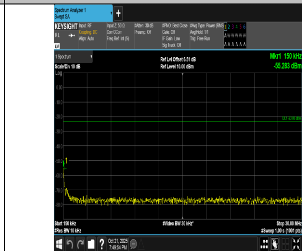
Band5-1.4MHz-QPSK-20407-6RB#0-0.15~30-PASS
