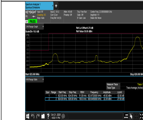
Band5-5MHz-16QAM-20425-1RB#24-PASS
