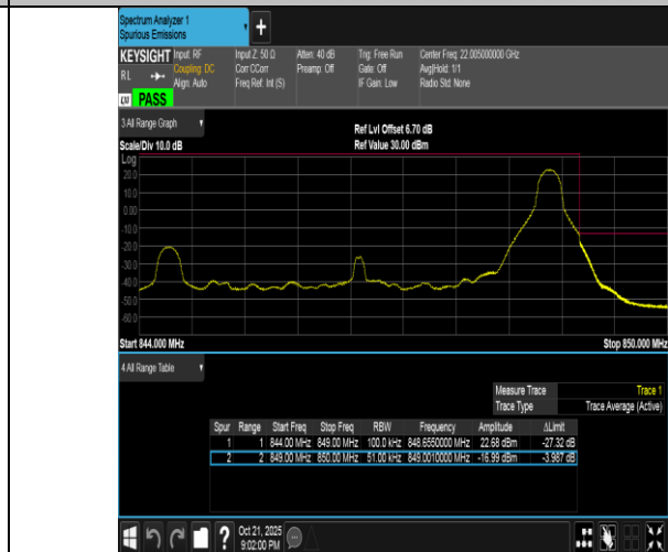
Band5-5MHz-QPSK-20625-1RB#24-PASS
