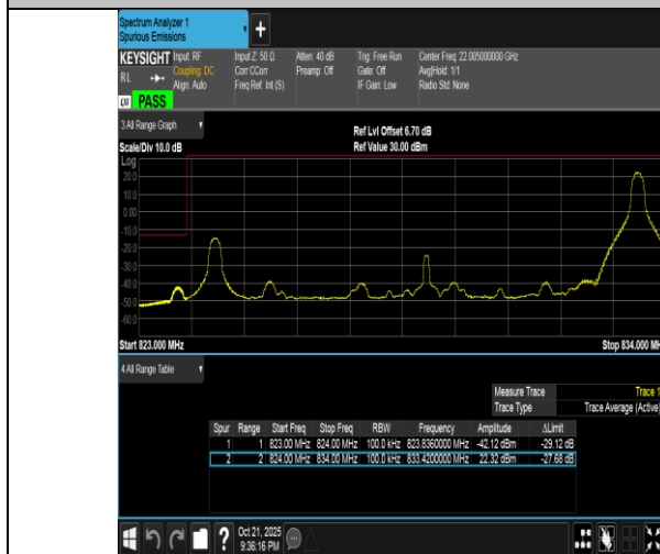
Band5-10MHz-16QAM-20450-1RB#49-PASS
