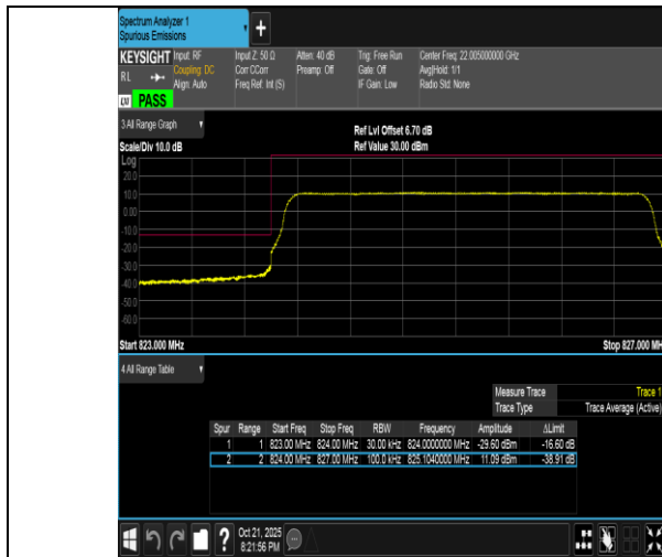
Band5-3MHz-QPSK-20415-15RB#0-PASS
