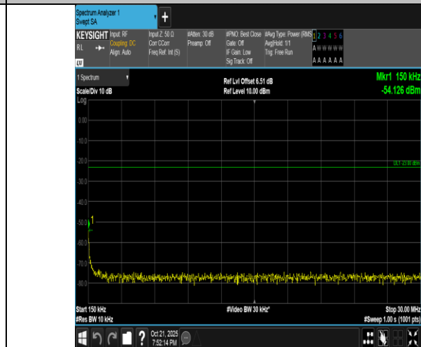
Band5-1.4MHz-QPSK-20525-1RB#0-0.15~30-PASS
