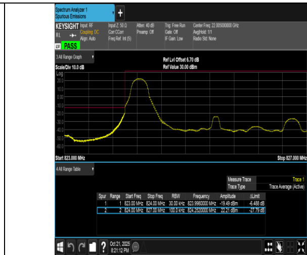
Band5-3MHz-16QAM-20415-1RB#0-PASS
