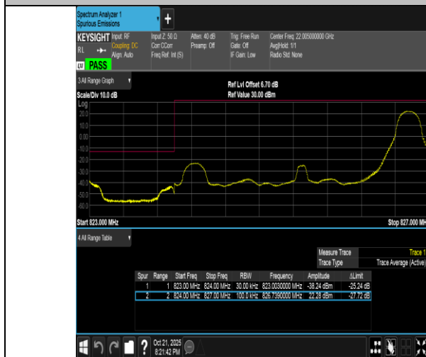
Band5-3MHz-16QAM-20415-1RB#14-PASS
