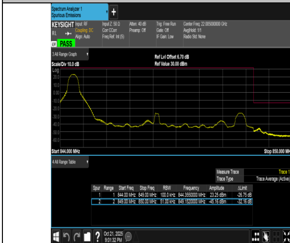
Band5-5MHz-QPSK-20625-1RB#0-PASS
