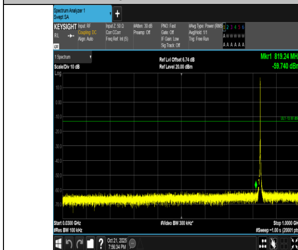
Band5-1.4MHz-QPSK-20525-6RB#0-30~1000-PASS
