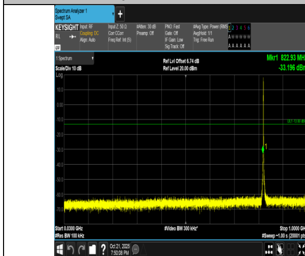
Band5-1.4MHz-QPSK-20407-6RB#0-30~1000-PASS
