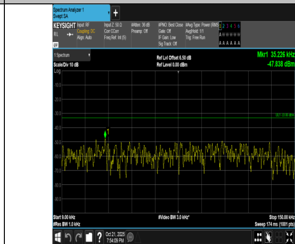
Band5-1.4MHz-QPSK-20525-1RB#5-0.009~0.15-PASS
