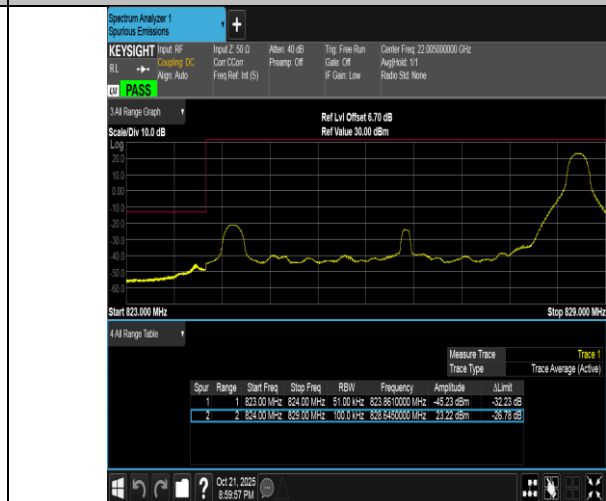
Band5-5MHz-QPSK-20425-1RB#24-PASS
