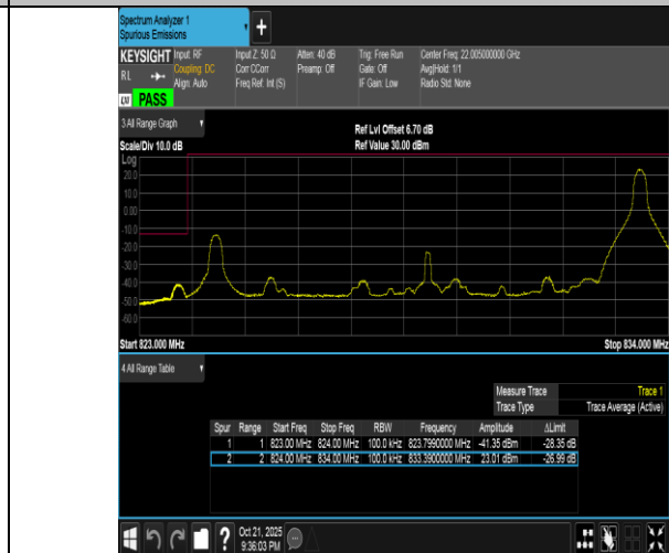
Band5-10MHz-QPSK-20450-1RB#49-PASS
