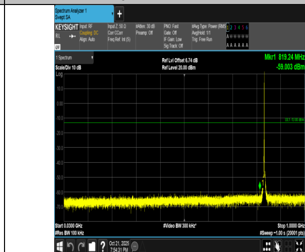
Band5-1.4MHz-QPSK-20525-1RB#5-30~1000-PASS
