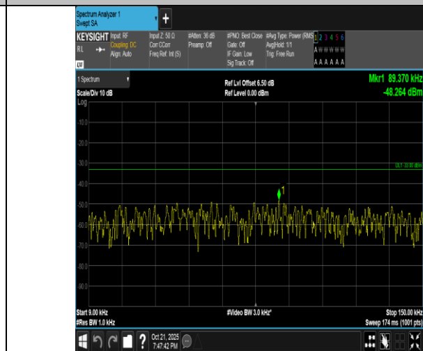
Band5-1.4MHz-QPSK-20407-1RB#5-0.009~0.15-PASS
