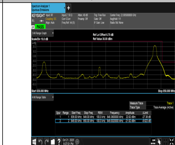
Band5-10MHz-QPSK-20600-1RB#49-PASS
