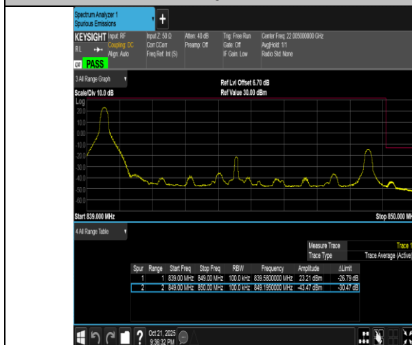
Band5-10MHz-QPSK-20600-1RB#0-PASS
