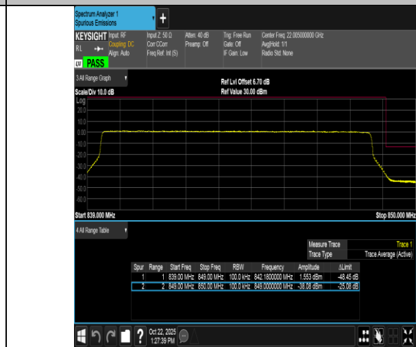
Band5-10MHz-16QAM-20600-50RB#0-PASS
