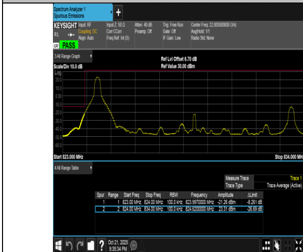
Band5-10MHz-QPSK-20450-1RB#0-PASS
