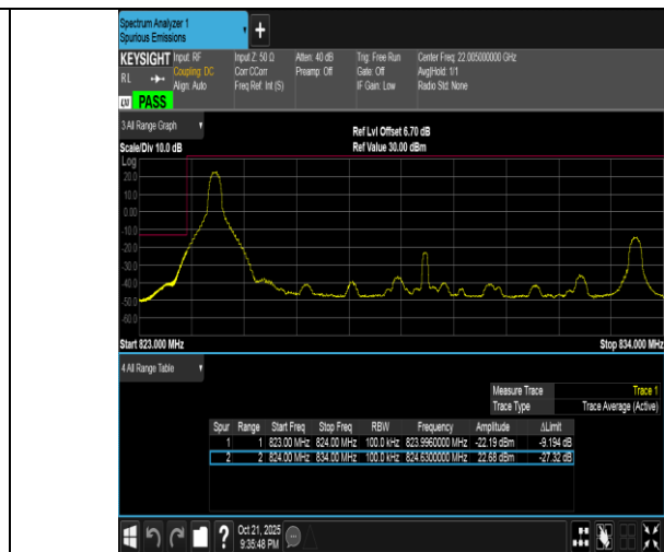
Band5-10MHz-16QAM-20450-1RB#0-PASS
