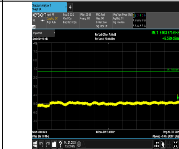
Band5-1.4MHz-16QAM-20407-6RB#0-3000~10000-PASS
