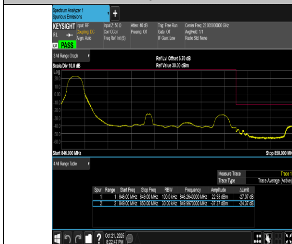
Band5-3MHz-QPSK-20635-1RB#0-PASS
