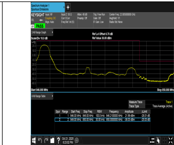
Band5-3MHz-16QAM-20635-1RB#0-PASS
