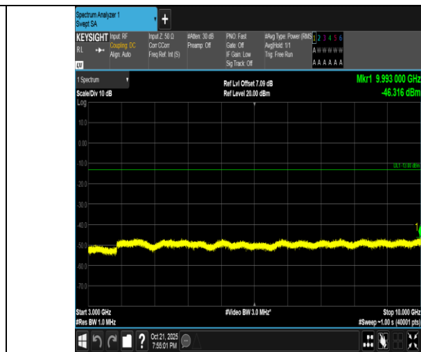
Band5-1.4MHz-QPSK-20525-1RB#5-3000~10000-PASS
