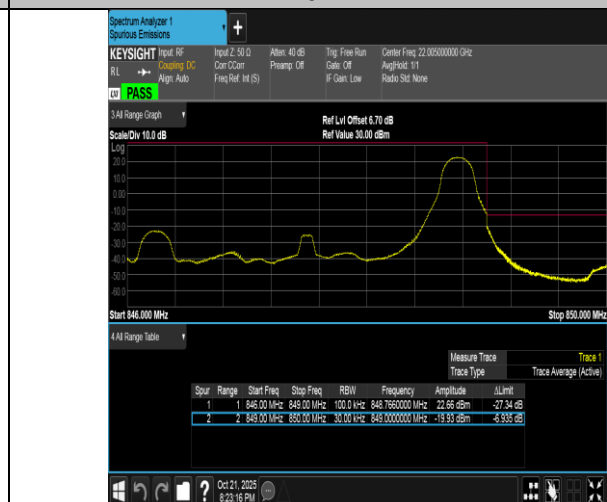
Band5-3MHz-QPSK-20635-1RB#14-PASS
