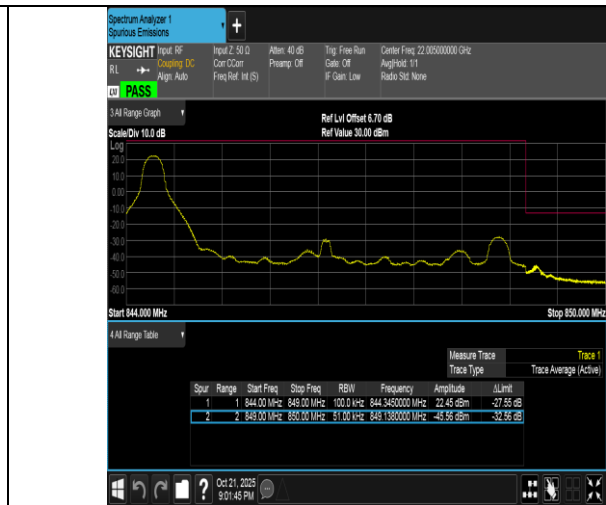
Band5-5MHz-16QAM-20625-1RB#0-PASS
