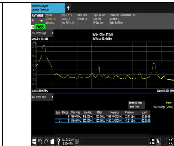
Band5-10MHz-16QAM-20600-1RB#0-PASS
