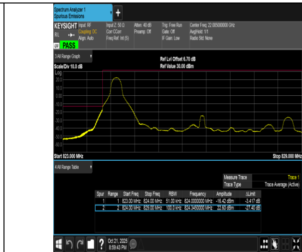
Band5-5MHz-16QAM-20425-1RB#0-PASS
