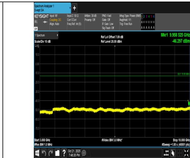
Band5-1.4MHz-QPSK-20407-1RB#5-3000~10000-PASS
