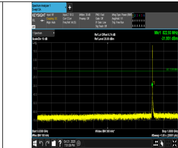
Band5-1.4MHz-16QAM-20407-6RB#0-30~1000-PASS
