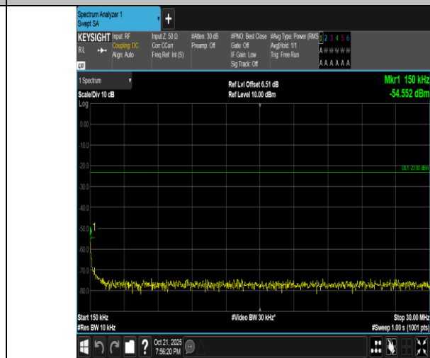
Band5-1.4MHz-QPSK-20525-6RB#0-0.15~30-PASS
