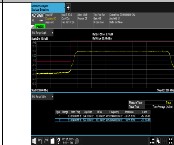
Band5-3MHz-16QAM-20415-15RB#0-PASS
