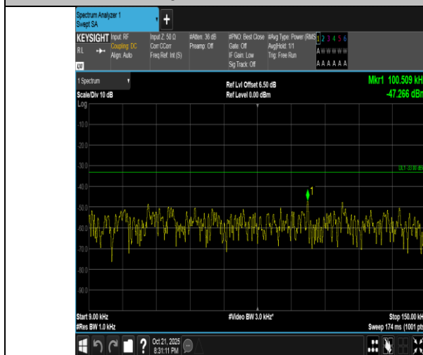
Band5-3MHz-QPSK-20525-1RB#0-0.009~0.15-PASS
