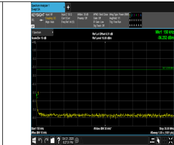
Band5-3MHz-16QAM-20415-1RB#14-0.15~30-PASS
