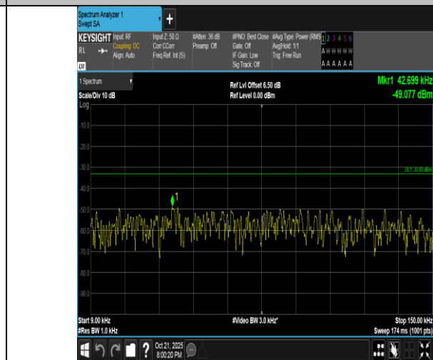
Band5-1.4MHz-QPSK-20643-1RB#5-0.009~0.15-PASS
