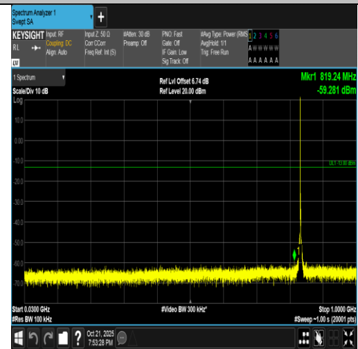
Band5-1.4MHz-16QAM-20525-1RB#0-30~1000-PASS
