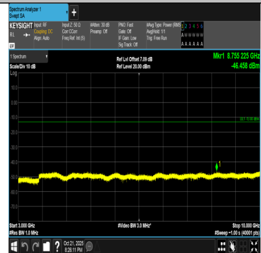
Band5-3MHz-16QAM-20415-1RB#0-3000~10000-PASS
