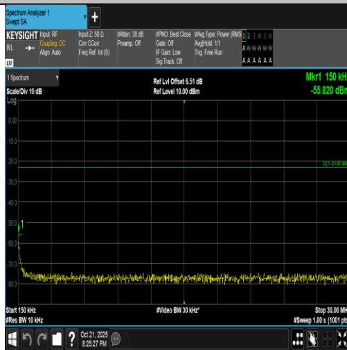
Band5-3MHz-16QAM-20415-1RB#0-0.15~30-PASS
