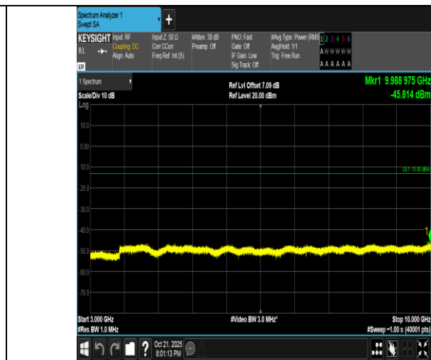
Band5-1.4MHz-QPSK-20643-1RB#5-3000~10000-PASS
