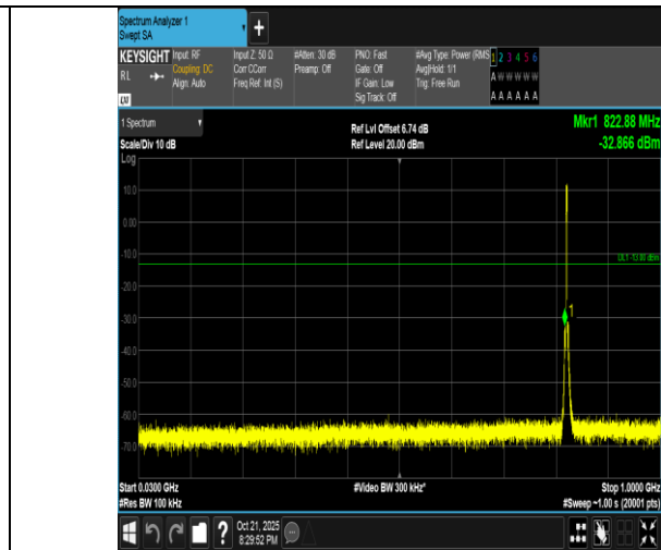
Band5-3MHz-16QAM-20415-15RB#0-30~1000-PASS
