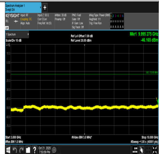
Band5-1.4MHz-16QAM-20525-1RB#0-3000~10000-PASS
