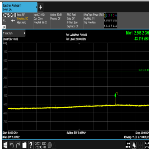
Band5-1.4MHz-16QAM-20525-1RB#0-1000~3000-PASS
