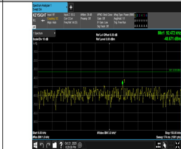
Band5-3MHz-16QAM-20415-15RB#0-0.009~0.15-PASS
