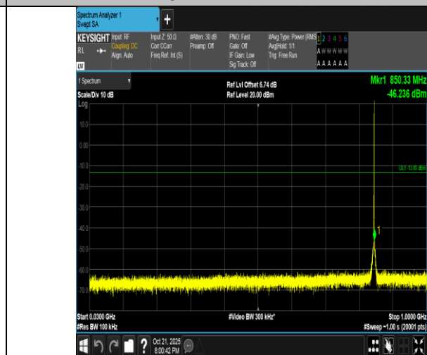
Band5-1.4MHz-QPSK-20643-1RB#5-30~1000-PASS
