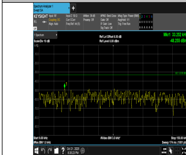
Band5-3MHz-QPSK-20525-15RB#0-0.009~0.15-PASS
