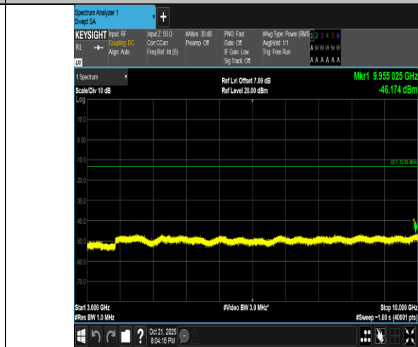
Band5-1.4MHz-16QAM-20643-6RB#0-3000~10000-PASS
