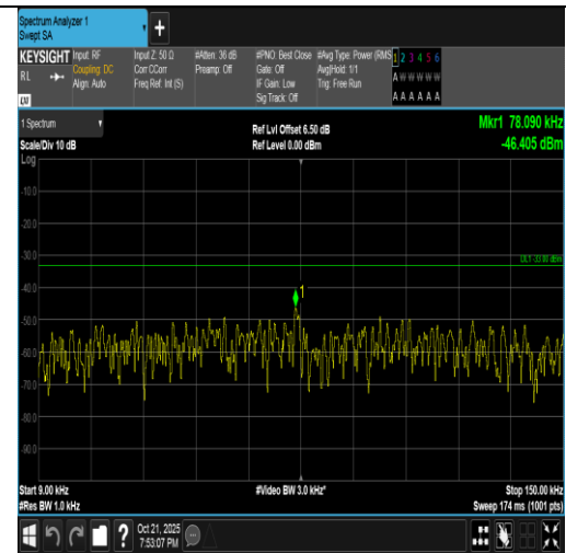
Band5-1.4MHz-16QAM-20525-1RB#0-0.009~0.15-PASS
