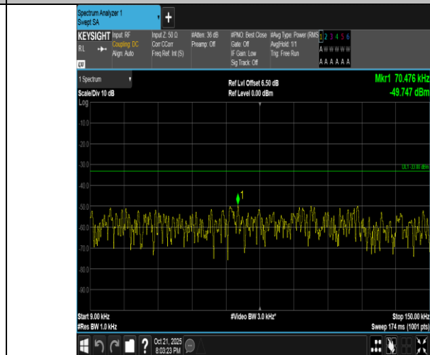
Band5-1.4MHz-16QAM-20643-6RB#0-0.009~0.15-PASS
