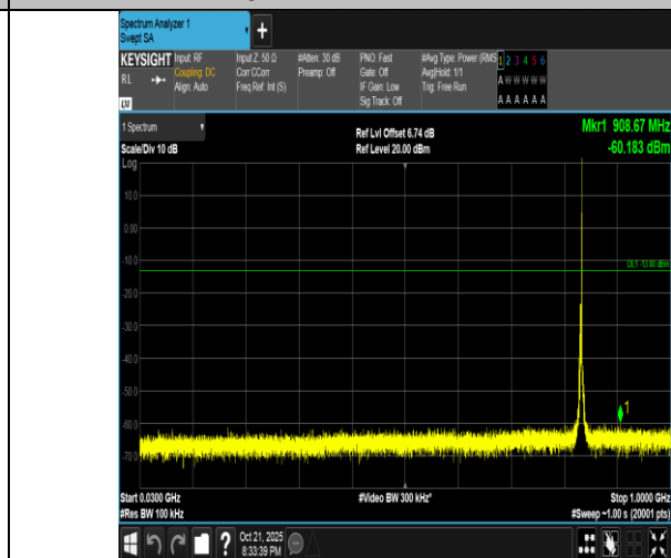
Band5-3MHz-QPSK-20525-1RB#14-30~1000-PASS
