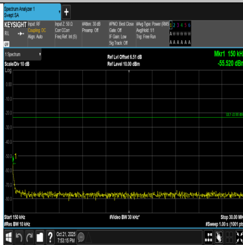
Band5-1.4MHz-16QAM-20525-1RB#0-0.15~30-PASS
