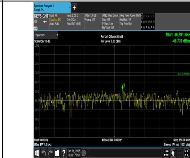
Band5-3MHz-QPSK-20525-1RB#14-0.009~0.15-PASS
