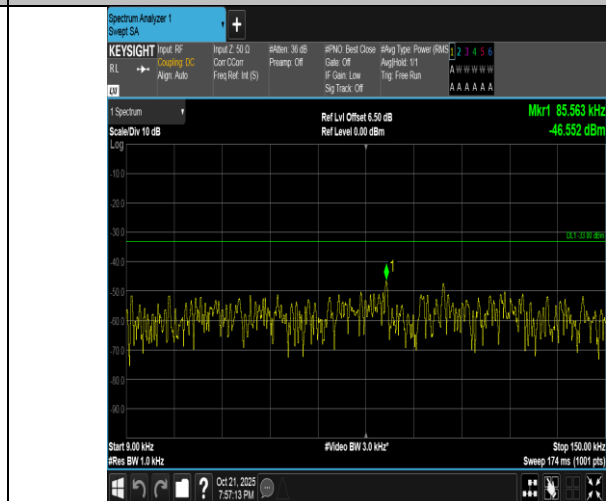
Band5-1.4MHz-16QAM-20525-6RB#0-0.009~0.15-PASS
