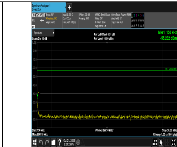
Band5-1.4MHz-16QAM-20643-1RB#5-0.15~30-PASS
