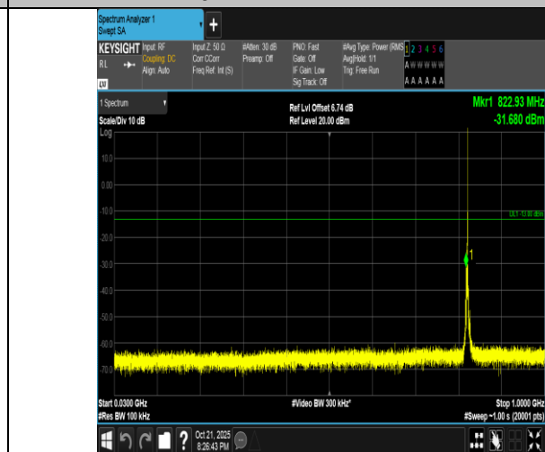
Band5-3MHz-QPSK-20415-1RB#14-30~1000-PASS
