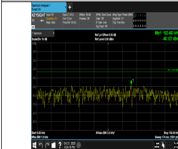
Band5-3MHz-QPSK-20415-1RB#0-0.009~0.15-PASS
