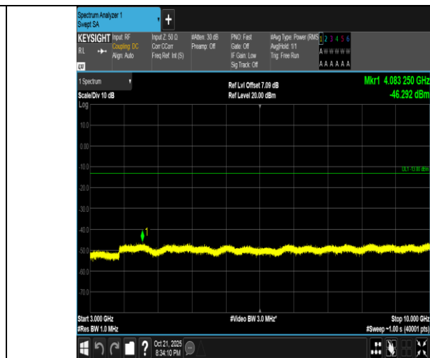
Band5-3MHz-QPSK-20525-1RB#14-3000~10000-PASS
