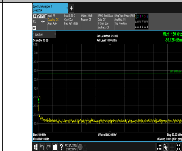
Band5-3MHz-QPSK-20525-1RB#0-0.15~30-PASS
