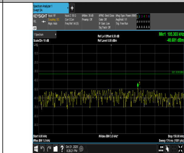
Band5-3MHz-QPSK-20415-1RB#14-0.009~0.15-PASS
