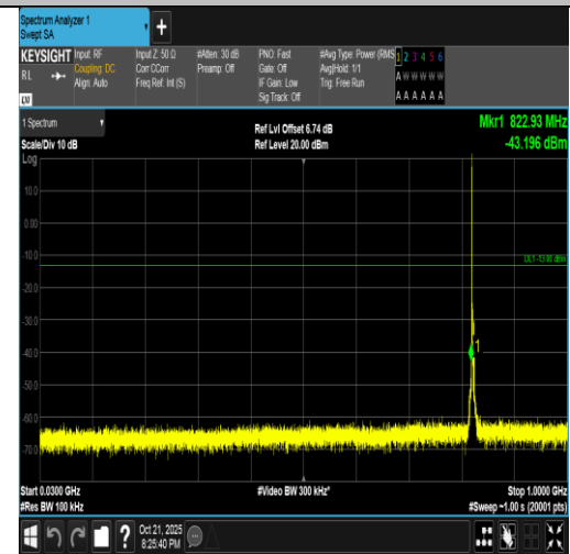
Band5-3MHz-16QAM-20415-1RB#0-30~1000-PASS
