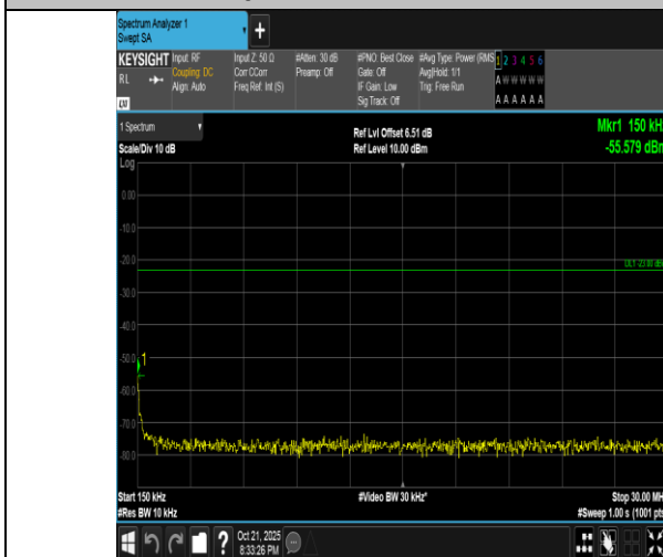
Band5-3MHz-QPSK-20525-1RB#14-0.15~30-PASS
