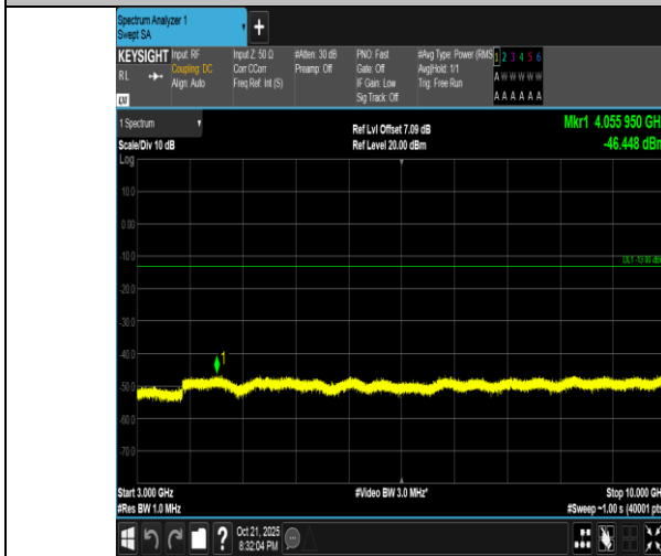
Band5-3MHz-QPSK-20525-1RB#0-3000~10000-PASS
