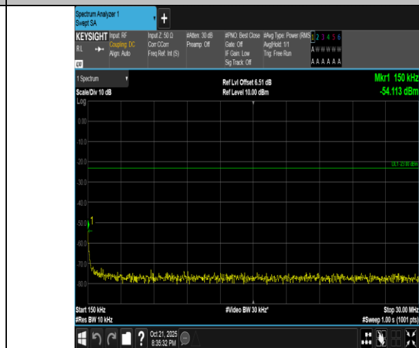
Band5-3MHz-QPSK-20525-15RB#0-0.15~30-PASS
