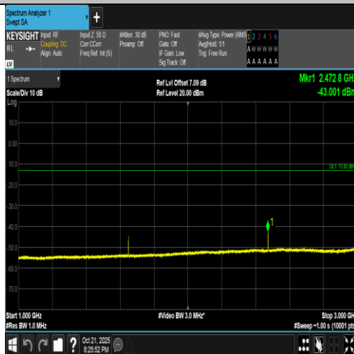
Band5-3MHz-16QAM-20415-1RB#0-1000~3000-PASS
