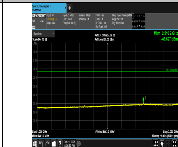
Band5-3MHz-QPSK-20525-15RB#0-1000~3000-PASS
