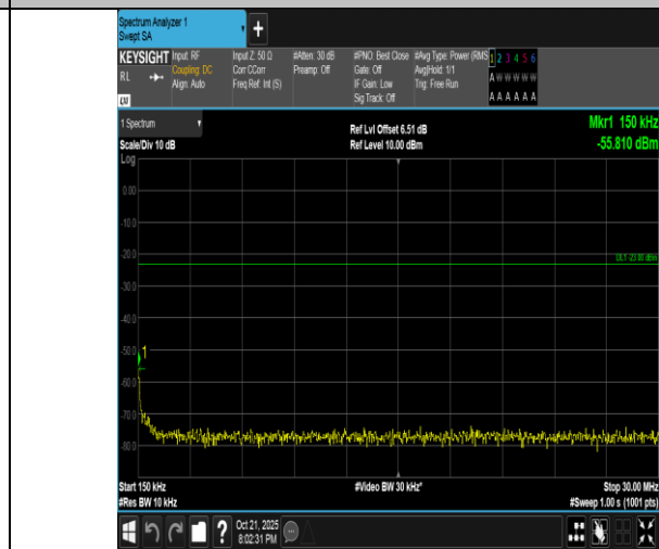
Band5-1.4MHz-QPSK-20643-6RB#0-0.15~30-PASS
