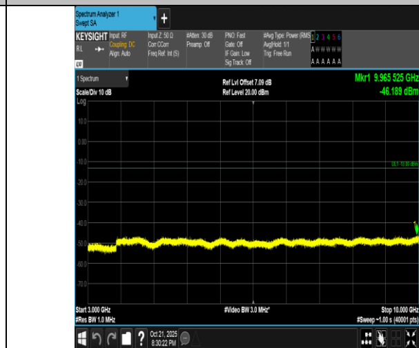
Band5-3MHz-16QAM-20415-15RB#0-3000~10000-PASS
