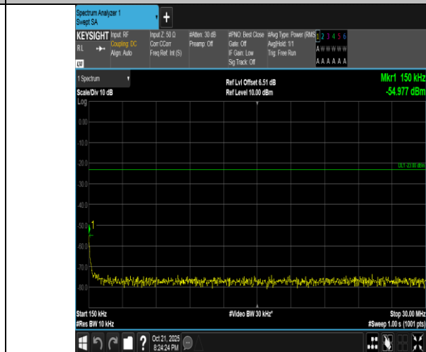
Band5-3MHz-QPSK-20415-1RB#0-0.15~30-PASS
