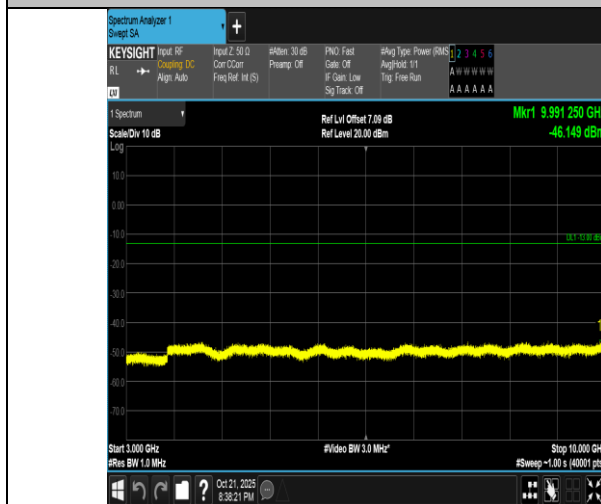
Band5-3MHz-QPSK-20635-1RB#0-3000~10000-PASS
