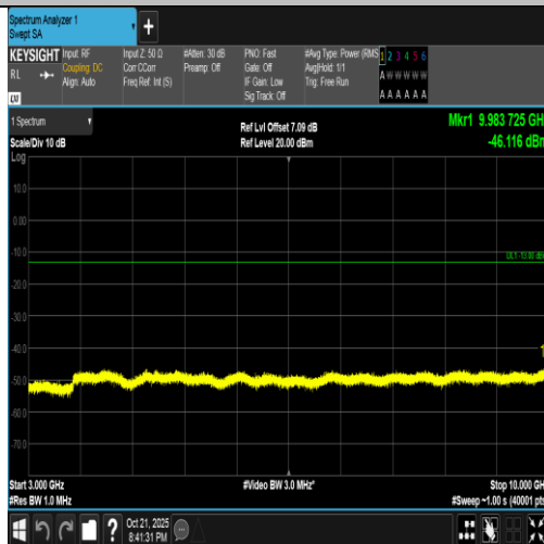
Band5-3MHz-16QAM-20635-1RB#14-3000~10000-PASS
