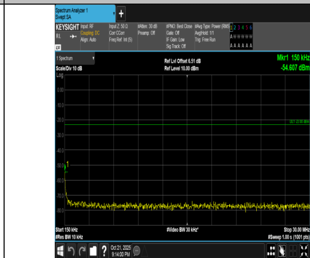
Band5-5MHz-QPSK-20525-25RB#0-0.15~30-PASS
