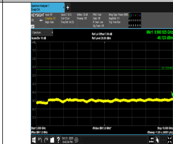
Band5-3MHz-16QAM-20635-15RB#0-3000~10000-PASS
