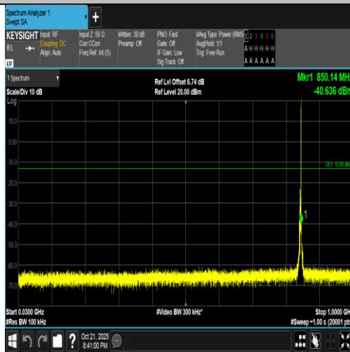
Band5-3MHz-16QAM-20635-1RB#14-30~1000-PASS
