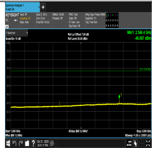
Band5-3MHz-16QAM-20635-1RB#14-1000~3000-PASS
