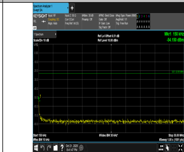
Band5-3MHz-QPSK-20635-15RB#0-0.15~30-PASS
