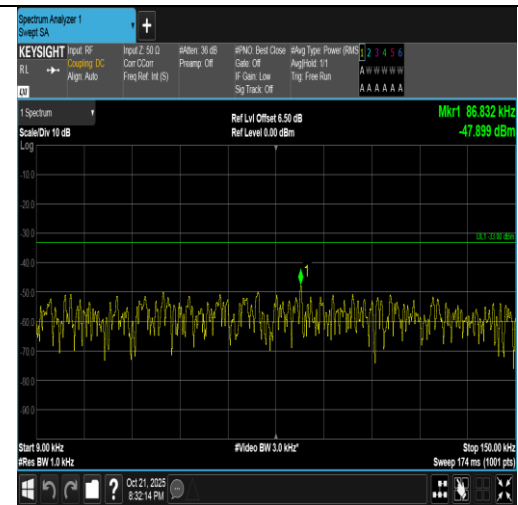
Band5-3MHz-16QAM-20525-1RB#0-0.009~0.15-PASS
