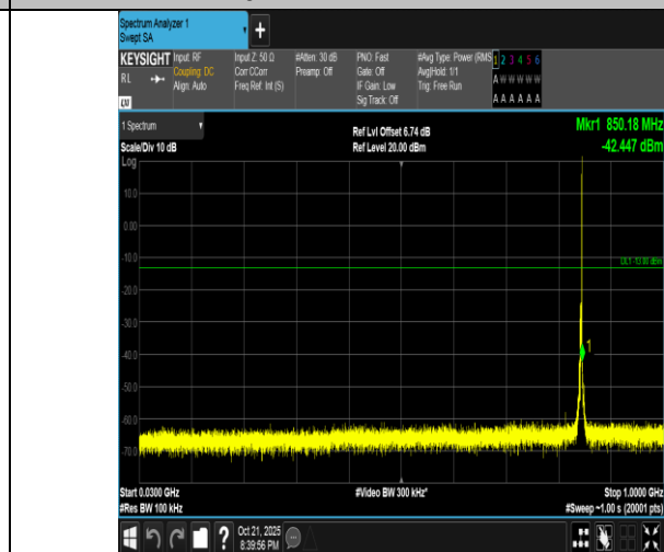
Band5-3MHz-QPSK-20635-1RB#14-30~1000-PASS
