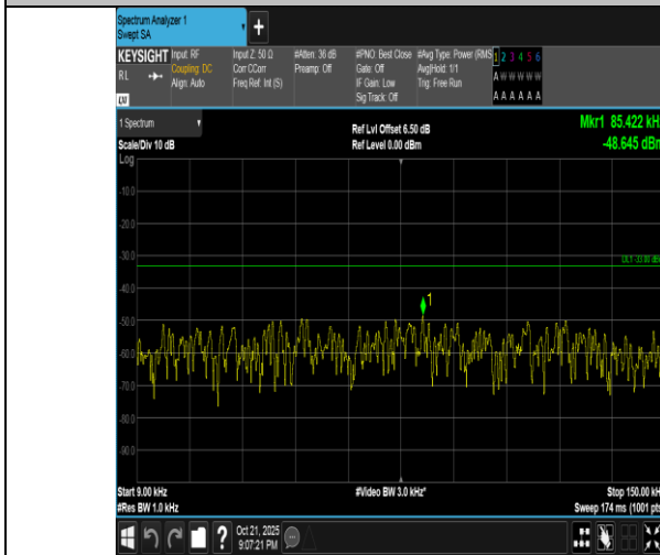
Band5-5MHz-QPSK-20425-25RB#0-0.009~0.15-PASS
