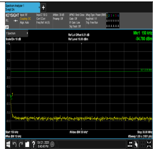
Band5-3MHz-16QAM-20635-1RB#14-0.15~30-PASS
