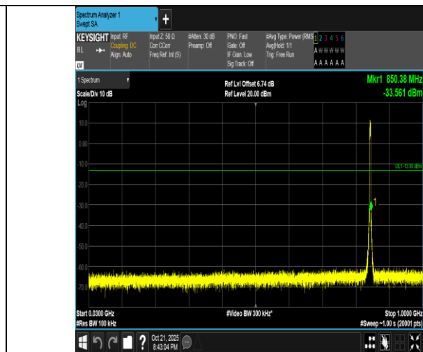
Band5-3MHz-16QAM-20635-15RB#0-30~1000-PASS
