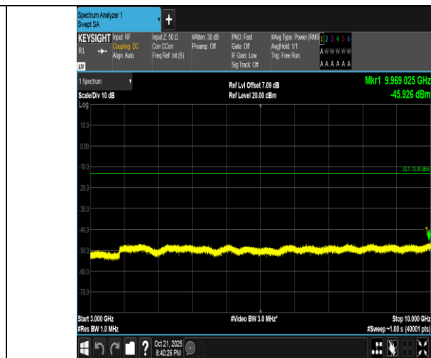
Band5-3MHz-QPSK-20635-1RB#14-3000~10000-PASS
