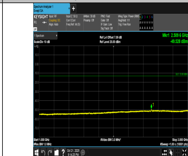
Band5-5MHz-QPSK-20525-25RB#0-1000~3000-PASS
