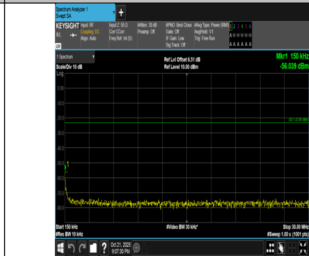
Band5-5MHz-QPSK-20425-25RB#0-0.15~30-PASS
