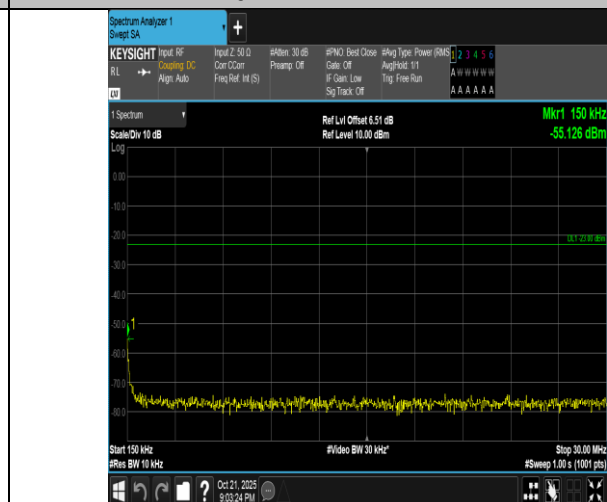
Band5-5MHz-QPSK-20425-1RB#0-0.15~30-PASS
