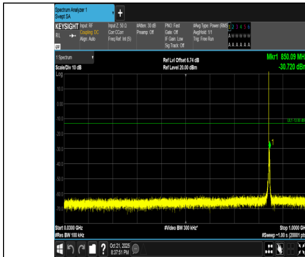
Band5-3MHz-QPSK-20635-1RB#0-30~1000-PASS
