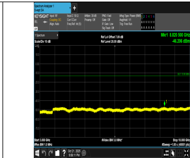
Band5-5MHz-QPSK-20425-1RB#24-3000~10000-PASS
