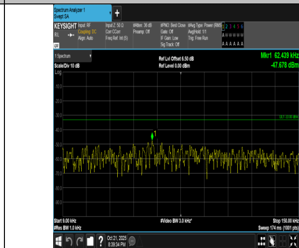
Band5-3MHz-QPSK-20635-1RB#14-0.009~0.15-PASS
