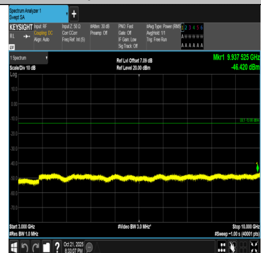
Band5-3MHz-16QAM-20525-1RB#0-3000~10000-PASS
