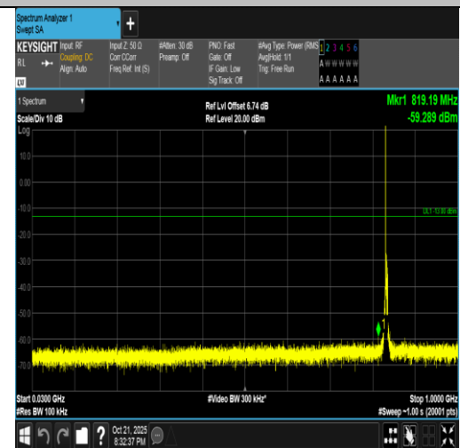
Band5-3MHz-16QAM-20525-1RB#0-30~1000-PASS
