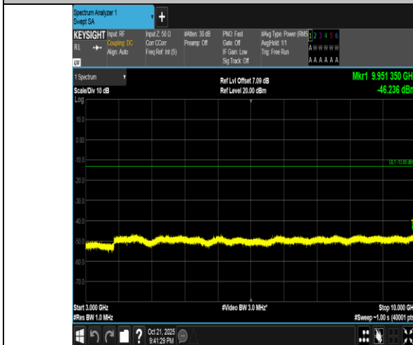
Band5-10MHz-16QAM-20450-1RB#49-3000~10000-PASS
