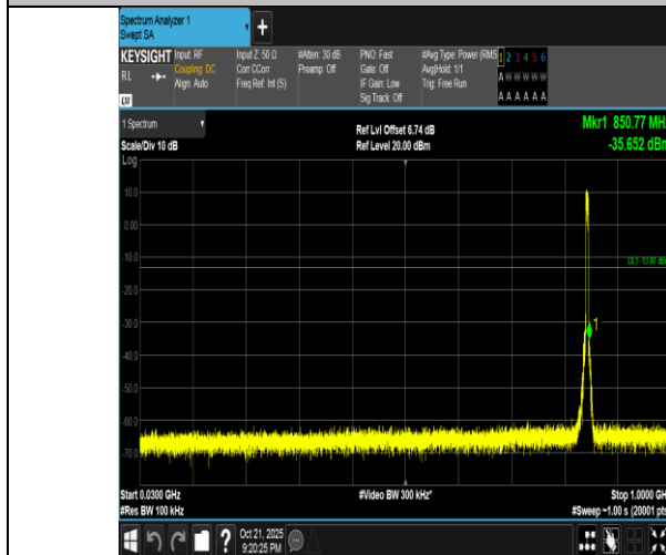
Band5-5MHz-QPSK-20625-25RB#0-30~1000-PASS
