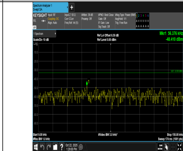
Band5-10MHz-16QAM-20450-50RB#0-0.009~0.15-PASS
