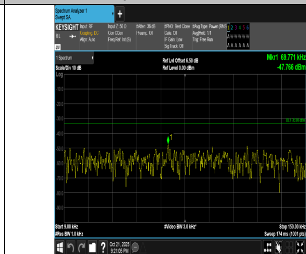
Band5-5MHz-16QAM-20625-25RB#0-0.009~0.15-PASS
