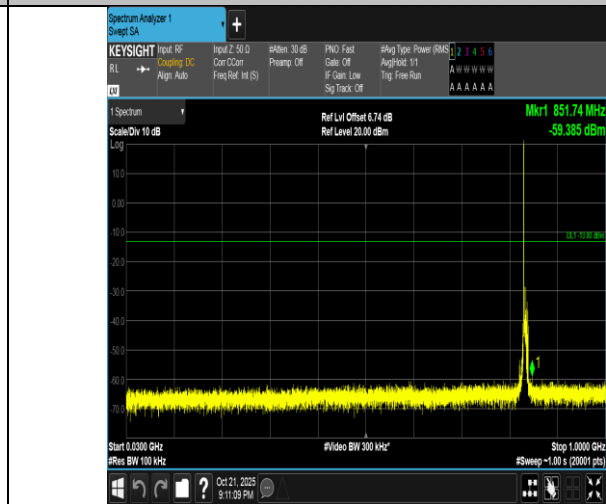
Band5-5MHz-16QAM-20525-1RB#0-30~1000-PASS
