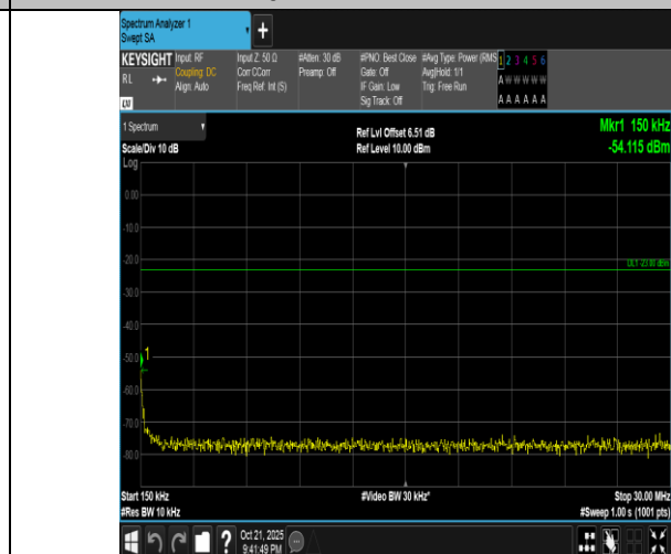
Band5-10MHz-QPSK-20525-1RB#0-0.15~30-PASS
