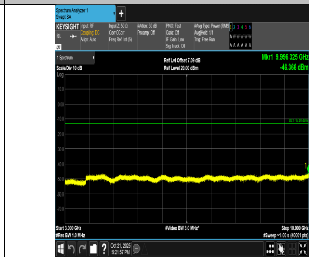
Band5-5MHz-16QAM-20625-25RB#0-3000~10000-PASS
