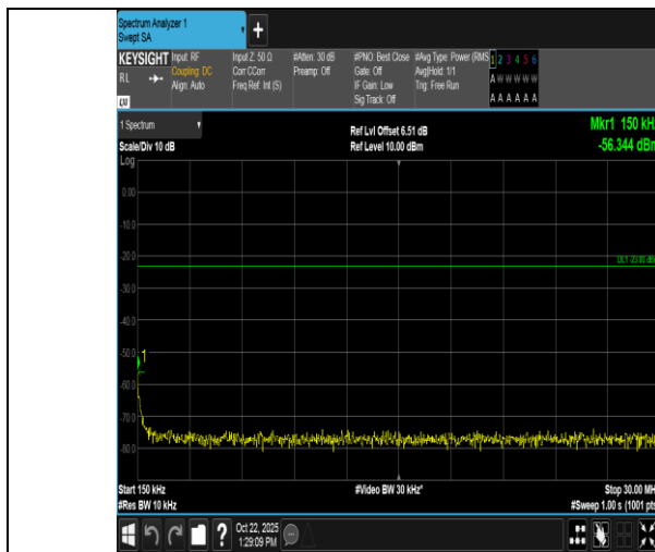
Band5-10MHz-16QAM-20450-50RB#0-0.15~30-PASS
