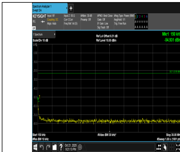
Band5-5MHz-16QAM-20625-25RB#0-0.15~30-PASS
