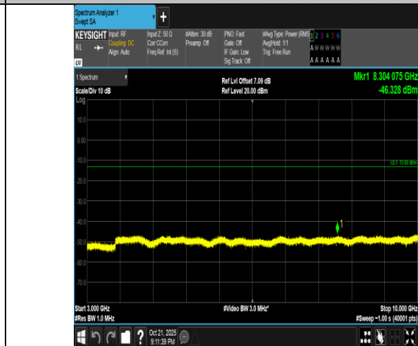
Band5-5MHz-16QAM-20525-1RB#0-3000~10000-PASS
