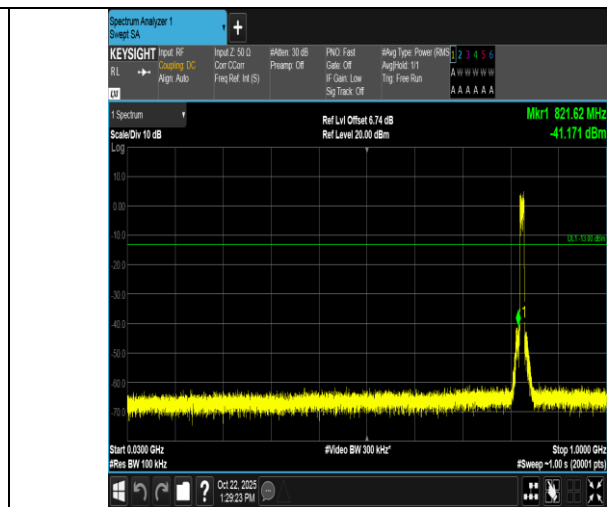
Band5-10MHz-16QAM-20450-50RB#0-30~1000-PASS
