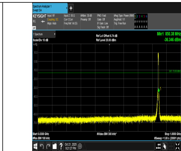
Band5-5MHz-16QAM-20625-25RB#0-30~1000-PASS
