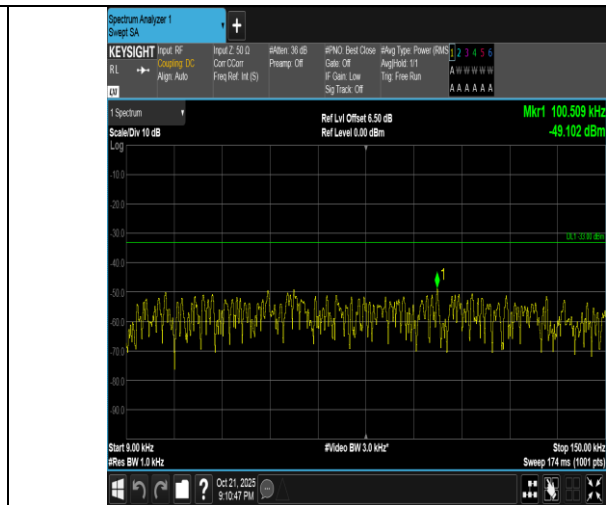
Band5-5MHz-16QAM-20525-1RB#0-0.009~0.15-PASS
