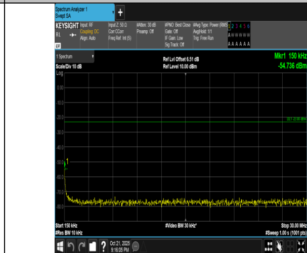
Band5-5MHz-QPSK-20625-1RB#0-0.15~30-PASS
