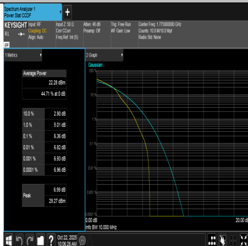
Band66-10MHz-16QAM-132622-1RB#0-PASS
