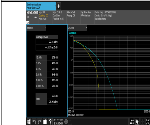
Band66-5MHz-16QAM-132647-1RB#0-PASS
