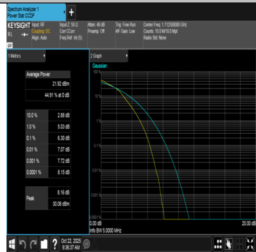
Band66-5MHz-16QAM-131997-25RB#0-PASS
