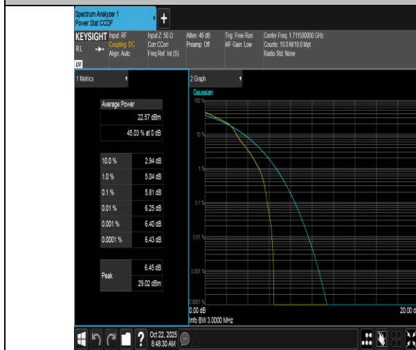
Band66-3MHz-16QAM-131987-1RB#0-PASS
