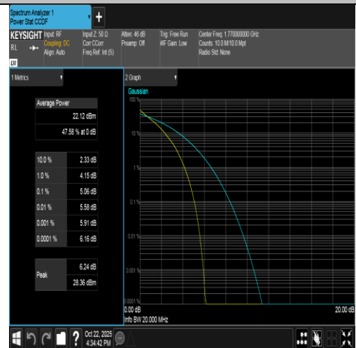
Band66-20MHz-QPSK-132572-100RB#0-PASS
