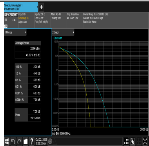
Band66-5MHz-QPSK-132647-25RB#0-PASS
