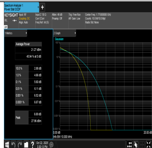
Band66-10MHz-16QAM-132622-50RB#0-PASS
