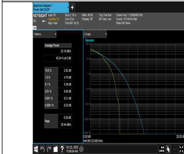
Band66-20MHz-16QAM-132072-1RB#0-PASS
