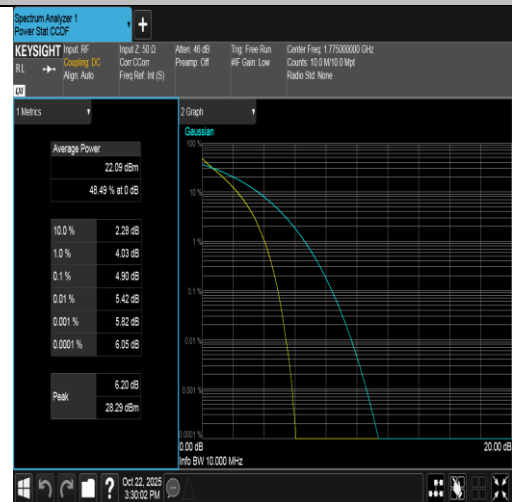
Band66-10MHz-QPSK-132622-50RB#0-PASS
