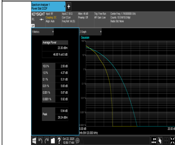
Band66-20MHz-QPSK-132322-1RB#0-PASS
