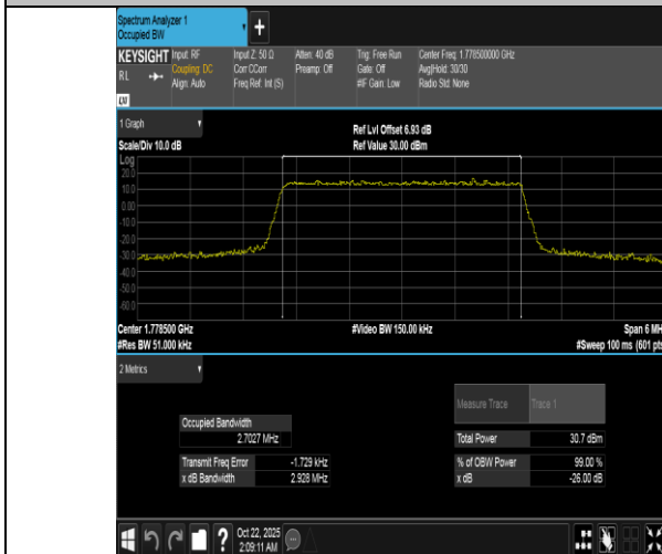
Band66-3MHz-QPSK-132657-15RB#0-PASS
