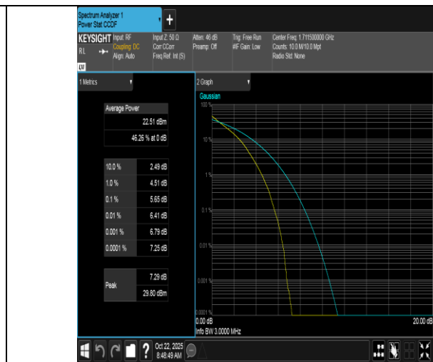
Band66-3MHz-QPSK-131987-15RB#0-PASS
