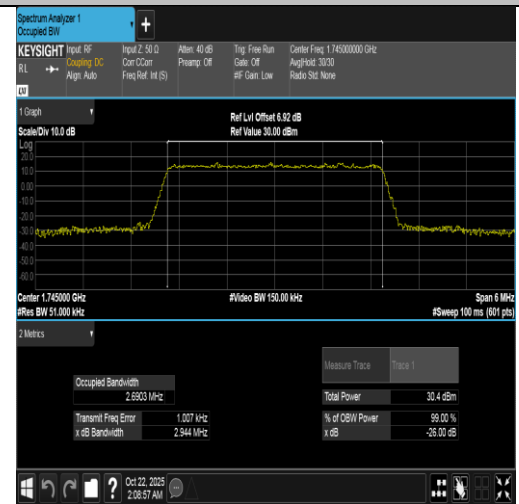
Band66-3MHz-16QAM-132322-15RB#0-PASS
