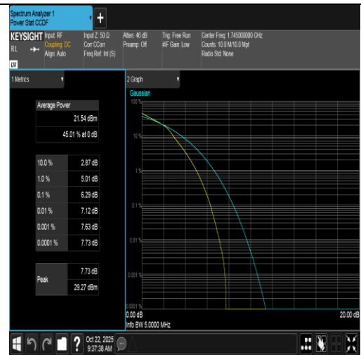
Band66-5MHz-16QAM-132322-25RB#0-PASS
