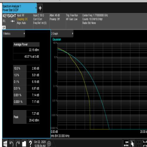
Band66-20MHz-16QAM-132572-1RB#0-PASS
