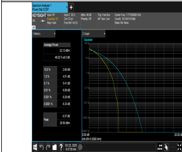
Band66-5MHz-QPSK-132647-1RB#0-PASS
