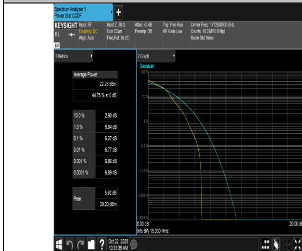
Band66-15MHz-16QAM-132597-1RB#0-PASS
