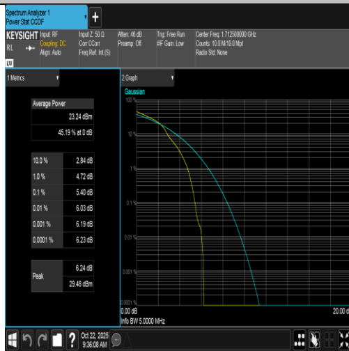
Band66-5MHz-16QAM-131997-1RB#0-PASS
