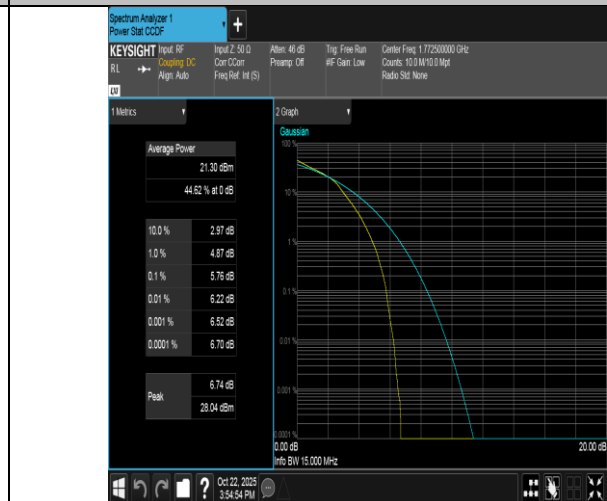
Band66-15MHz-16QAM-132597-75RB#0-PASS
