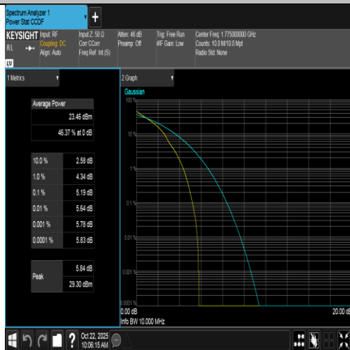
Band66-10MHz-QPSK-132622-1RB#0-PASS
