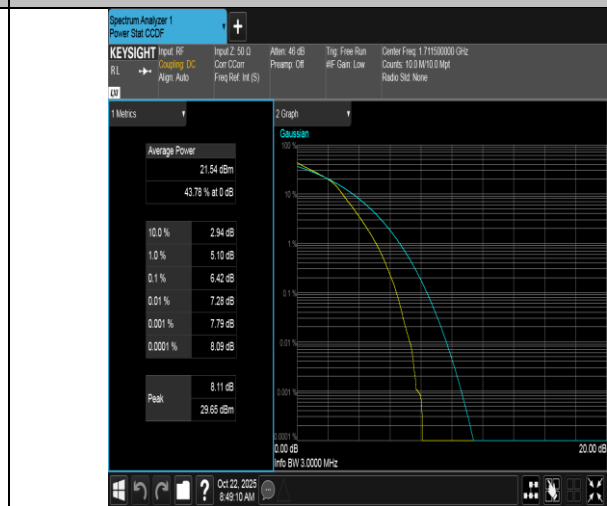
Band66-3MHz-16QAM-131987-15RB#0-PASS
