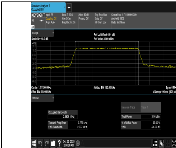
Band66-3MHz-QPSK-131987-15RB#0-PASS
