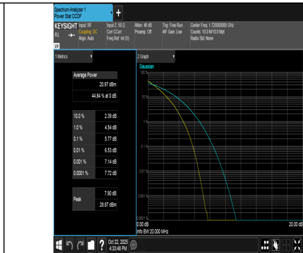
Band66-20MHz-QPSK-132072-100RB#0-PASS
