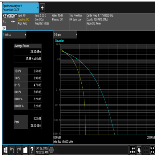
Band66-15MHz-QPSK-132047-1RB#0-PASS
