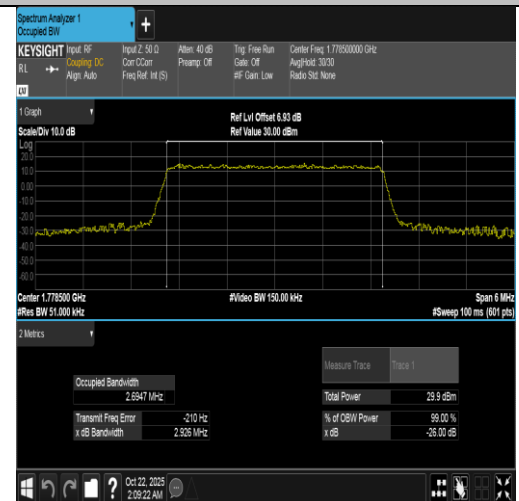
Band66-3MHz-16QAM-132657-15RB#0-PASS
