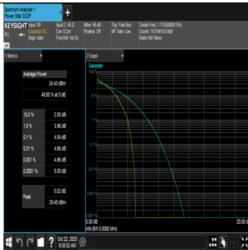
Band66-5MHz-QPSK-131997-1RB#0-PASS
