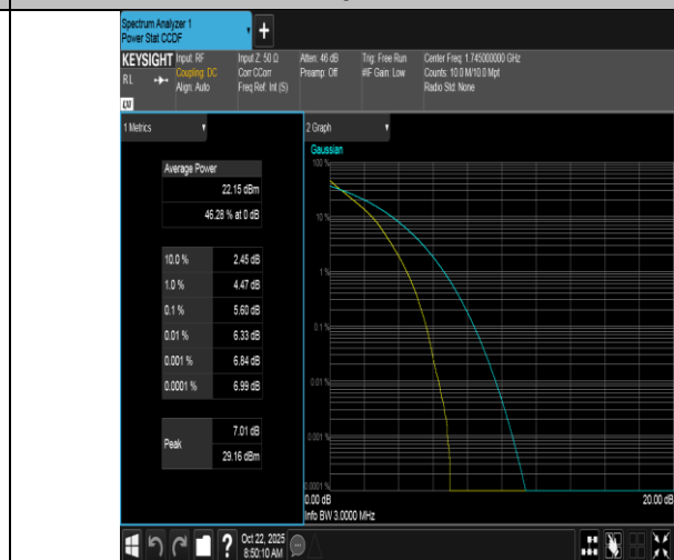
Band66-3MHz-QPSK-132322-15RB#0-PASS
