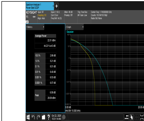
Band66-15MHz-16QAM-132322-1RB#0-PASS
