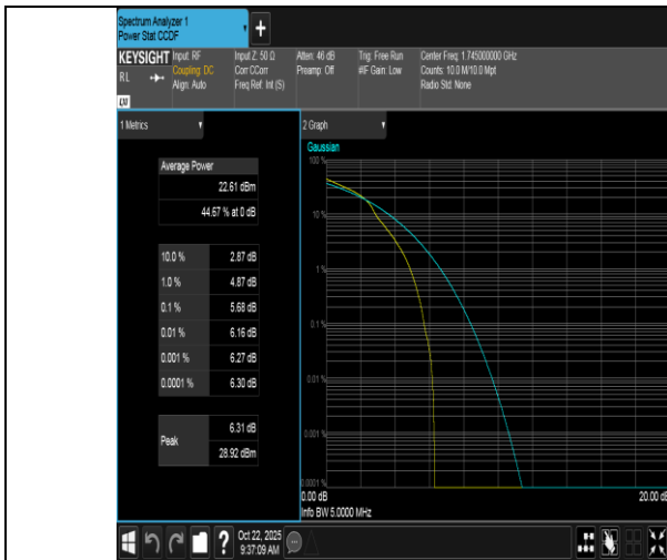
Band66-5MHz-16QAM-132322-1RB#0-PASS
