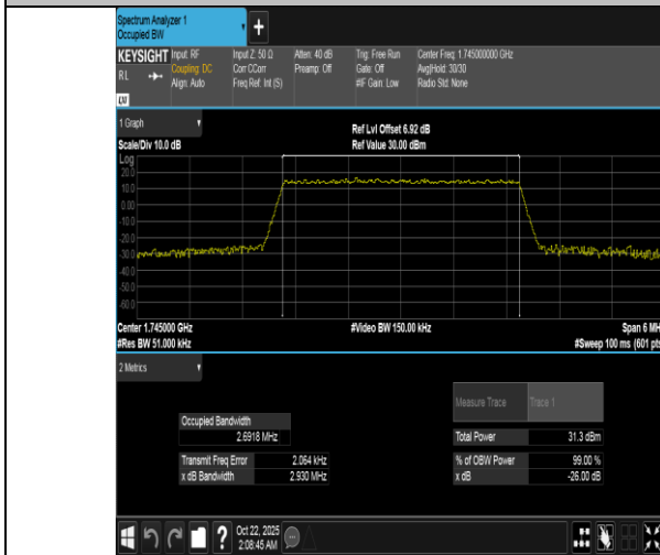
Band66-3MHz-QPSK-132322-15RB#0-PASS
