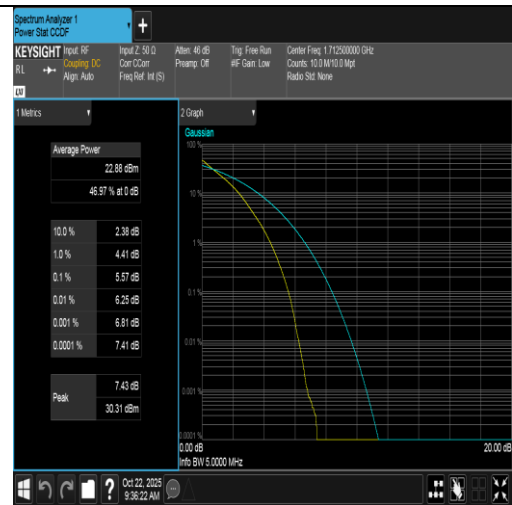
Band66-5MHz-QPSK-131997-25RB#0-PASS
