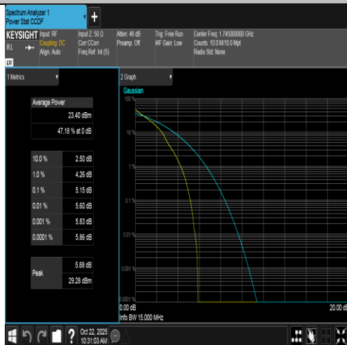
Band66-15MHz-QPSK-132322-1RB#0-PASS
