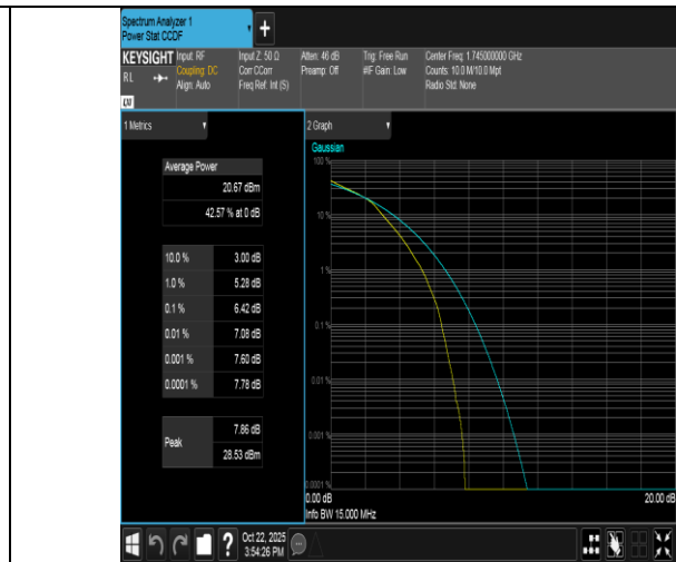
Band66-15MHz-16QAM-132322-75RB#0-PASS
