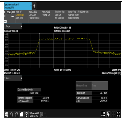
Band66-3MHz-16QAM-131987-15RB#0-PASS
