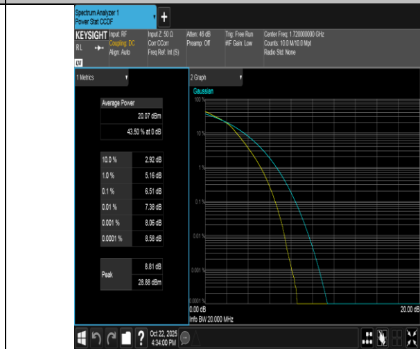
Band66-20MHz-16QAM-132072-100RB#0-PASS
