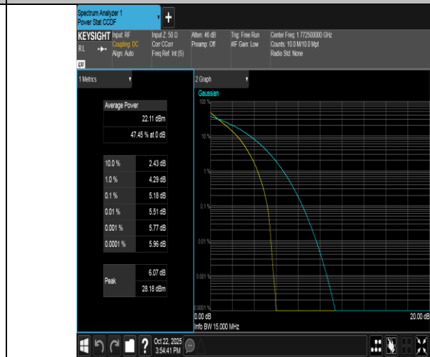
Band66-15MHz-QPSK-132597-75RB#0-PASS
