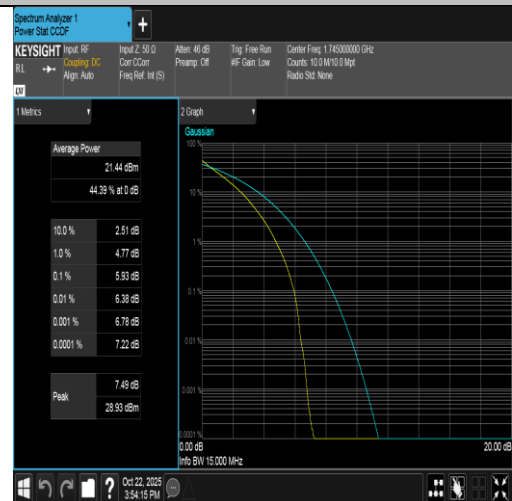
Band66-15MHz-QPSK-132322-75RB#0-PASS
