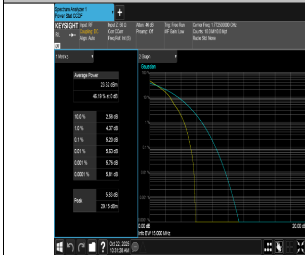
Band66-15MHz-QPSK-132597-1RB#0-PASS
