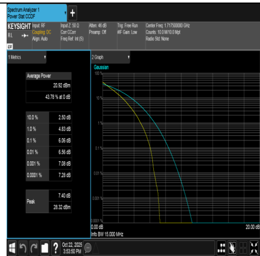
Band66-15MHz-QPSK-132047-75RB#0-PASS
