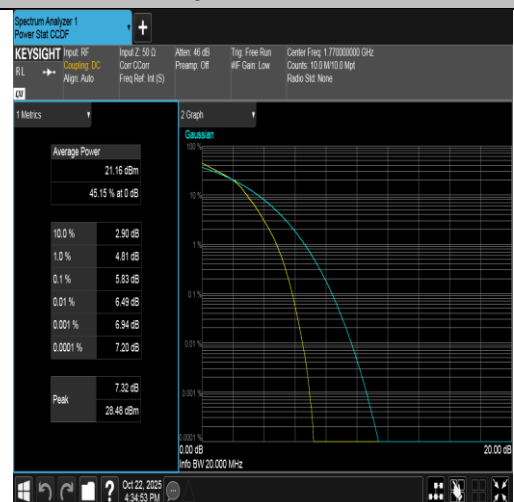
Band66-20MHz-16QAM-132572-100RB#0-PASS
