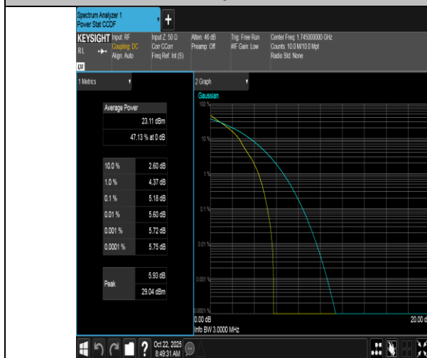
Band66-3MHz-QPSK-132322-1RB#0-PASS
