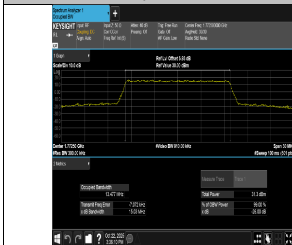
Band66-15MHz-QPSK-132597-75RB#0-PASS
