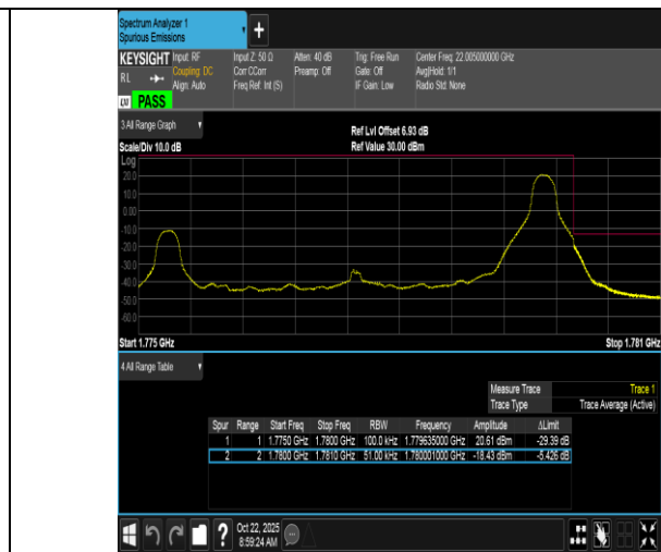
Band66-5MHz-QPSK-132647-1RB#24-PASS
