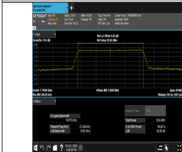
Band66-20MHz-QPSK-132322-100RB#0-PASS
