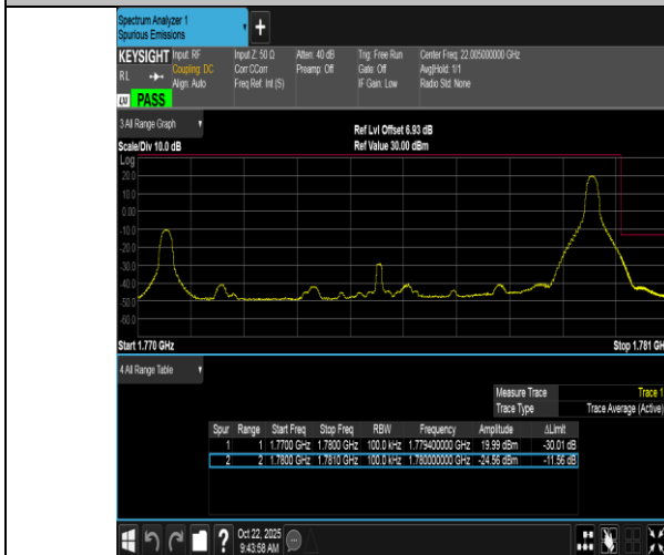
Band66-10MHz-16QAM-132622-1RB#49-PASS
