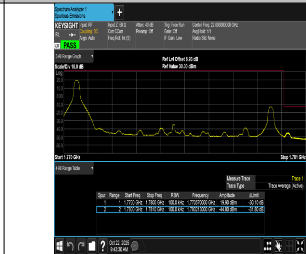
Band66-10MHz-16QAM-132622-1RB#0-PASS
