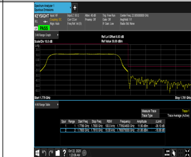
Band66-1.4MHz-16QAM-132665-6RB#0-PASS
