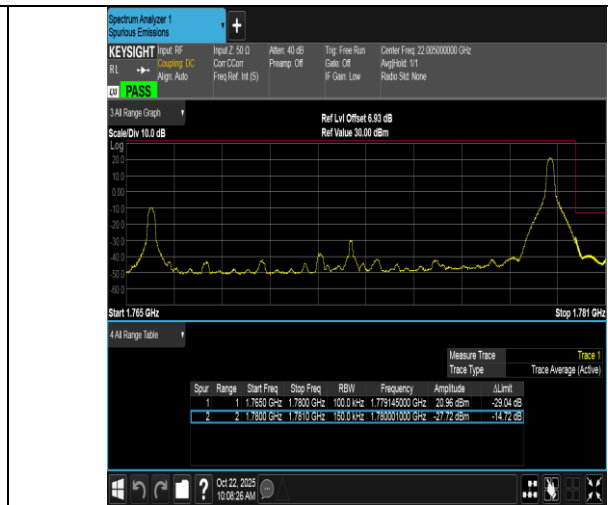
Band66-15MHz-QPSK-132597-1RB#74-PASS
