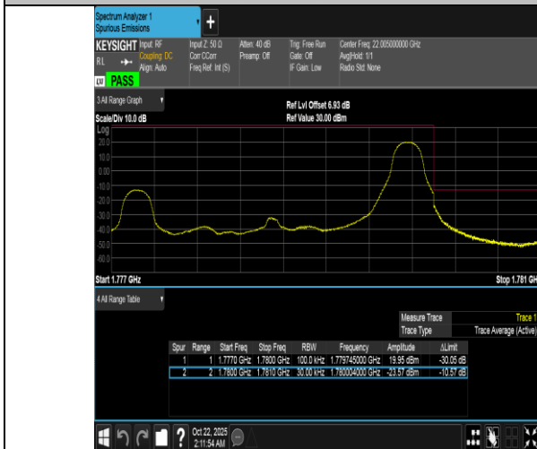
Band66-3MHz-16QAM-132657-1RB#14-PASS
