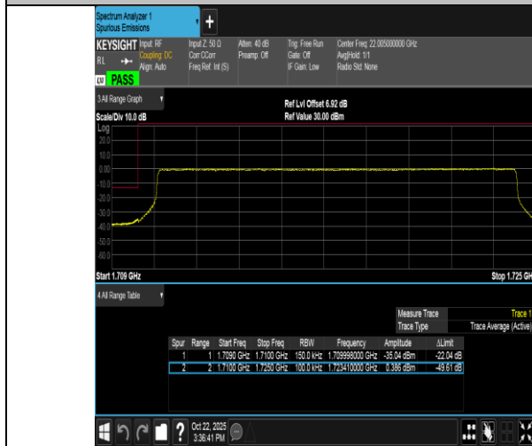
Band66-15MHz-QPSK-132047-75RB#0-PASS
