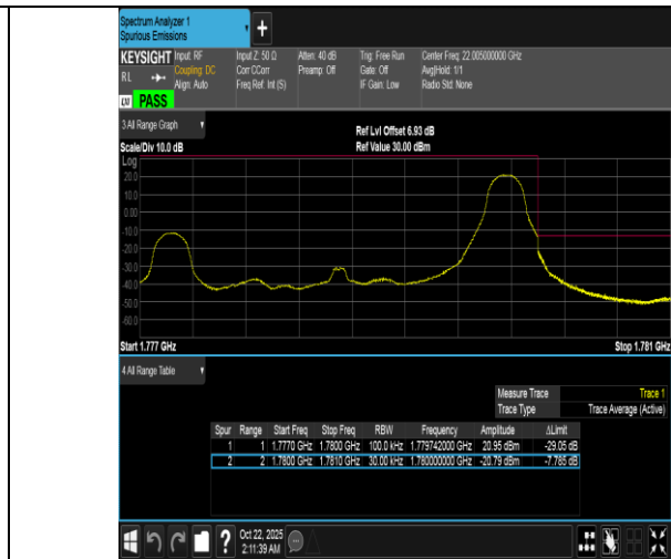
Band66-3MHz-QPSK-132657-1RB#14-PASS
