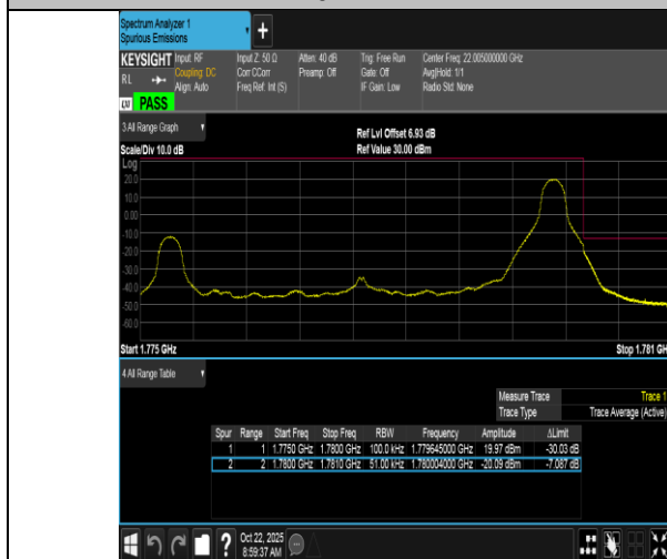
Band66-5MHz-16QAM-132647-1RB#24-PASS
