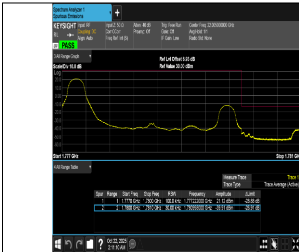
Band66-3MHz-QPSK-132657-1RB#0-PASS
