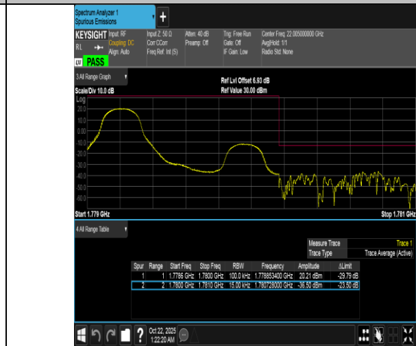
Band66-1.4MHz-16QAM-132665-1RB#0-PASS
