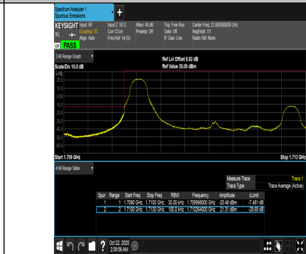
Band66-3MHz-16QAM-131987-1RB#0-PASS
