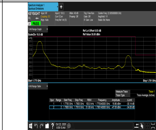
Band66-5MHz-16QAM-132647-1RB#0-PASS
