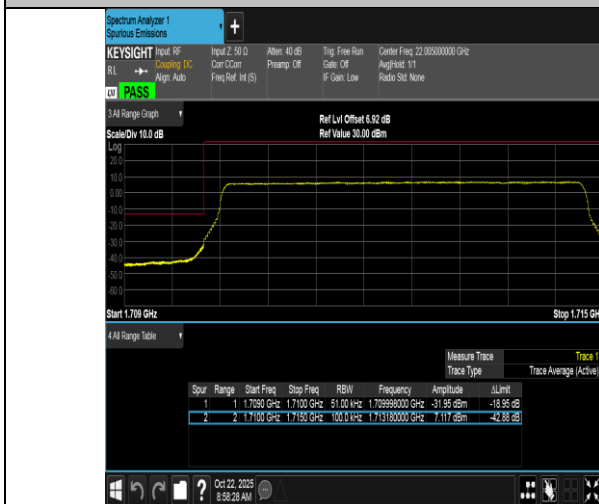
Band66-5MHz-QPSK-131997-25RB#0-PASS
