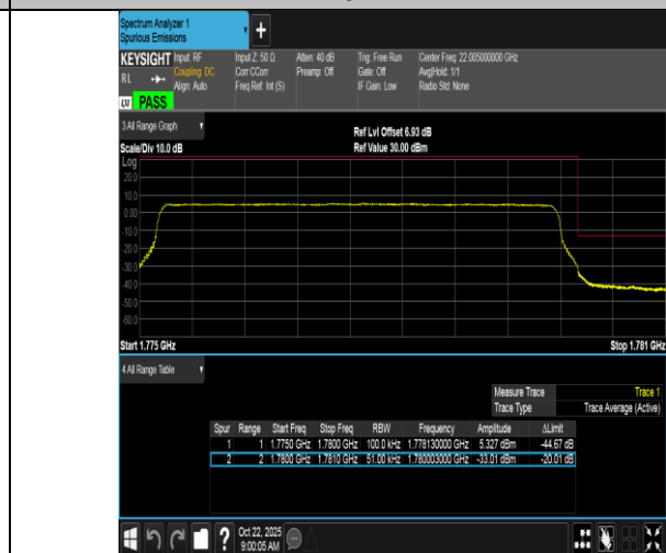
Band66-5MHz-16QAM-132647-25RB#0-PASS
