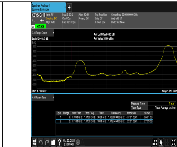
Band66-3MHz-QPSK-131987-1RB#14-PASS
