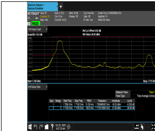
Band66-5MHz-QPSK-131997-1RB#0-PASS
