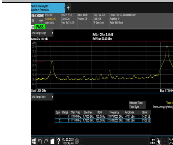
Band66-15MHz-16QAM-132047-1RB#74-PASS
