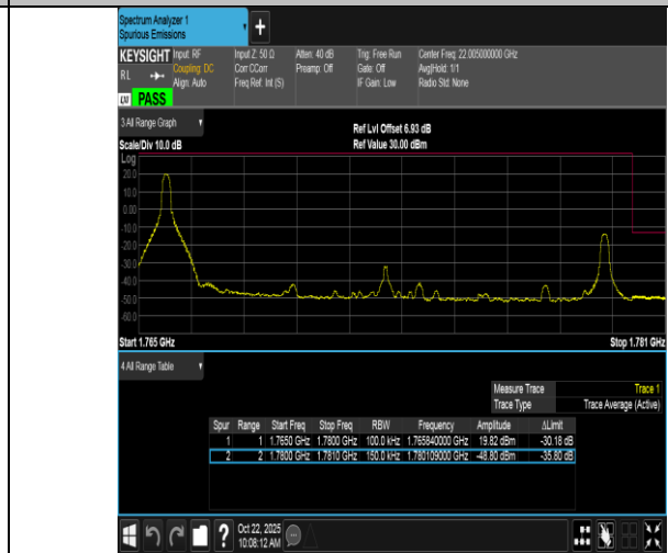
Band66-15MHz-16QAM-132597-1RB#0-PASS
