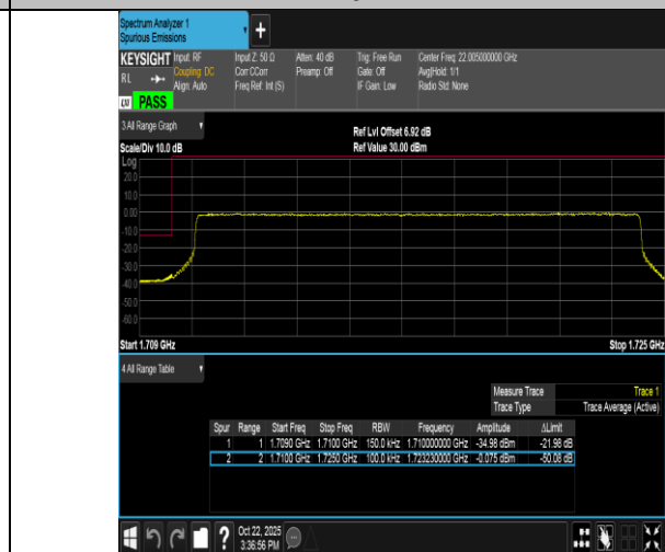
Band66-15MHz-16QAM-132047-75RB#0-PASS
