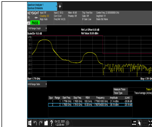
Band66-1.4MHz-QPSK-132665-1RB#0-PASS
