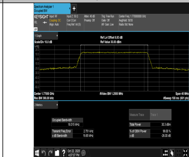
Band66-20MHz-16QAM-132572-100RB#0-PASS
