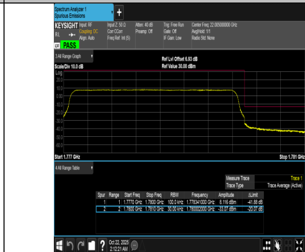
Band66-3MHz-16QAM-132657-15RB#0-PASS
