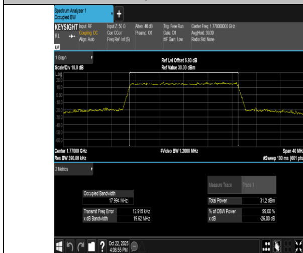
Band66-20MHz-QPSK-132572-100RB#0-PASS
