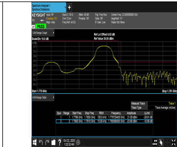
Band66-1.4MHz-QPSK-132665-1RB#5-PASS
