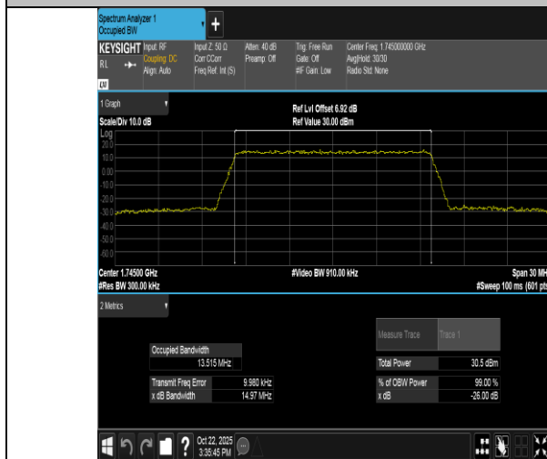
Band66-15MHz-QPSK-132322-75RB#0-PASS
