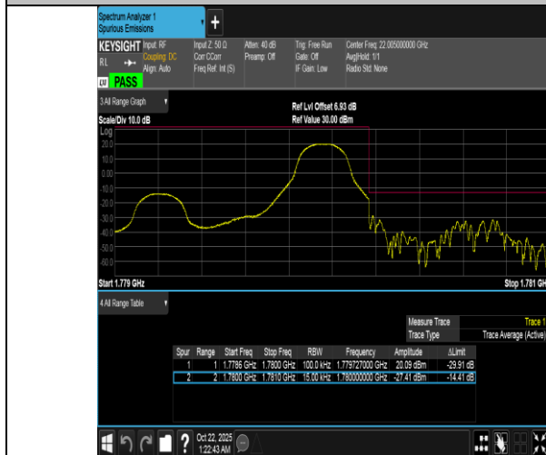
Band66-1.4MHz-16QAM-132665-1RB#5-PASS
