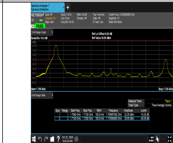
Band66-10MHz-16QAM-132022-1RB#0-PASS
