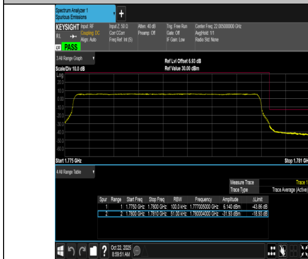
Band66-5MHz-QPSK-132647-25RB#0-PASS
