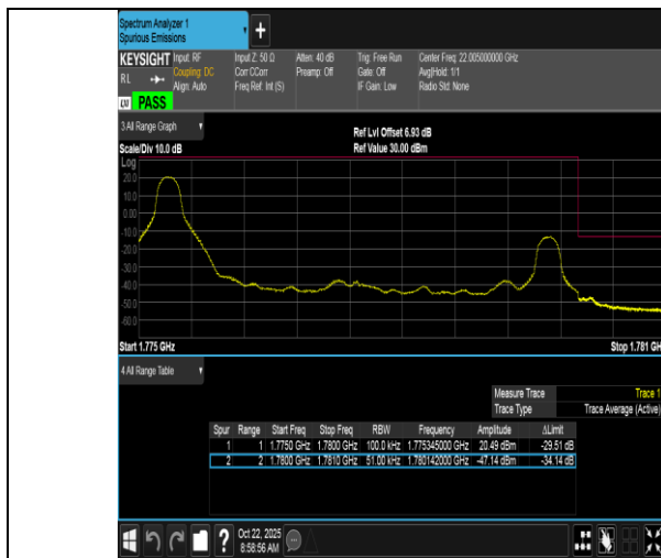
Band66-5MHz-QPSK-132647-1RB#0-PASS
