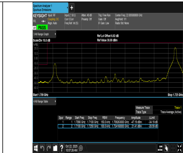
Band66-15MHz-QPSK-132047-1RB#74-PASS
