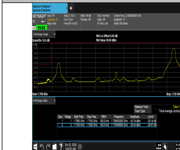
Band66-10MHz-16QAM-132022-1RB#49-PASS
