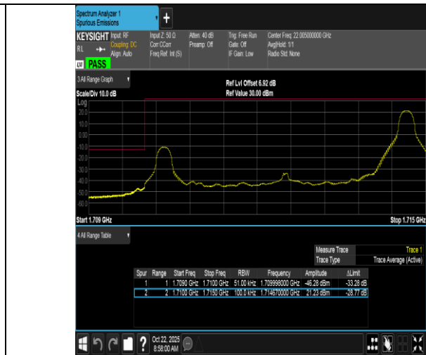
Band66-5MHz-QPSK-131997-1RB#24-PASS
