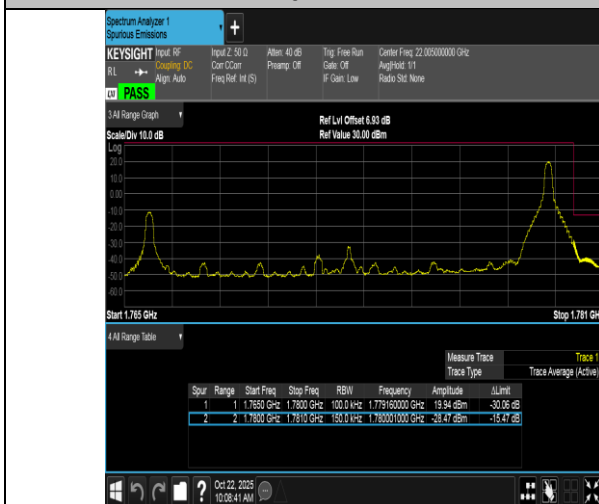
Band66-15MHz-16QAM-132597-1RB#74-PASS
