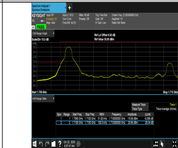
Band66-5MHz-16QAM-131997-1RB#0-PASS
