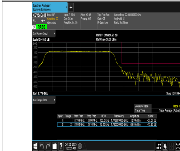
Band66-1.4MHz-QPSK-132665-6RB#0-PASS
