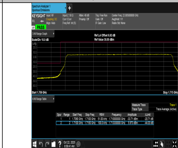
Band66-5MHz-16QAM-131997-25RB#0-PASS
