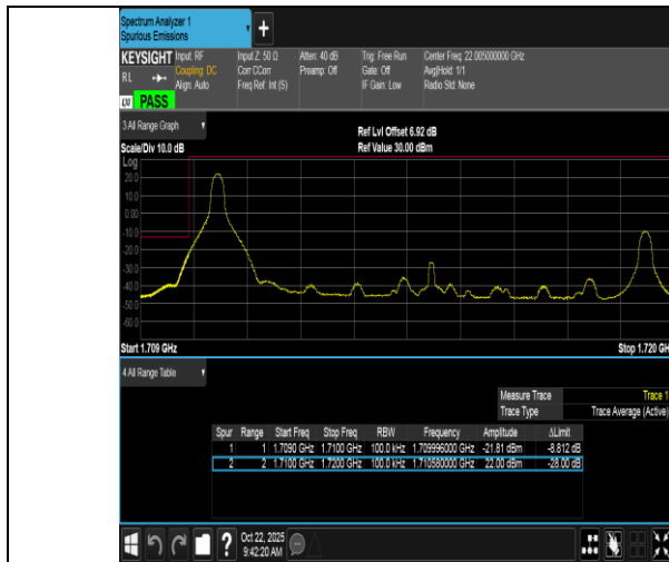
Band66-10MHz-QPSK-132022-1RB#0-PASS
