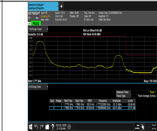
Band66-3MHz-16QAM-132657-1RB#0-PASS
