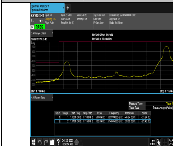
Band66-5MHz-16QAM-131997-1RB#24-PASS
