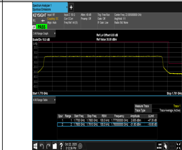
Band66-10MHz-16QAM-132622-50RB#0-PASS
