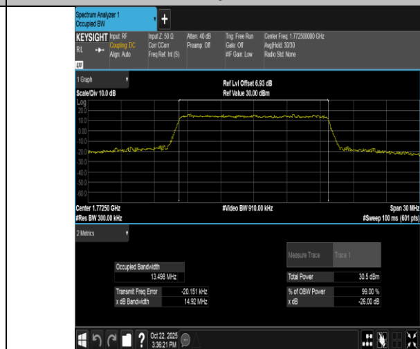
Band66-15MHz-16QAM-132597-75RB#0-PASS
