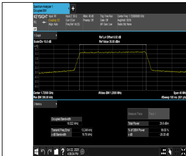
Band66-20MHz-QPSK-132072-100RB#0-PASS
