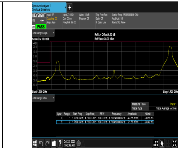
Band66-10MHz-QPSK-132022-1RB#49-PASS
