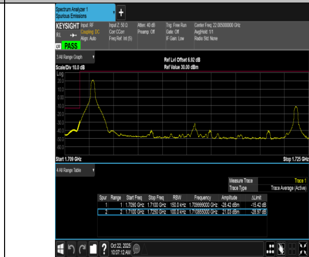
Band66-15MHz-16QAM-132047-1RB#0-PASS
