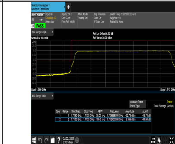
Band66-3MHz-16QAM-131987-15RB#0-PASS
