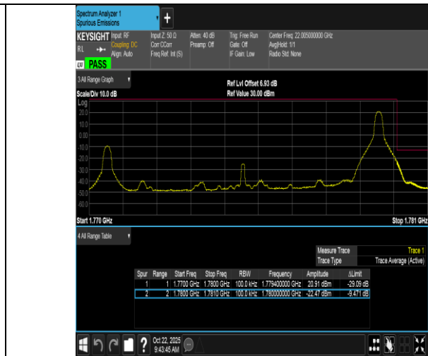
Band66-10MHz-QPSK-132622-1RB#49-PASS
