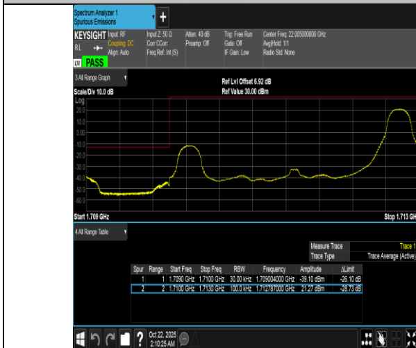
Band66-3MHz-16QAM-131987-1RB#14-PASS
