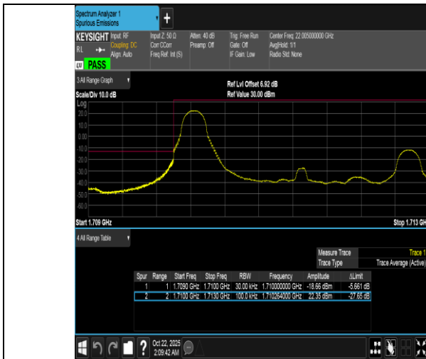
Band66-3MHz-QPSK-131987-1RB#0-PASS
