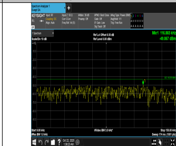
Band66-1.4MHz-QPSK-132665-1RB#5-0.009~0.15-PASS
