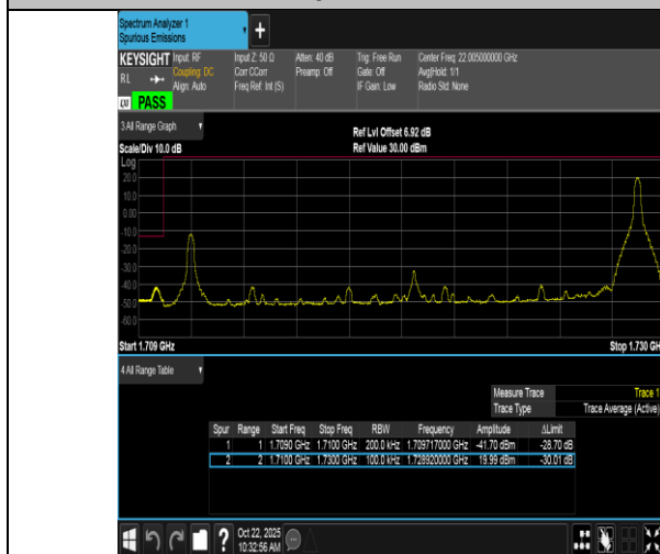
Band66-20MHz-16QAM-132072-1RB#99-PASS
