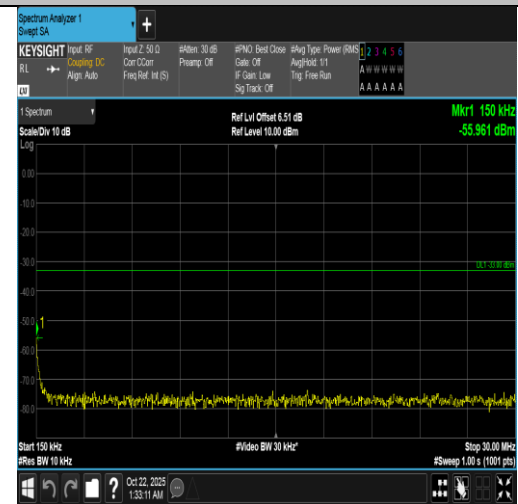
Band66-1.4MHz-16QAM-132322-1RB#5-0.15~30-PASS
