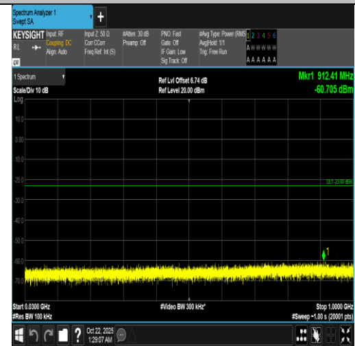
Band66-1.4MHz-16QAM-131979-6RB#0-30~1000-PASS
