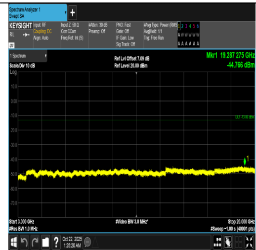
Band66-1.4MHz-16QAM-131979-1RB#0-3000~20000-PASS
