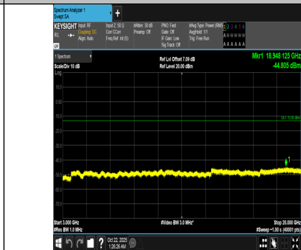
Band66-1.4MHz-QPSK-131979-1RB#5-3000~20000-PASS
