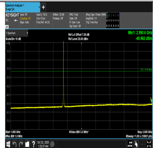
Band66-1.4MHz-16QAM-132322-1RB#5-1000~3000-PASS
