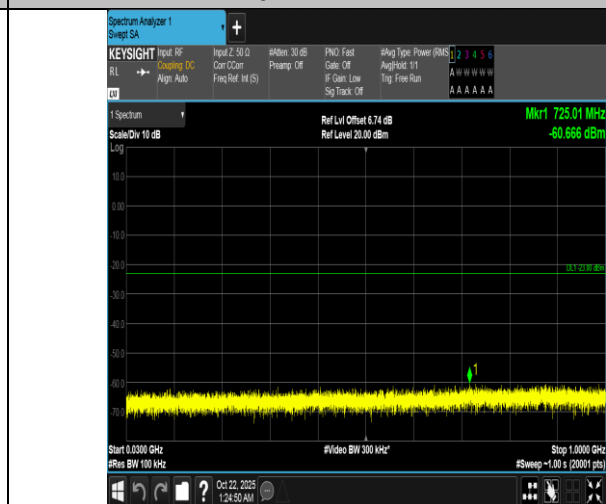
Band66-1.4MHz-16QAM-131979-1RB#0-30~1000-PASS
