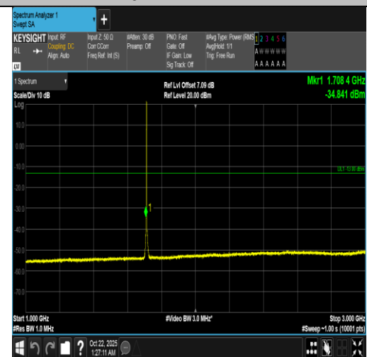
Band66-1.4MHz-16QAM-131979-1RB#5-1000~3000-PASS
