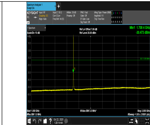
Band66-1.4MHz-QPSK-131979-6RB#0-1000~3000-PASS
