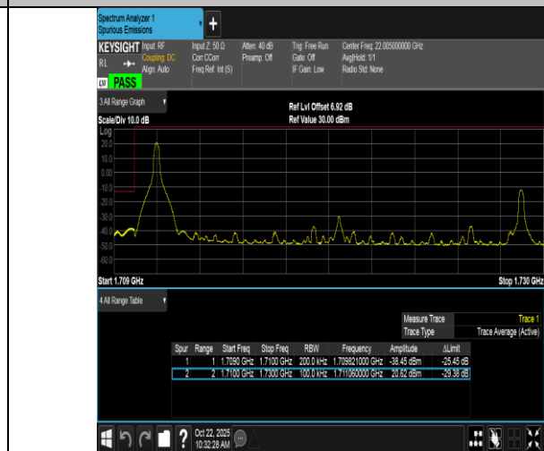
Band66-20MHz-16QAM-132072-1RB#0-PASS
