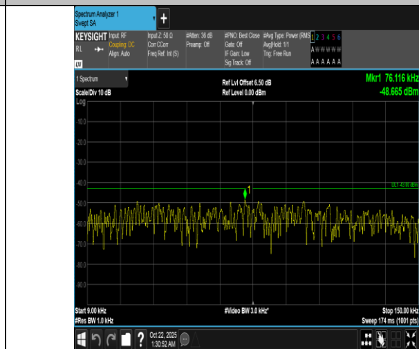
Band66-1.4MHz-16QAM-132322-1RB#0-0.009~0.15-PASS
