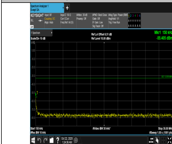
Band66-1.4MHz-16QAM-131979-1RB#0-0.15~30-PASS
