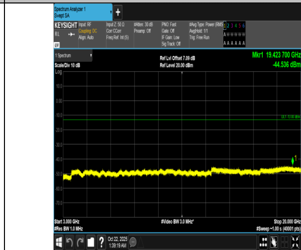
Band66-1.4MHz-QPSK-132665-1RB#5-3000~20000-PASS
