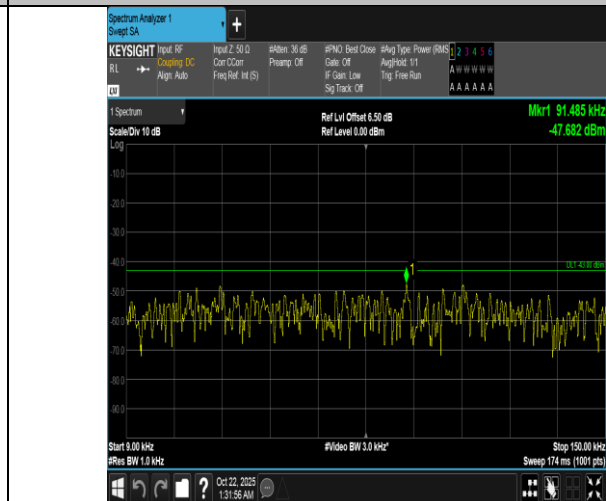
Band66-1.4MHz-QPSK-132322-1RB#5-0.009~0.15-PASS
