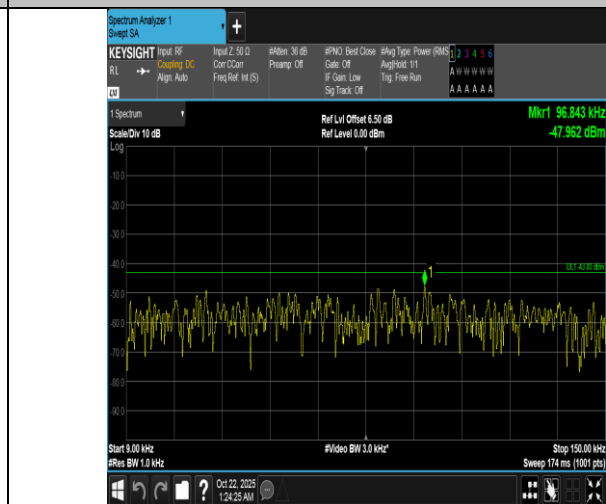
Band66-1.4MHz-16QAM-131979-1RB#0-0.009~0.15-PASS
