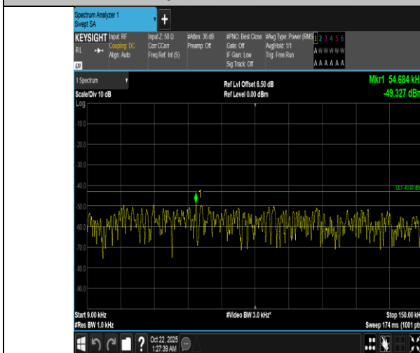
Band66-1.4MHz-QPSK-131979-6RB#0-0.009~0.15-PASS
