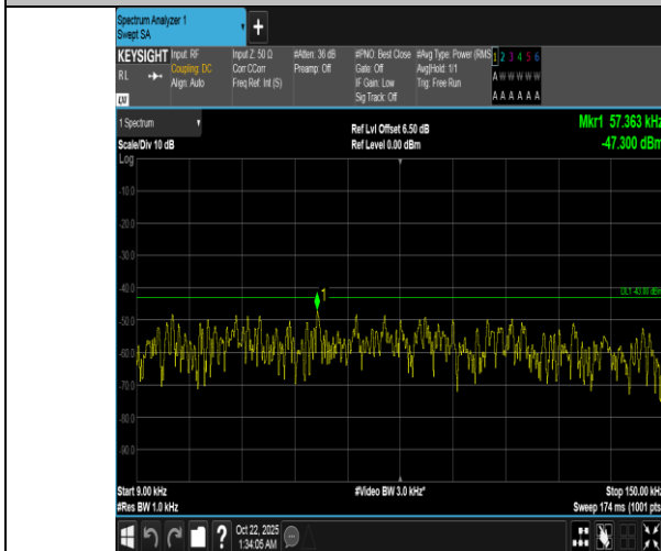
Band66-1.4MHz-QPSK-132322-6RB#0-0.009~0.15-PASS
