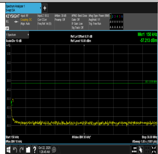
Band66-1.4MHz-16QAM-131979-1RB#5-0.15~30-PASS
