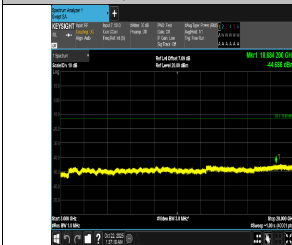
Band66-1.4MHz-QPSK-132665-1RB#0-3000~20000-PASS
