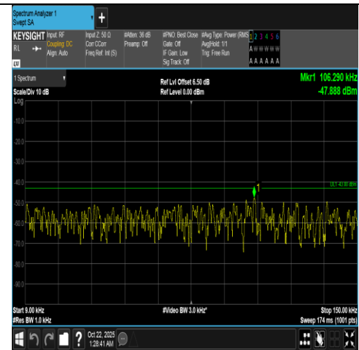
Band66-1.4MHz-16QAM-131979-6RB#0-0.009~0.15-PASS
