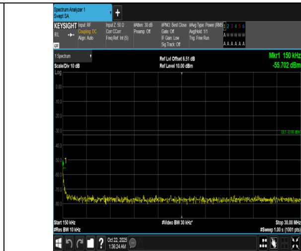
Band66-1.4MHz-QPSK-132665-1RB#0-0.15~30-PASS
