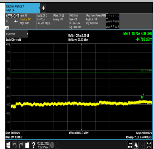
Band66-1.4MHz-16QAM-131979-6RB#0-3000~20000-PASS
