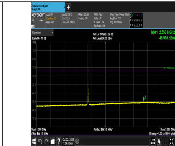
Band66-1.4MHz-QPSK-132322-6RB#0-1000~3000-PASS
