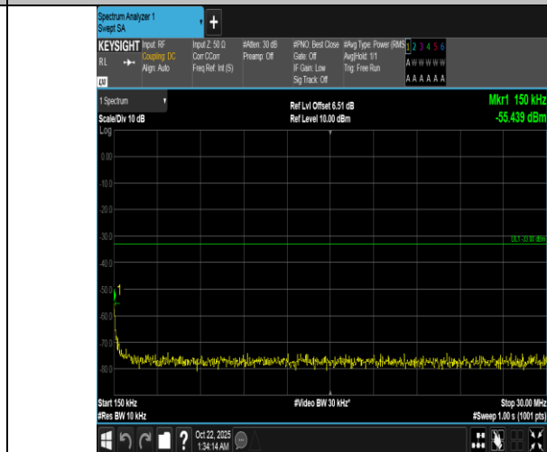
Band66-1.4MHz-QPSK-132322-6RB#0-0.15~30-PASS
