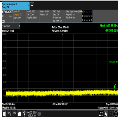
Band66-1.4MHz-16QAM-132322-1RB#5-30~1000-PASS
