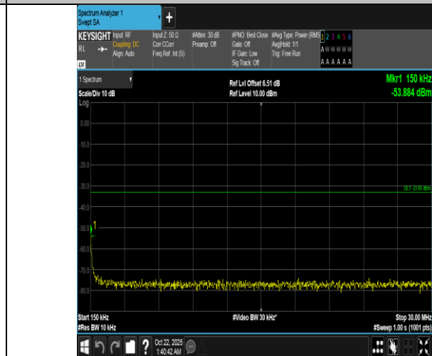
Band66-1.4MHz-QPSK-132665-6RB#0-0.15~30-PASS
