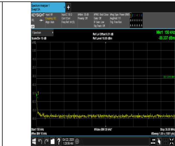
Band66-1.4MHz-QPSK-132322-1RB#0-0.15~30-PASS
