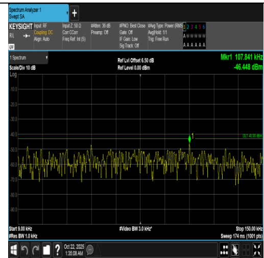
Band66-1.4MHz-16QAM-132322-6RB#0-0.009~0.15-PASS
