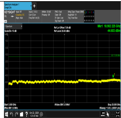
Band66-1.4MHz-16QAM-132322-1RB#0-3000~20000-PASS
