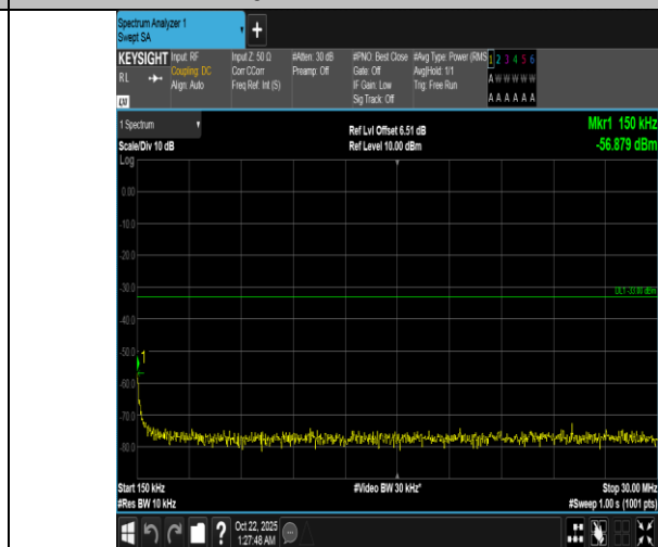
Band66-1.4MHz-QPSK-131979-6RB#0-0.15~30-PASS
