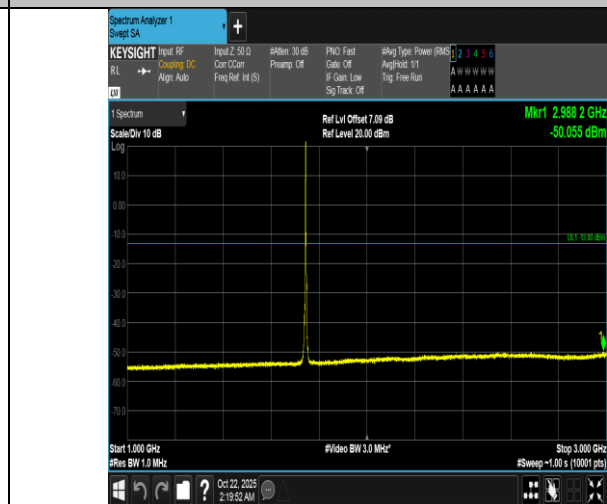
Band66-3MHz-QPSK-132322-1RB#0-1000~3000-PASS
