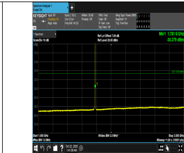
Band66-1.4MHz-QPSK-132665-6RB#0-1000~3000-PASS
