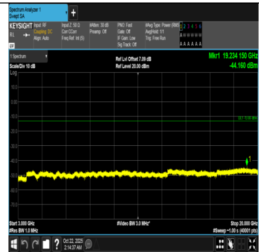
Band66-3MHz-16QAM-131987-1RB#0-3000~20000-PASS
