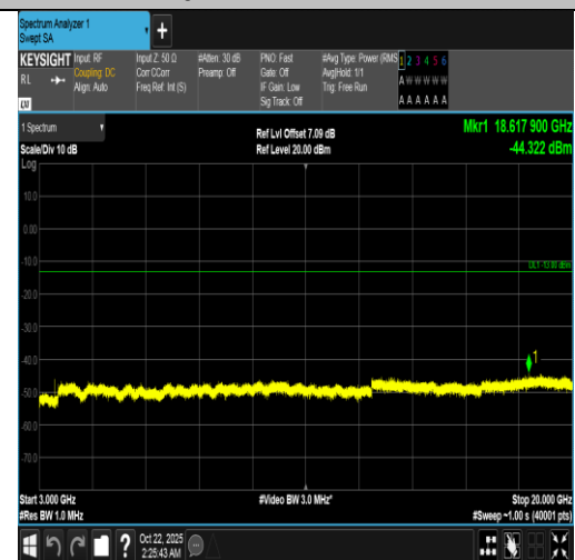
Band66-3MHz-16QAM-132322-15RB#0-3000~20000-PASS
