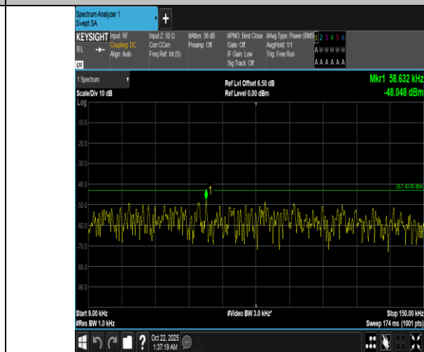
Band66-1.4MHz-16QAM-132665-1RB#0-0.009~0.15-PASS
