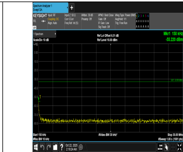
Band66-3MHz-QPSK-132322-1RB#0-0.15~30-PASS
