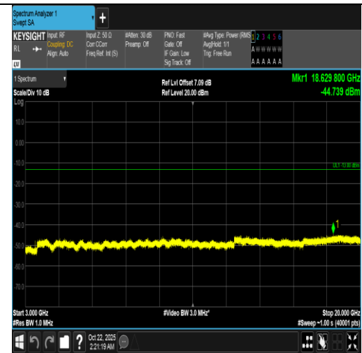
Band66-3MHz-16QAM-132322-1RB#0-3000~20000-PASS
