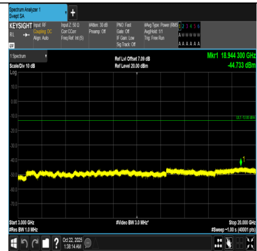
Band66-1.4MHz-16QAM-132665-1RB#0-3000~20000-PASS
