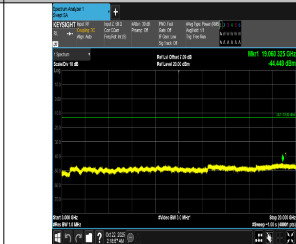
Band66-3MHz-16QAM-131987-15RB#0-3000~20000-PASS
