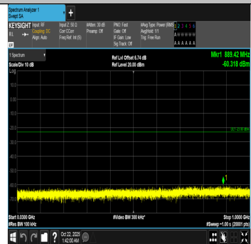
Band66-1.4MHz-16QAM-132665-6RB#0-30~1000-PASS
