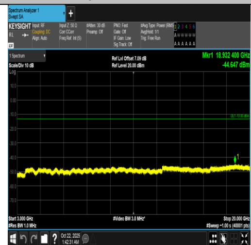
Band66-1.4MHz-16QAM-132665-6RB#0-3000~20000-PASS
