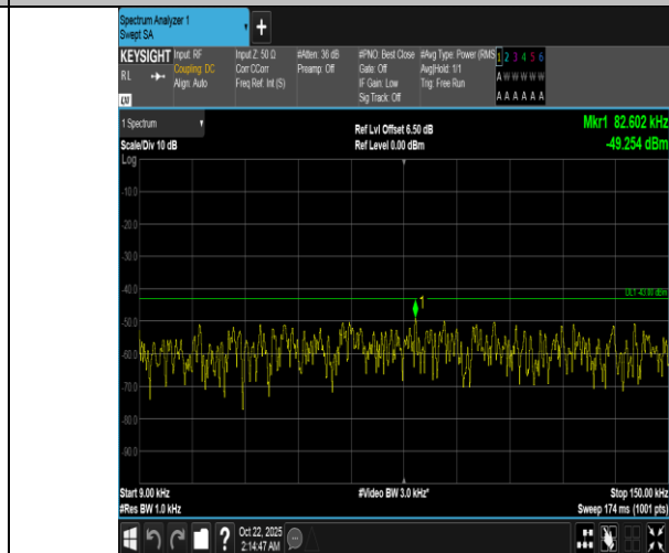
Band66-3MHz-QPSK-131987-1RB#14-0.009~0.15-PASS
