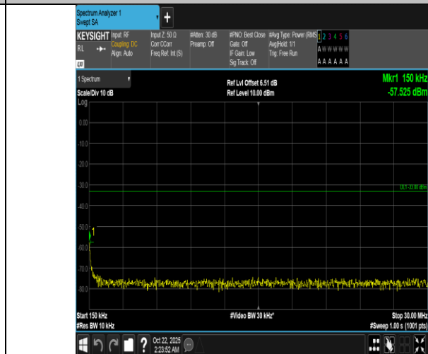
Band66-3MHz-QPSK-132322-15RB#0-0.15~30-PASS
