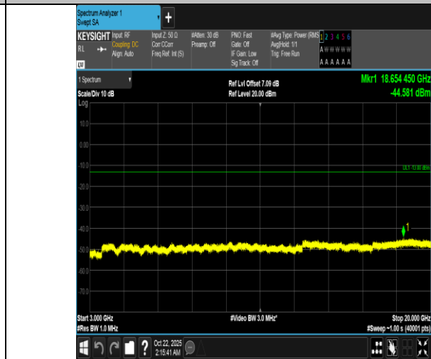
Band66-3MHz-QPSK-131987-1RB#14-3000~20000-PASS
