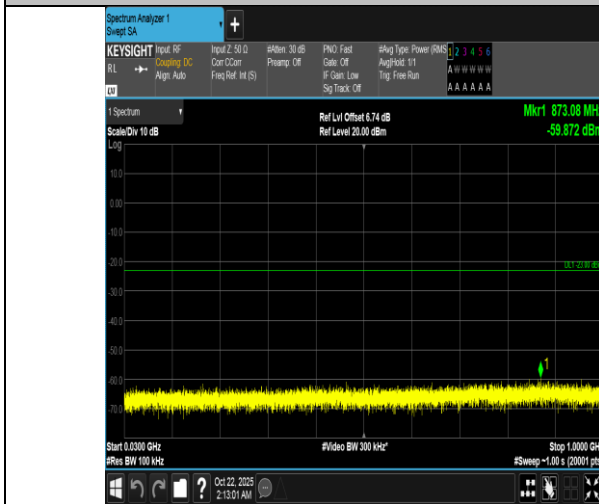
Band66-3MHz-QPSK-131987-1RB#0-30~1000-PASS
