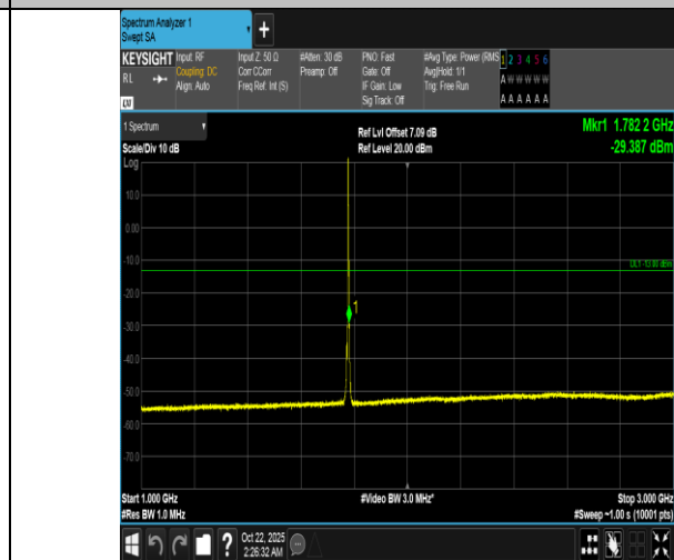
Band66-3MHz-QPSK-132657-1RB#0-1000~3000-PASS
