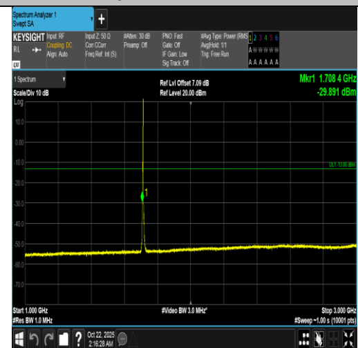
Band66-3MHz-16QAM-131987-1RB#14-1000~3000-PASS
