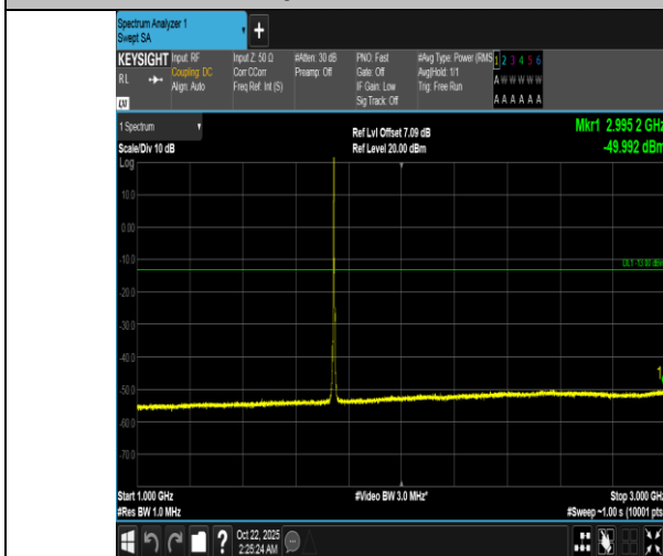
Band66-3MHz-16QAM-132322-15RB#0-1000~3000-PASS
