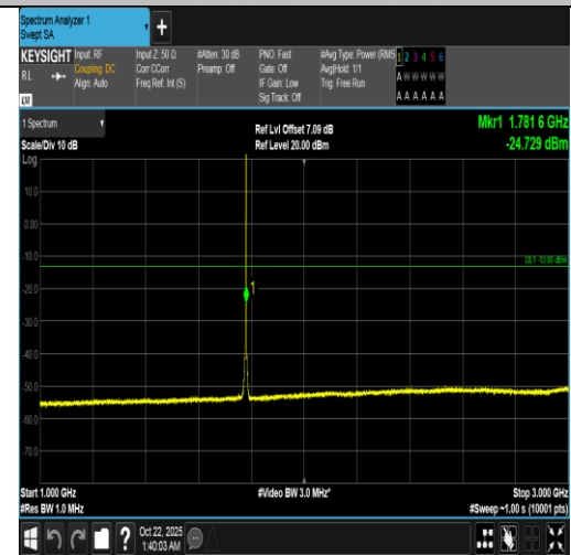
Band66-1.4MHz-16QAM-132665-1RB#5-1000~3000-PASS
