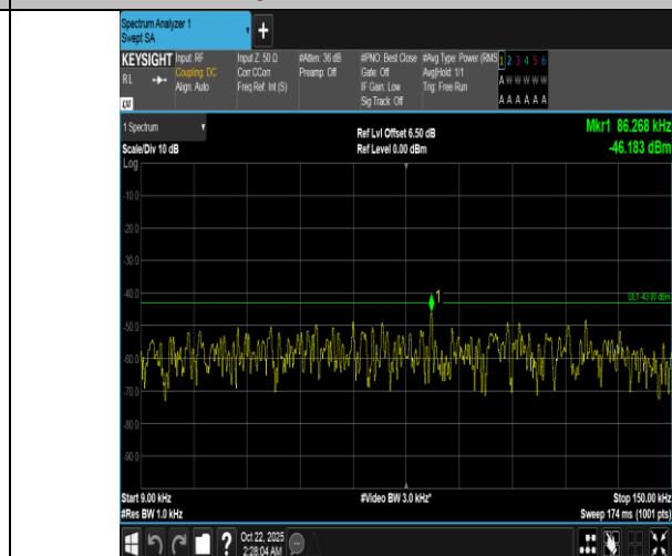
Band66-3MHz-QPSK-132657-1RB#14-0.009~0.15-PASS
