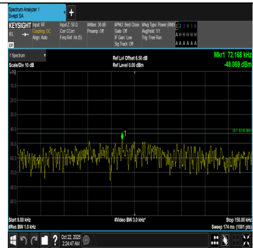
Band66-3MHz-16QAM-132322-15RB#0-0.009~0.15-PASS
