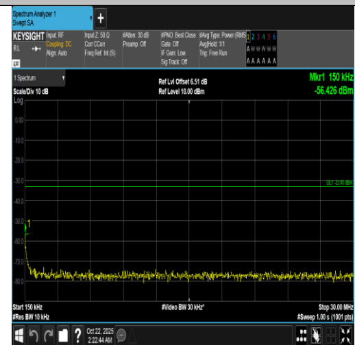
Band66-3MHz-16QAM-132322-1RB#14-0.15~30-PASS
