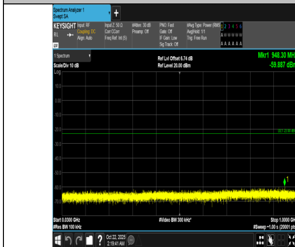
Band66-3MHz-QPSK-132322-1RB#0-30~1000-PASS
