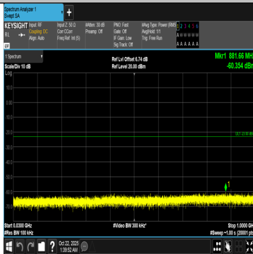
Band66-1.4MHz-16QAM-132665-1RB#5-30~1000-PASS
