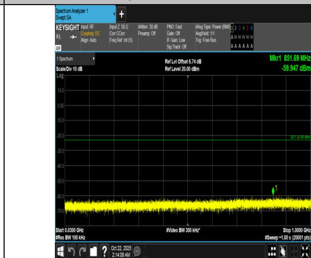
Band66-3MHz-16QAM-131987-1RB#0-30~1000-PASS
