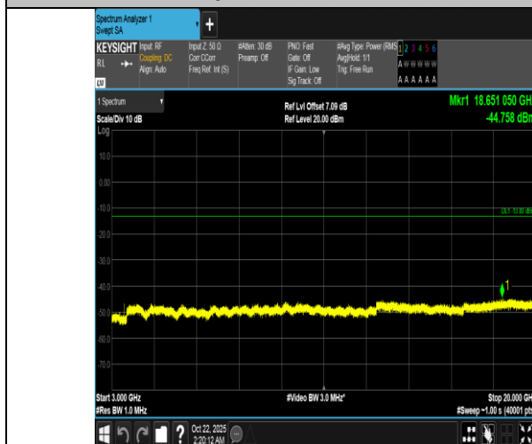
Band66-3MHz-QPSK-132322-1RB#0-3000~20000-PASS
