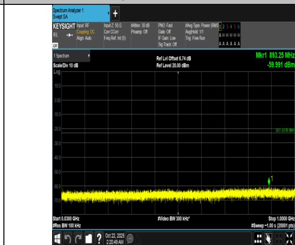
Band66-3MHz-16QAM-132322-1RB#0-30~1000-PASS
