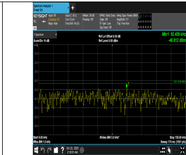
Band66-3MHz-16QAM-131987-15RB#0-0.009~0.15-PASS
