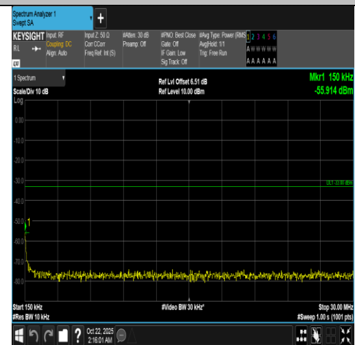
Band66-3MHz-16QAM-131987-1RB#14-0.15~30-PASS
