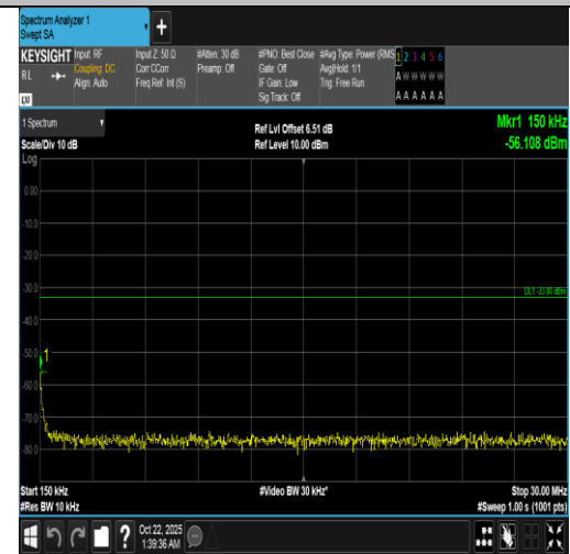
Band66-1.4MHz-16QAM-132665-1RB#5-0.15~30-PASS
