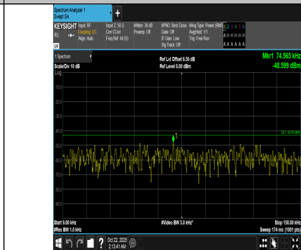
Band66-3MHz-16QAM-131987-1RB#0-0.009~0.15-PASS
