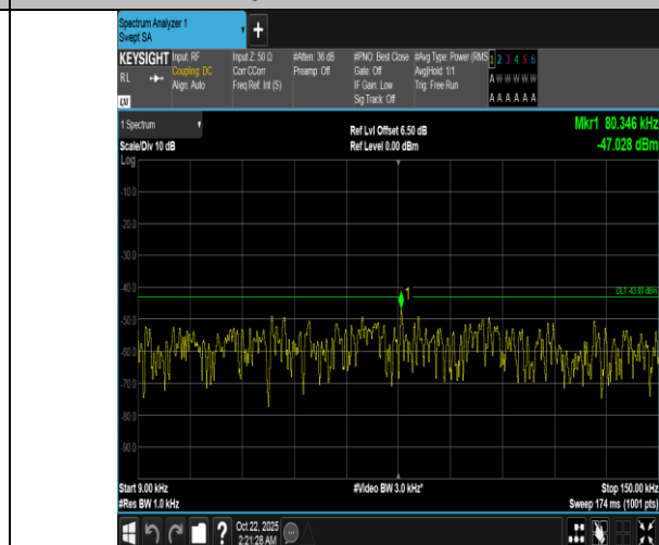
Band66-3MHz-QPSK-132322-1RB#14-0.009~0.15-PASS
