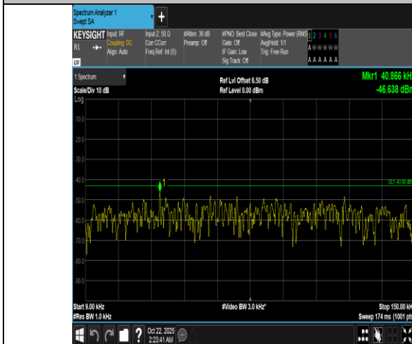
Band66-3MHz-QPSK-132322-15RB#0-0.009~0.15-PASS
