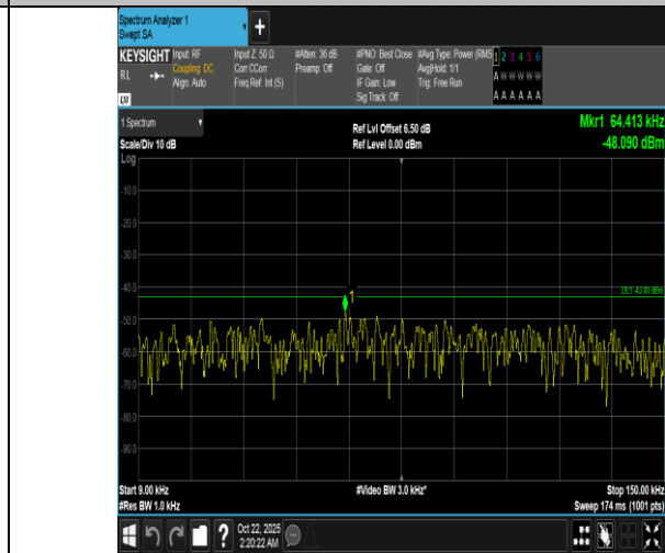
Band66-3MHz-16QAM-132322-1RB#0-0.009~0.15-PASS
