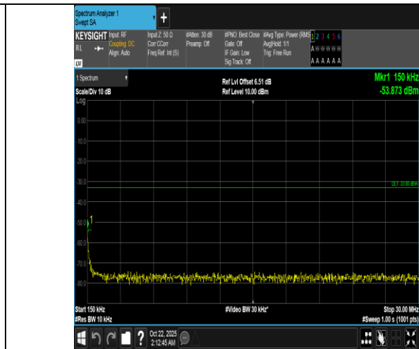
Band66-3MHz-QPSK-131987-1RB#0-0.15~30-PASS
