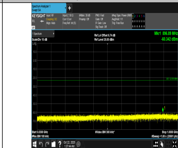
Band66-1.4MHz-16QAM-132665-1RB#0-30~1000-PASS
