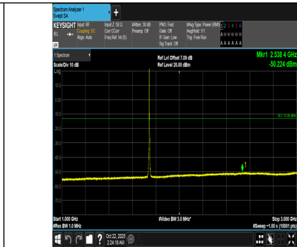
Band66-3MHz-QPSK-132322-15RB#0-1000~3000-PASS
