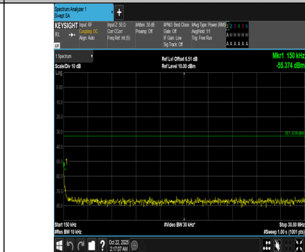
Band66-3MHz-QPSK-131987-15RB#0-0.15~30-PASS
