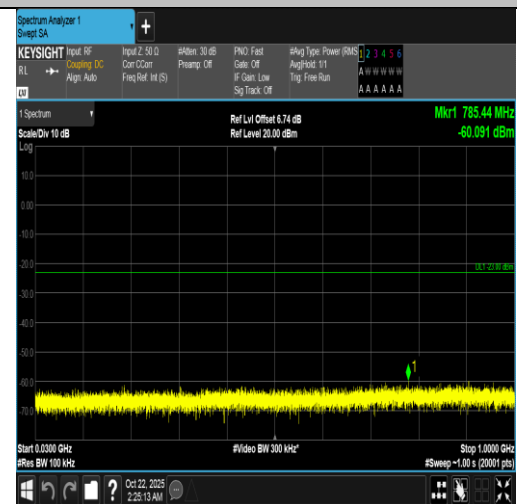
Band66-3MHz-16QAM-132322-15RB#0-30~1000-PASS
