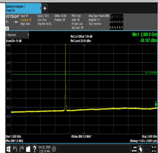
Band66-3MHz-16QAM-132322-1RB#14-1000~3000-PASS
