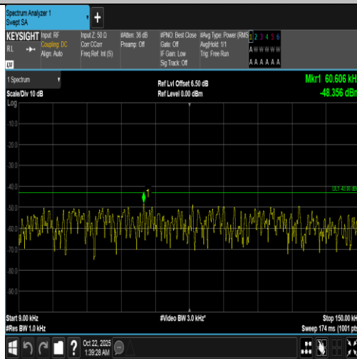
Band66-1.4MHz-16QAM-132665-1RB#5-0.009~0.15-PASS
