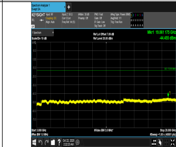
Band66-3MHz-QPSK-132322-1RB#14-3000~20000-PASS
