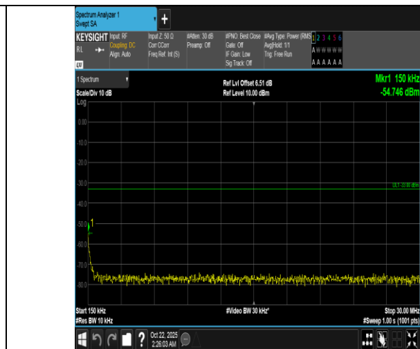
Band66-3MHz-QPSK-132657-1RB#0-0.15~30-PASS
