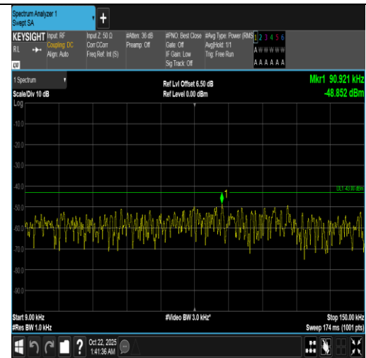
Band66-1.4MHz-16QAM-132665-6RB#0-0.009~0.15-PASS
