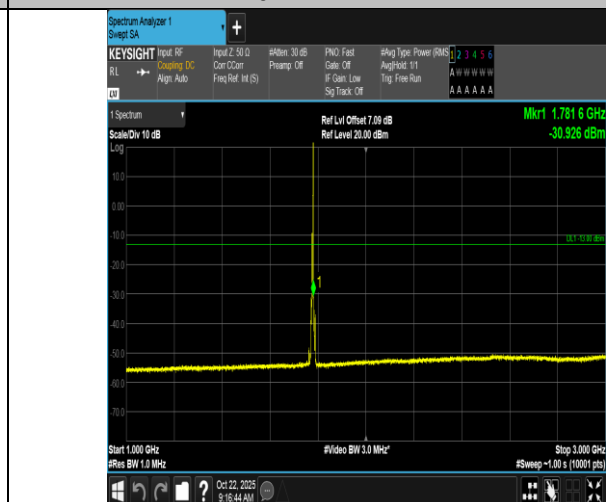
Band66-5MHz-16QAM-132647-1RB#24-1000~3000-PASS
