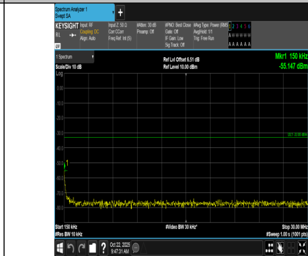
Band66-10MHz-16QAM-132022-1RB#49-0.15~30-PASS
