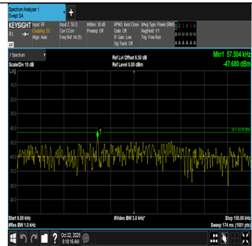
Band66-5MHz-16QAM-132647-25RB#0-0.009~0.15-PASS
