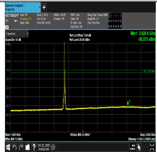
Band66-10MHz-QPSK-132322-1RB#0-1000~3000-PASS
