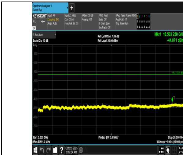
Band66-5MHz-16QAM-132647-1RB#24-3000~20000-PASS
