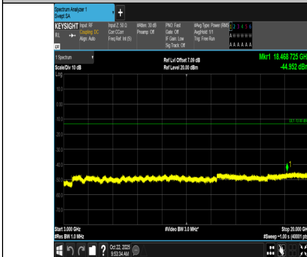
Band66-10MHz-QPSK-132622-1RB#0-3000~20000-PASS
