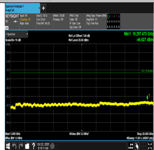
Band66-5MHz-16QAM-132647-25RB#0-3000~20000-PASS
