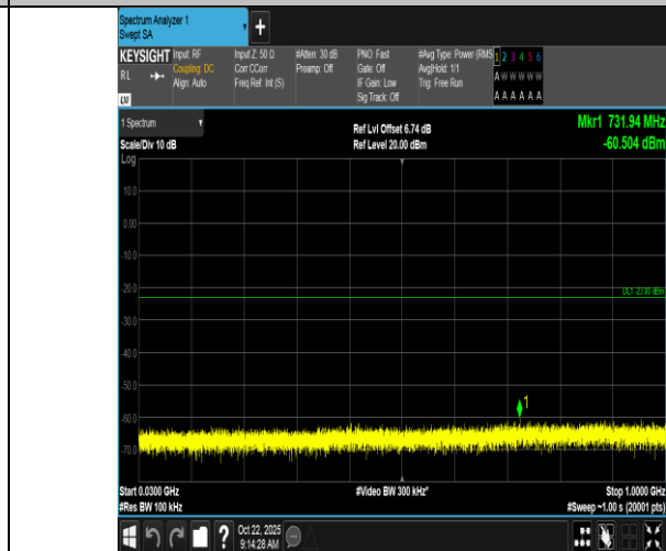
Band66-5MHz-16QAM-132647-1RB#0-30~1000-PASS
