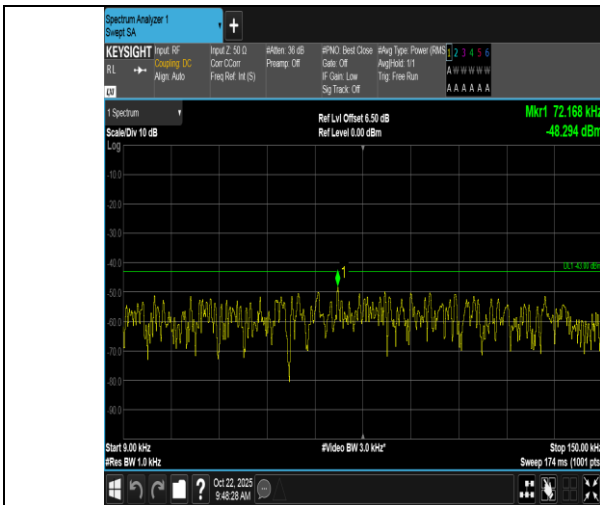
Band66-10MHz-QPSK-132322-1RB#0-0.009~0.15-PASS
