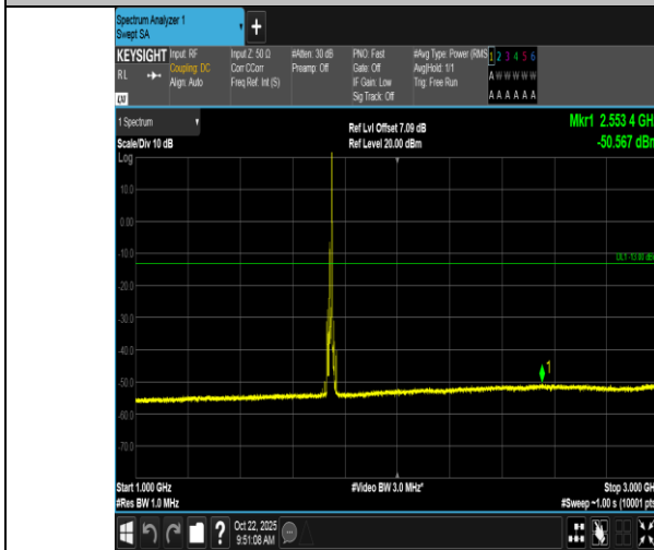
Band66-10MHz-QPSK-132322-1RB#49-1000~3000-PASS
