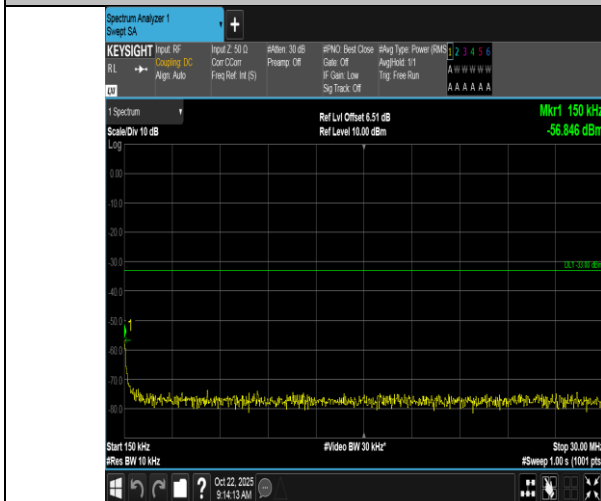
Band66-5MHz-16QAM-132647-1RB#0-0.15~30-PASS
