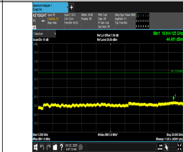
Band66-10MHz-QPSK-132022-1RB#49-3000~20000-PASS
