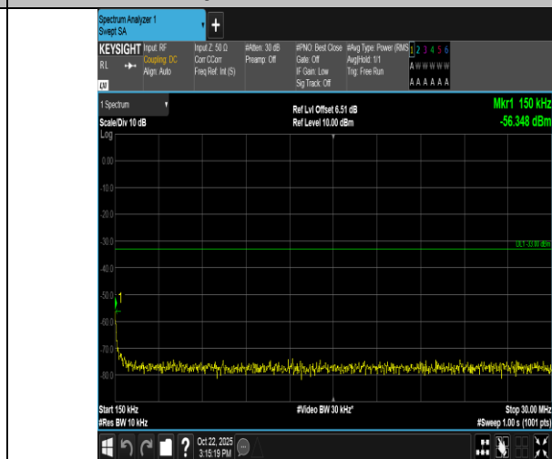
Band66-10MHz-QPSK-132322-50RB#0-0.15~30-PASS
