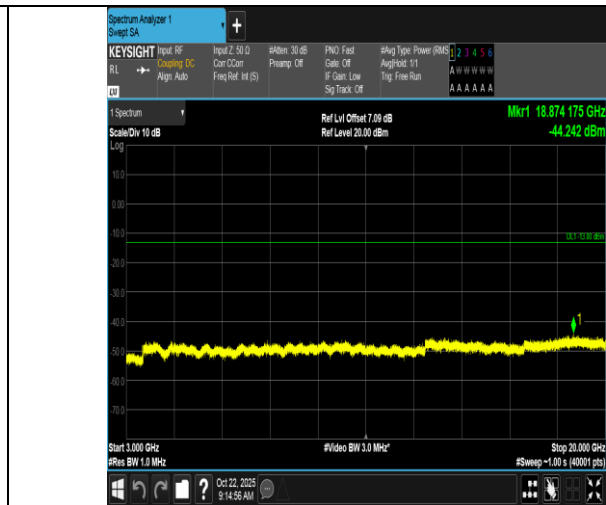
Band66-5MHz-16QAM-132647-1RB#0-3000~20000-PASS
