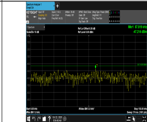
Band66-10MHz-QPSK-132622-1RB#49-0.009~0.15-PASS
