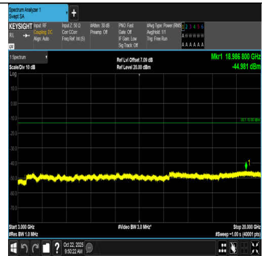
Band66-10MHz-16QAM-132322-1RB#0-3000~20000-PASS
