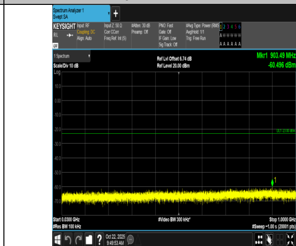
Band66-10MHz-16QAM-132322-1RB#0-30~1000-PASS
