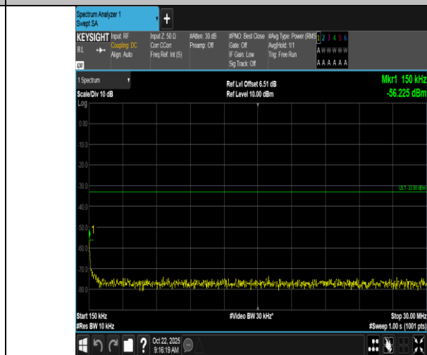
Band66-5MHz-16QAM-132647-1RB#24-0.15~30-PASS
