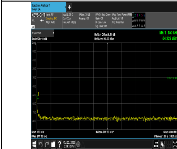
Band66-10MHz-16QAM-132022-50RB#0-0.15~30-PASS
