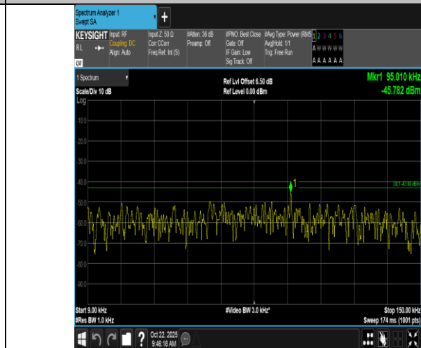
Band66-10MHz-QPSK-132022-1RB#49-0.009~0.15-PASS
