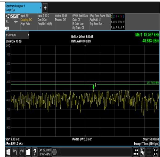
Band66-10MHz-16QAM-132322-50RB#0-0.009~0.15-PASS
