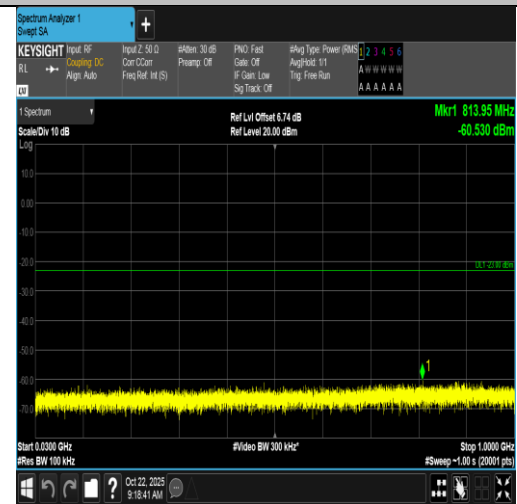
Band66-5MHz-16QAM-132647-25RB#0-30~1000-PASS
