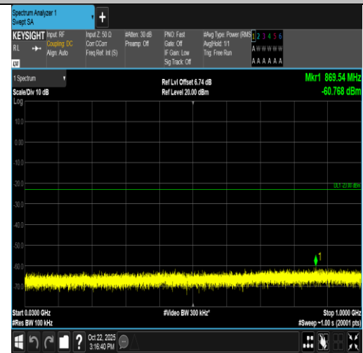
Band66-10MHz-16QAM-132322-50RB#0-30~1000-PASS
