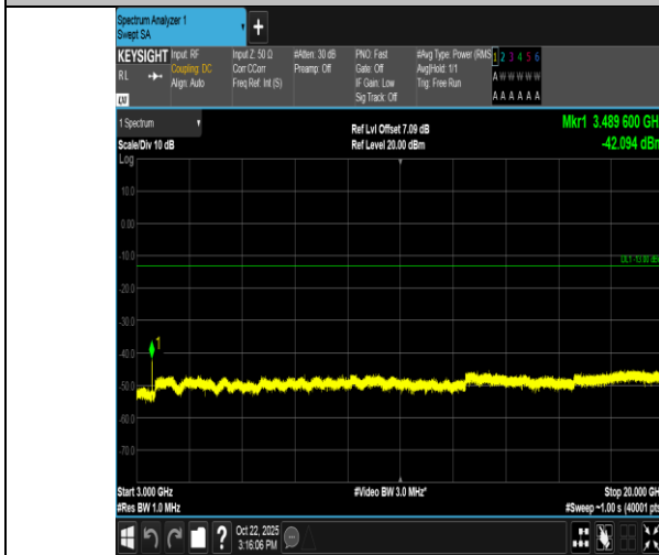
Band66-10MHz-QPSK-132322-50RB#0-3000~20000-PASS
