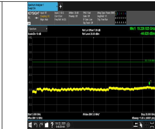
Band66-10MHz-16QAM-132022-1RB#0-3000~20000-PASS
