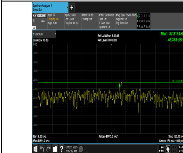
Band66-5MHz-QPSK-132647-25RB#0-0.009~0.15-PASS
