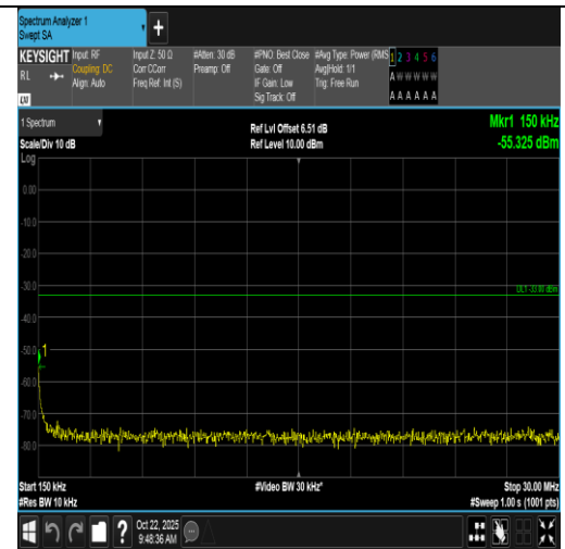
Band66-10MHz-QPSK-132322-1RB#0-0.15~30-PASS
