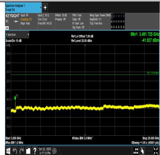
Band66-10MHz-16QAM-132322-50RB#0-3000~20000-PASS
