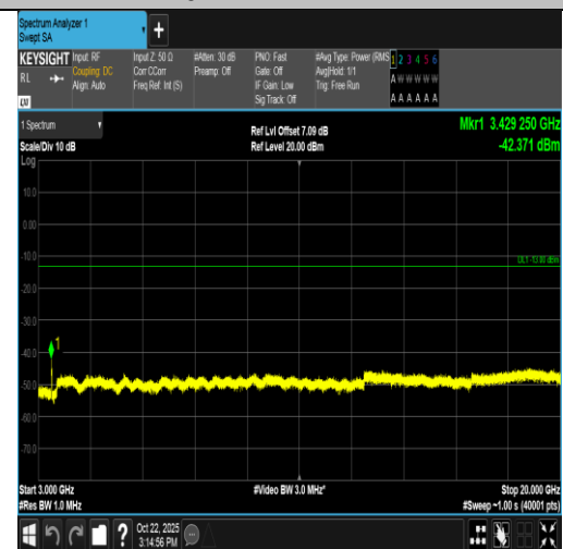
Band66-10MHz-16QAM-132022-50RB#0-3000~20000-PASS
