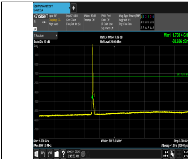
Band66-10MHz-16QAM-132022-1RB#0-1000~3000-PASS
