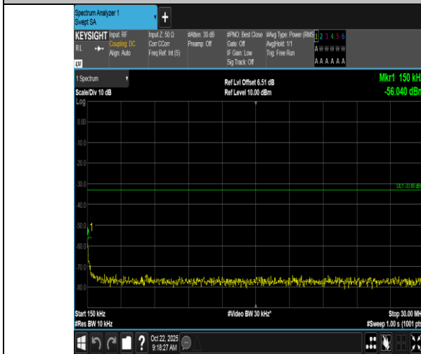
Band66-5MHz-16QAM-132647-25RB#0-0.15~30-PASS
