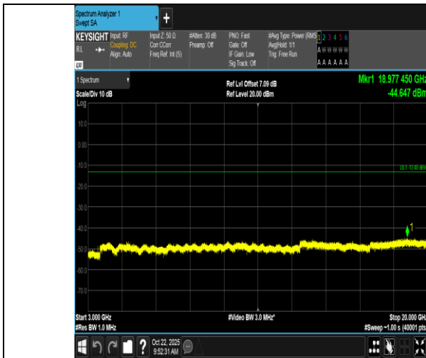
Band66-10MHz-16QAM-132322-1RB#49-3000~20000-PASS
