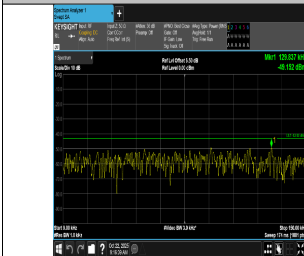
Band66-5MHz-16QAM-132647-1RB#24-0.009~0.15-PASS
