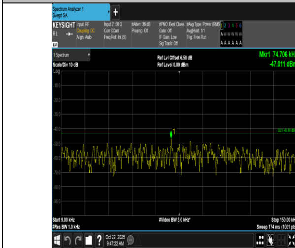
Band66-10MHz-16QAM-132022-1RB#49-0.009~0.15-PASS
