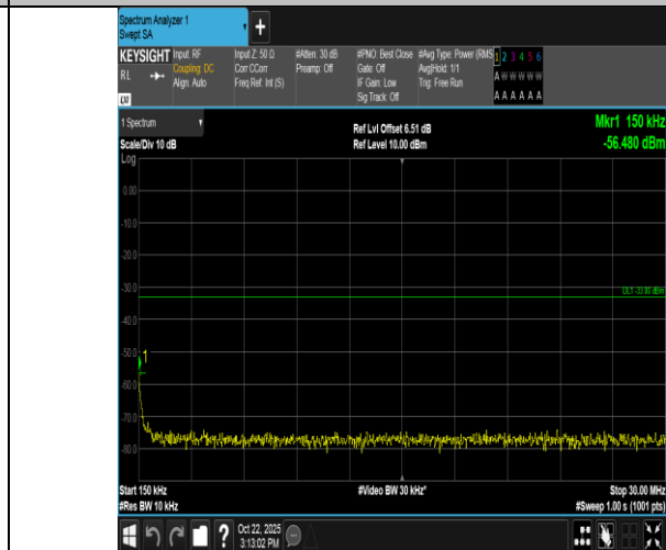
Band66-10MHz-QPSK-132022-50RB#0-0.15~30-PASS
