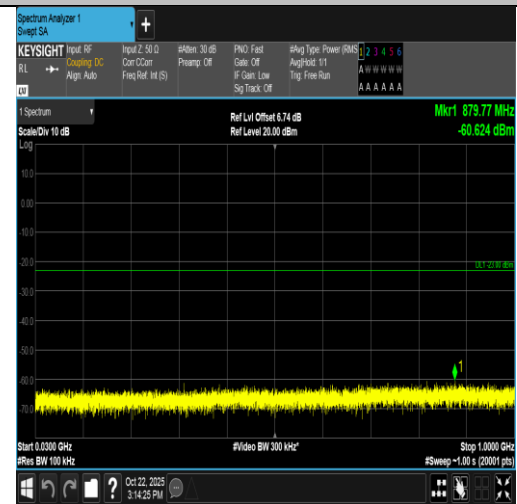
Band66-10MHz-16QAM-132022-50RB#0-30~1000-PASS
