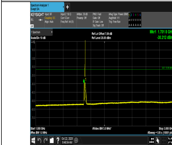
Band66-10MHz-QPSK-132022-1RB#49-1000~3000-PASS
