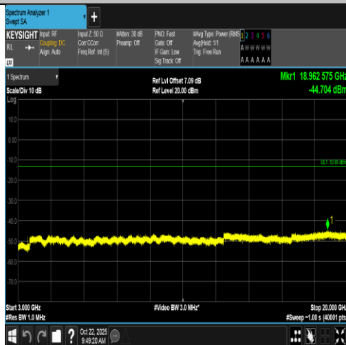
Band66-10MHz-QPSK-132322-1RB#0-3000~20000-PASS
