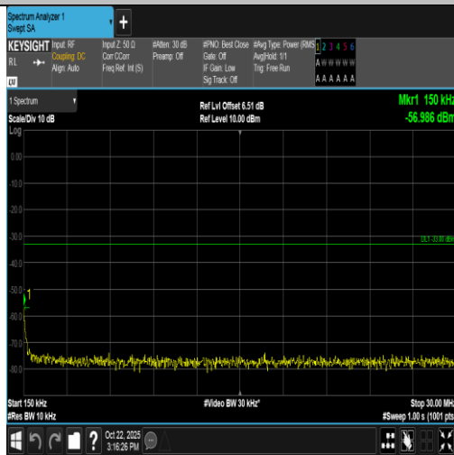
Band66-10MHz-16QAM-132322-50RB#0-0.15~30-PASS
