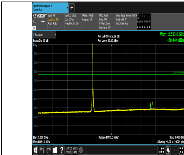
Band66-10MHz-16QAM-132322-1RB#0-1000~3000-PASS
