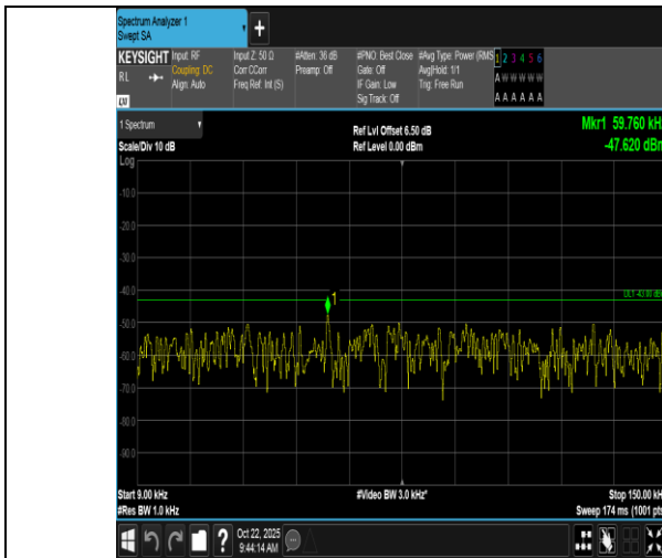
Band66-10MHz-QPSK-132022-1RB#0-0.009~0.15-PASS
