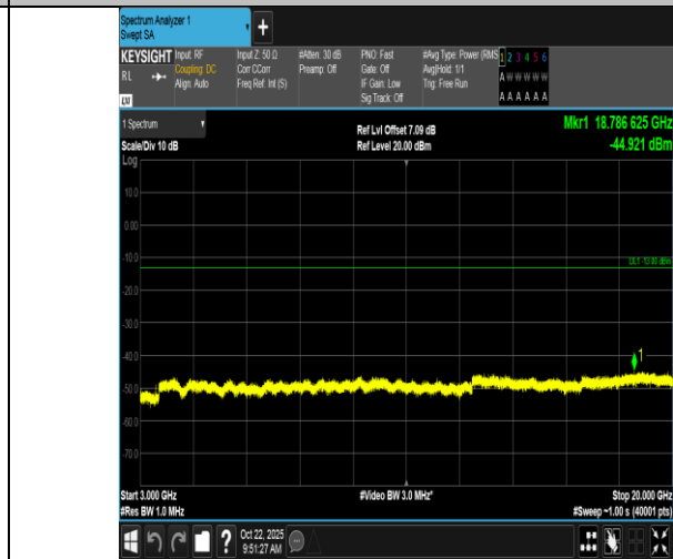
Band66-10MHz-QPSK-132322-1RB#49-3000~20000-PASS
