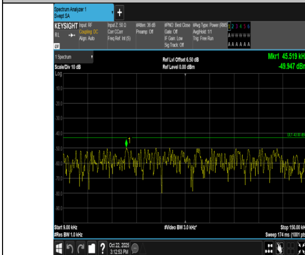
Band66-10MHz-QPSK-132022-50RB#0-0.009~0.15-PASS
