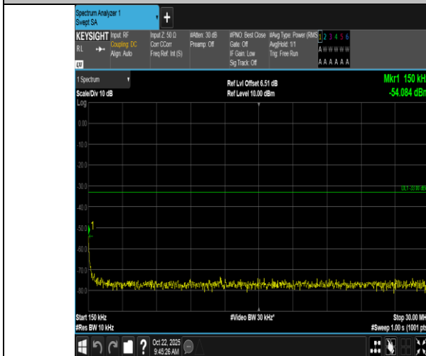
Band66-10MHz-16QAM-132022-1RB#0-0.15~30-PASS
