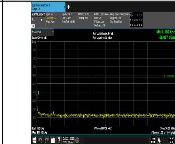
Band66-5MHz-QPSK-132647-25RB#0-0.15~30-PASS
