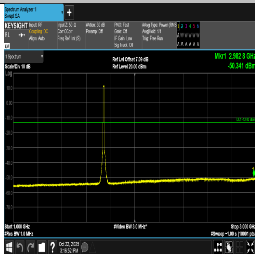
Band66-10MHz-16QAM-132322-50RB#0-1000~3000-PASS
