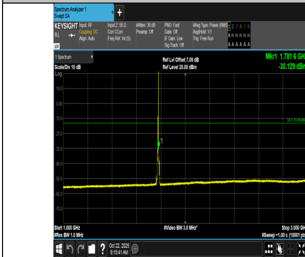
Band66-5MHz-QPSK-132647-1RB#24-1000~3000-PASS
