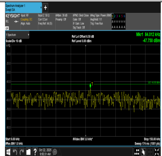
Band66-10MHz-QPSK-132322-1RB#49-0.009~0.15-PASS
