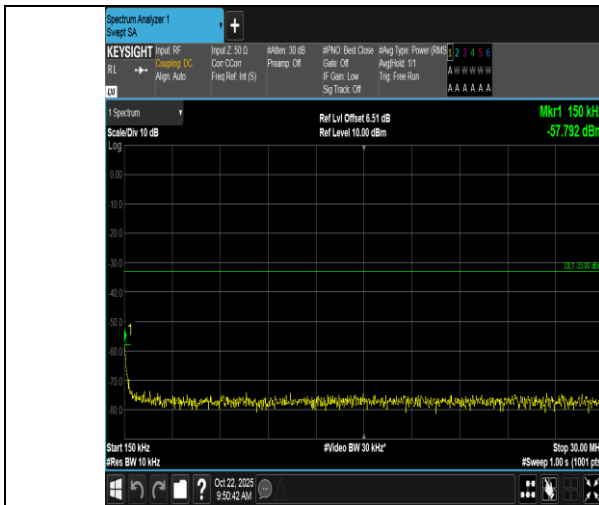
Band66-10MHz-QPSK-132322-1RB#49-0.15~30-PASS
