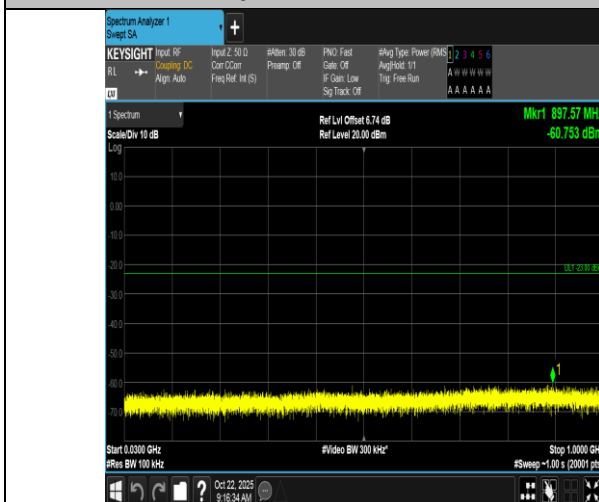
Band66-5MHz-16QAM-132647-1RB#24-30~1000-PASS
