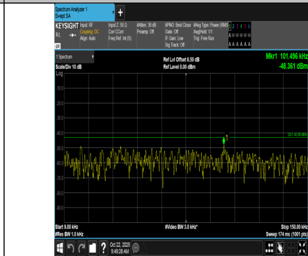
Band66-10MHz-16QAM-132322-1RB#0-0.009~0.15-PASS
