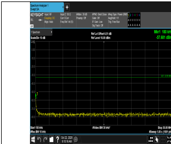
Band66-5MHz-QPSK-132647-1RB#24-0.15~30-PASS
