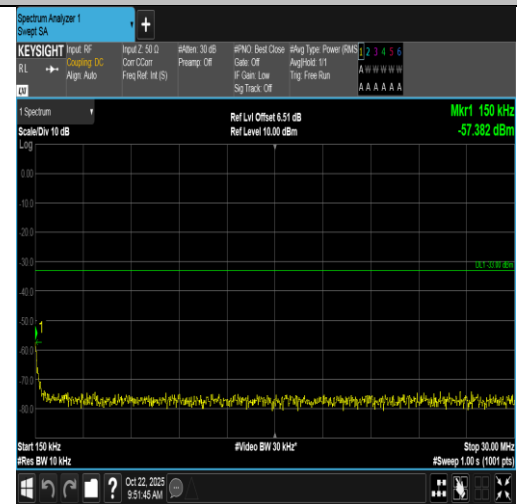
Band66-10MHz-16QAM-132322-1RB#49-0.15~30-PASS
