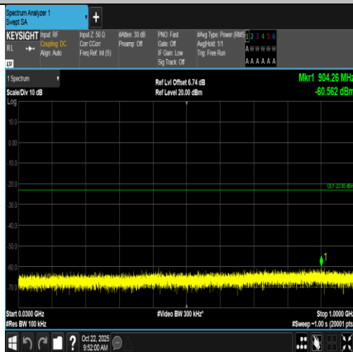
Band66-10MHz-16QAM-132322-1RB#49-30~1000-PASS
