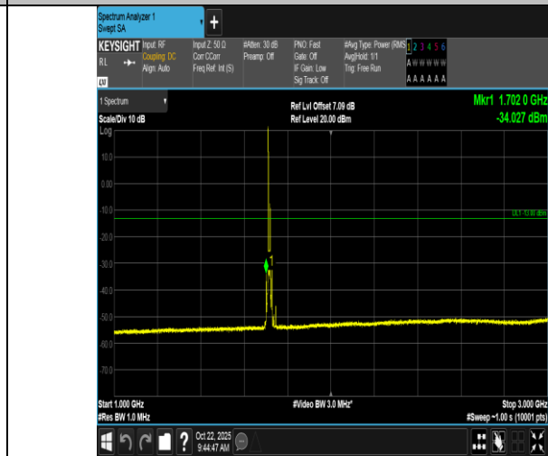
Band66-10MHz-QPSK-132022-1RB#0-1000~3000-PASS
