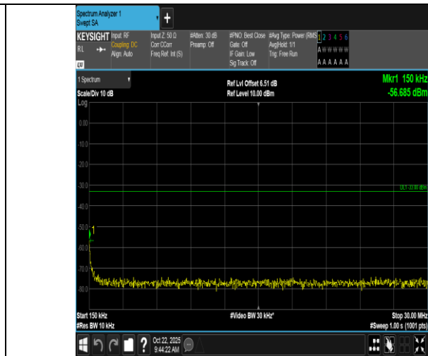
Band66-10MHz-QPSK-132022-1RB#0-0.15~30-PASS
