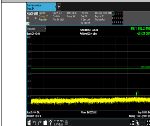
Band66-10MHz-16QAM-132022-1RB#49-30~1000-PASS
