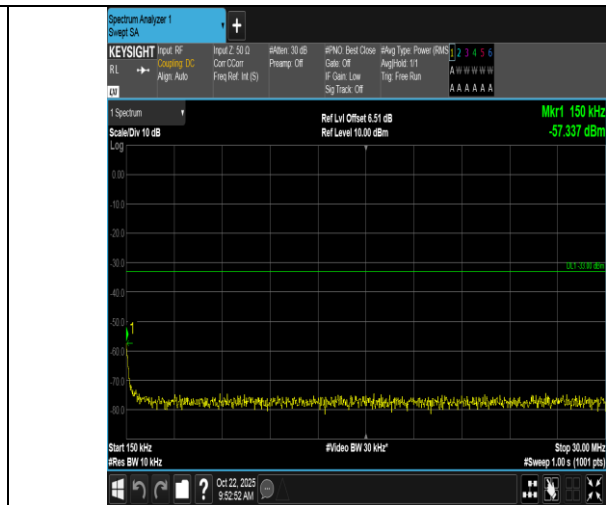
Band66-10MHz-QPSK-132622-1RB#0-0.15~30-PASS
