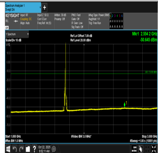
Band66-10MHz-16QAM-132322-1RB#49-1000~3000-PASS
