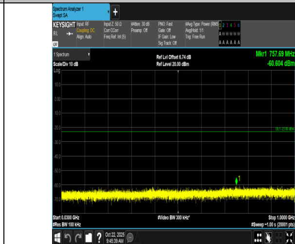
Band66-10MHz-16QAM-132022-1RB#0-30~1000-PASS
