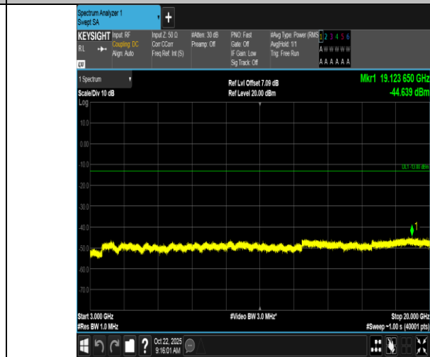
Band66-5MHz-QPSK-132647-1RB#24-3000~20000-PASS
