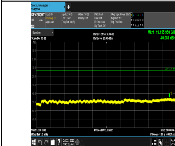
Band66-10MHz-QPSK-132022-1RB#0-3000~20000-PASS
