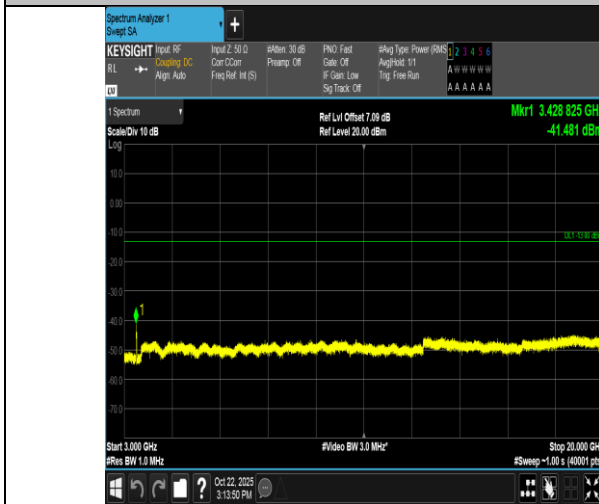
Band66-10MHz-QPSK-132022-50RB#0-3000~20000-PASS
