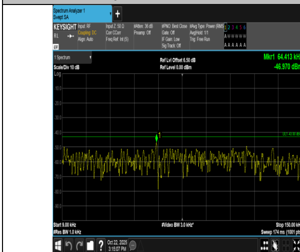
Band66-10MHz-QPSK-132322-50RB#0-0.009~0.15-PASS
