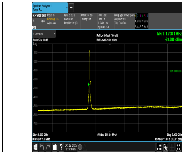
Band66-10MHz-QPSK-132022-50RB#0-1000~3000-PASS
