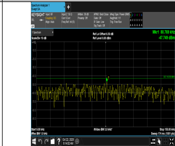
Band66-5MHz-16QAM-132647-1RB#0-0.009~0.15-PASS
