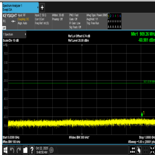
Band66-10MHz-QPSK-132322-1RB#0-30~1000-PASS
