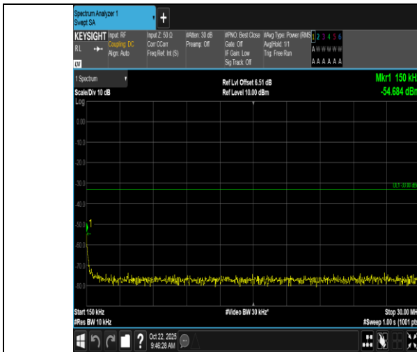
Band66-10MHz-QPSK-132022-1RB#49-0.15~30-PASS
