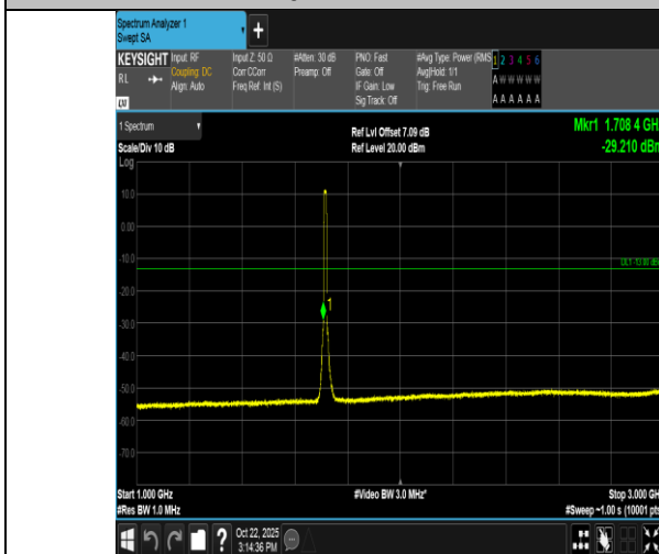
Band66-10MHz-16QAM-132022-50RB#0-1000~3000-PASS
