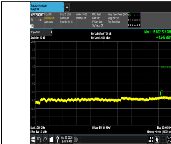
Band66-10MHz-16QAM-132022-1RB#49-3000~20000-PASS
