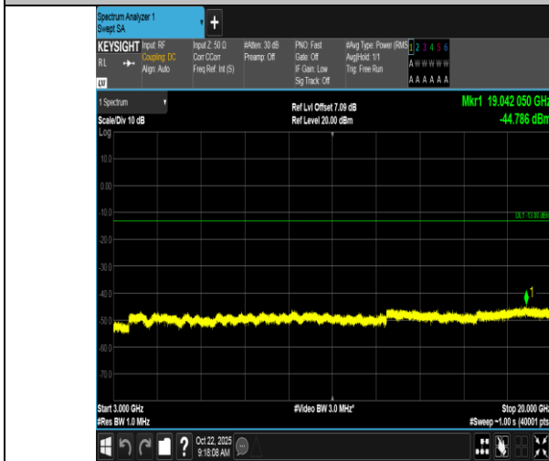
Band66-5MHz-QPSK-132647-25RB#0-3000~20000-PASS
