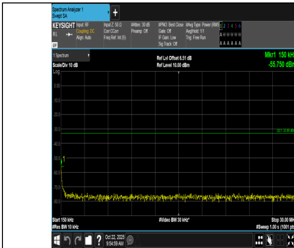
Band66-10MHz-QPSK-132622-1RB#49-0.15~30-PASS
