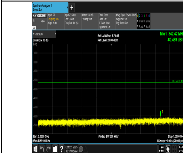
Band66-15MHz-16QAM-132322-1RB#74-30~1000-PASS
