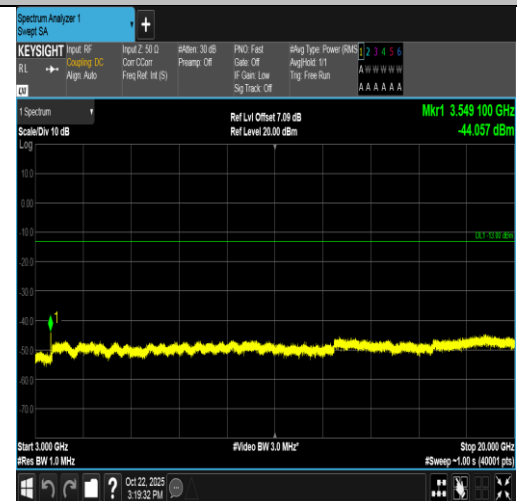
Band66-10MHz-16QAM-132622-50RB#0-3000~20000-PASS
