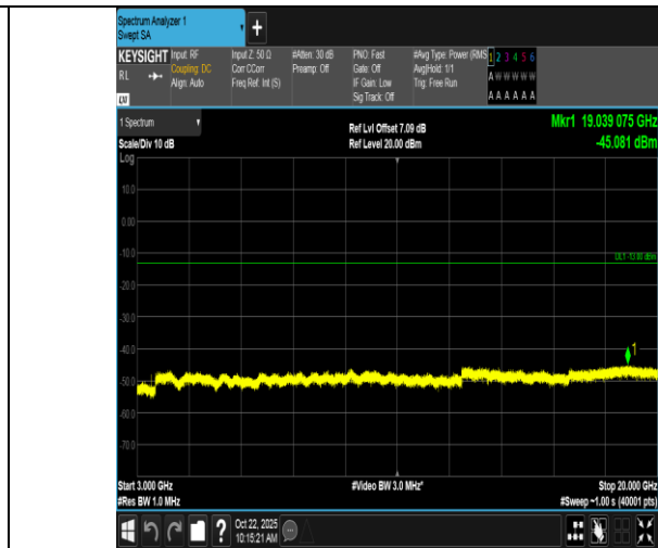
Band66-15MHz-16QAM-132322-1RB#0-3000~20000-PASS
