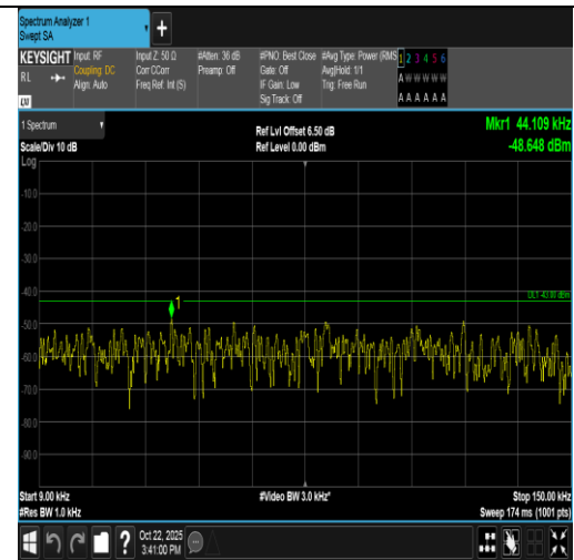
Band66-15MHz-16QAM-132322-75RB#0-0.009~0.15-PASS
