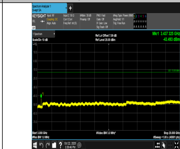
Band66-15MHz-16QAM-132047-75RB#0-3000~20000-PASS
