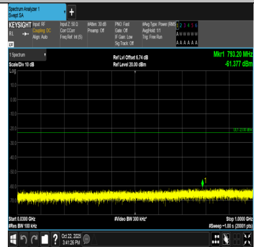
Band66-15MHz-16QAM-132322-75RB#0-30~1000-PASS
