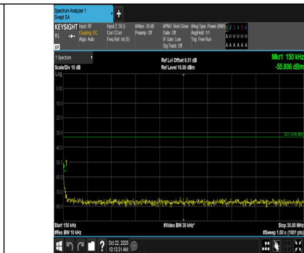
Band66-15MHz-QPSK-132322-1RB#0-0.15~30-PASS
