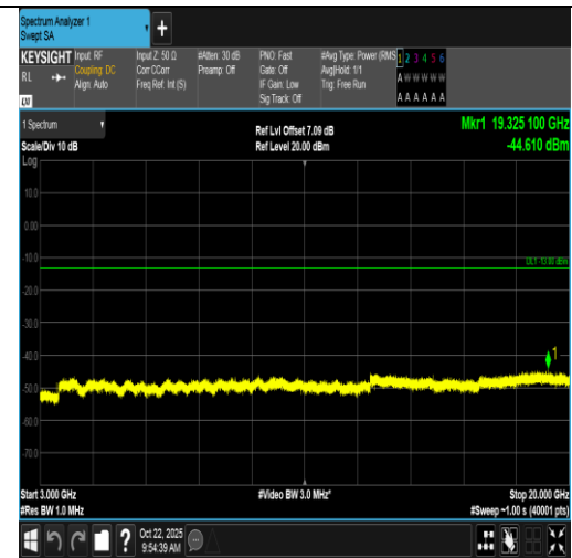
Band66-10MHz-16QAM-132622-1RB#0-3000~20000-PASS
