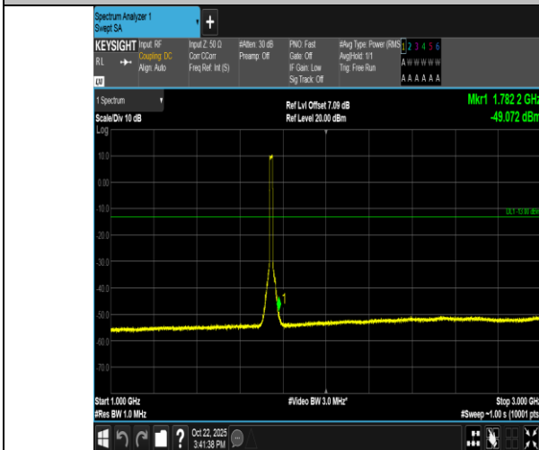
Band66-15MHz-16QAM-132322-75RB#0-1000~3000-PASS
