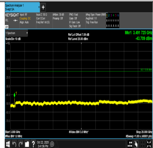
Band66-15MHz-16QAM-132322-75RB#0-3000~20000-PASS
