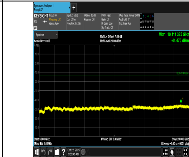
Band66-10MHz-QPSK-132622-1RB#49-3000~20000-PASS
