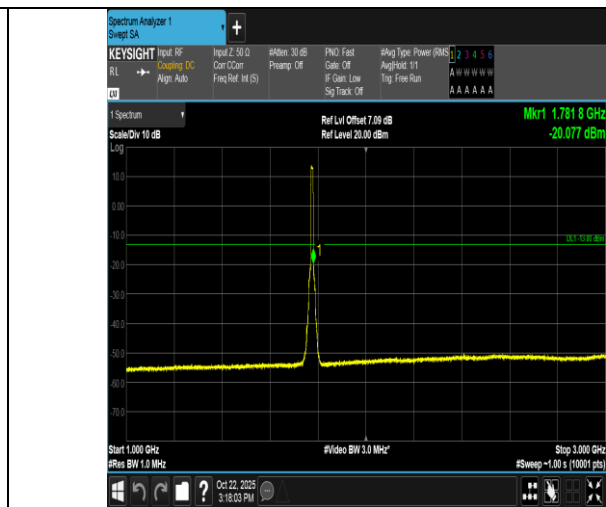
Band66-10MHz-QPSK-132622-50RB#0-1000~3000-PASS
