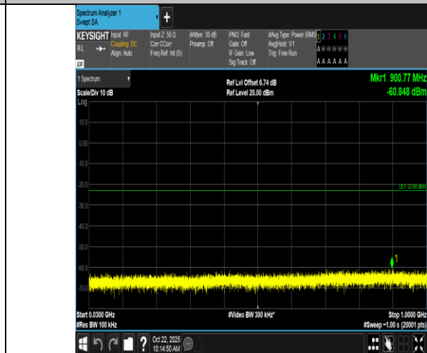
Band66-15MHz-16QAM-132322-1RB#0-30~1000-PASS
