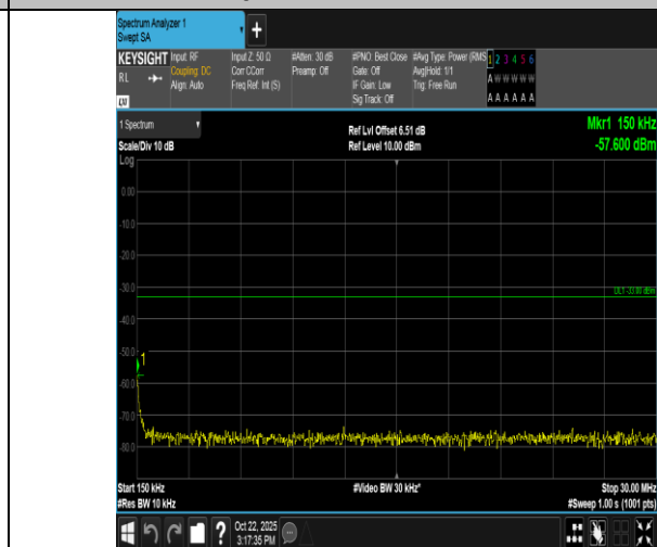
Band66-10MHz-QPSK-132622-50RB#0-0.15~30-PASS
