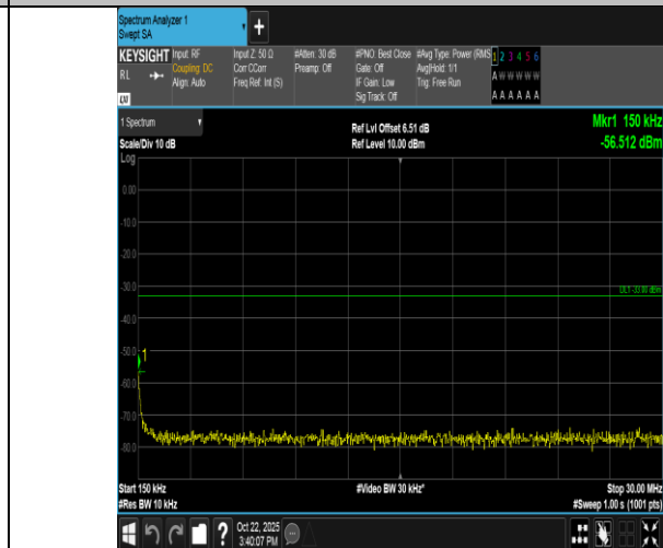
Band66-15MHz-QPSK-132322-75RB#0-0.15~30-PASS
