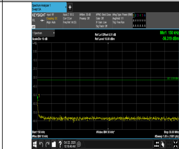
Band66-15MHz-16QAM-132322-1RB#74-0.15~30-PASS
