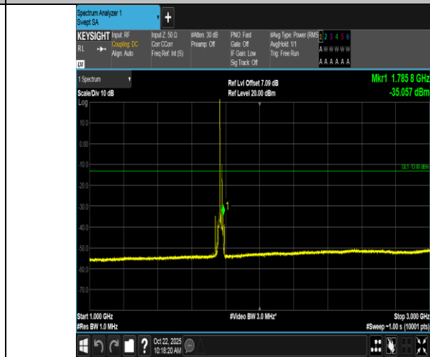
Band66-15MHz-QPSK-132597-1RB#0-1000~3000-PASS
