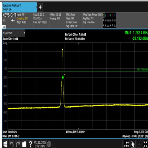
Band66-10MHz-16QAM-132622-50RB#0-1000~3000-PASS
