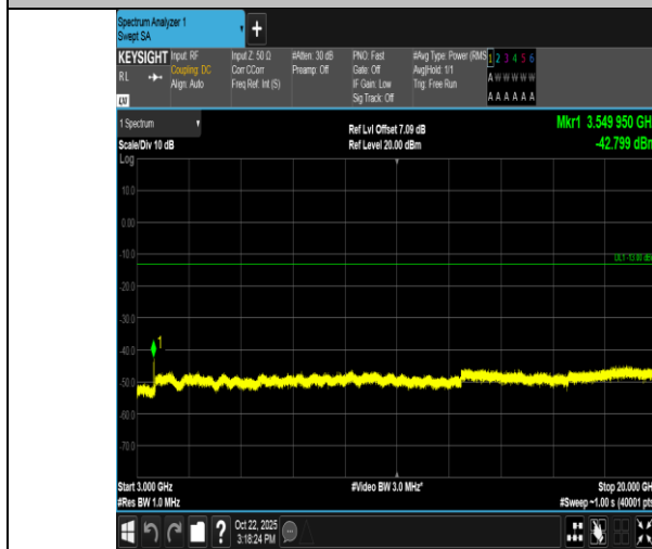
Band66-10MHz-QPSK-132622-50RB#0-3000~20000-PASS
