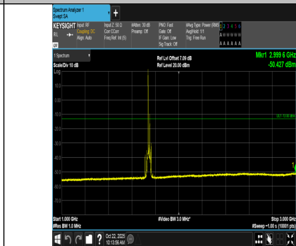
Band66-15MHz-QPSK-132322-1RB#0-1000~3000-PASS
