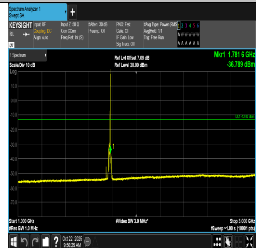
Band66-10MHz-16QAM-132622-1RB#49-1000~3000-PASS
