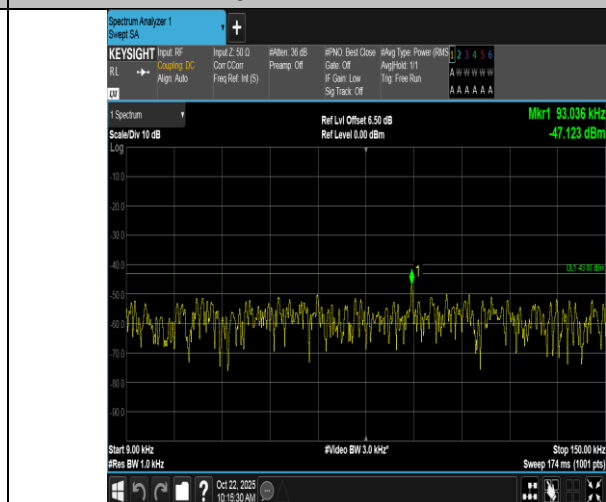
Band66-15MHz-QPSK-132322-1RB#74-0.009~0.15-PASS
