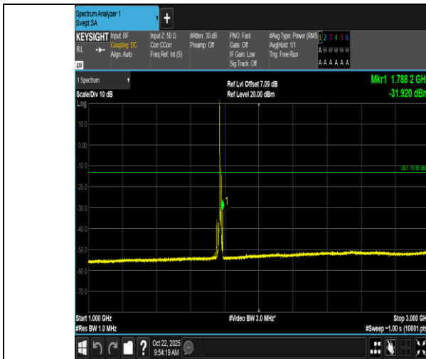
Band66-10MHz-16QAM-132622-1RB#0-1000~3000-PASS
