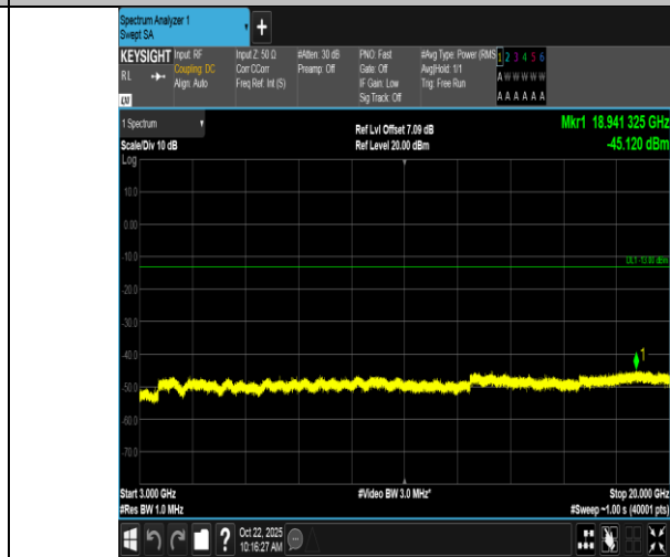
Band66-15MHz-QPSK-132322-1RB#74-3000~20000-PASS
