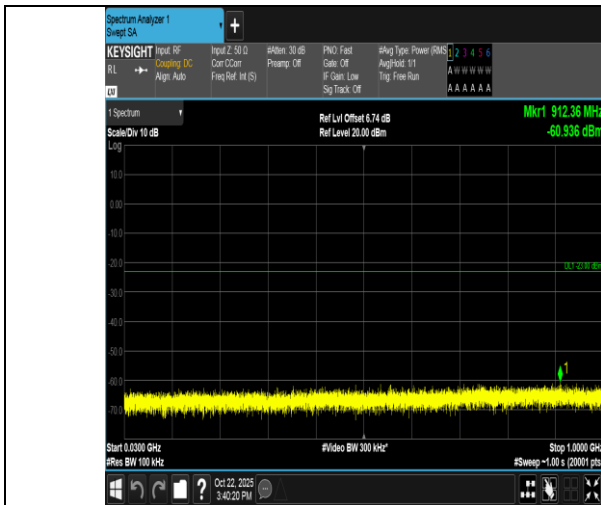
Band66-15MHz-QPSK-132322-75RB#0-30~1000-PASS
