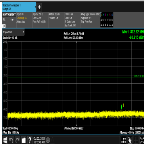
Band66-15MHz-16QAM-132047-1RB#74-30~1000-PASS
