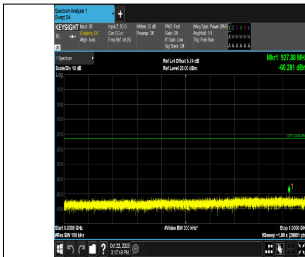
Band66-10MHz-QPSK-132622-50RB#0-30~1000-PASS
