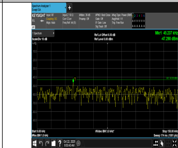
Band66-10MHz-16QAM-132622-1RB#0-0.009~0.15-PASS
