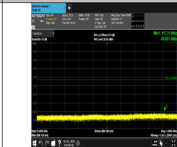
Band66-10MHz-16QAM-132622-1RB#0-30~1000-PASS
