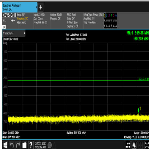
Band66-10MHz-16QAM-132622-1RB#49-30~1000-PASS
