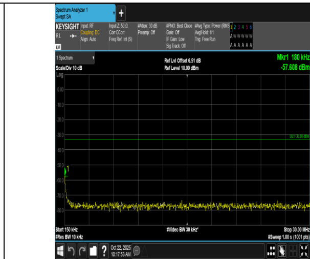
Band66-15MHz-QPSK-132597-1RB#0-0.15~30-PASS
