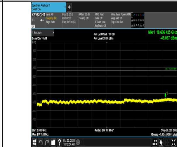
Band66-15MHz-QPSK-132047-1RB#74-3000~20000-PASS
