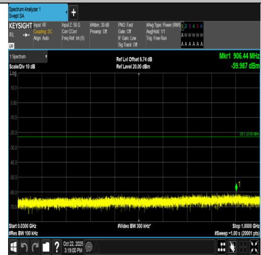
Band66-10MHz-16QAM-132622-50RB#0-30~1000-PASS
