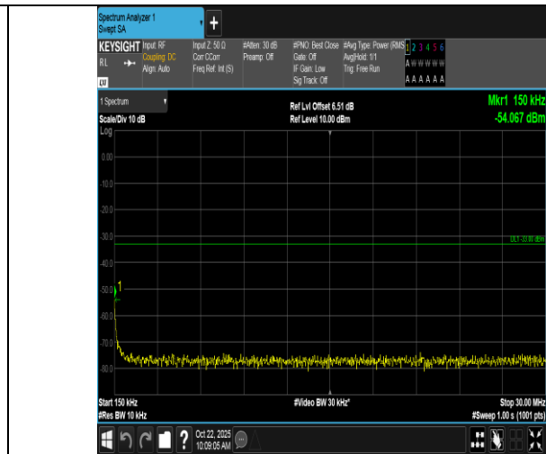
Band66-15MHz-QPSK-132047-1RB#0-0.15~30-PASS
