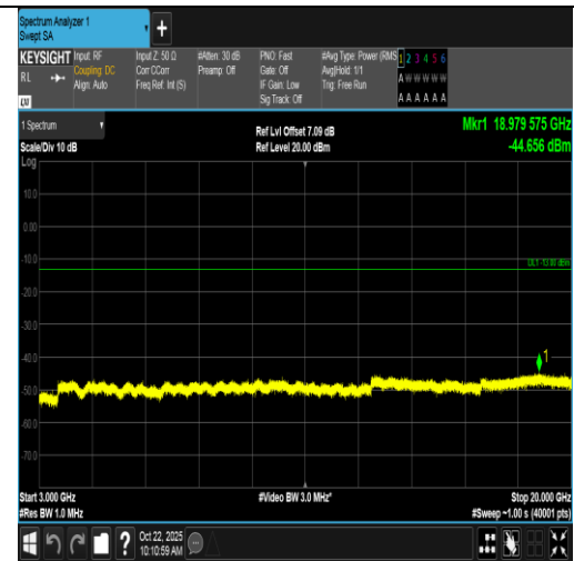
Band66-15MHz-16QAM-132047-1RB#0-3000~20000-PASS
