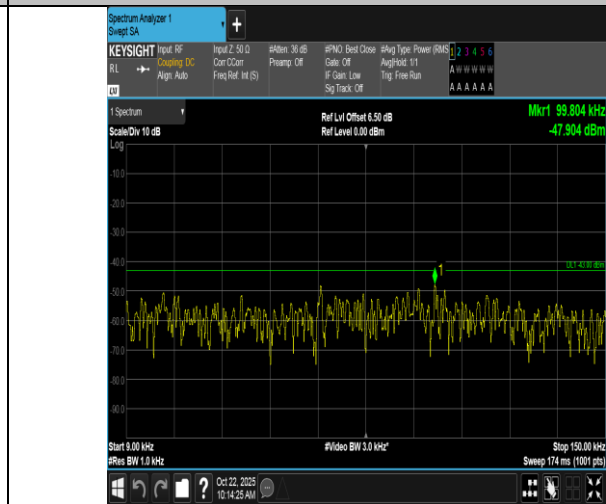
Band66-15MHz-16QAM-132322-1RB#0-0.009~0.15-PASS
