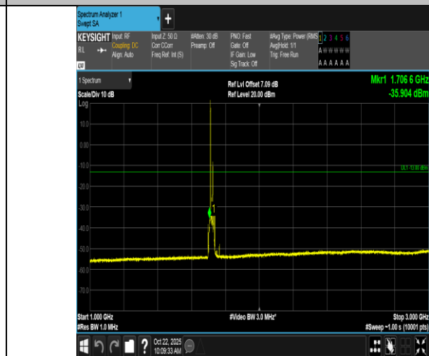
Band66-15MHz-QPSK-132047-1RB#0-1000~3000-PASS
