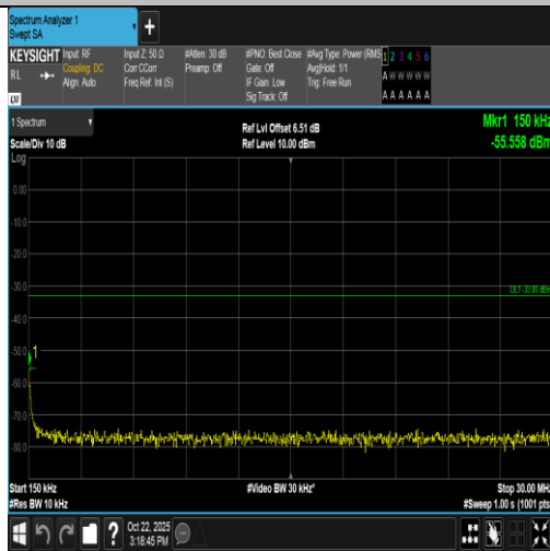
Band66-10MHz-16QAM-132622-50RB#0-0.15~30-PASS
