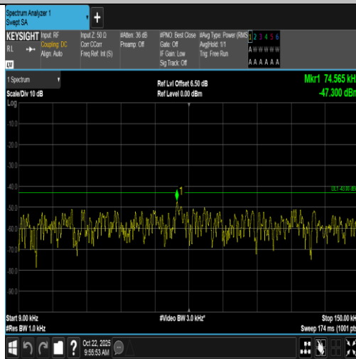
Band66-10MHz-16QAM-132622-1RB#49-0.009~0.15-PASS
