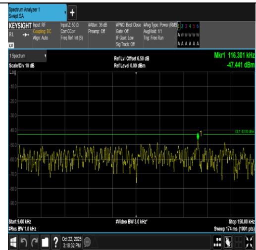
Band66-10MHz-16QAM-132622-50RB#0-0.009~0.15-PASS
