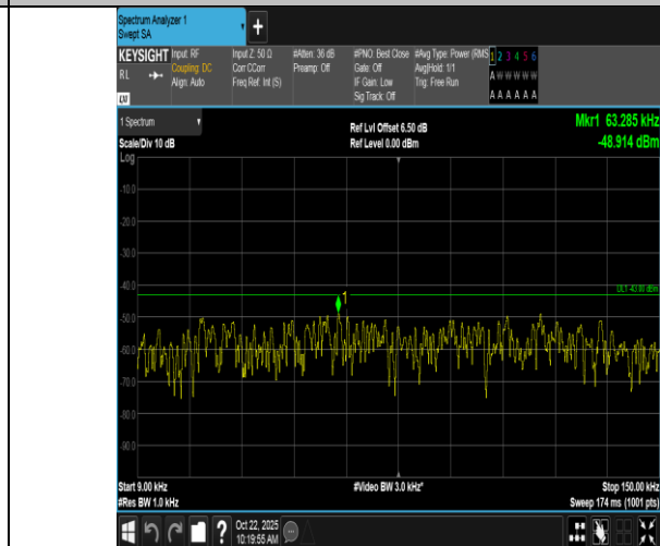
Band66-15MHz-QPSK-132597-1RB#74-0.009~0.15-PASS
