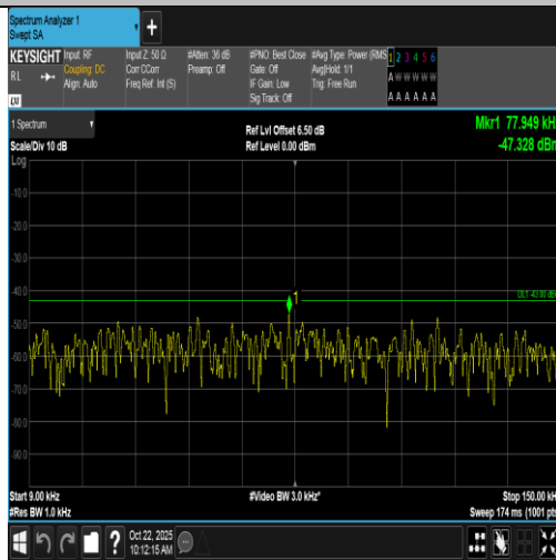
Band66-15MHz-16QAM-132047-1RB#74-0.009~0.15-PASS
