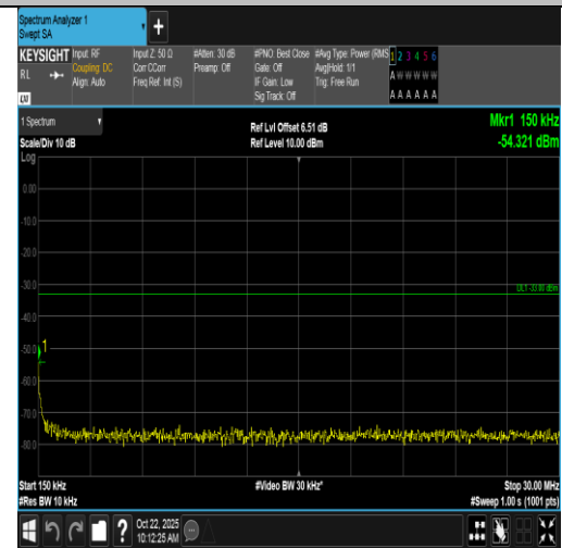
Band66-15MHz-16QAM-132047-1RB#74-0.15~30-PASS
