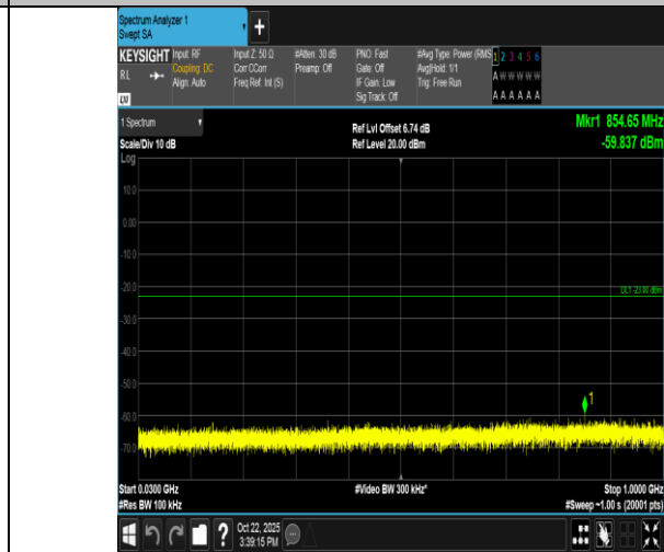
Band66-15MHz-16QAM-132047-75RB#0-30~1000-PASS
