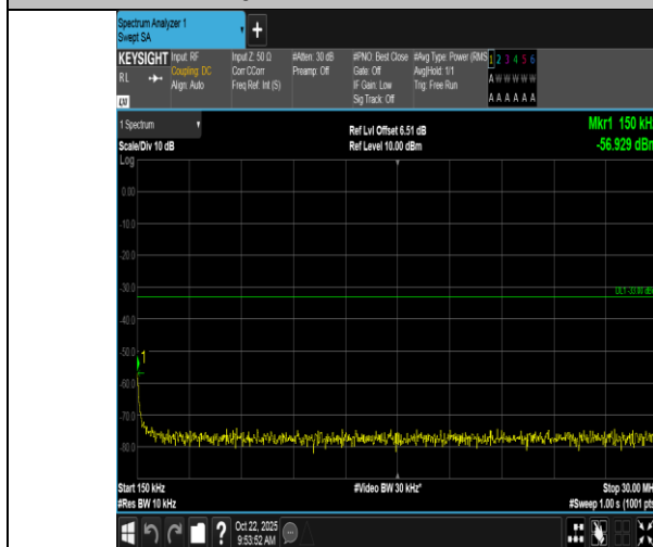
Band66-10MHz-16QAM-132622-1RB#0-0.15~30-PASS
