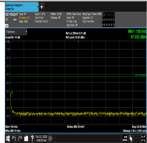
Band66-10MHz-16QAM-132622-1RB#49-0.15~30-PASS
