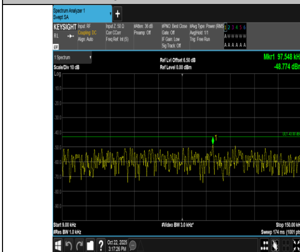
Band66-10MHz-QPSK-132622-50RB#0-0.009~0.15-PASS
