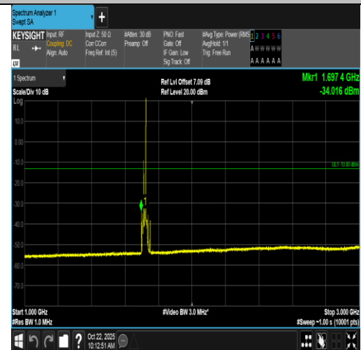
Band66-15MHz-16QAM-132047-1RB#74-1000~3000-PASS
