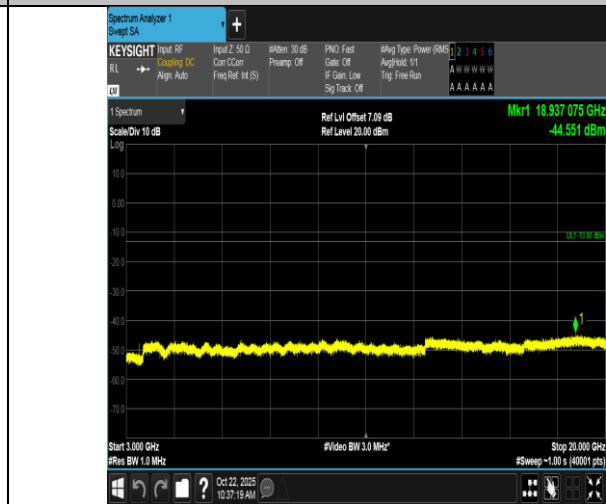
Band66-20MHz-QPSK-132072-1RB#99-3000~20000-PASS
