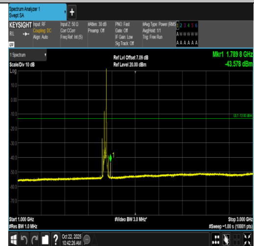
Band66-20MHz-16QAM-132322-1RB#99-1000~3000-PASS
