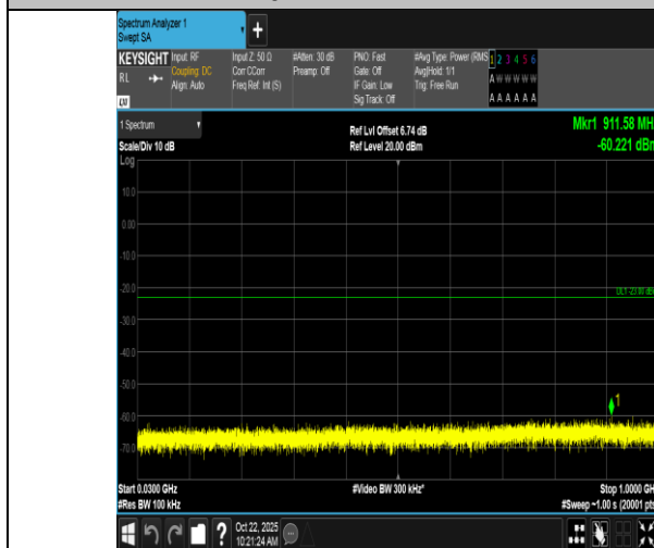
Band66-15MHz-16QAM-132597-1RB#74-30~1000-PASS
