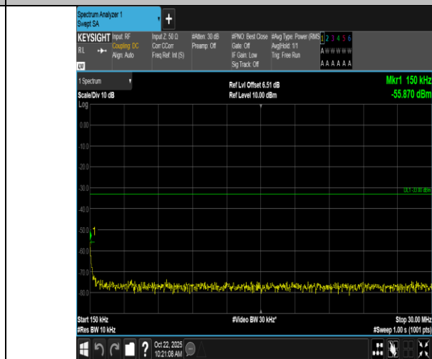
Band66-15MHz-16QAM-132597-1RB#74-0.15~30-PASS
