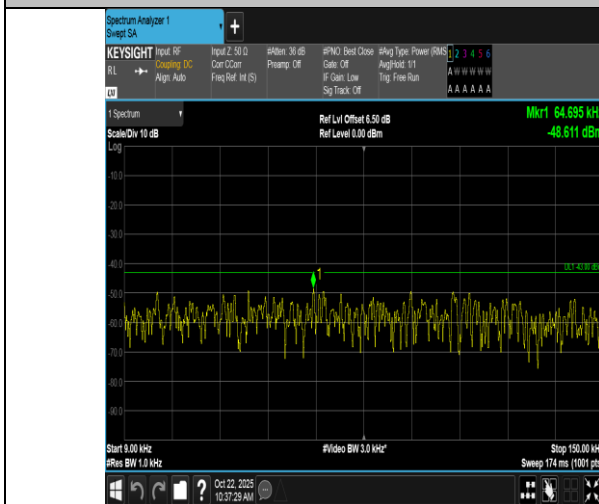
Band66-20MHz-16QAM-132072-1RB#99-0.009~0.15-PASS
