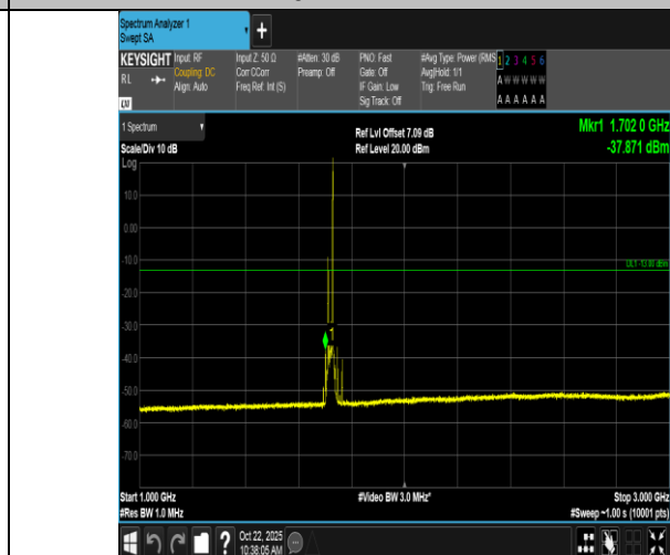
Band66-20MHz-16QAM-132072-1RB#99-1000~3000-PASS
