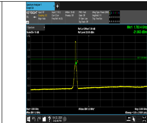
Band66-15MHz-QPSK-132597-75RB#0-1000~3000-PASS
