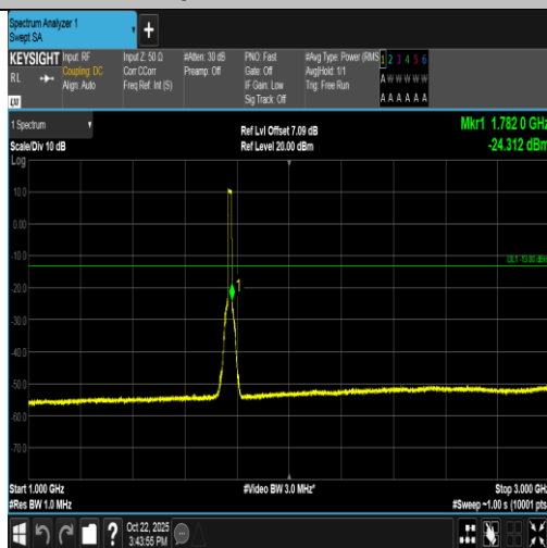
Band66-15MHz-16QAM-132597-75RB#0-1000~3000-PASS
