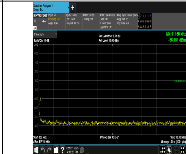
Band66-20MHz-QPSK-132072-100RB#0-0.15~30-PASS
