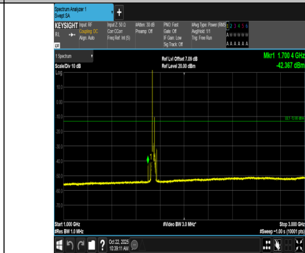
Band66-20MHz-QPSK-132322-1RB#0-1000~3000-PASS
