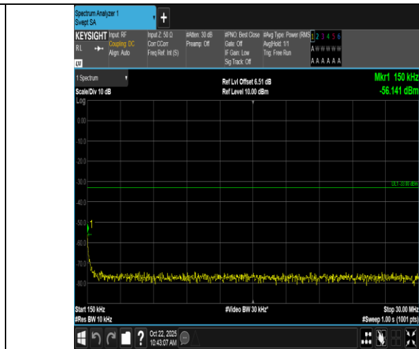
Band66-20MHz-QPSK-132572-1RB#0-0.15~30-PASS
