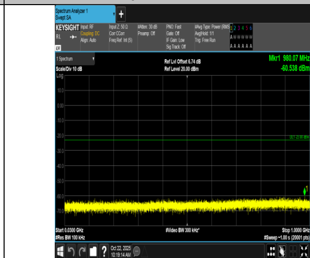
Band66-15MHz-16QAM-132597-1RB#0-30~1000-PASS
