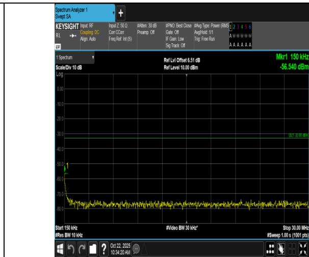
Band66-20MHz-QPSK-132072-1RB#0-0.15~30-PASS
