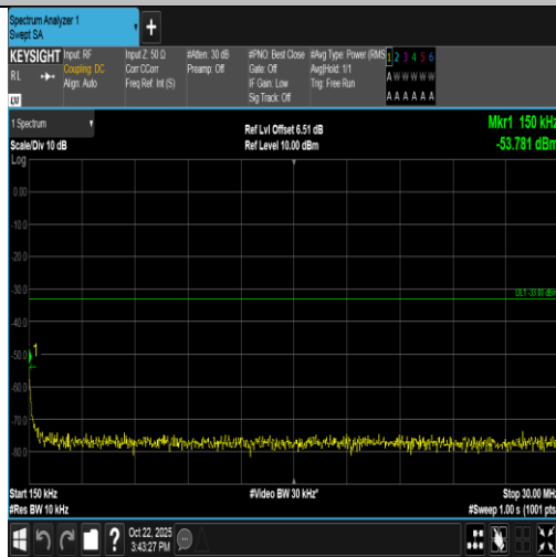
Band66-15MHz-16QAM-132597-75RB#0-0.15~30-PASS
