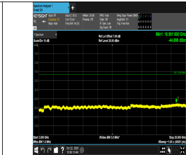
Band66-20MHz-16QAM-132072-1RB#0-3000~20000-PASS
