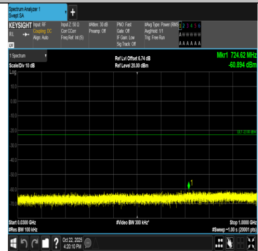
Band66-20MHz-16QAM-132322-100RB#0-30~1000-PASS
