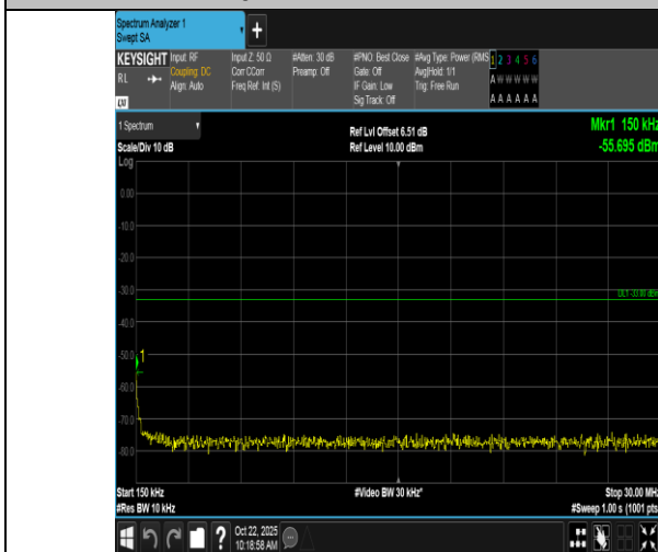
Band66-15MHz-16QAM-132597-1RB#0-0.15~30-PASS
