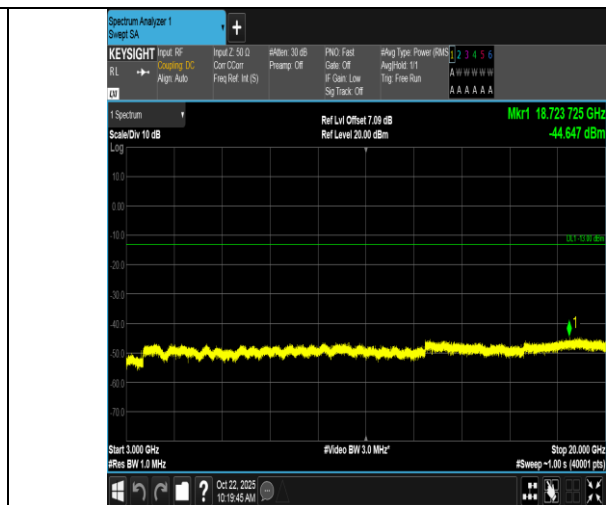
Band66-15MHz-16QAM-132597-1RB#0-3000~20000-PASS
