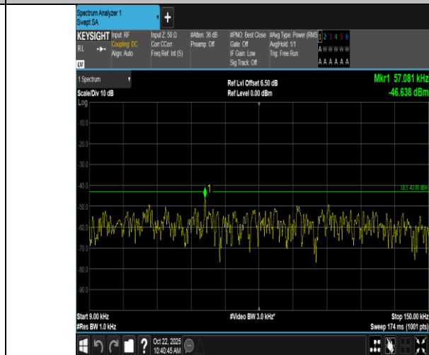
Band66-20MHz-QPSK-132322-1RB#99-0.009~0.15-PASS
