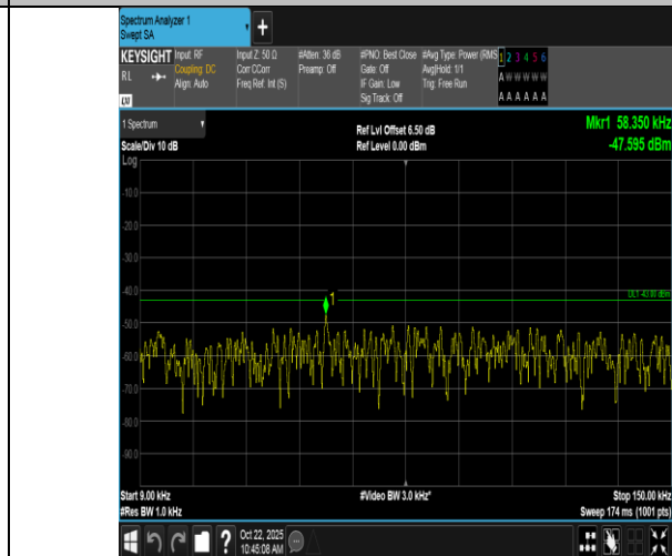
Band66-20MHz-QPSK-132572-1RB#99-0.009~0.15-PASS
