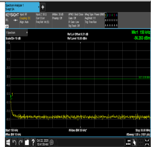
Band66-20MHz-16QAM-132322-1RB#99-0.15~30-PASS
