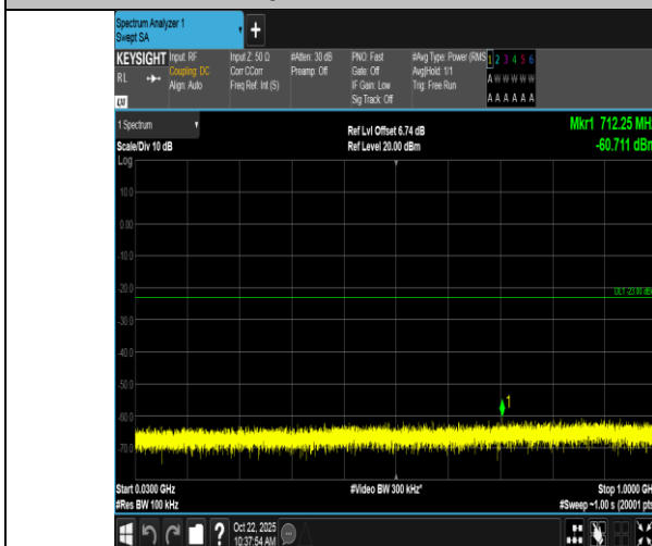
Band66-20MHz-16QAM-132072-1RB#99-30~1000-PASS
