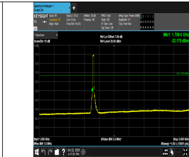
Band66-20MHz-QPSK-132072-100RB#0-1000~3000-PASS
