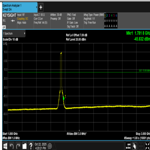
Band66-20MHz-16QAM-132322-100RB#0-1000~3000-PASS
