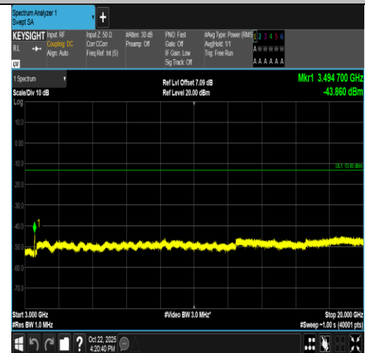
Band66-20MHz-16QAM-132322-100RB#0-3000~20000-PASS
