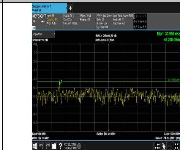
Band66-20MHz-QPSK-132072-1RB#99-0.009~0.15-PASS
