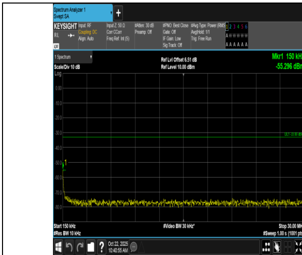
Band66-20MHz-QPSK-132322-1RB#99-0.15~30-PASS
