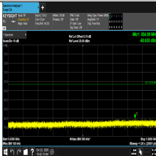
Band66-20MHz-16QAM-132322-1RB#99-30~1000-PASS
