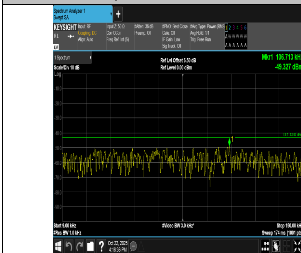
Band66-20MHz-QPSK-132322-100RB#0-0.009~0.15-PASS
