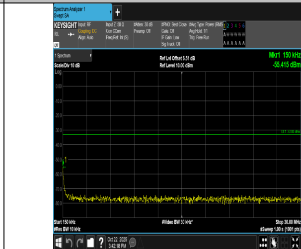
Band66-15MHz-QPSK-132597-75RB#0-0.15~30-PASS
