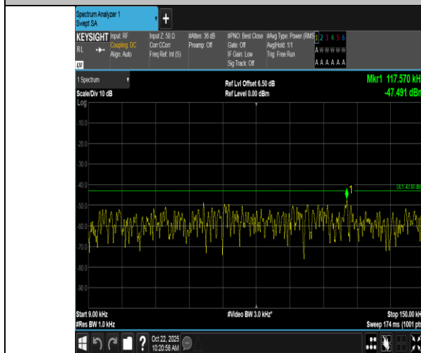
Band66-15MHz-16QAM-132597-1RB#74-0.009~0.15-PASS
