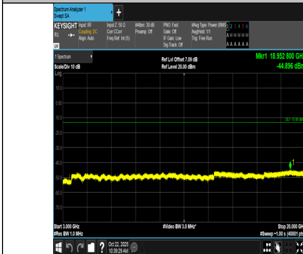
Band66-20MHz-QPSK-132322-1RB#0-3000~20000-PASS
