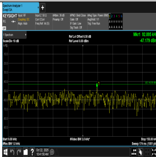
Band66-20MHz-16QAM-132322-1RB#99-0.009~0.15-PASS
