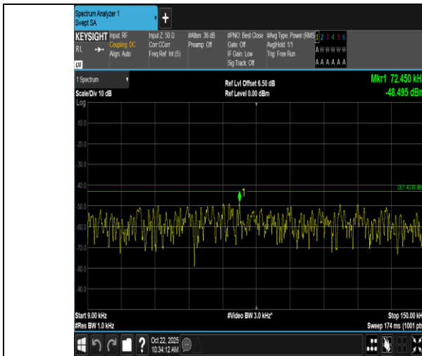
Band66-20MHz-QPSK-132072-1RB#0-0.009~0.15-PASS
