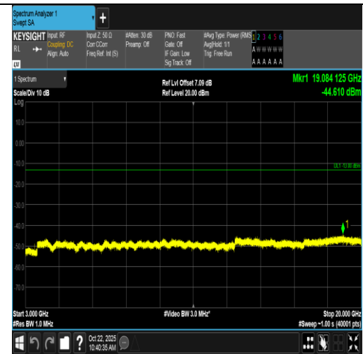
Band66-20MHz-16QAM-132322-1RB#0-3000~20000-PASS
