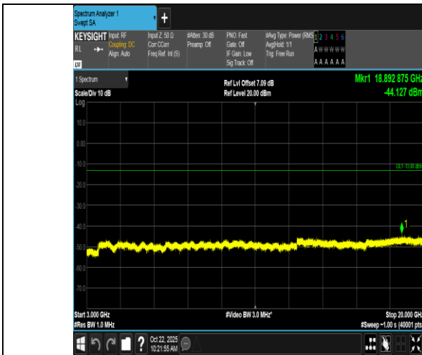
Band66-15MHz-16QAM-132597-1RB#74-3000~20000-PASS
