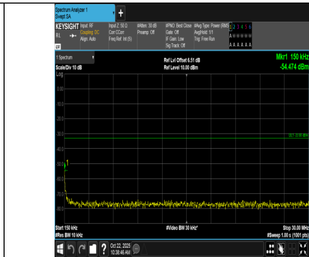
Band66-20MHz-QPSK-132322-1RB#0-0.15~30-PASS
