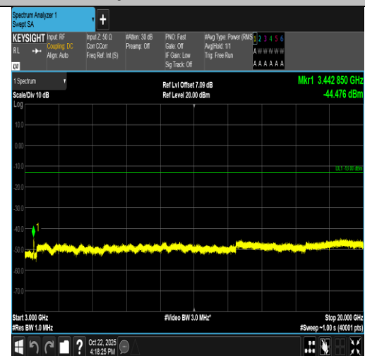
Band66-20MHz-16QAM-132072-100RB#0-3000~20000-PASS
