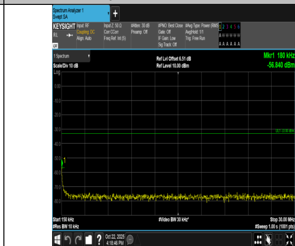
Band66-20MHz-QPSK-132322-100RB#0-0.15~30-PASS
