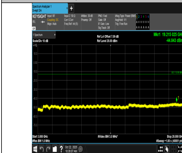
Band66-20MHz-QPSK-132072-1RB#0-3000~20000-PASS
