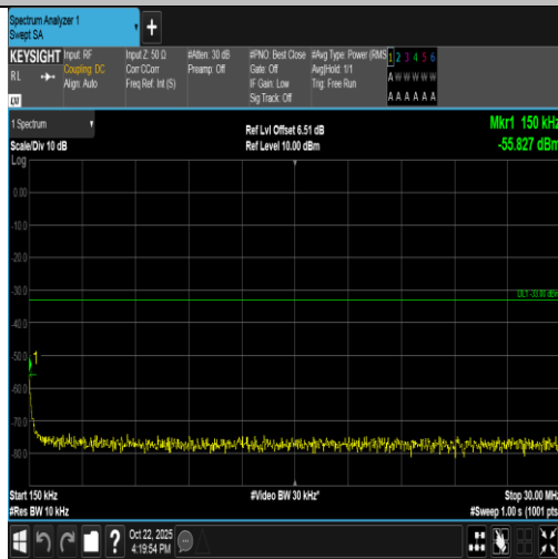
Band66-20MHz-16QAM-132322-100RB#0-0.15~30-PASS
