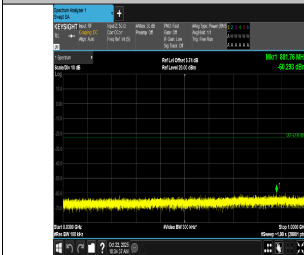
Band66-20MHz-QPSK-132072-1RB#0-30~1000-PASS
