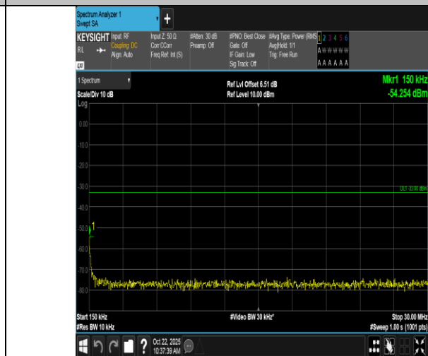
Band66-20MHz-16QAM-132072-1RB#99-0.15~30-PASS
