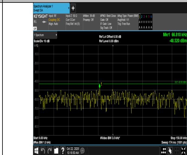
Band66-15MHz-16QAM-132597-1RB#0-0.009~0.15-PASS
