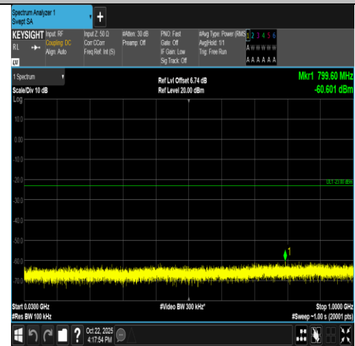
Band66-20MHz-16QAM-132072-100RB#0-30~1000-PASS
