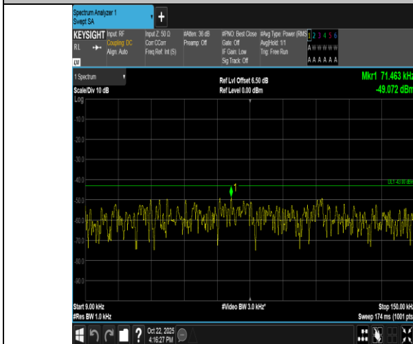
Band66-20MHz-QPSK-132072-100RB#0-0.009~0.15-PASS
