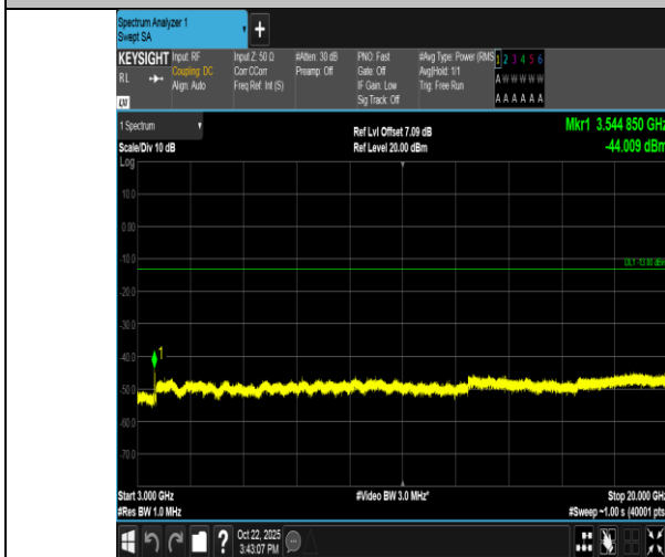
Band66-15MHz-QPSK-132597-75RB#0-3000~20000-PASS
