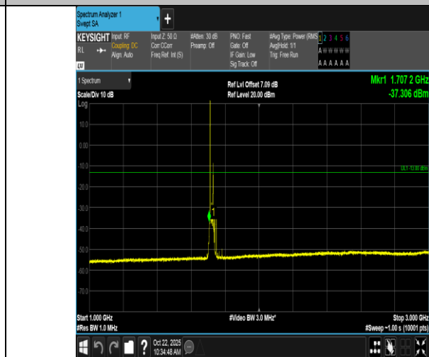
Band66-20MHz-QPSK-132072-1RB#0-1000~3000-PASS
