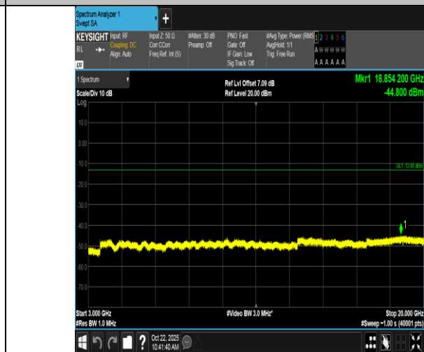
Band66-20MHz-QPSK-132322-1RB#99-3000~20000-PASS
