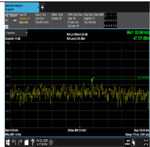
Band66-20MHz-16QAM-132072-100RB#0-0.009~0.15-PASS
