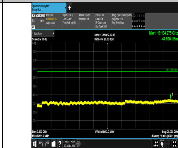
Band66-20MHz-QPSK-132572-1RB#99-3000~20000-PASS
