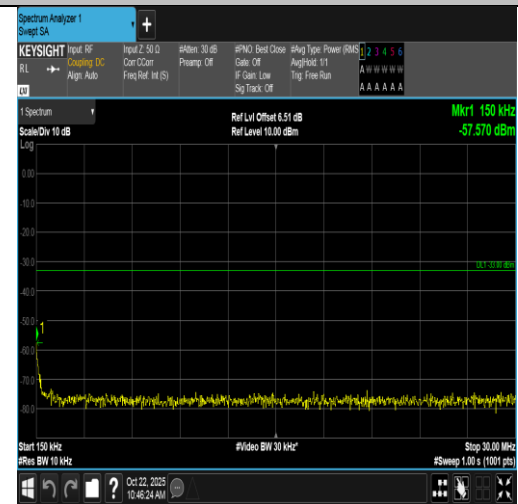
Band66-20MHz-16QAM-132572-1RB#99-0.15~30-PASS
