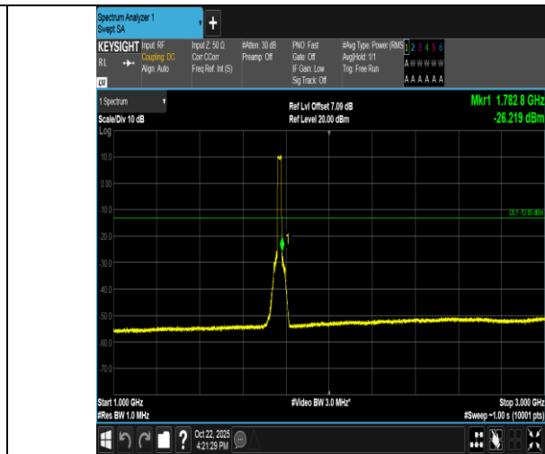
Band66-20MHz-QPSK-132572-100RB#0-1000~3000-PASS
