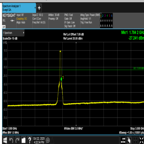
Band66-20MHz-16QAM-132572-100RB#0-1000~3000-PASS
