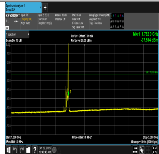
Band66-20MHz-16QAM-132572-1RB#99-1000~3000-PASS
