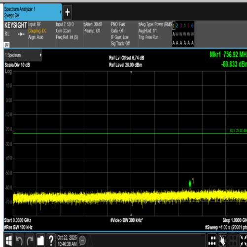
Band66-20MHz-16QAM-132572-1RB#99-30~1000-PASS
