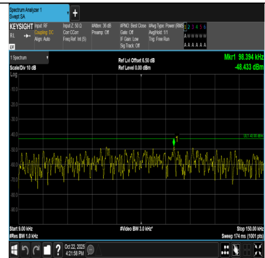
Band66-20MHz-16QAM-132572-100RB#0-0.009~0.15-PASS
