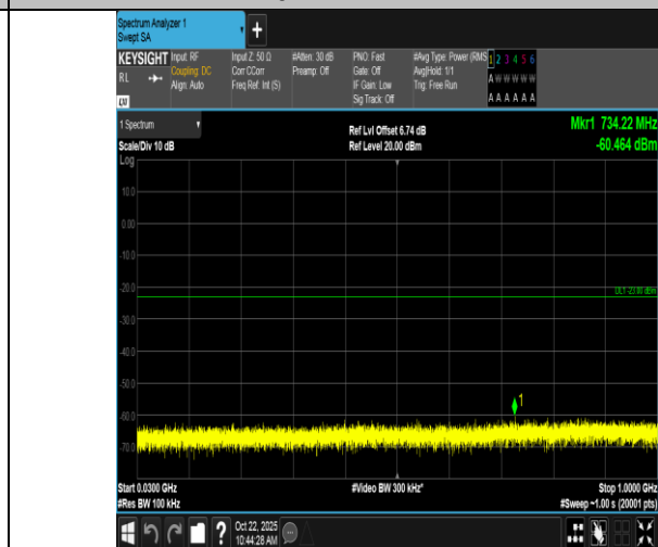
Band66-20MHz-16QAM-132572-1RB#0-30~1000-PASS
