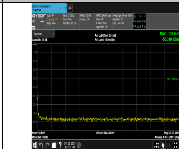
Band66-20MHz-QPSK-132572-100RB#0-0.15~30-PASS
