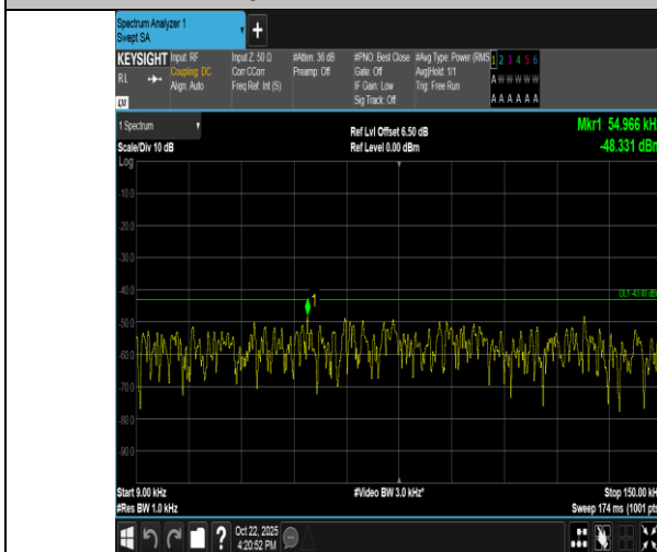
Band66-20MHz-QPSK-132572-100RB#0-0.009~0.15-PASS
