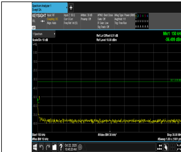
Band66-20MHz-QPSK-132572-1RB#99-0.15~30-PASS
