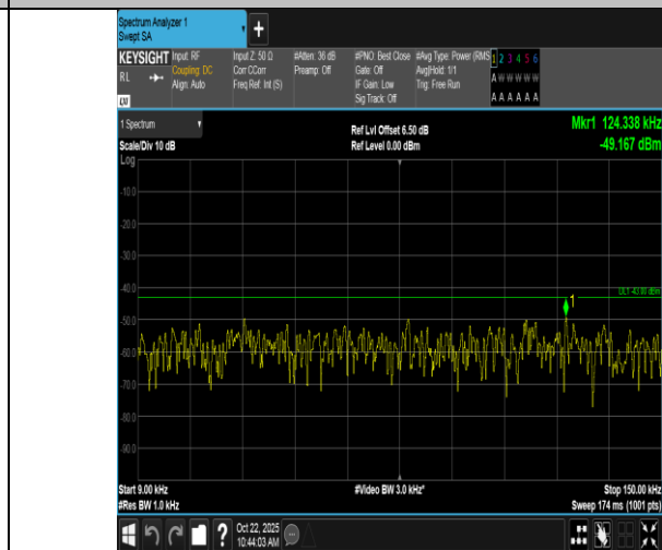
Band66-20MHz-16QAM-132572-1RB#0-0.009~0.15-PASS
