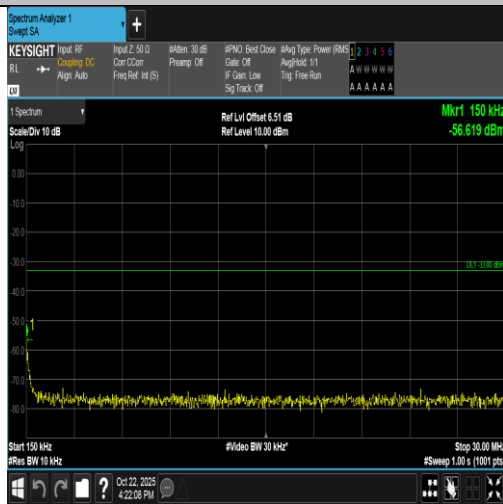
Band66-20MHz-16QAM-132572-100RB#0-0.15~30-PASS
