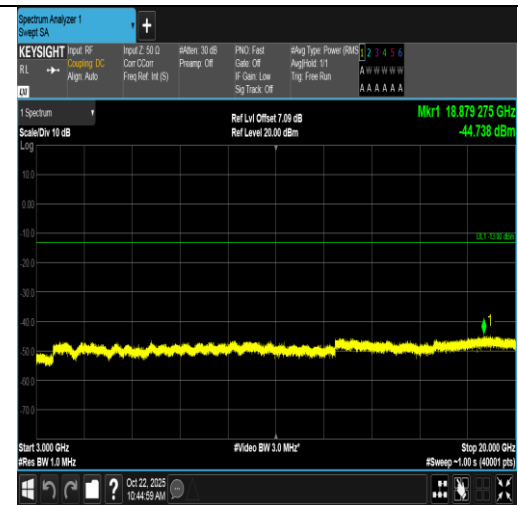
Band66-20MHz-16QAM-132572-1RB#0-3000~20000-PASS
