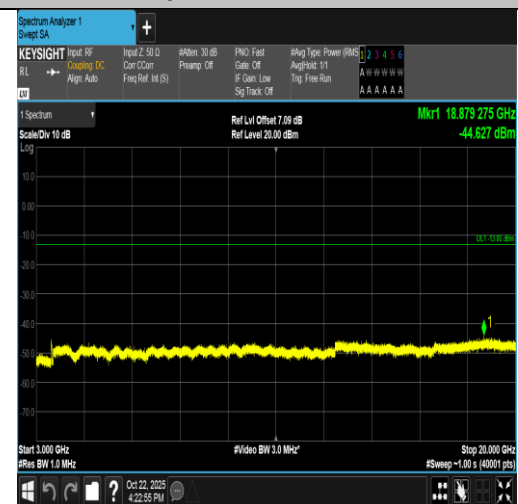
Band66-20MHz-16QAM-132572-100RB#0-3000~20000-PASS
