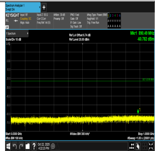
Band66-20MHz-16QAM-132572-100RB#0-30~1000-PASS
