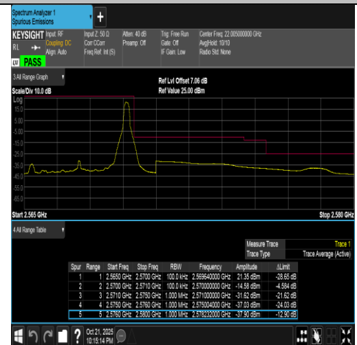
Band7-5MHz-QPSK-21425-1RB#24-PASS
