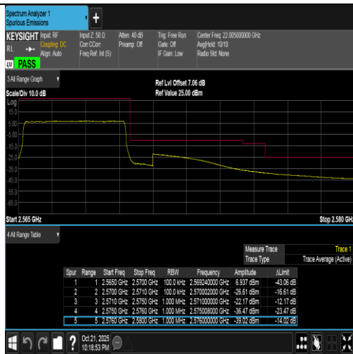
Band7-5MHz-QPSK-21425-25RB#0-PASS
