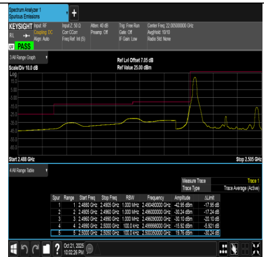
Band7-5MHz-16QAM-20775-1RB#0-PASS
