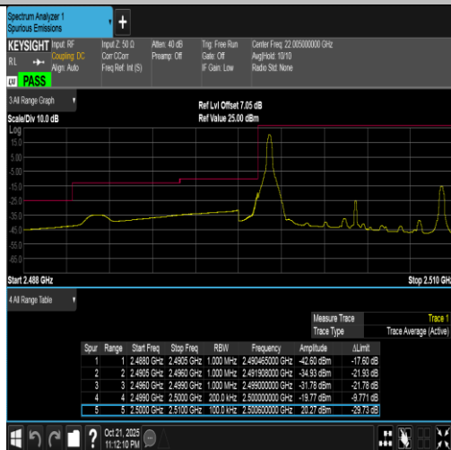
Band7-10MHz-QPSK-20800-1RB#0-PASS
