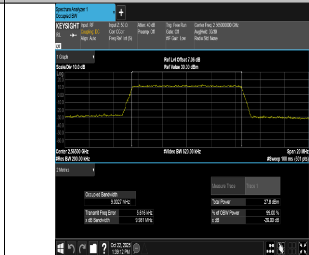
Band7-10MHz-16QAM-21400-50RB#0-PASS
