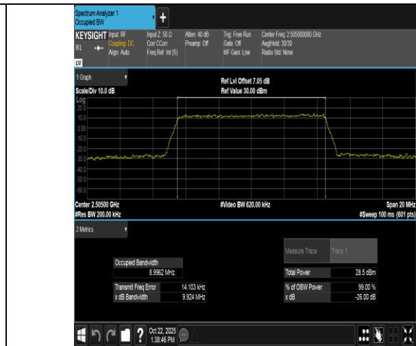
Band7-10MHz-16QAM-20800-50RB#0-PASS
