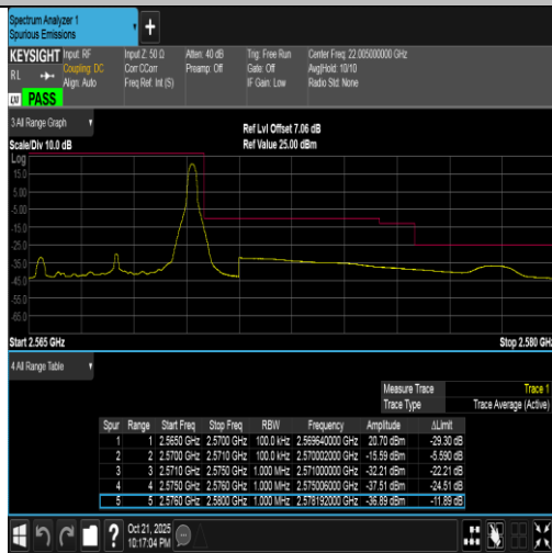
Band7-5MHz-16QAM-21425-1RB#24-PASS
