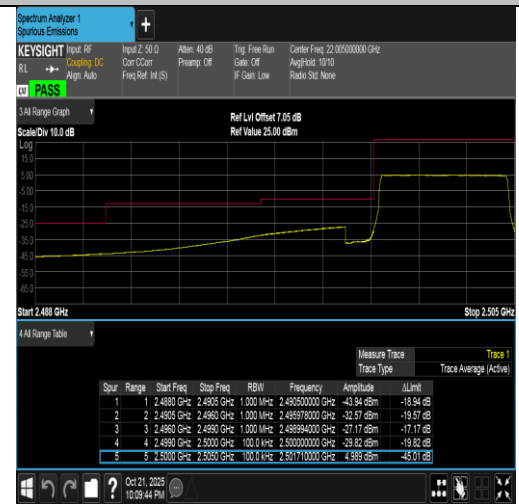
Band7-5MHz-16QAM-20775-25RB#0-PASS
