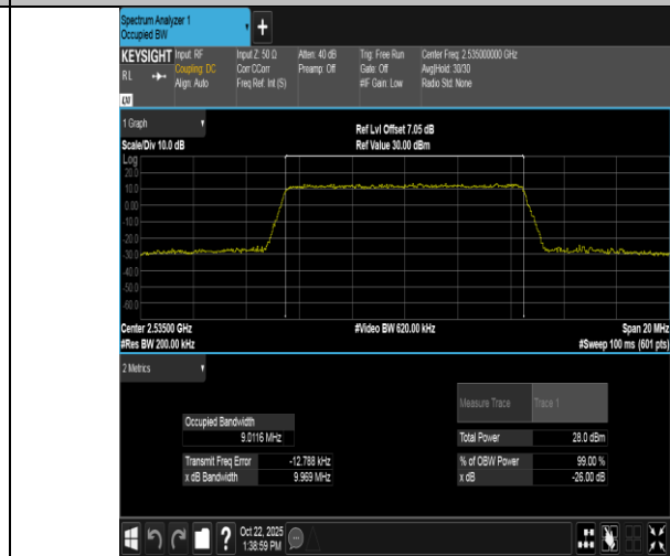
Band7-10MHz-16QAM-21100-50RB#0-PASS
