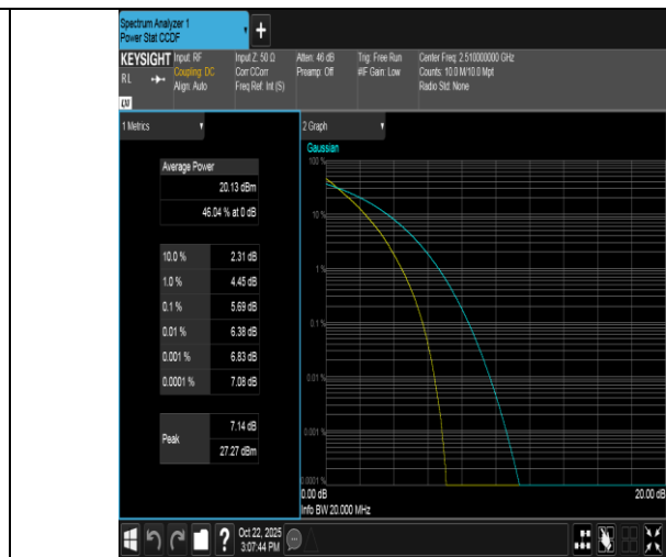
Band7-20MHz-QPSK-20850-100RB#0-PASS
