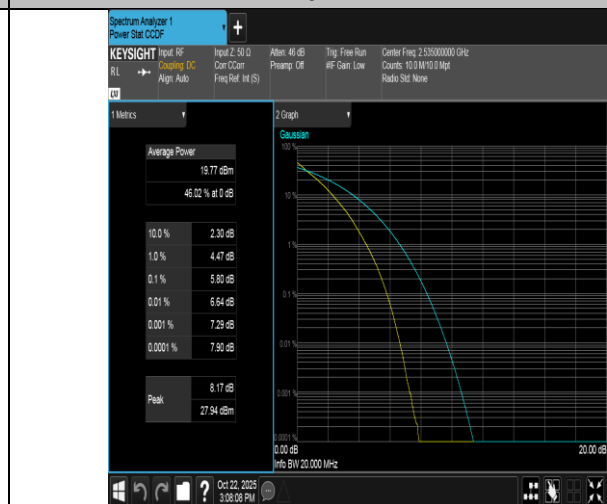
Band7-20MHz-QPSK-21100-100RB#0-PASS
