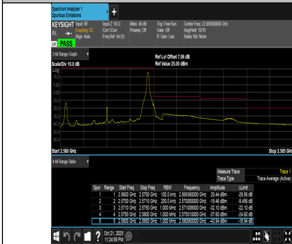
Band7-10MHz-16QAM-21400-1RB#49-PASS
