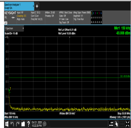
Band7-5MHz-16QAM-20775-1RB#0-0.15~30-PASS
