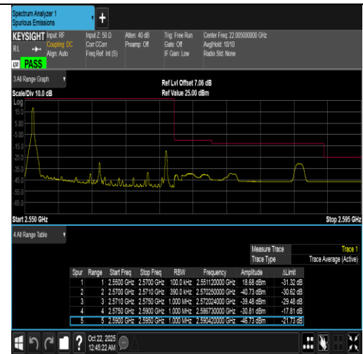
Band7-20MHz-16QAM-21350-1RB#0-PASS
