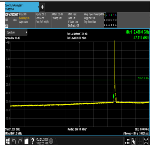
Band7-5MHz-16QAM-20775-1RB#0-1000~3000-PASS
