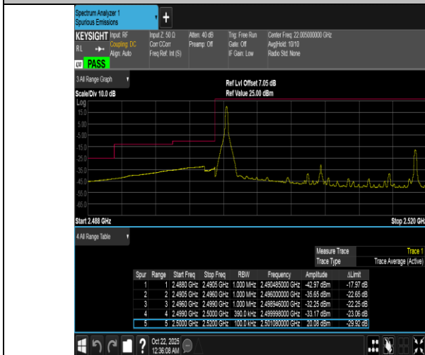
Band7-20MHz-QPSK-20850-1RB#0-PASS
