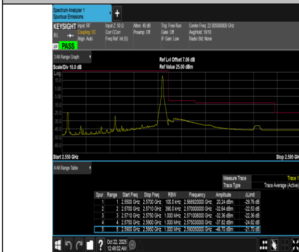
Band7-20MHz-16QAM-21350-1RB#99-PASS
