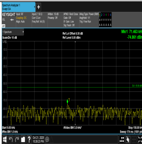
Band7-5MHz-QPSK-20775-25RB#0-0.009~0.15-PASS
