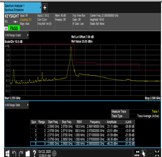
Band7-15MHz-QPSK-21375-1RB#74-PASS
