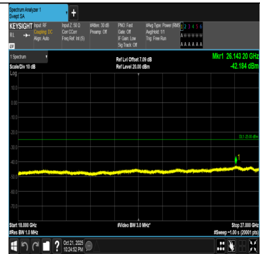
Band7-5MHz-QPSK-20775-1RB#24-18000~27000-PASS
