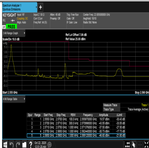
Band7-15MHz-QPSK-21375-1RB#0-PASS
