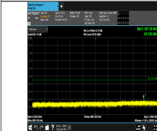
Band7-5MHz-16QAM-20775-1RB#0-30~1000-PASS
