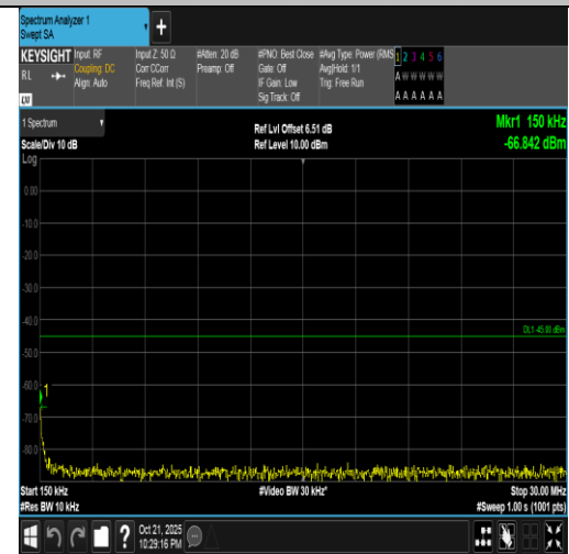
Band7-5MHz-QPSK-21100-1RB#0-0.15~30-PASS
