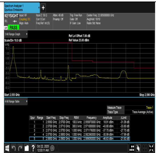
Band7-15MHz-16QAM-21375-1RB#0-PASS
