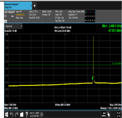
Band7-5MHz-QPSK-20775-25RB#0-1000~3000-PASS
