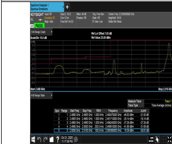
Band7-10MHz-16QAM-20800-1RB#49-PASS
