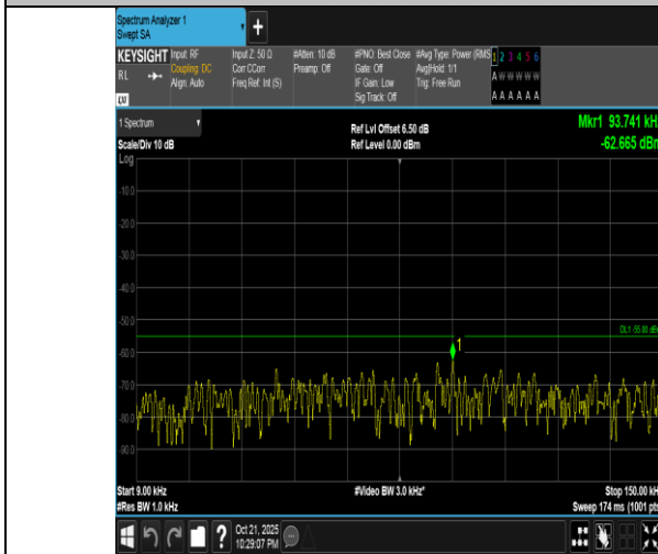
Band7-5MHz-QPSK-21100-1RB#0-0.009~0.15-PASS
