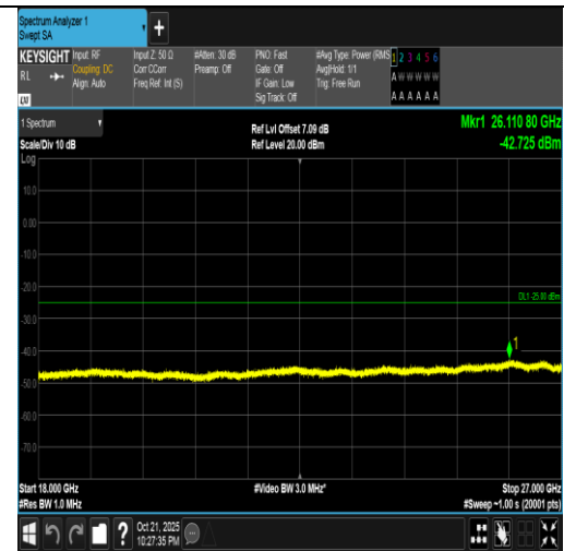
Band7-5MHz-QPSK-20775-25RB#0-18000~27000-PASS
