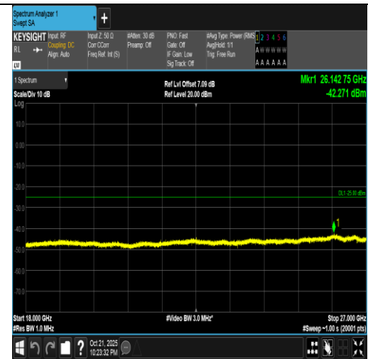
Band7-5MHz-16QAM-20775-1RB#0-18000~27000-PASS
