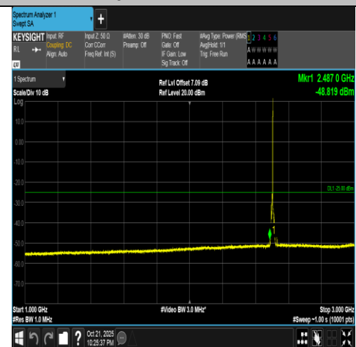
Band7-5MHz-16QAM-20775-1RB#24-1000~3000-PASS
