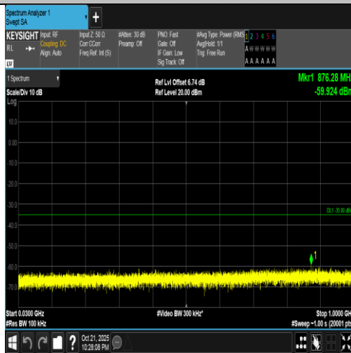
Band7-5MHz-16QAM-20775-25RB#0-30~1000-PASS
