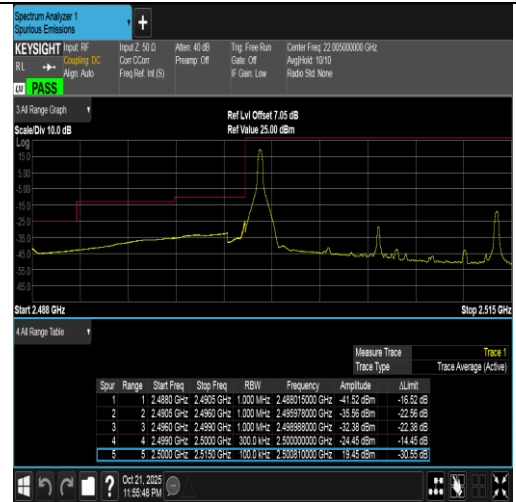
Band7-15MHz-16QAM-20825-1RB#0-PASS
