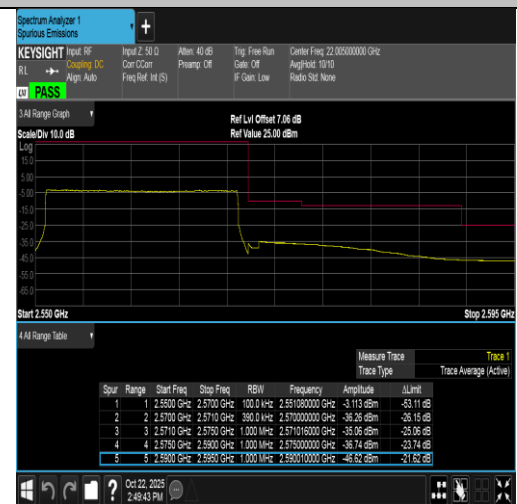
Band7-20MHz-16QAM-21350-100RB#0-PASS
