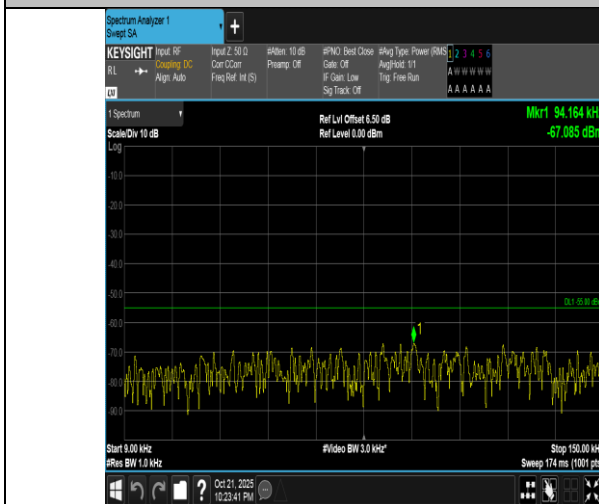
Band7-5MHz-QPSK-20775-1RB#24-0.009~0.15-PASS
