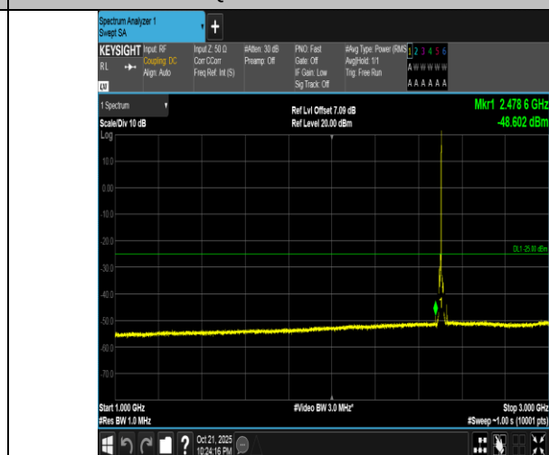
Band7-5MHz-QPSK-20775-1RB#24-1000~3000-PASS
