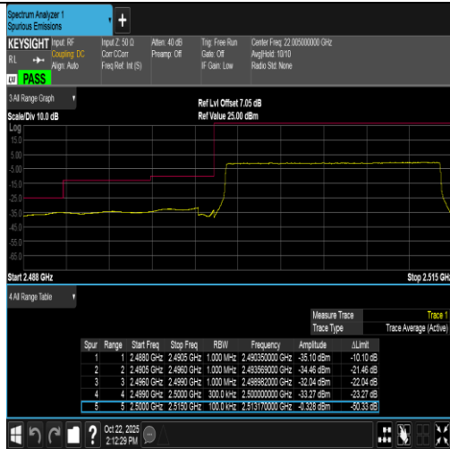
Band7-15MHz-QPSK-20825-75RB#0-PASS
