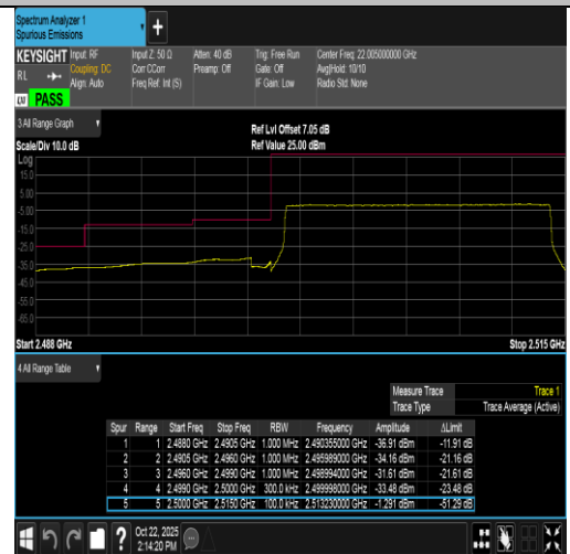
Band7-15MHz-16QAM-20825-75RB#0-PASS
