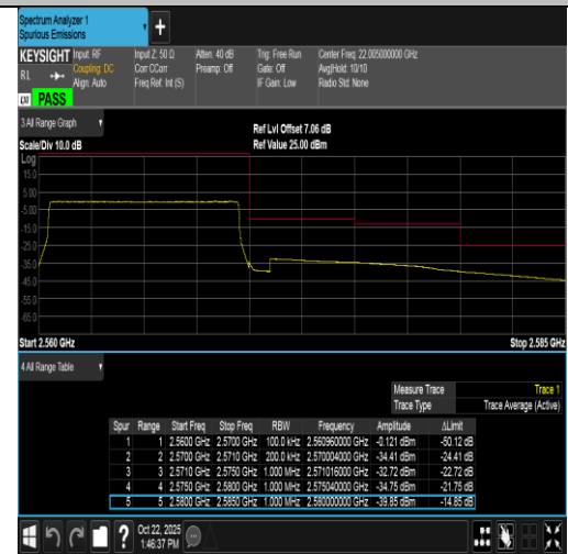
Band7-10MHz-16QAM-21400-50RB#0-PASS
