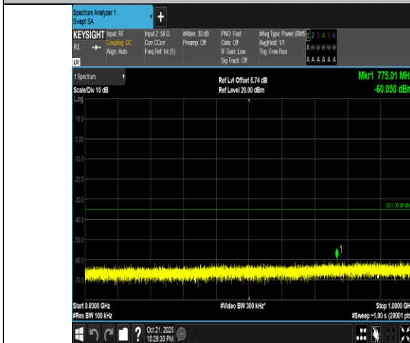
Band7-5MHz-QPSK-21100-1RB#0-30~1000-PASS
