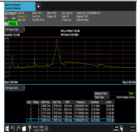
Band7-10MHz-QPSK-21400-1RB#49-PASS
