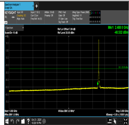
Band7-5MHz-16QAM-20775-25RB#0-1000~3000-PASS
