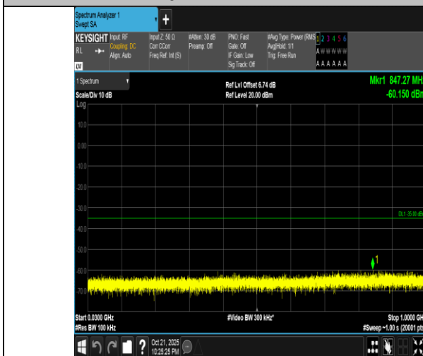
Band7-5MHz-16QAM-20775-1RB#24-30~1000-PASS
