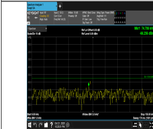
Band7-5MHz-16QAM-20775-1RB#24-0.009~0.15-PASS
