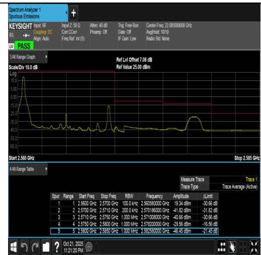
Band7-10MHz-16QAM-21400-1RB#0-PASS
