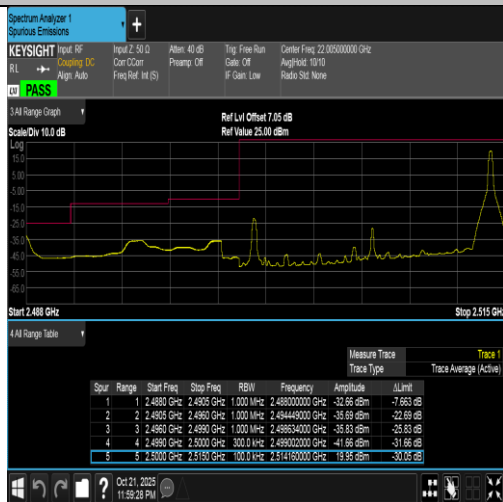
Band7-15MHz-16QAM-20825-1RB#74-PASS
