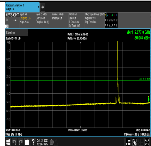
Band7-5MHz-QPSK-21100-1RB#0-1000~3000-PASS
