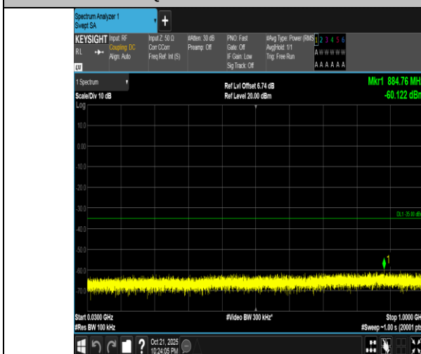
Band7-5MHz-QPSK-20775-1RB#24-30~1000-PASS
