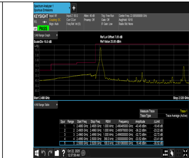
Band7-20MHz-16QAM-20850-1RB#0-PASS
