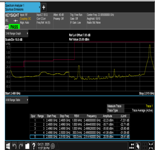
Band7-15MHz-QPSK-20825-1RB#74-PASS
