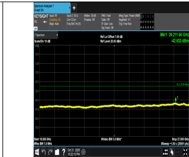
Band7-5MHz-QPSK-20775-1RB#0-18000~27000-PASS
