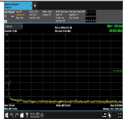
Band7-5MHz-16QAM-20775-25RB#0-0.15~30-PASS
