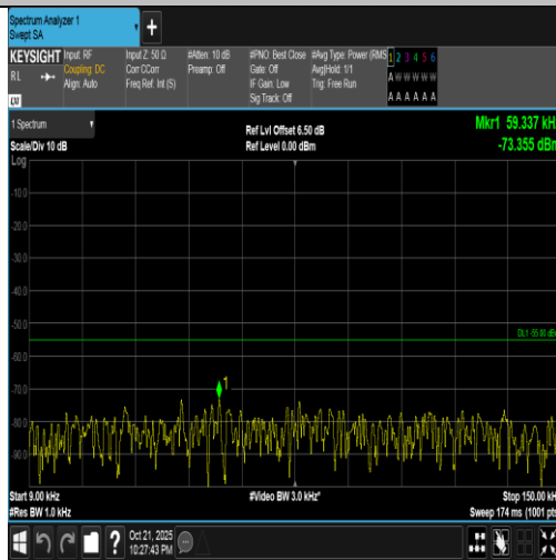
Band7-5MHz-16QAM-20775-25RB#0-0.009~0.15-PASS
