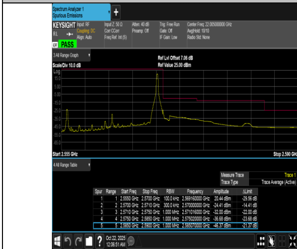
Band7-15MHz-16QAM-21375-1RB#74-PASS
