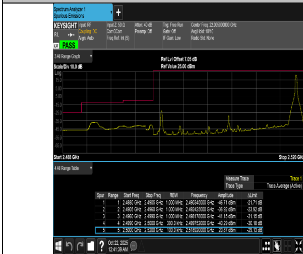
Band7-20MHz-16QAM-20850-1RB#99-PASS
