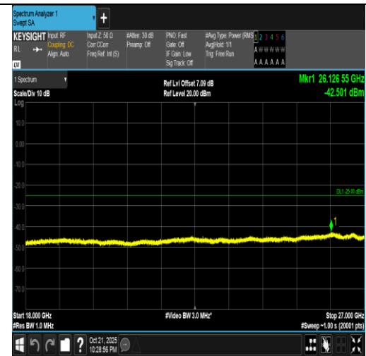
Band7-5MHz-16QAM-20775-25RB#0-18000~27000-PASS
