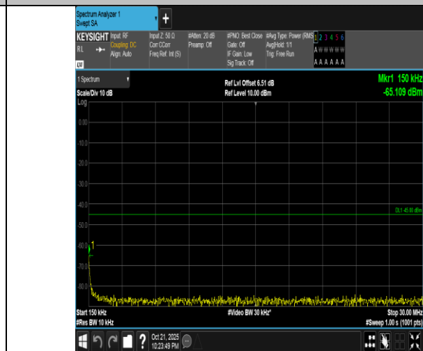
Band7-5MHz-QPSK-20775-1RB#24-0.15~30-PASS
