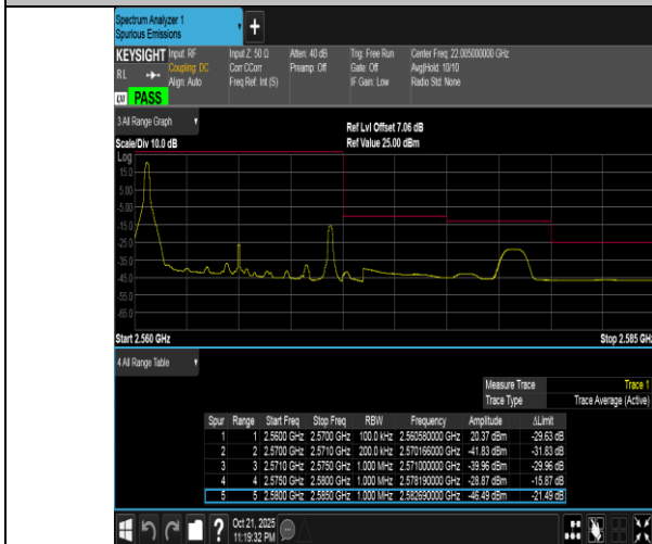
Band7-10MHz-QPSK-21400-1RB#0-PASS
