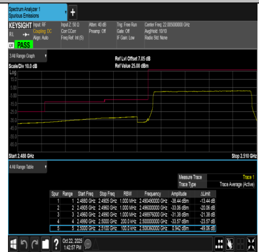
Band7-10MHz-16QAM-20800-50RB#0-PASS
