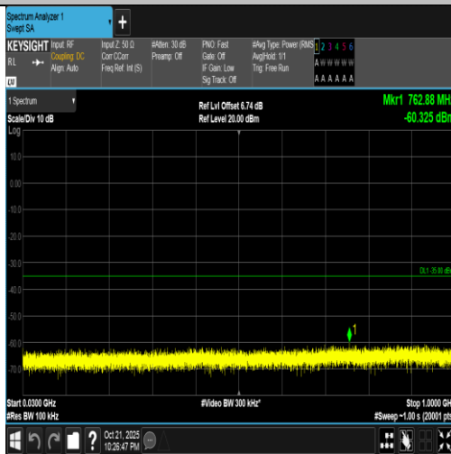
Band7-5MHz-QPSK-20775-25RB#0-30~1000-PASS
