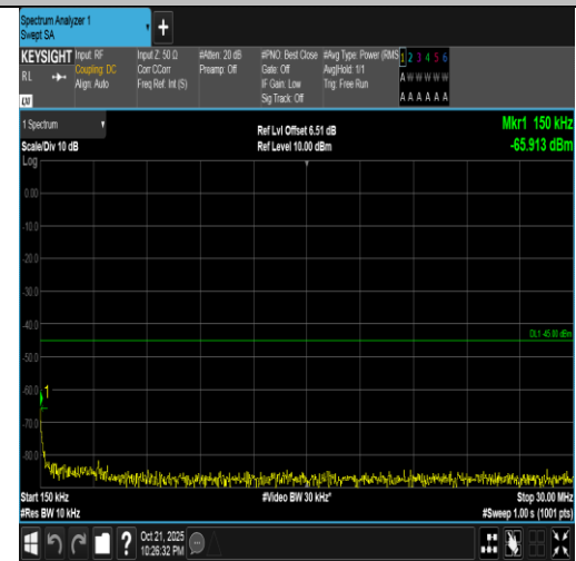
Band7-5MHz-QPSK-20775-25RB#0-0.15~30-PASS
