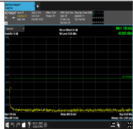
Band7-5MHz-16QAM-20775-1RB#24-0.15~30-PASS
