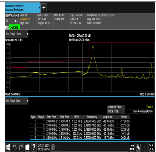
Band7-10MHz-16QAM-20800-1RB#0-PASS
