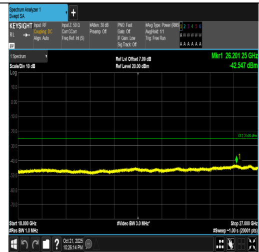
Band7-5MHz-16QAM-20775-1RB#24-18000~27000-PASS
