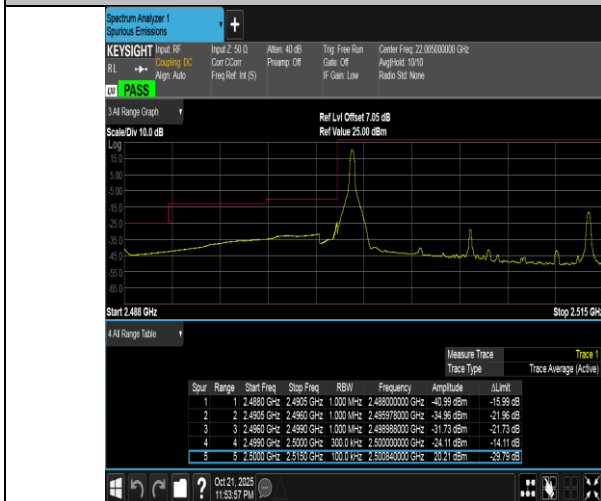
Band7-15MHz-QPSK-20825-1RB#0-PASS
